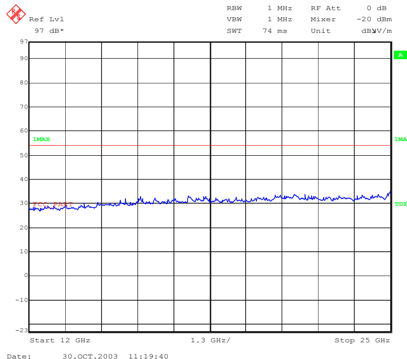
Plot 3: 12- 25 GHz (receiver)
