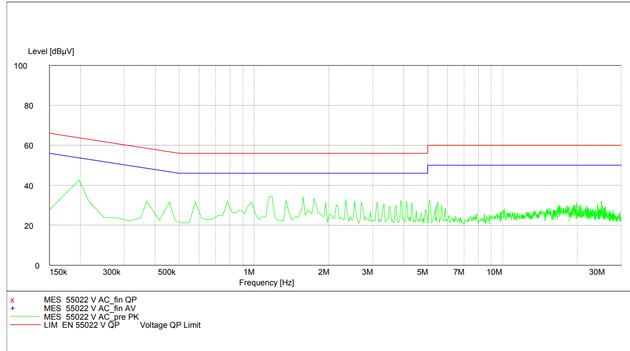
Plot 1 TX: CISPR 22
