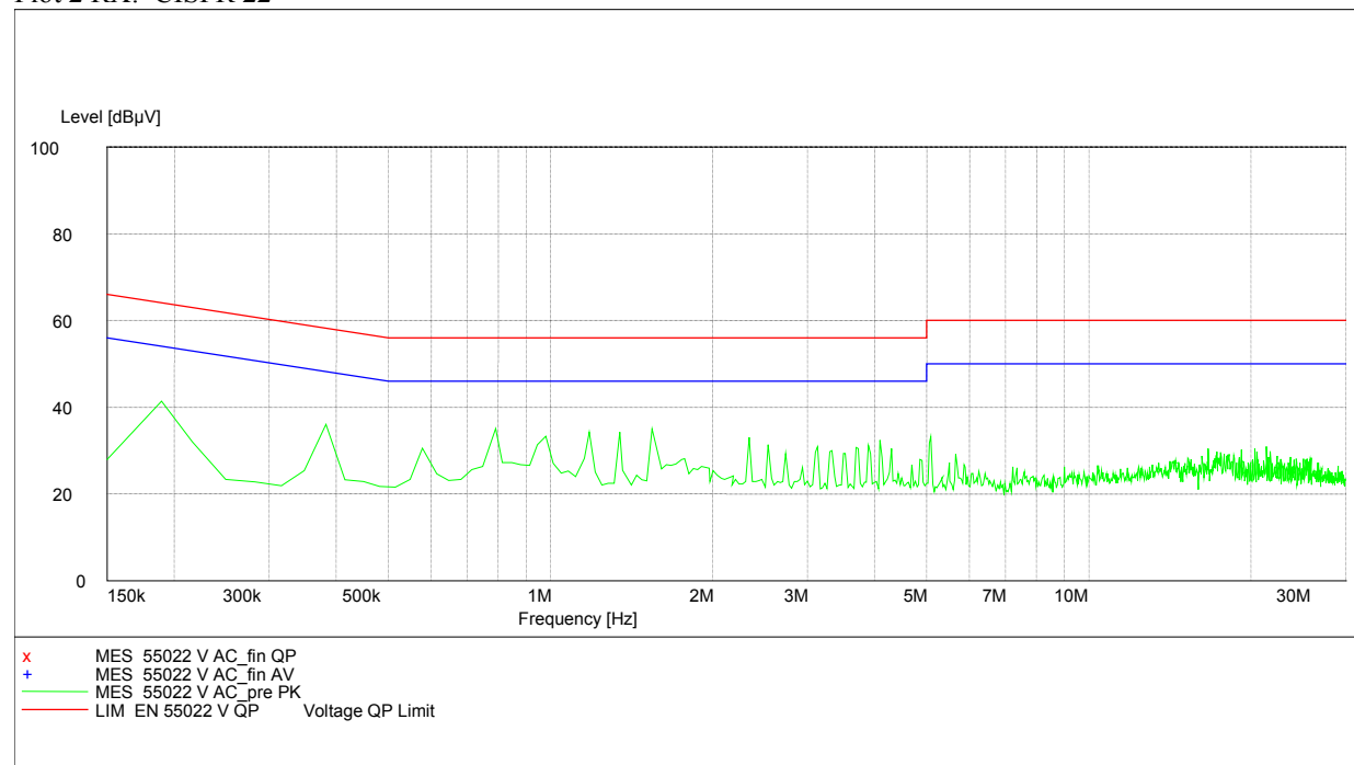
Plot 2 RX: CISPR 22
