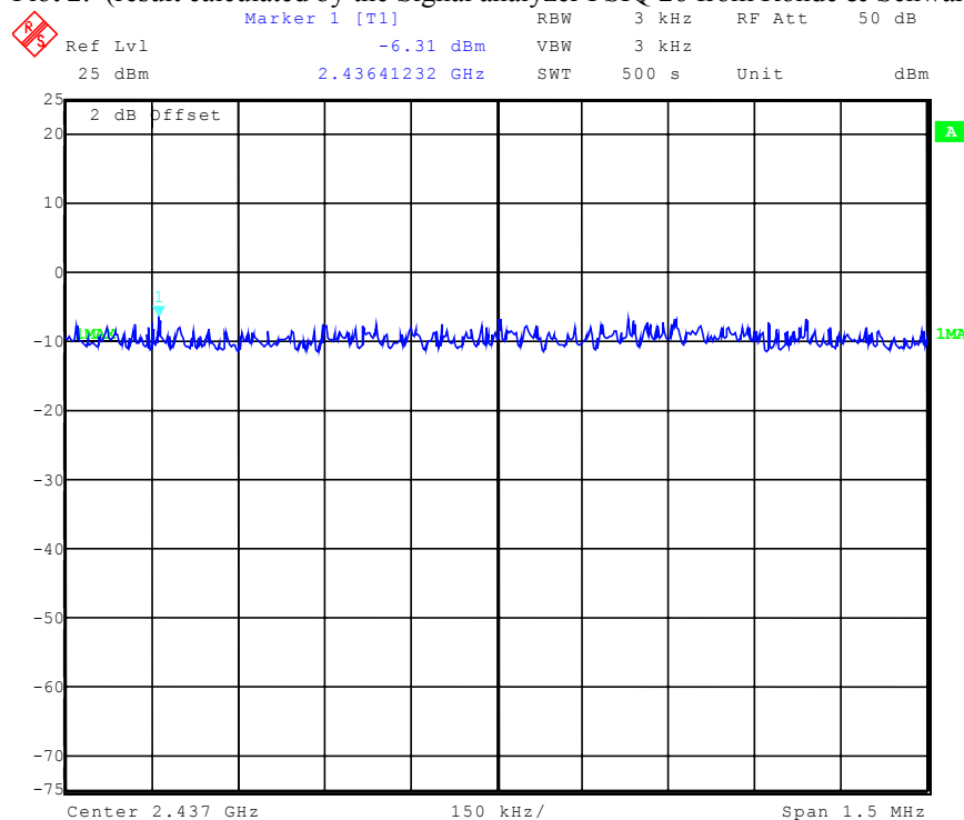
Plot 2: (result calculated by the Signal analyzer FSIQ 26 from Rohde & Schwarz)
