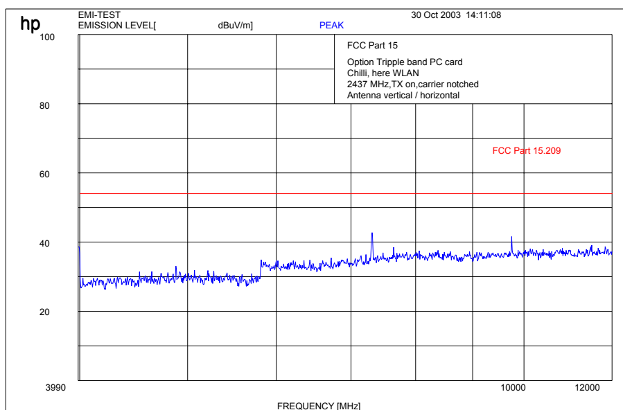
Plot 5: 4- 12 GHz (middle channel)
