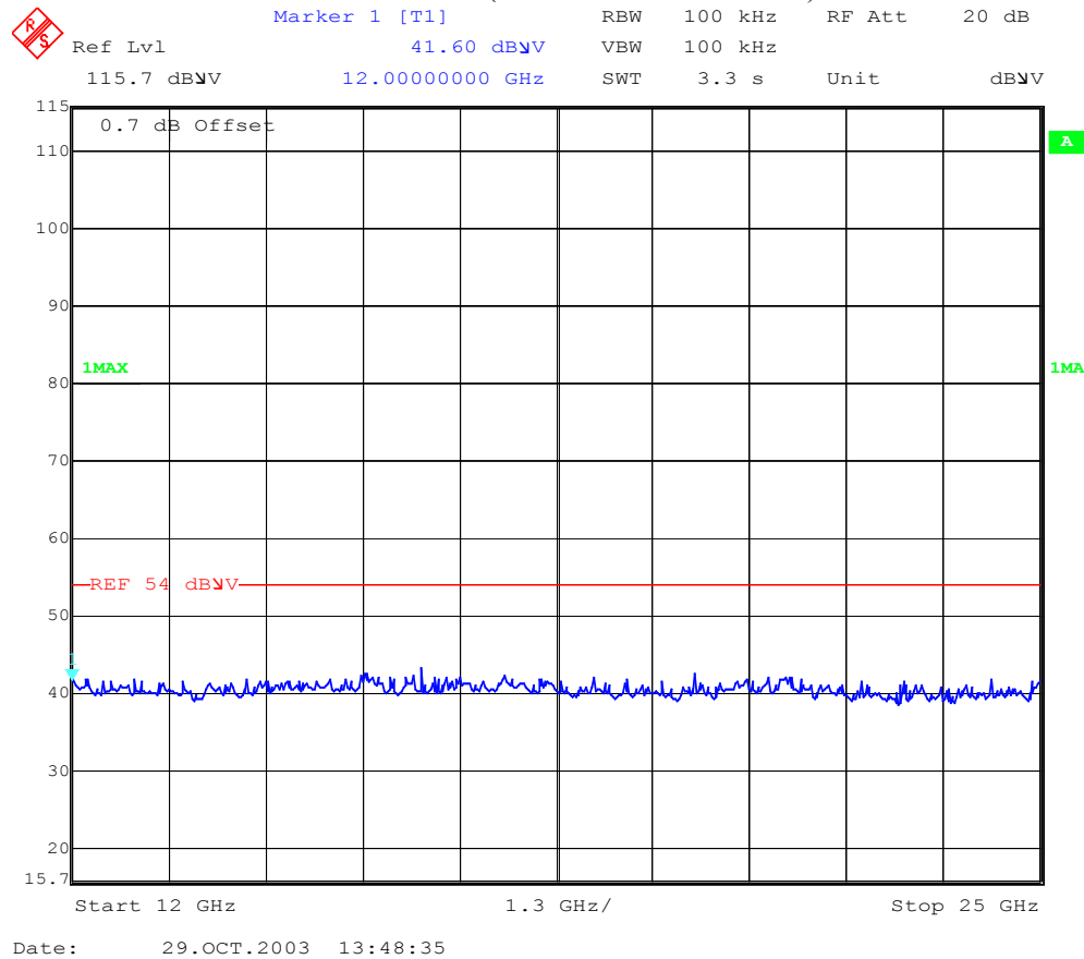
Plot 3: 12 – 25 GHz horizontal / vertical (valid for all three channels)
