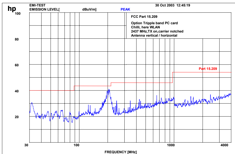
Plot 4: 0.03 - 4 GHz vertical / horizontal (middle channel)
