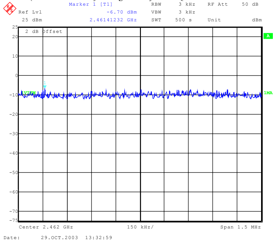
Plot 3: (result calculated by the Signal analyzer FSIQ 26 from Rohde & Schwarz)
