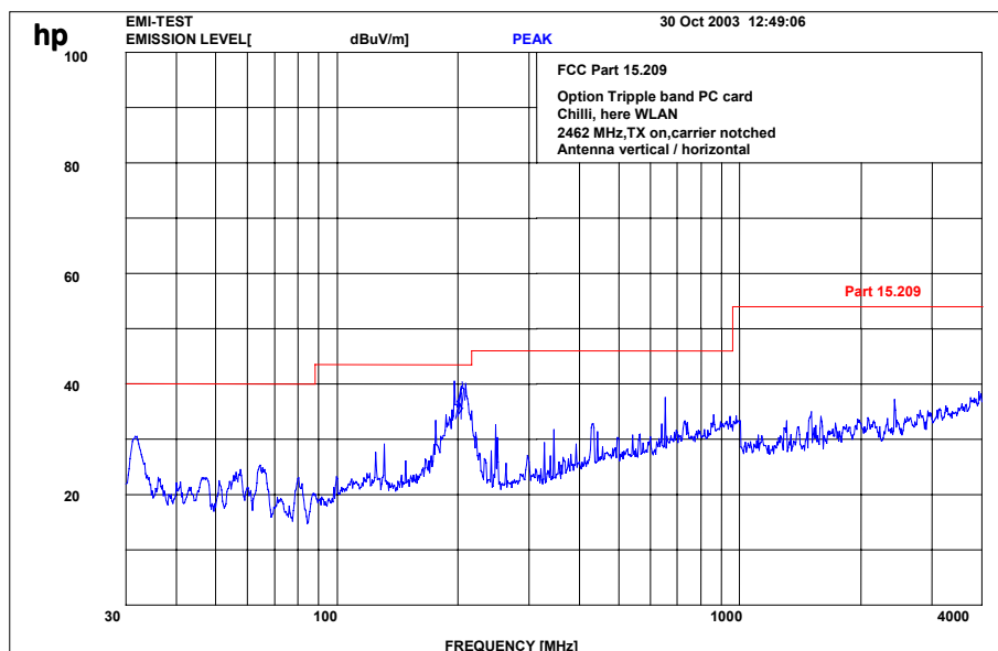
Plot 6: 0.03 - 4 GHz vertical / horizontal (highest channel)
