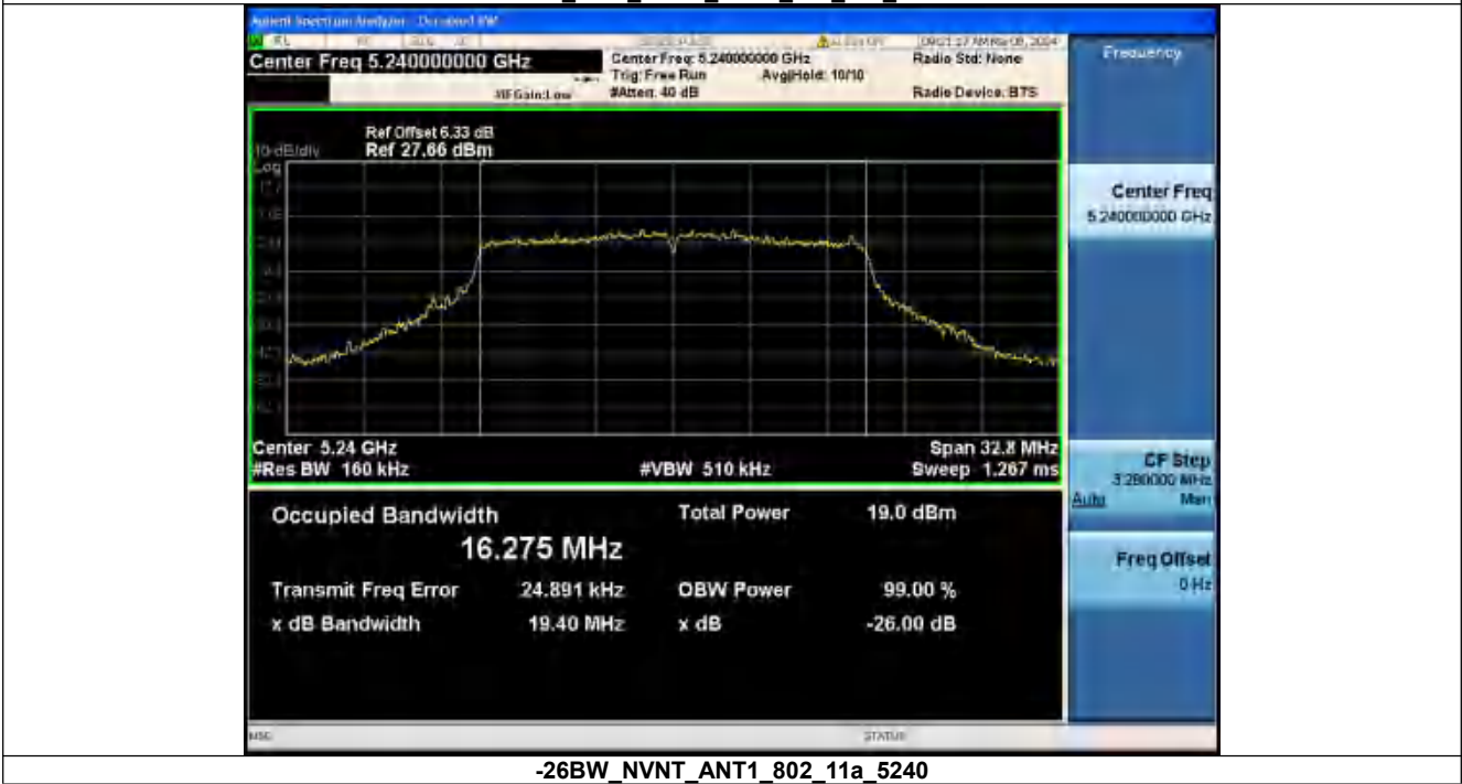
-26BW_NVNT_ANT1_802_11a_5240
