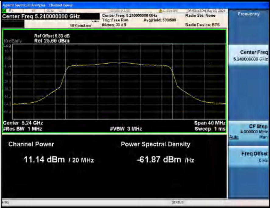
Maximum_Conducted_Output_Power_NVHT_ANT2_802_11ax(HE20)_5240_20M
