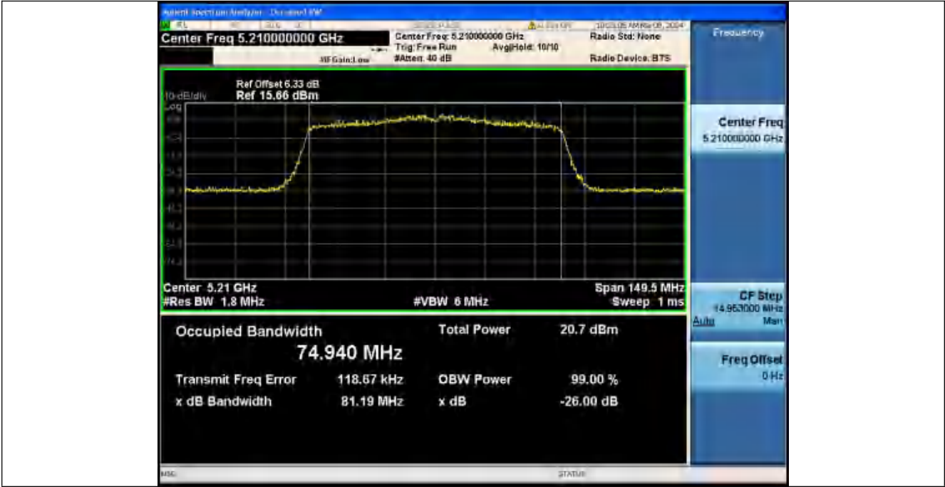
99%_OCB_NVNT_ANT1_802_11ax(HE80)_5210
