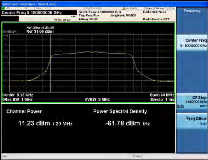
Maximum Conducted Output Power NVHT_ANT2_802_11ax(HE20)_5180_20M
