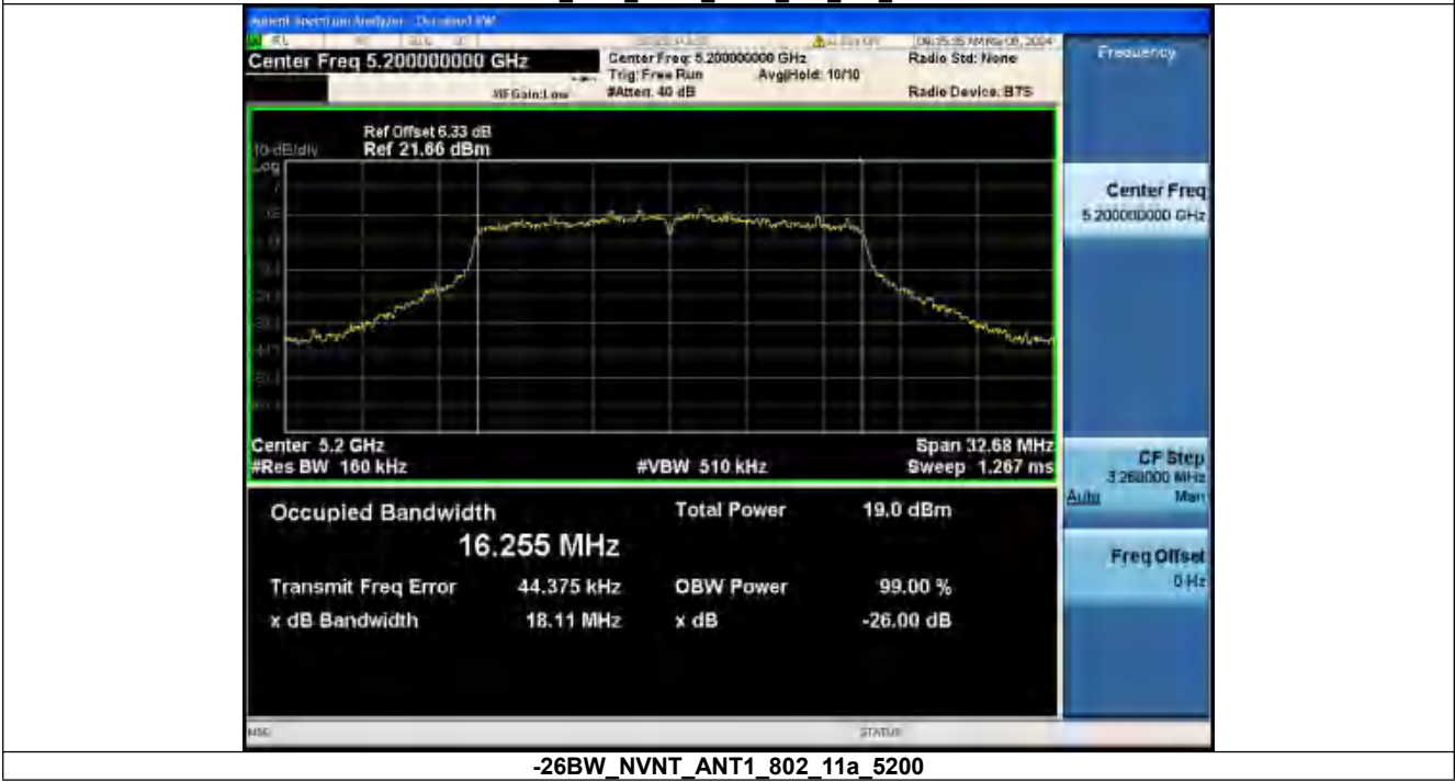
-26BW_NVNT_ANT1_802_11a_5200
