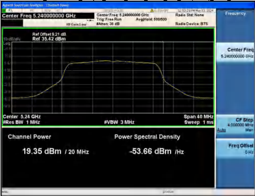
Maximum_Conducted_Output_Power_NVNT_ANT2_802_11n(HT20)_5240_20M
