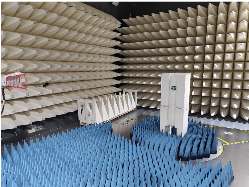
Figure B8. Radiated emission Setup – High Range 1 to 18 GHz
