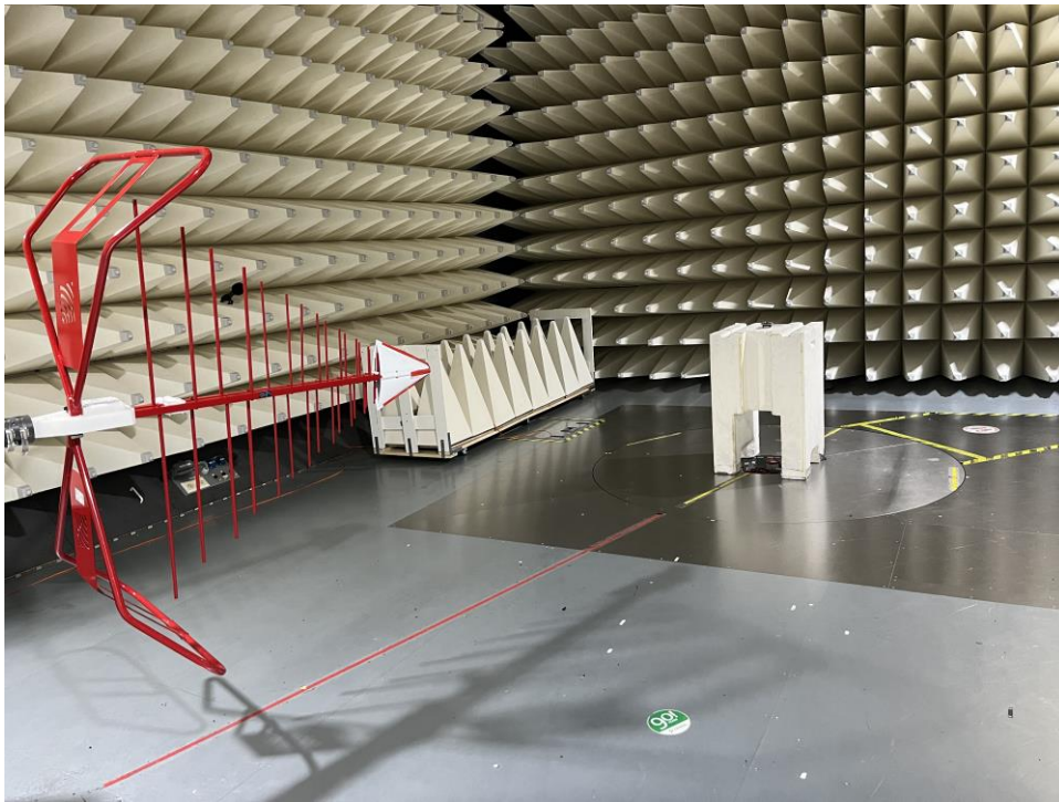
Figure B7. Radiated emission Setup – Low Range 30 to 1000MHz
