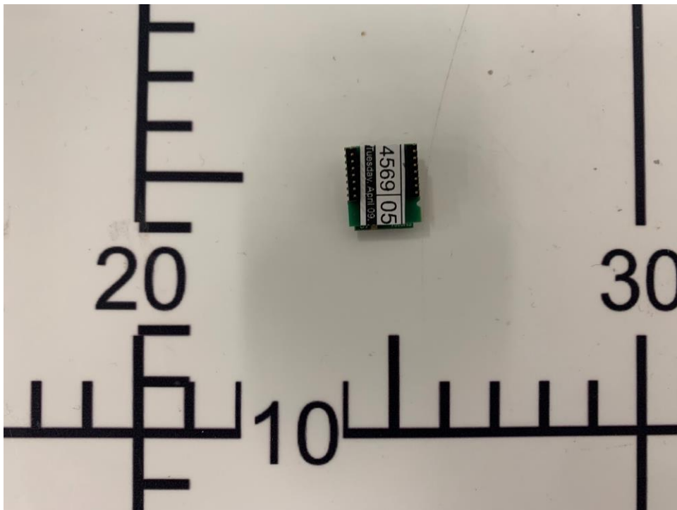
Figure B4. Bottom View of DUT (Radiated)
