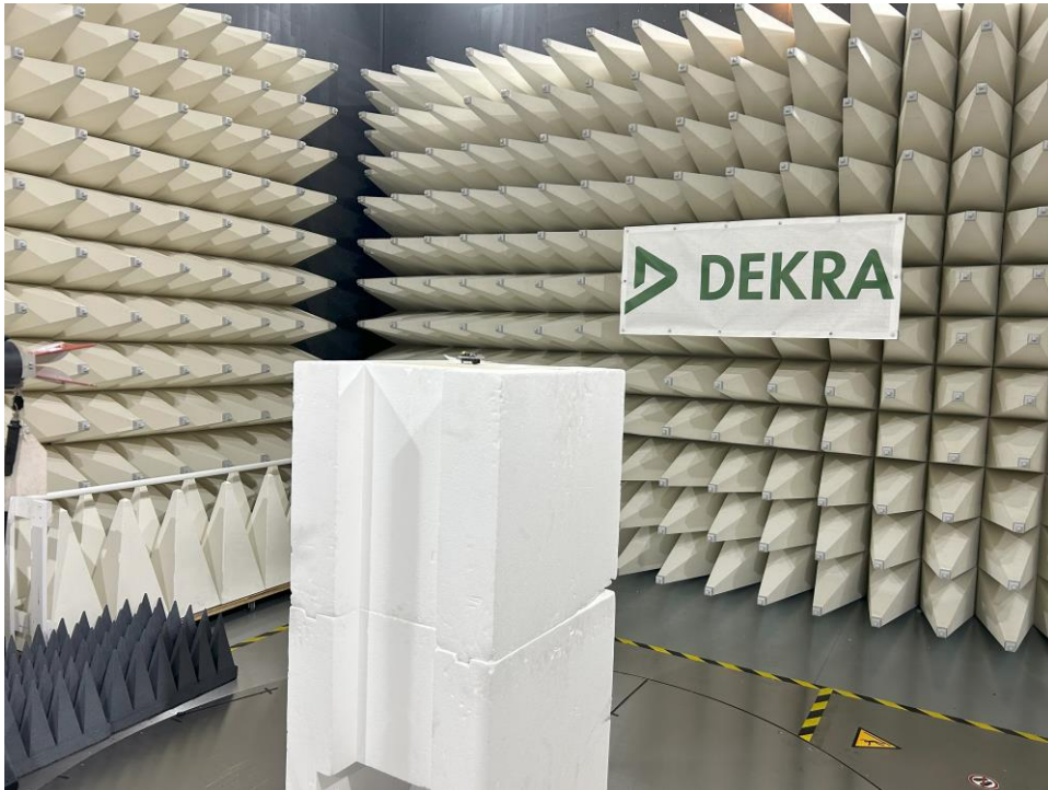
Figure B9. Radiated emission Setup – High Range 18 to 26 GHz
