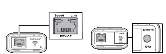
Figure 1 SA201 Ethernet port and 12V DC Power Supply
