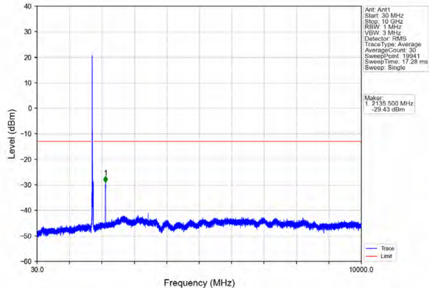
Band4_20MHz_64QAM_MCH_1732.5MHz_RB_1_0_NTNV
