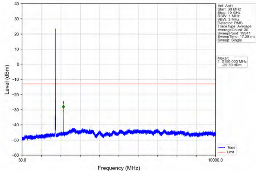
Band4_10MHz_16QAM_HCH_1750MHz_RB_1_0_NTNV
