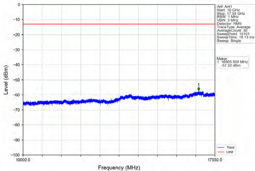
Band4_10MHz_16QAM_HCH_1750MHz_RB_1_0_NTNV
