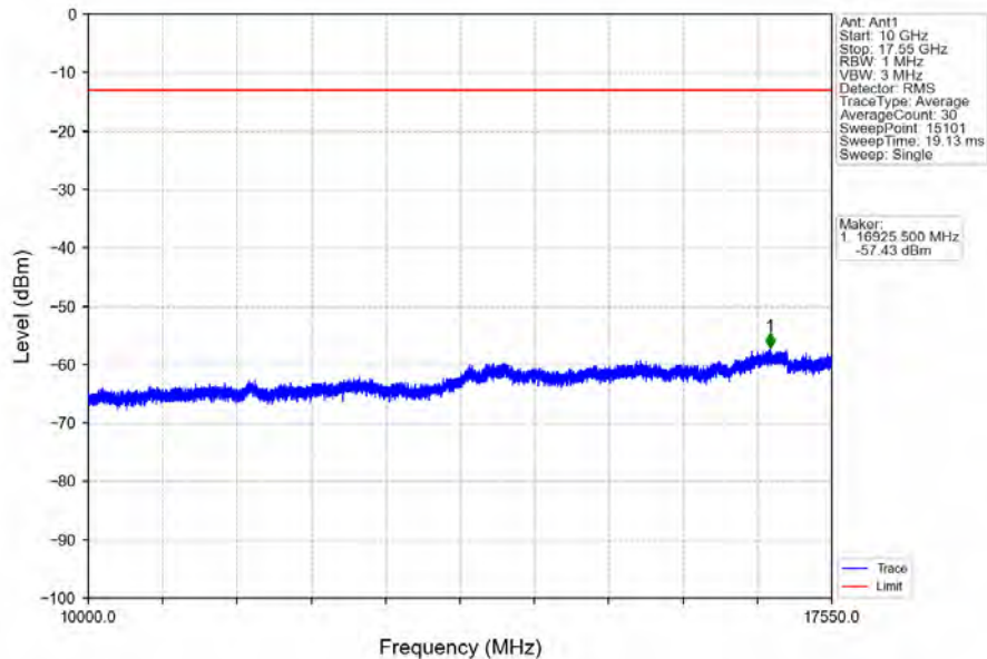
Band4_15MHz_16QAM_LCH_1717.5MHz_RB_75_0_NTNV
