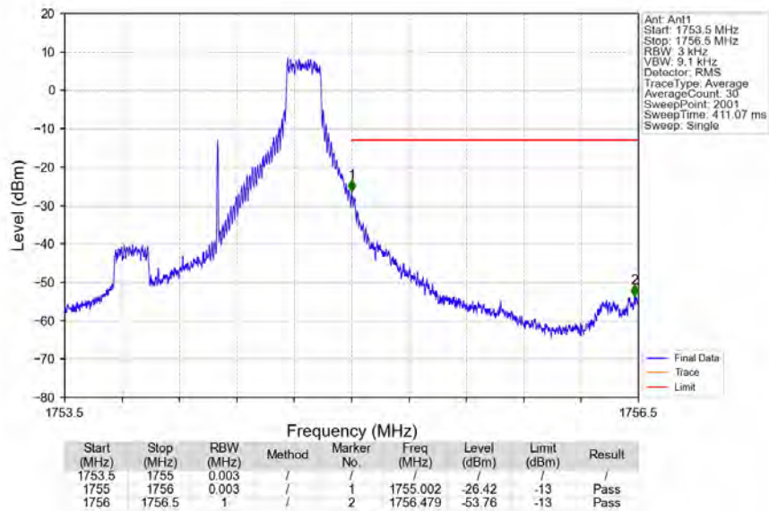
Band4_1.4MHz_QPSK_HCH_1754.3MHz_RB_1_5_NTNV
