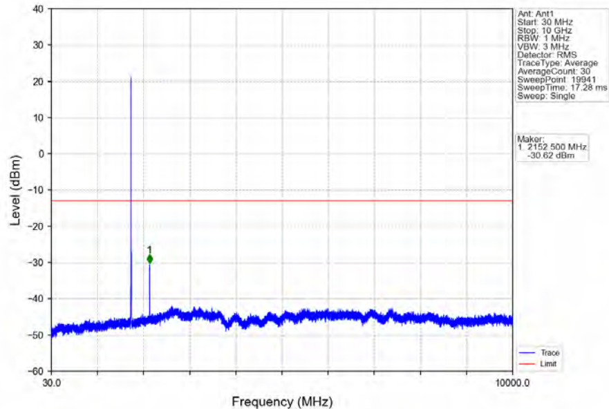
Band4_5MHz_64QAM_HCH_1752.5MHz_RB_1_0_NTNV
