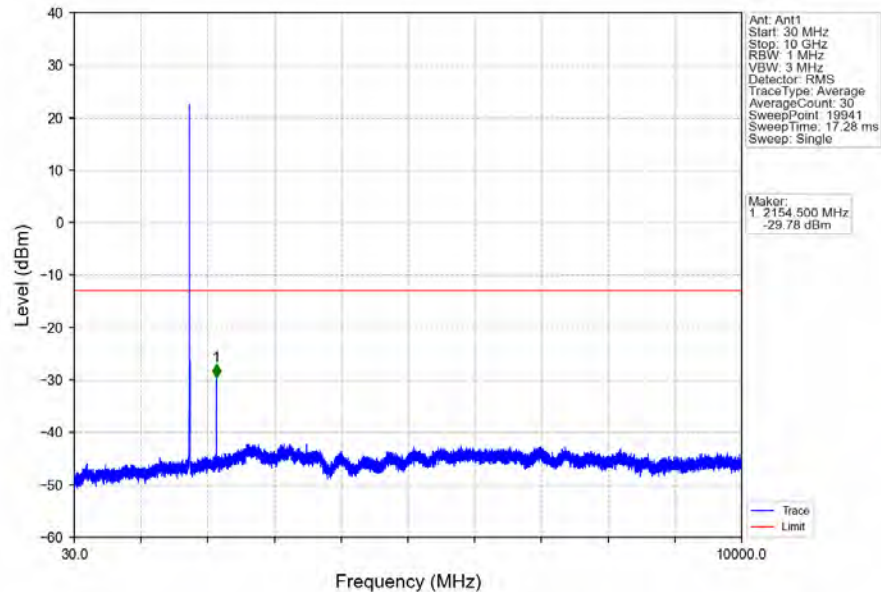
Band4_5MHz_16QAM_HCH_1752.5MHz_RB_1_0_NTNV
