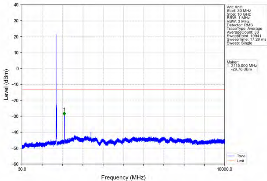
Band4_15MHz_64QAM_LCH_1717.5MHz_RB_1_0_NTNV
