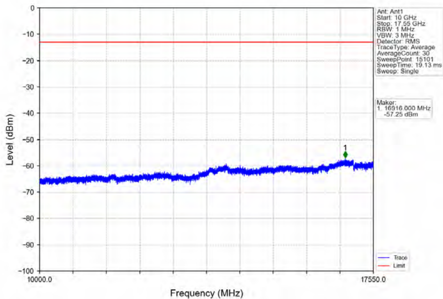
Band4_15MHz_64QAM_HCH_1747.5MHz_RB_1_0_NTNV
