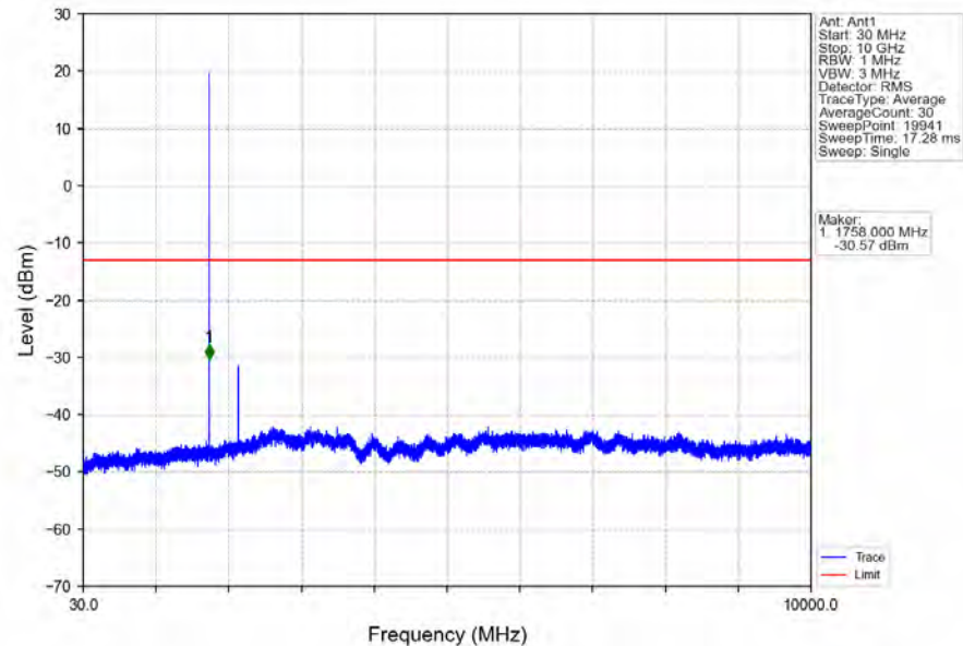
Band4_1.4MHz_64QAM_HCH_1754.3MHz_RB_1_0_NTNV
