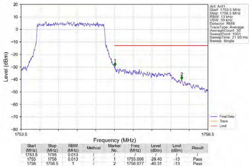
Band4_1.4MHz_QPSK_HCH_1754.3MHz_RB_6_0_NTNV
