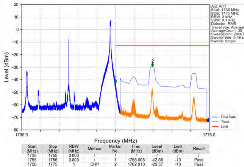
Band4_20MHz_16QAM_HCH_1745MHz_RB_1_99_NTNV
