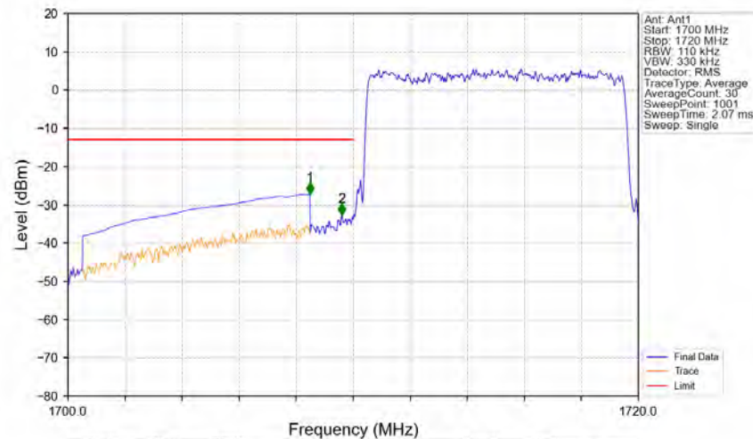
Band4_10MHz_16QAM_LCH_1715MHz_RB_50_0_NTNV
