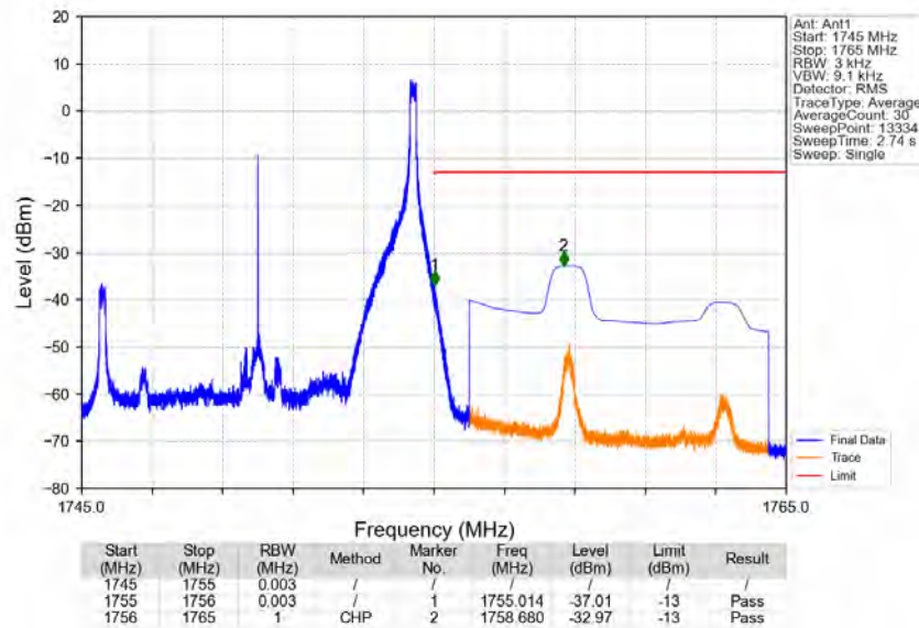
Band4_10MHz_64QAM_HCH_1750MHz_RB_1_49_NTNV
