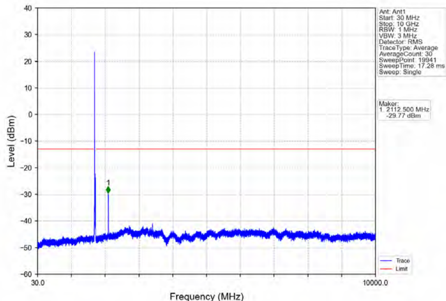
Band4_15MHz_16QAM_LCH_1717.5MHz_RB_1_0_NTNV
