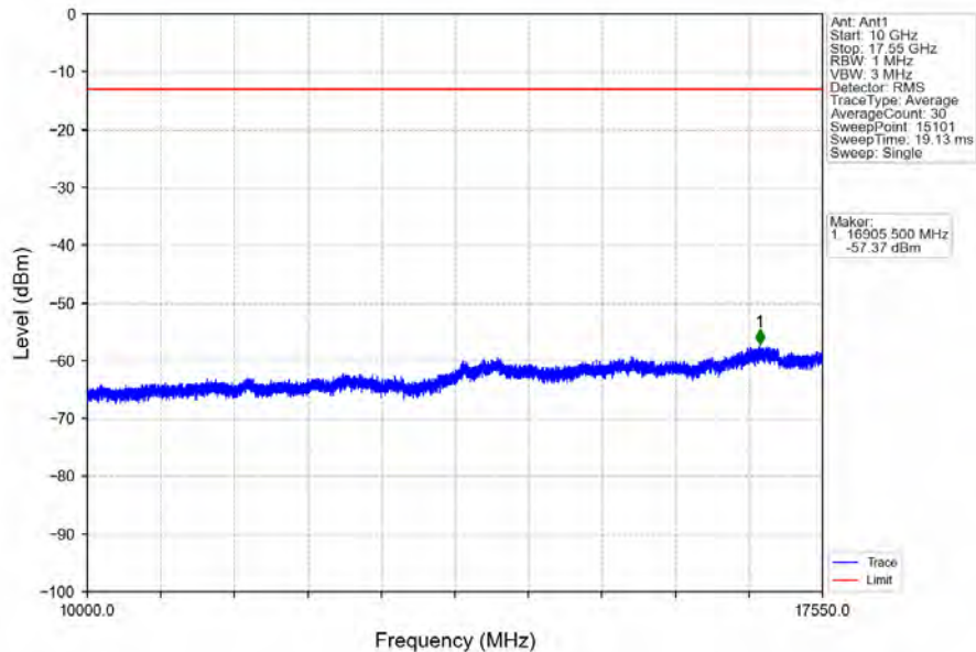
Band4_15MHz_64QAM_LCH_1717.5MHz_RB_75_0_NTNV
