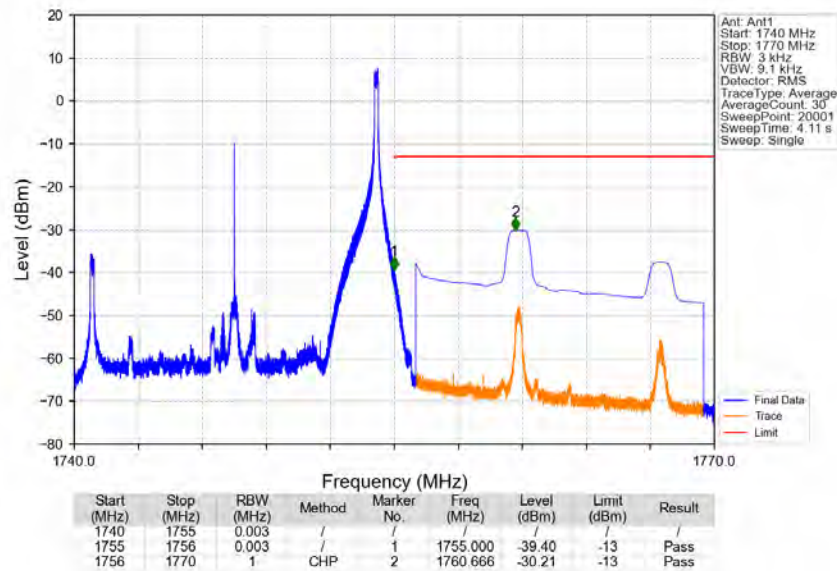
Band4_15MHz_16QAM_HCH_1747.5MHz_RB_1_74_NTNV
