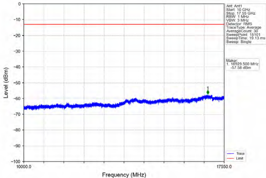
Band4_3MHz_16QAM_LCH_1711.5MHz_RB_15_0_NTNV
