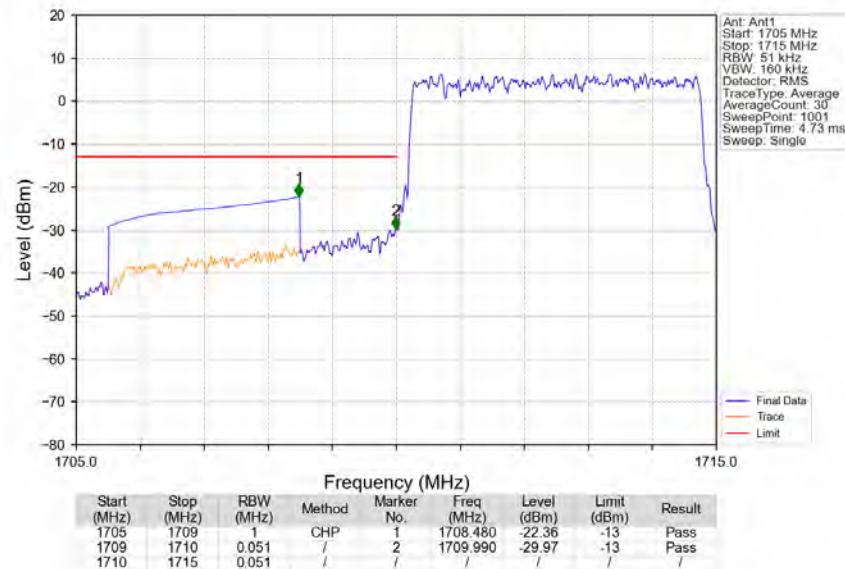
Band4_5MHz_QPSK_LCH_1712.5MHz_RB_25_0_NTNV
