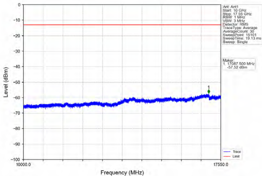
Band4_10MHz_64QAM_MCH_1732.5MHz_RB_1_0_NTNV
