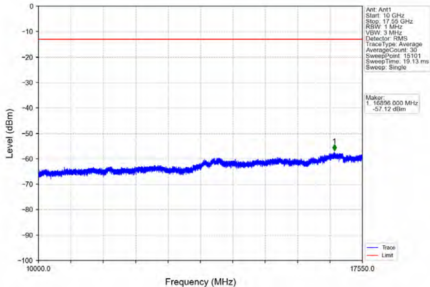
Band4_1.4MHz_64QAM_LCH_1710.7MHz_RB_6_0_NTNV
