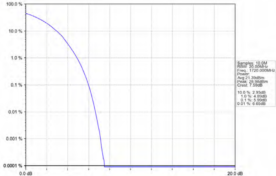
Band4_20MHz_64QAM_LCH_1720MHz_RB_100_0_NTNV
