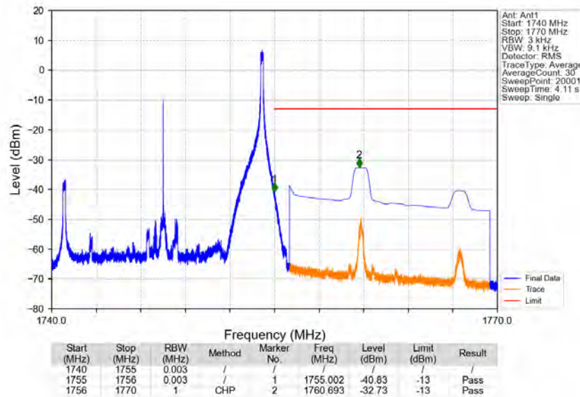
Band4_15MHz_64QAM_HCH_1747.5MHz_RB_1_74_NTNV
