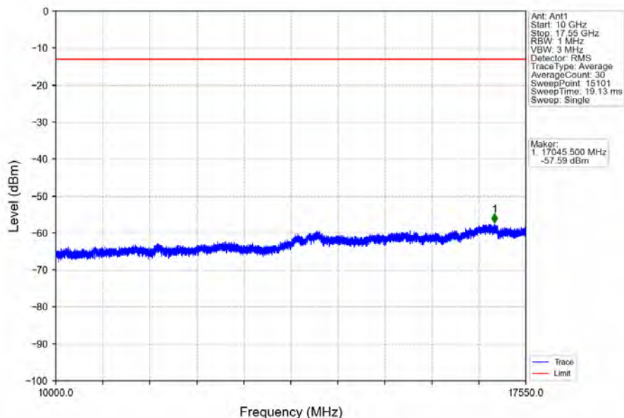
Band4_1.4MHz_64QAM_HCH_1754.3MHz_RB_1_0_NTNV
