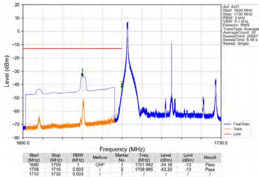
Band4_20MHz_64QAM_LCH_1720MHz_RB_1_0_NTNV
