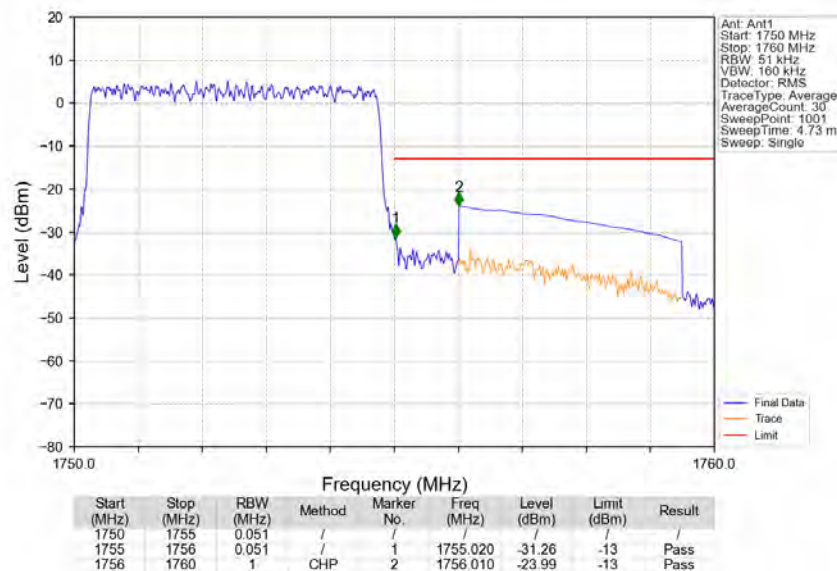
Band4_5MHz_16QAM_HCH_1752.5MHz_RB_25_0_NTNV
