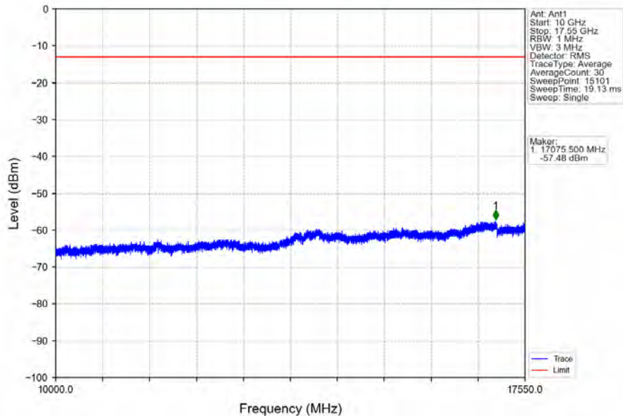
Band4_1.4MHz_16QAM_LCH_1710.7MHz_RB_6_0_NTNV
