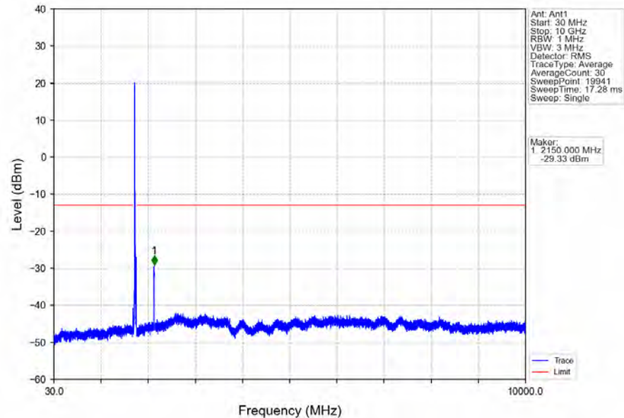
Band4_20MHz_64QAM_HCH_1745MHz_RB_1_0_NTNV
