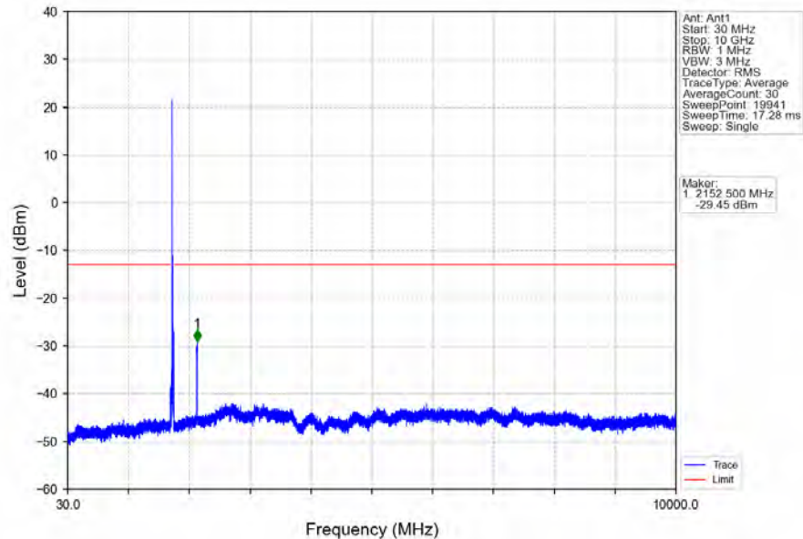
Band4_15MHz_64QAM_HCH_1747.5MHz_RB_1_0_NTNV
