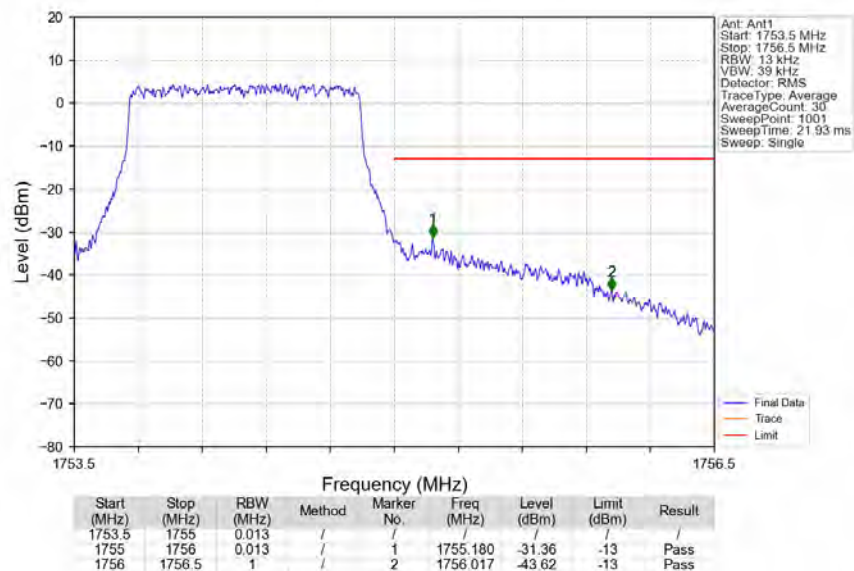
Band4_1.4MHz_16QAM_HCH_1754.3MHz_RB_6_0_NTNV
