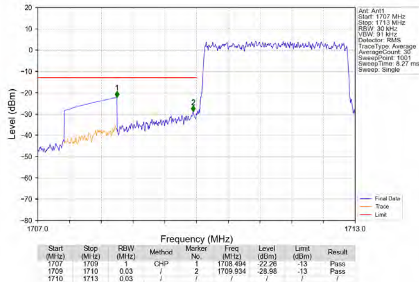
Band4_3MHz_64QAM_LCH_1711.5MHz_RB_15_0_NTNV
