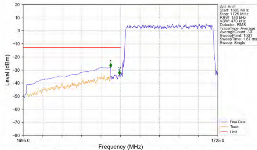
Band4_15MHz_16QAM_LCH_1717.5MHz_RB_75_0_NTNV
