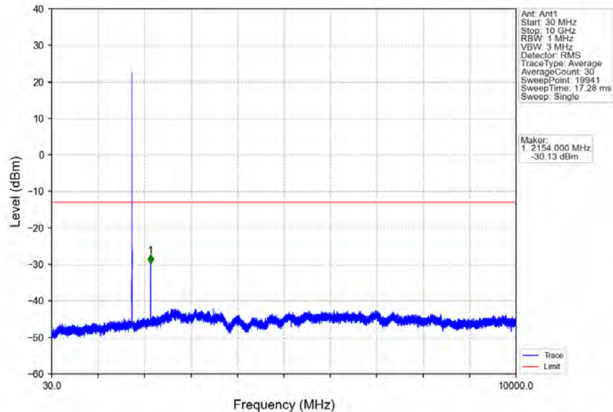
Band4_3MHz_16QAM_HCH_1753.5MHz_RB_1_0_NTNV
