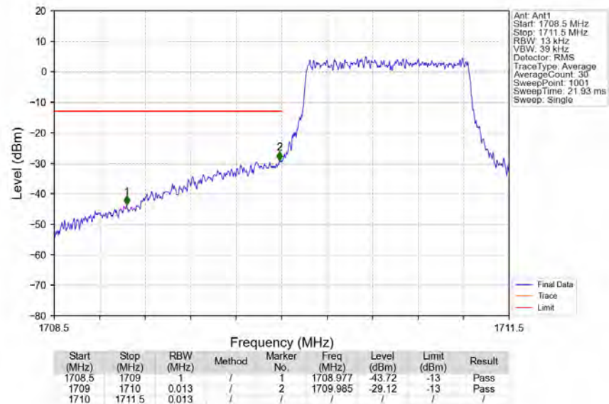
Band4_1.4MHz_64QAM_LCH_1710.7MHz_RB_6_0_NTNV
