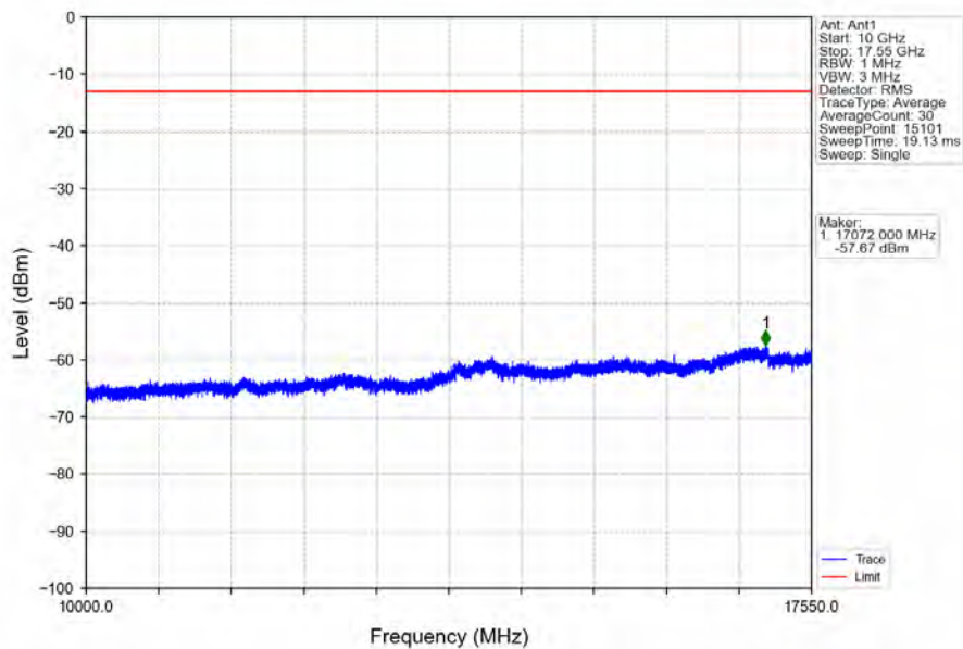
Band4_5MHz_16QAM_MCH_1732.5MHz_RB_1_0_NTNV
