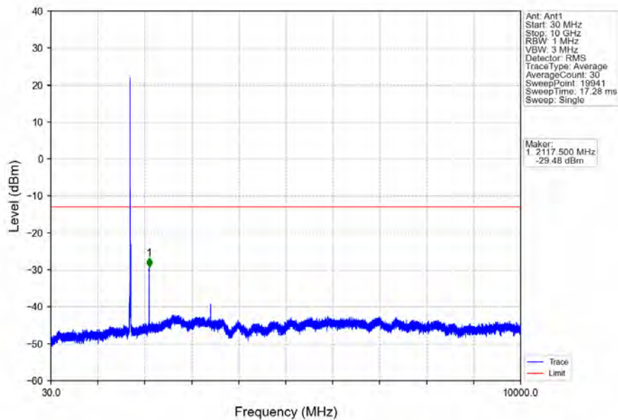
Band4_10MHz_16QAM_LCH_1715MHz_RB_1_0_NTNV
