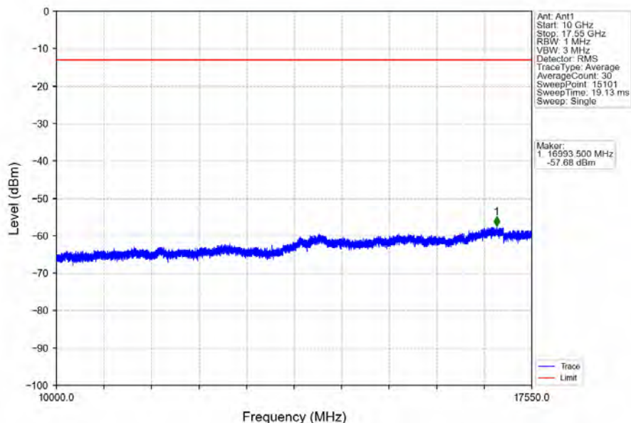
Band4_20MHz_16QAM_HCH_1745MHz_RB_1_0_NTNV
