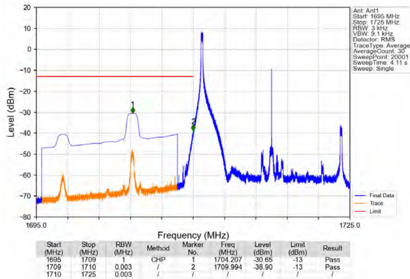
Band4_15MHz_16QAM_LCH_1717.5MHz_RB_1_0_NTNV
