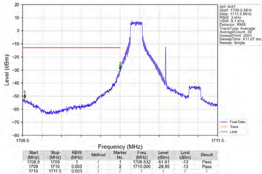
Band4_1.4MHz_16QAM_LCH_1710.7MHz_RB_1_0_NTNV
