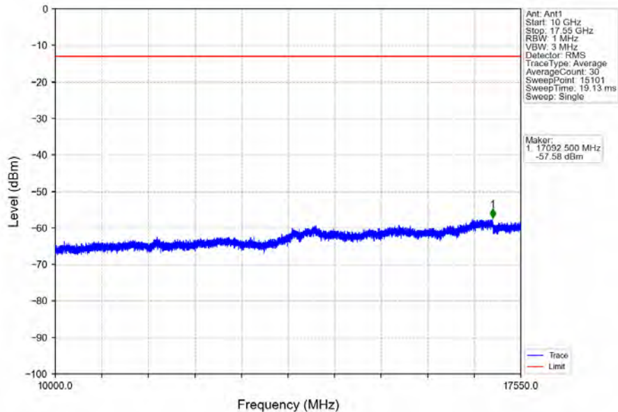
Band4_5MHz_64QAM_LCH_1712.5MHz_RB_25_0_NTNV
