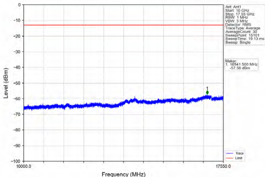
Band4_10MHz_64QAM_HCH_1750MHz_RB_1_0_NTNV
