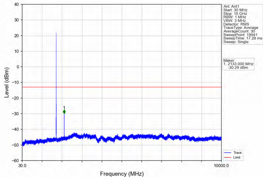
Band4_3MHz_64QAM_MCH_1732.5MHz_RB_1_0_NTNV
