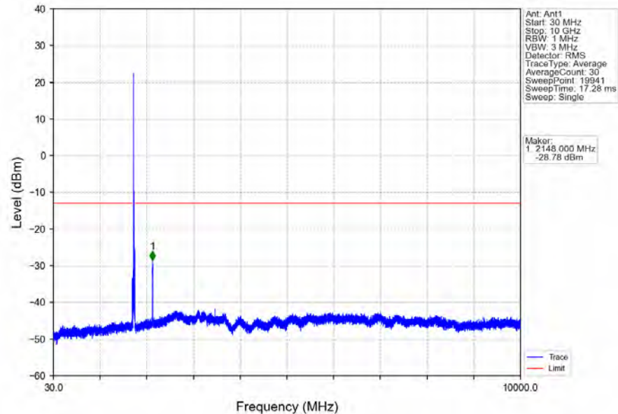
Band4_15MHz_16QAM_HCH_1747.5MHz_RB_1_0_NTNV
