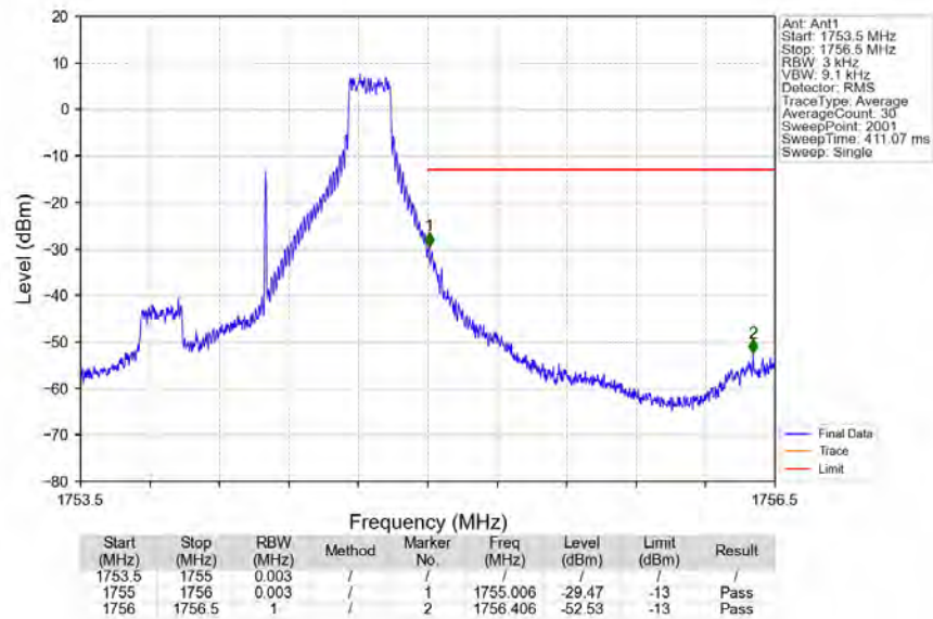
Band4_1.4MHz_16QAM_HCH_1754.3MHz_RB_1_5_NTNV
