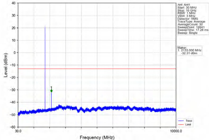
Band4_1.4MHz_64QAM_MCH_1732.5MHz_RB_1_0_NTNV
