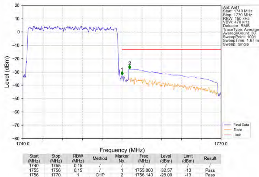
Band4_15MHz_16QAM_HCH_1747.5MHz_RB_75_0_NTNV
