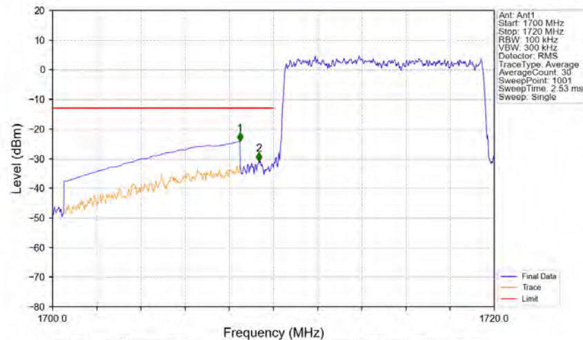
Band4_10MHz_64QAM_LCH_1715MHz_RB_50_0_NTNV
