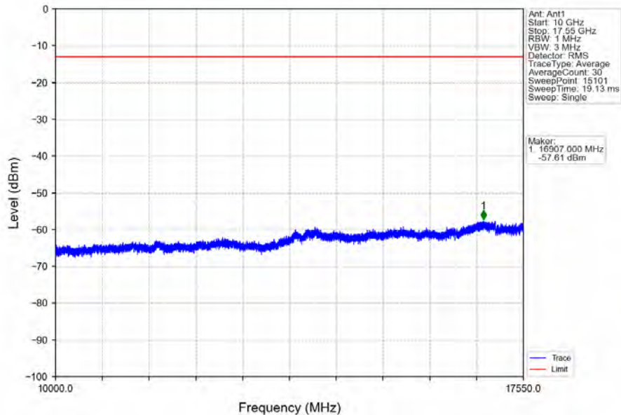
Band4_5MHz_QPSK_LCH_1712.5MHz_RB_25_0_NTNV
