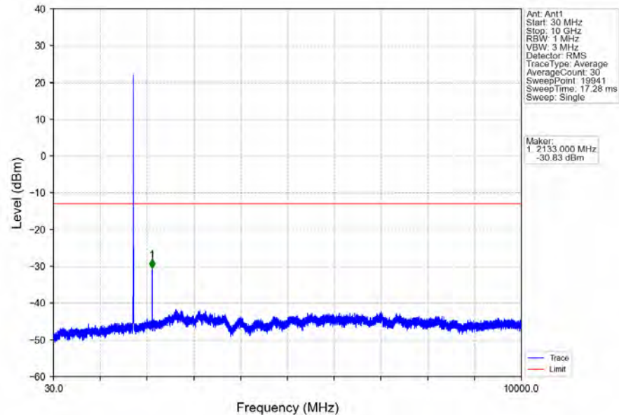
Band4_5MHz_64QAM_MCH_1732.5MHz_RB_1_0_NTNV
