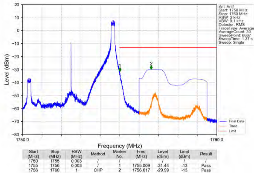
Band4_5MHz_16QAM_HCH_1752.5MHz_RB_1_24_NTNV
