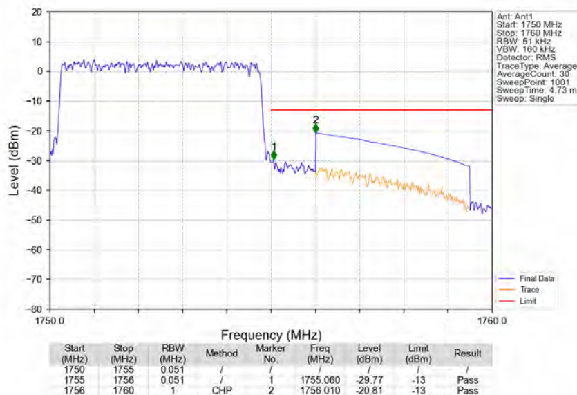
Band4_5MHz_64QAM_HCH_1752.5MHz_RB_25_0_NTNV
