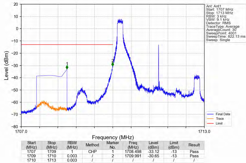
Band4_3MHz_16QAM_LCH_1711.5MHz_RB_1_0_NTNV
