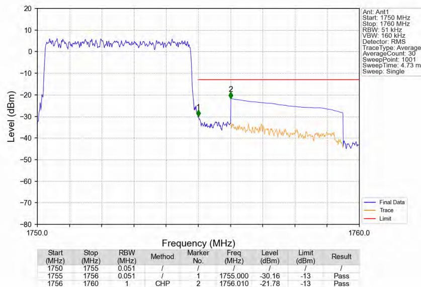
Band4_5MHz_QPSK_HCH_1752.5MHz_RB_25_0_NTNV
