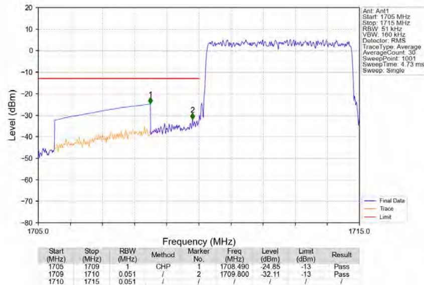
Band4_5MHz_16QAM_LCH_1712.5MHz_RB_25_0_NTNV
