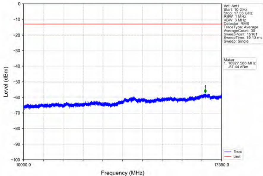
Band4_5MHz_16QAM_LCH_1712.5MHz_RB_25_0_NTNV
