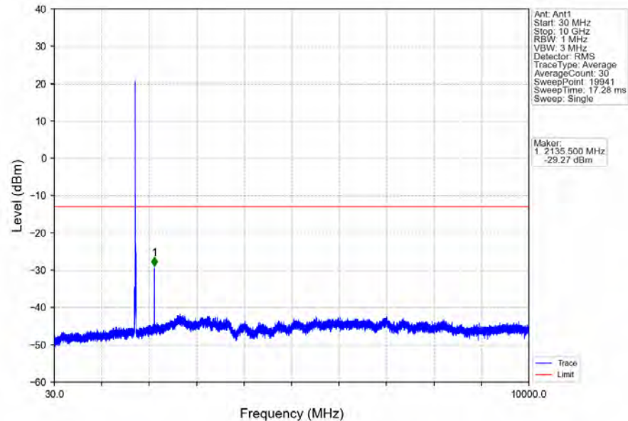
Band4_10MHz_64QAM_MCH_1732.5MHz_RB_1_0_NTNV
