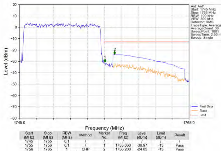
Band4_10MHz_64QAM_HCH_1750MHz_RB_50_0_NTNV
