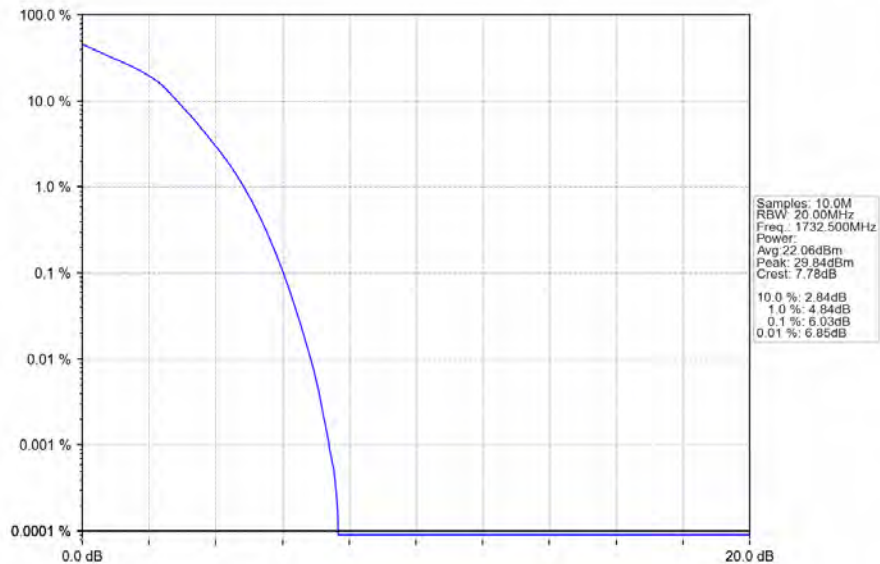
Band4_20MHz_16QAM_MCH_1732.5MHz_RB_100_0_NTNV
