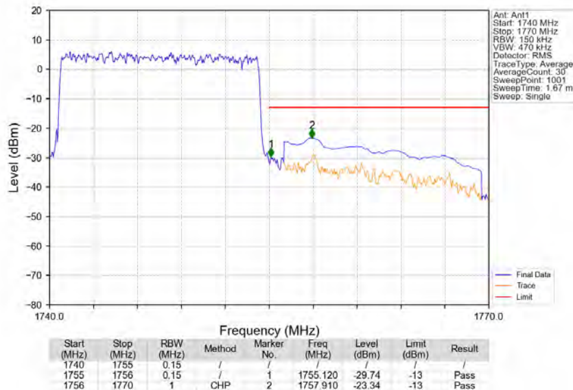
Band4_15MHz_QPSK_HCH_1747.5MHz_RB_75_0_NTNV
