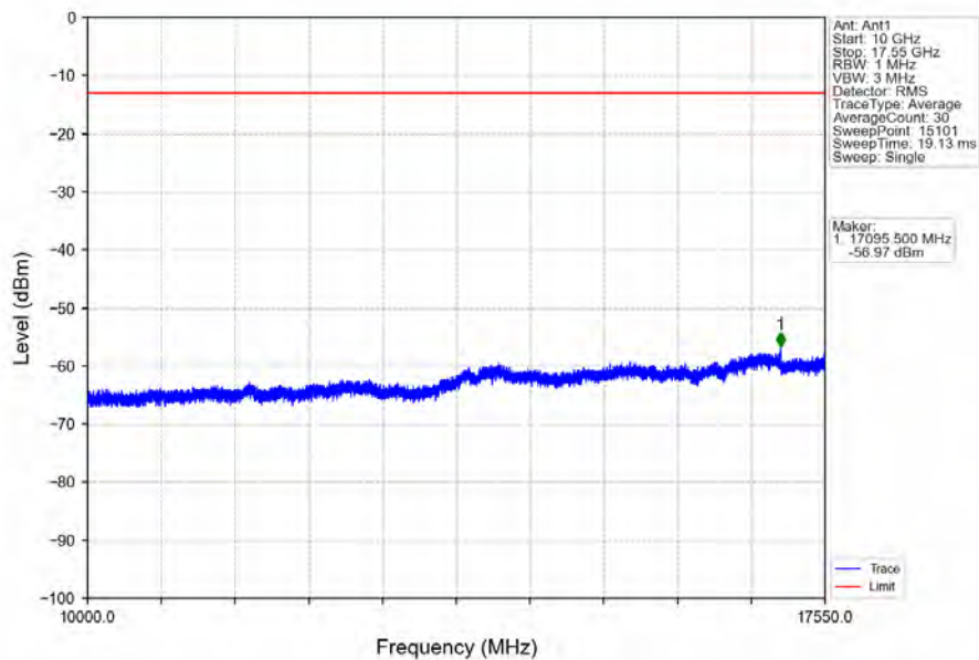
Band4_20MHz_64QAM_MCH_1732.5MHz_RB_1_0_NTNV
