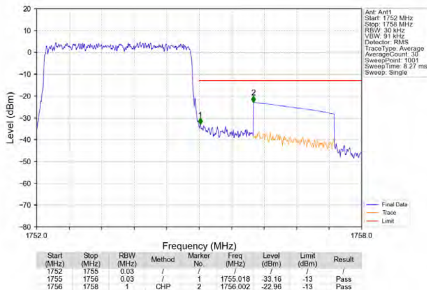
Band4_3MHz_16QAM_HCH_1753.5MHz_RB_15_0_NTNV
