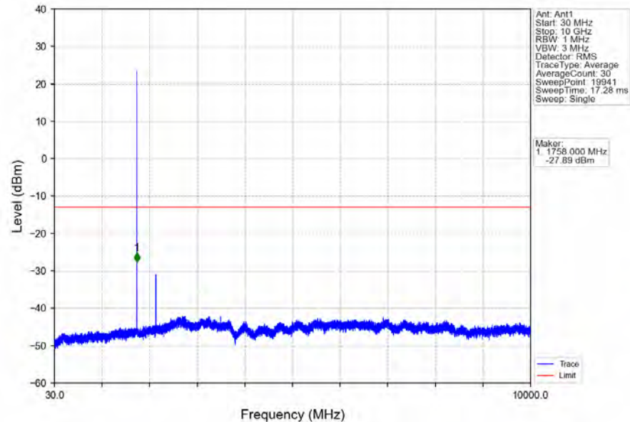
Band4_1.4MHz_QPSK_HCH_1754.3MHz_RB_1_0_NTNV
