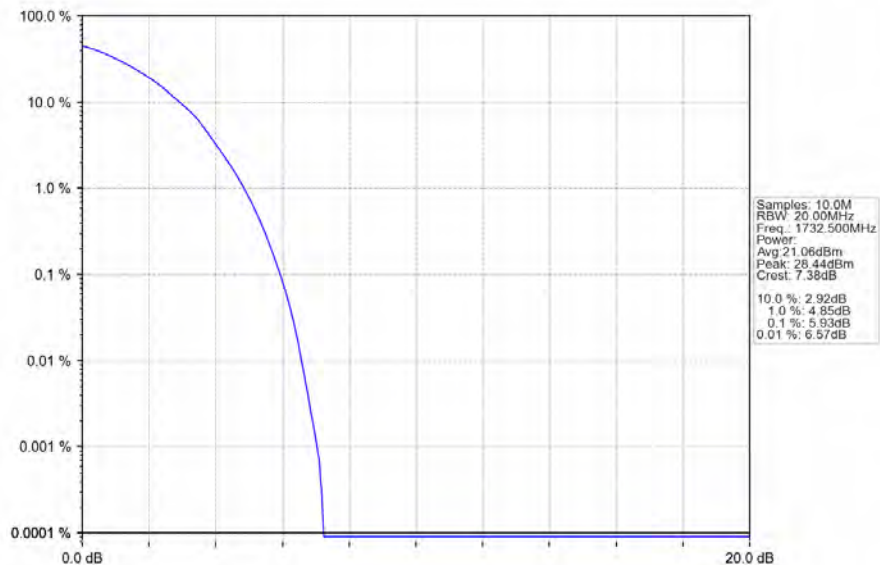
Band4_20MHz_64QAM_MCH_1732.5MHz_RB_100_0_NTNV
