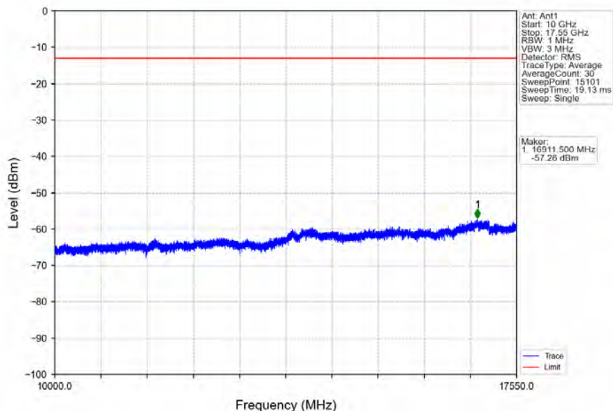
Band4_15MHz_64QAM_MCH_1732.5MHz_RB_1_0_NTNV
