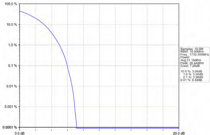
Band4_15MHz_64QAM_MCH_1732.5MHz_RB_75_0_NTNV
