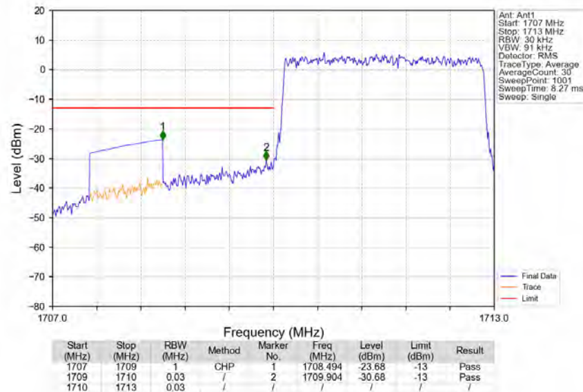
Band4_3MHz_16QAM_LCH_1711.5MHz_RB_15_0_NTNV
