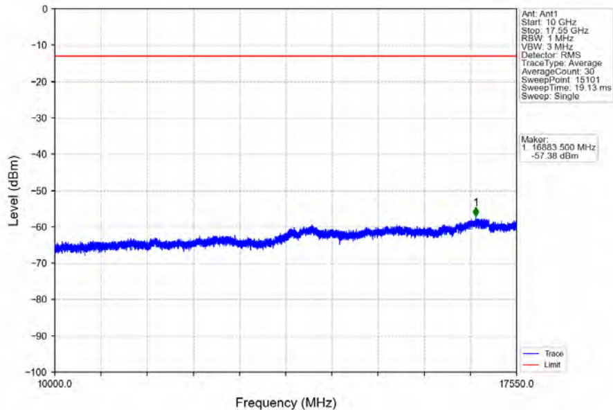
Band4_20MHz_64QAM_LCH_1720MHz_RB_100_0_NTNV
