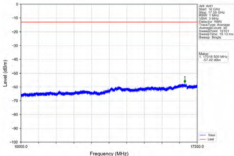
Band4_15MHz_16QAM_MCH_1732.5MHz_RB_1_0_NTNV
