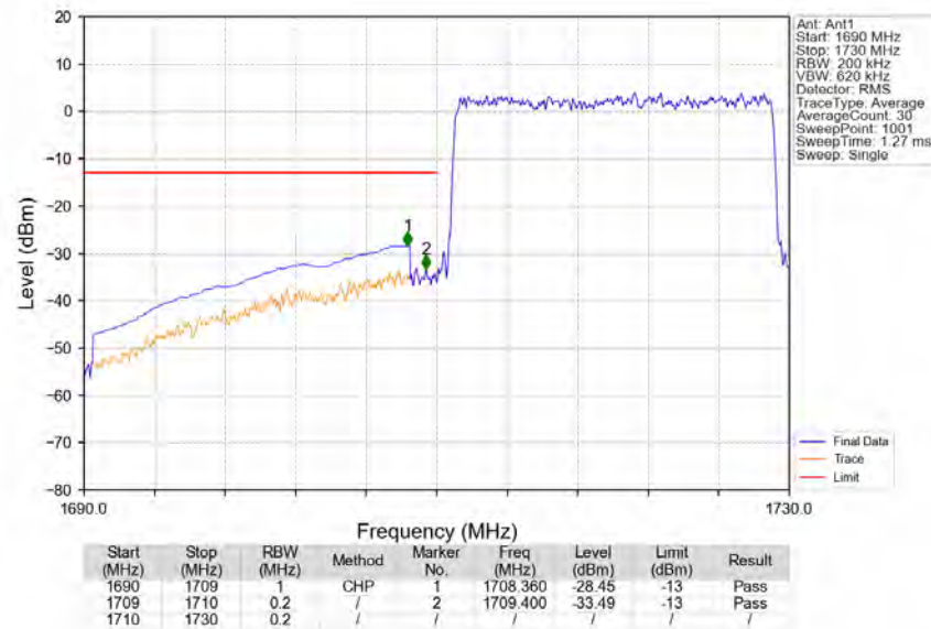
Band4_20MHz_64QAM_LCH_1720MHz_RB_100_0_NTNV
