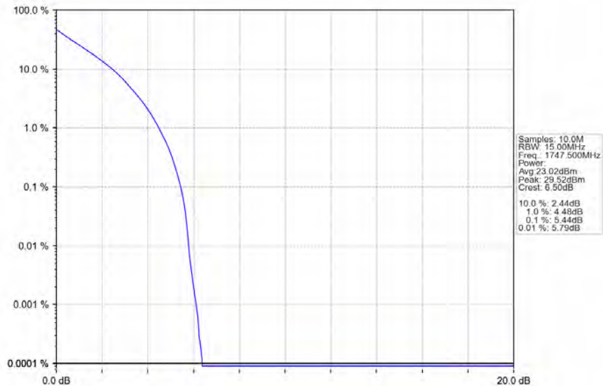
Band4_15MHz_QPSK_HCH_1747.5MHz_RB_75_0_NTNV
