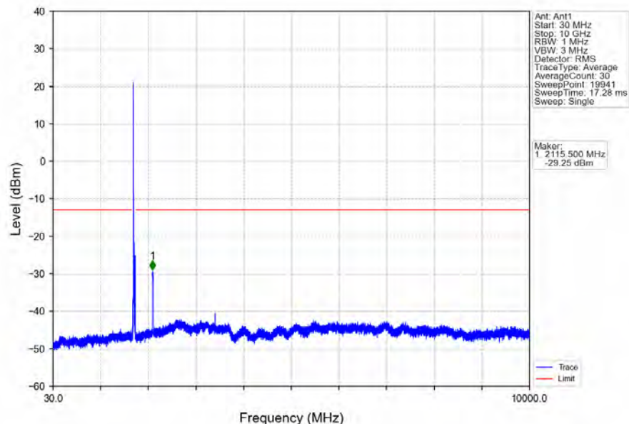
Band4_20MHz_64QAM_LCH_1720MHz_RB_1_0_NTNV
