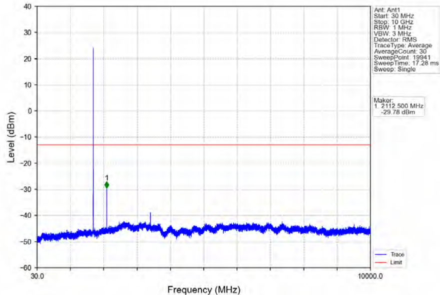
Band4_3MHz_QPSK_LCH_1711.5MHz_RB_1_0_NTNV
