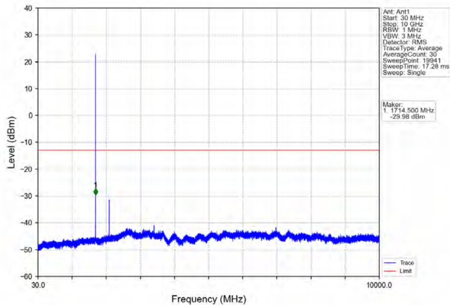
Band4_1.4MHz_64QAM_LCH_1710.7MHz_RB_1_0_NTNV
