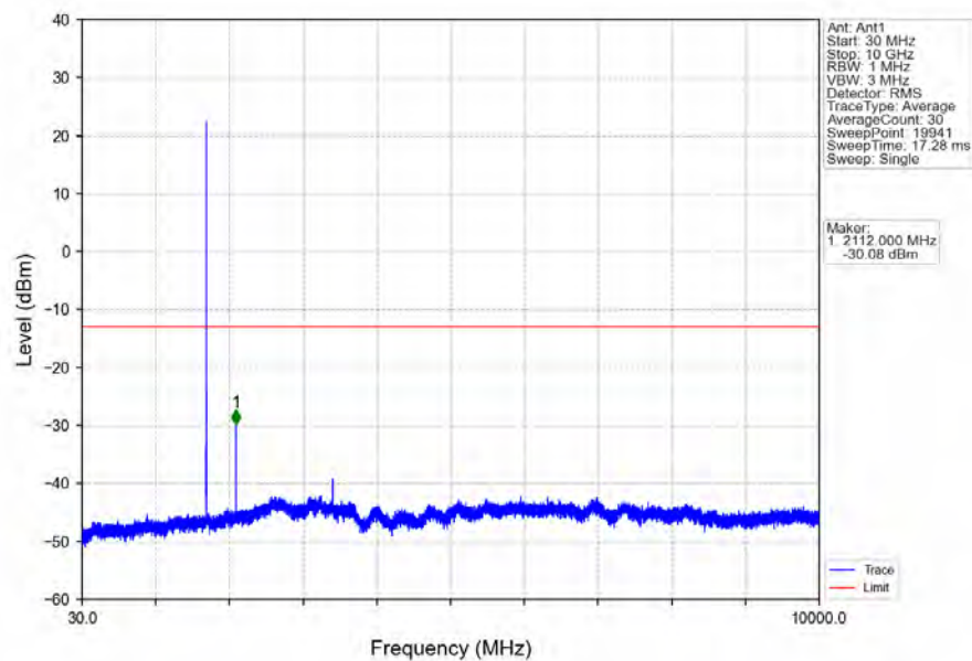
Band4_3MHz_16QAM_LCH_1711.5MHz_RB_1_0_NTNV
