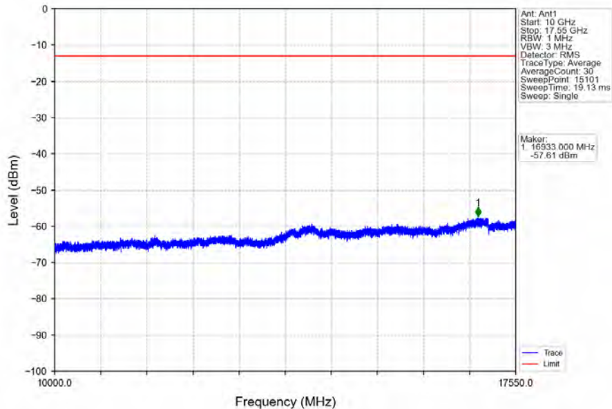
Band4_10MHz_64QAM_LCH_1715MHz_RB_50_0_NTNV
