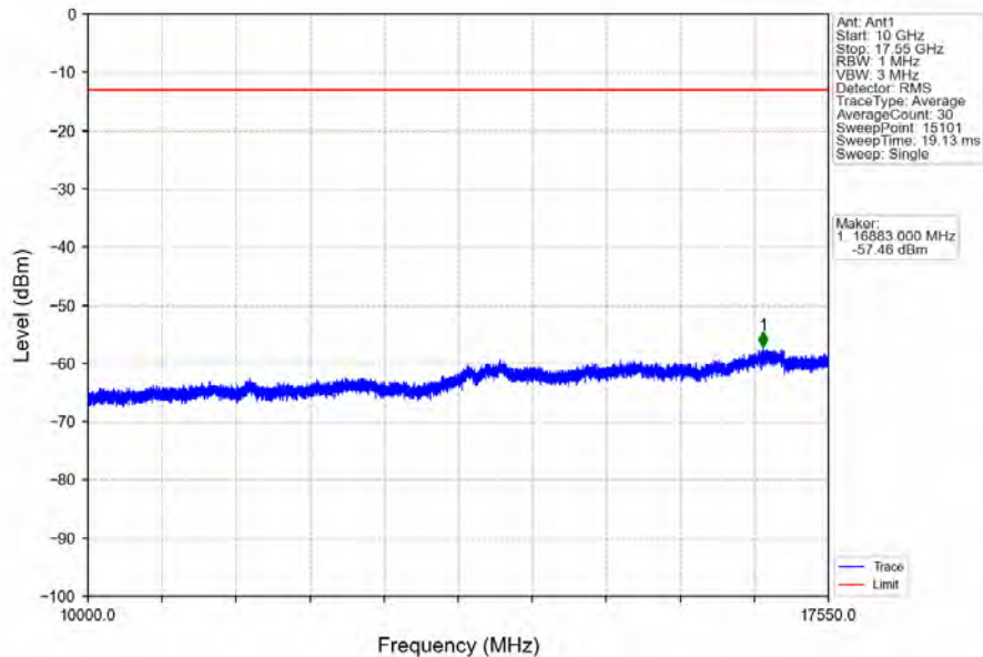
Band4_3MHz_QPSK_LCH_1711.5MHz_RB_15_0_NTNV
