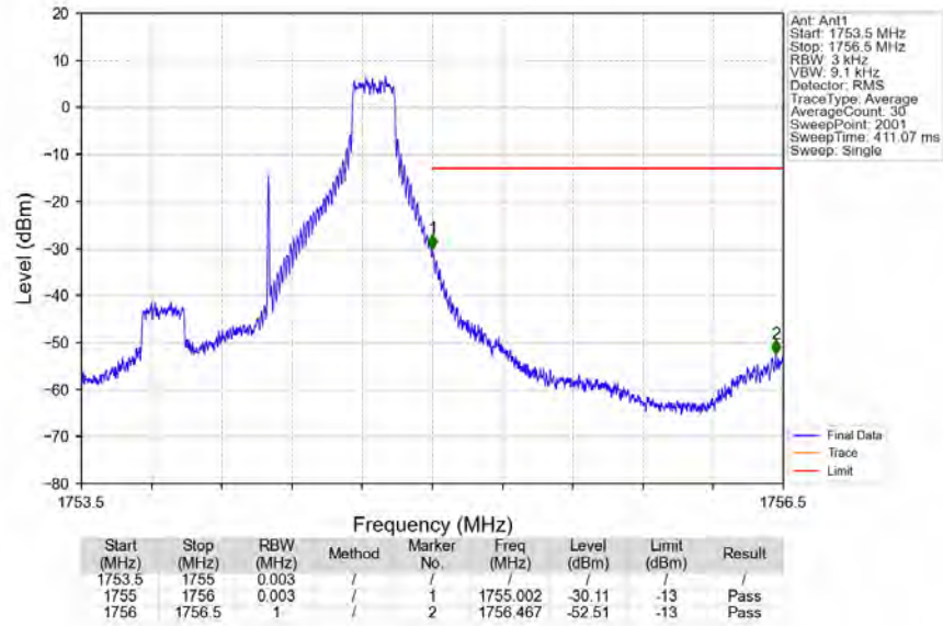
Band4_1.4MHz_64QAM_HCH_1754.3MHz_RB_1_5_NTNV
