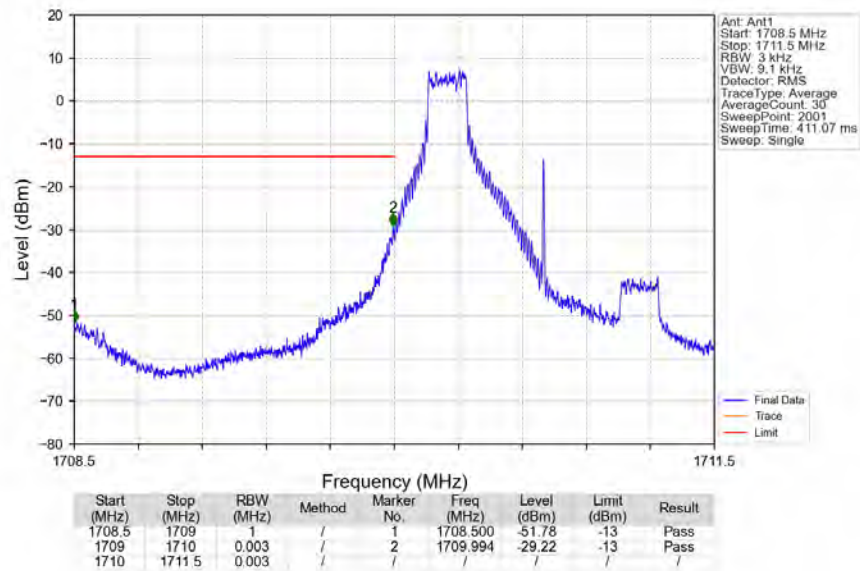
Band4_1.4MHz_64QAM_LCH_1710.7MHz_RB_1_0_NTNV
