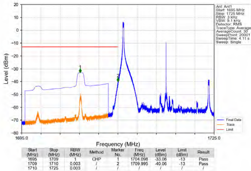
Band4_15MHz_64QAM_LCH_1717.5MHz_RB_1_0_NTNV
