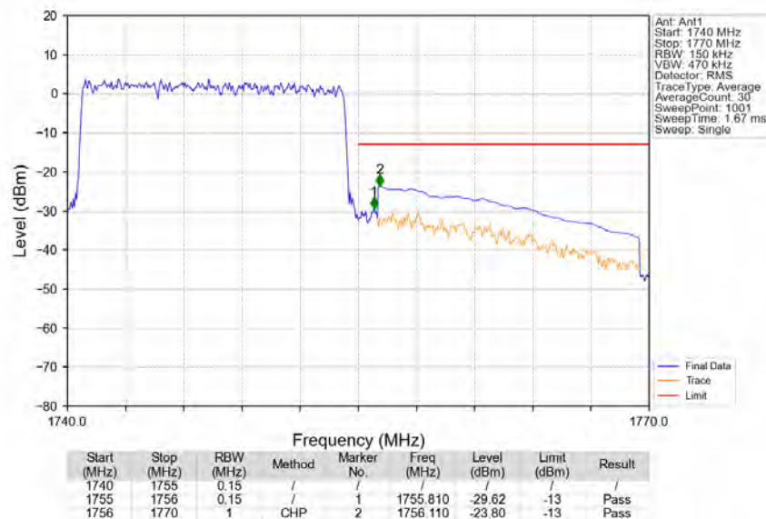
Band4_15MHz_64QAM_HCH_1747.5MHz_RB_75_0_NTNV
