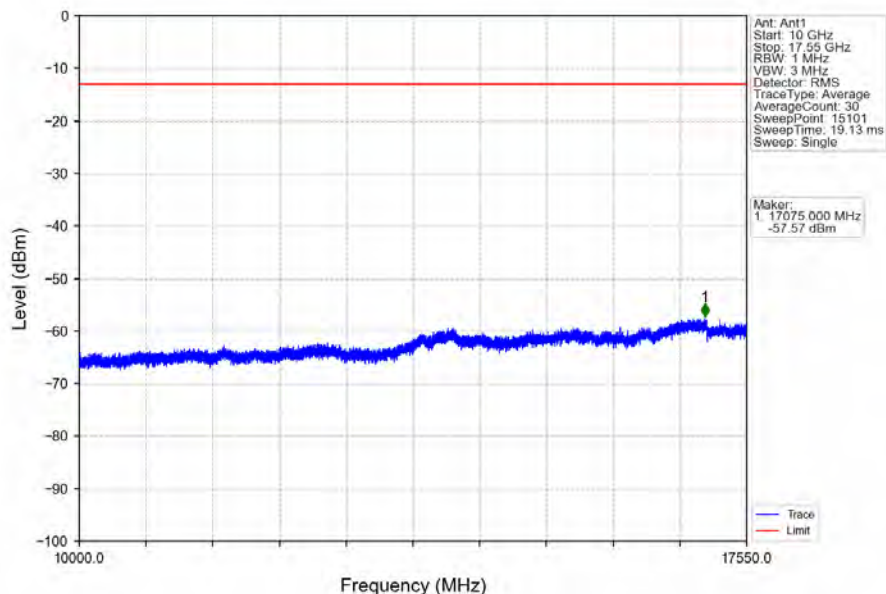
Band4_20MHz_16QAM_MCH_1732.5MHz_RB_1_0_NTNV
