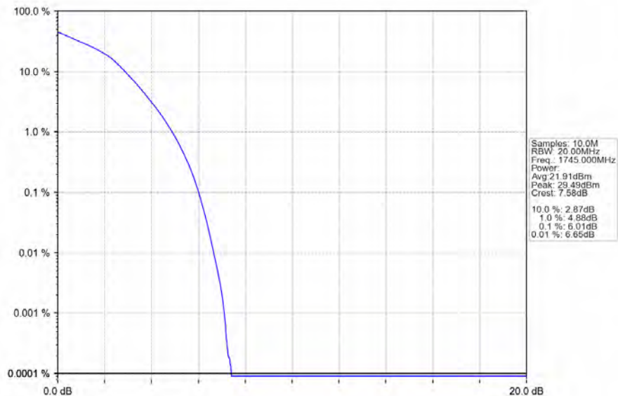
Band4_20MHz_16QAM_HCH_1745MHz_RB_100_0_NTNV
