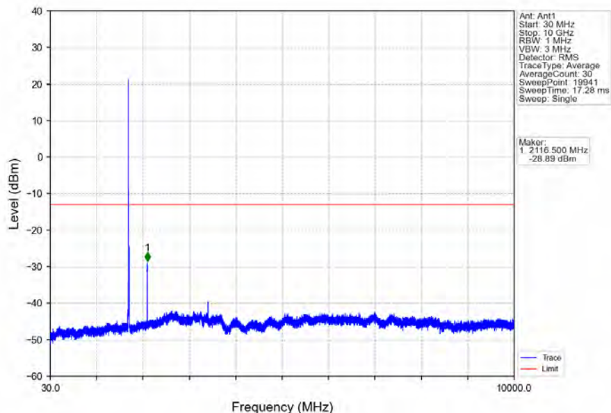
Band4_10MHz_64QAM_LCH_1715MHz_RB_1_0_NTNV
