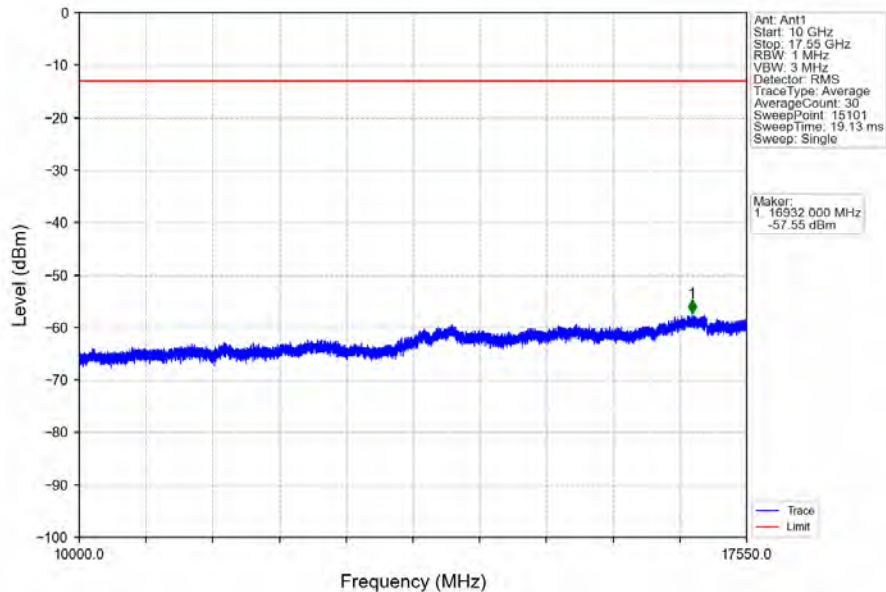
Band4_10MHz_QPSK_LCH_1715MHz_RB_50_0_NTNV
