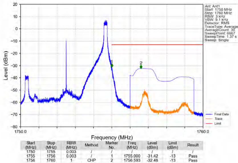
Band4_5MHz_64QAM_HCH_1752.5MHz_RB_1_24_NTNV
