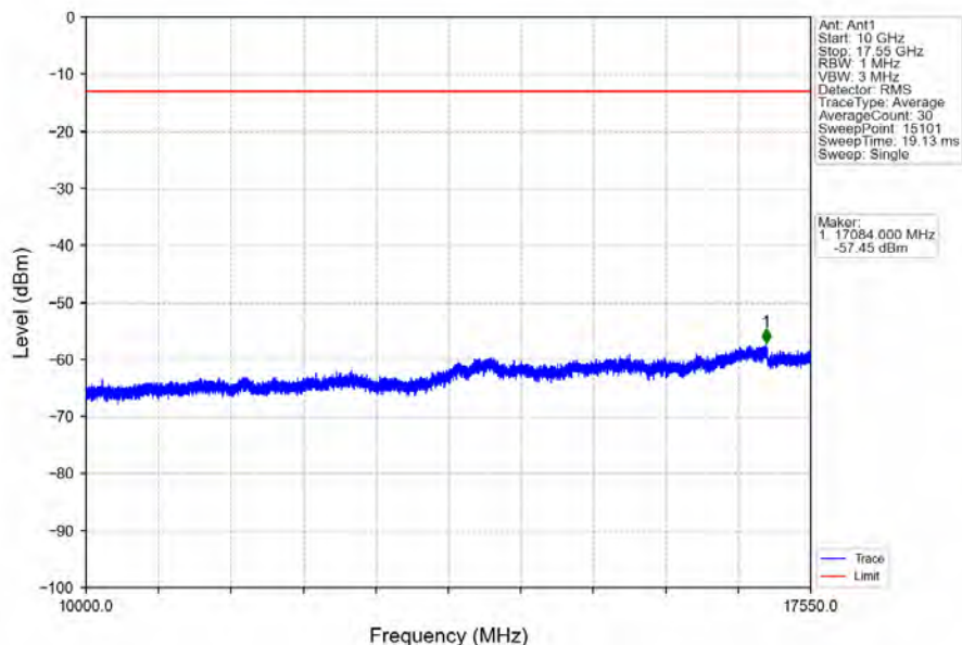
Band4_5MHz_QPSK_HCH_1752.5MHz_RB_1_0_NTNV
