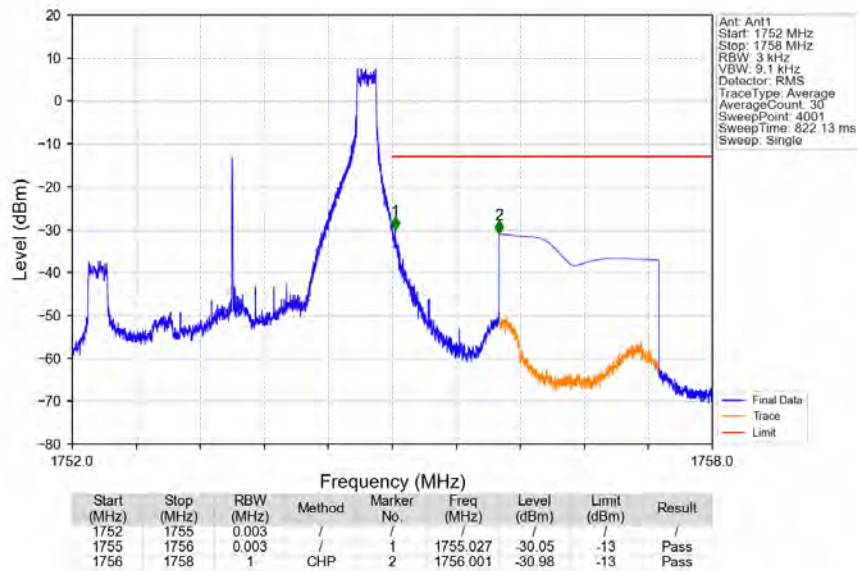
Band4_3MHz_16QAM_HCH_1753.5MHz_RB_1_14_NTNV
