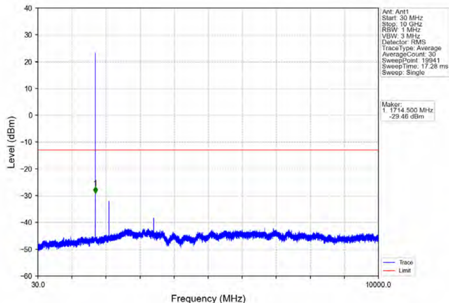
Band4_1.4MHz_16QAM_LCH_1710.7MHz_RB_1_0_NTNV
