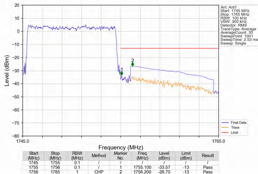
Band4_10MHz_16QAM_HCH_1750MHz_RB_50_0_NTNV
