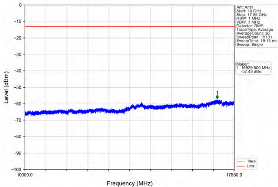
Band4_10MHz_QPSK_MCH_1732.5MHz_RB_1_0_NTNV
