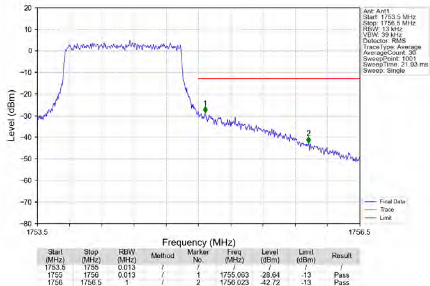
Band4_1.4MHz_64QAM_HCH_1754.3MHz_RB_6_0_NTNV
