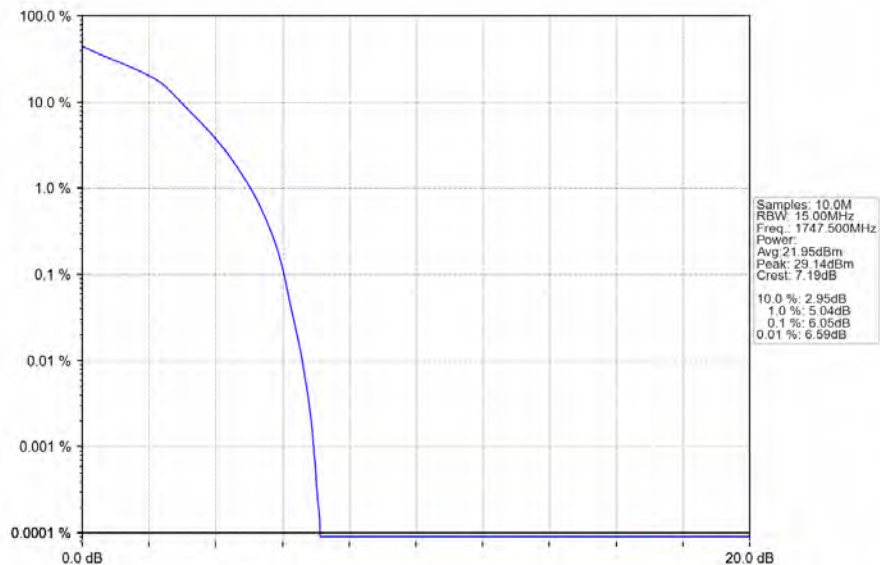
Band4_15MHz_16QAM_HCH_1747.5MHz_RB_75_0_NTNV
