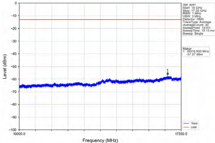
Band4_3MHz_64QAM_LCH_1711.5MHz_RB_15_0_NTNV
