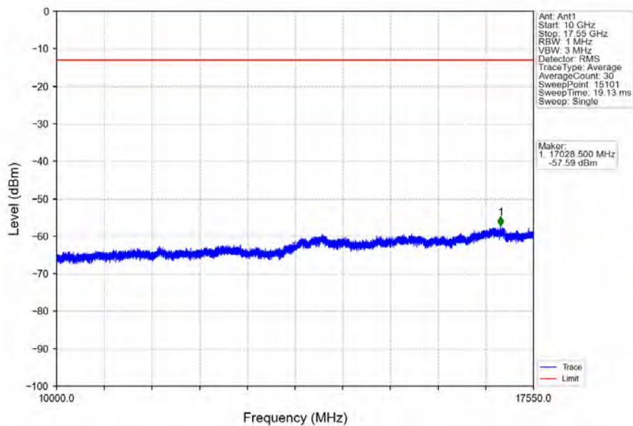
Band4_5MHz_64QAM_MCH_1732.5MHz_RB_1_0_NTNV
