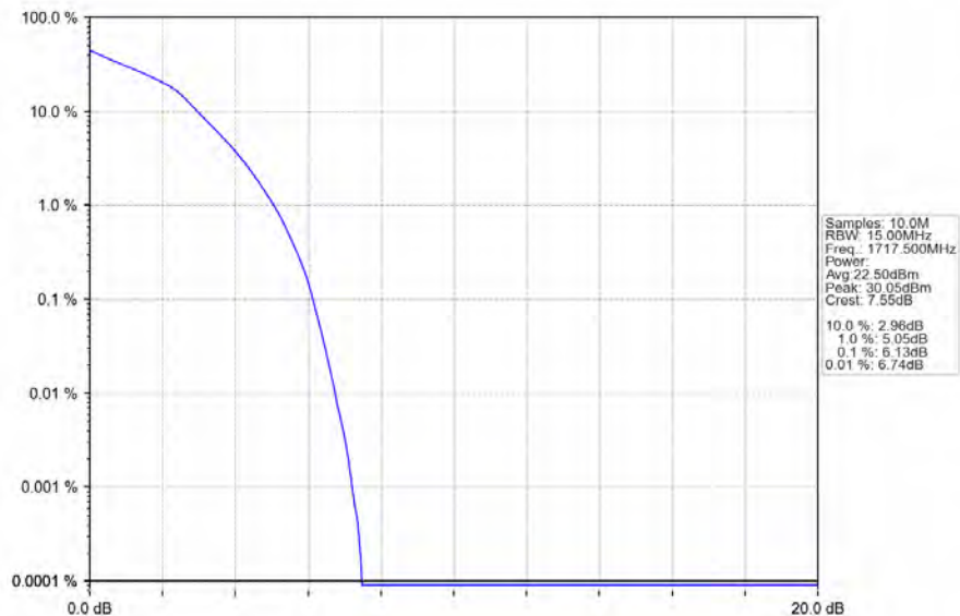
Band4_15MHz_16QAM_LCH_1717.5MHz_RB_75_0_NTNV
