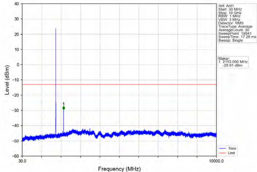
Band4_5MHz_QPSK_HCH_1752.5MHz_RB_1_0_NTNV
