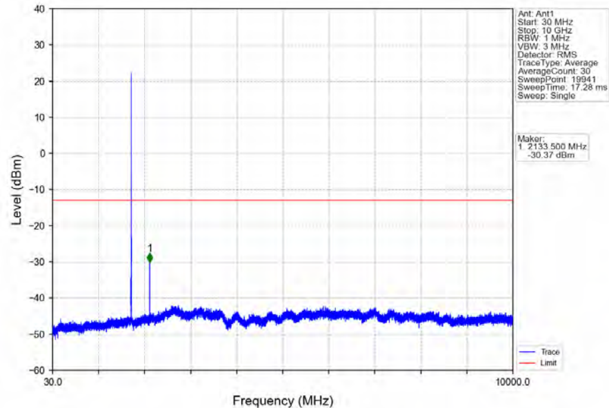
Band4_3MHz_16QAM_MCH_1732.5MHz_RB_1_0_NTNV
