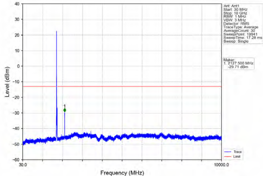
Band4_20MHz_16QAM_MCH_1732.5MHz_RB_1_0_NTNV
