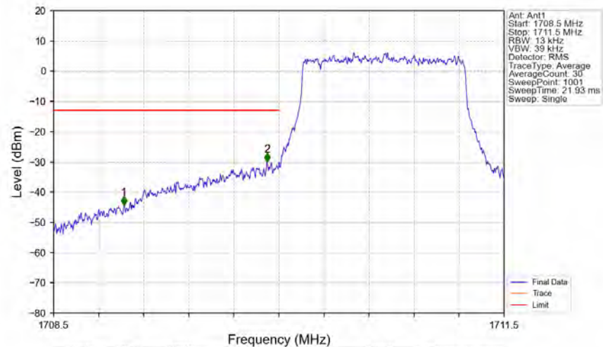
Band4_1.4MHz_16QAM_LCH_1710.7MHz_RB_6_0_NTNV
