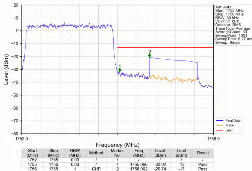
Band4_3MHz_QPSK_HCH_1753.5MHz_RB_15_0_NTNV
