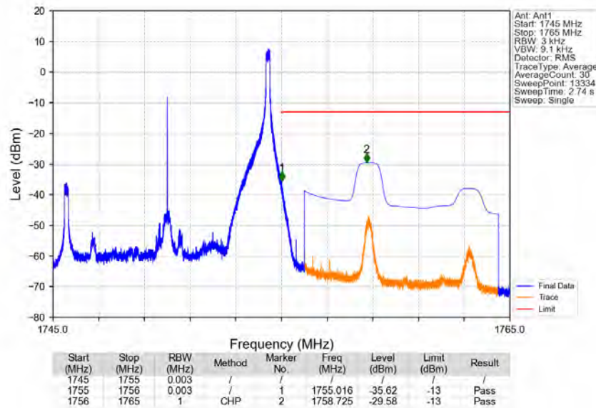
Band4_10MHz_16QAM_HCH_1750MHz_RB_1_49_NTNV
