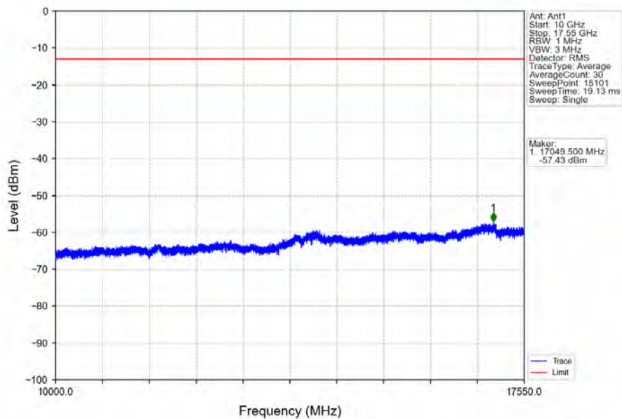
Band4_3MHz_64QAM_HCH_1753.5MHz_RB_1_0_NTNV
