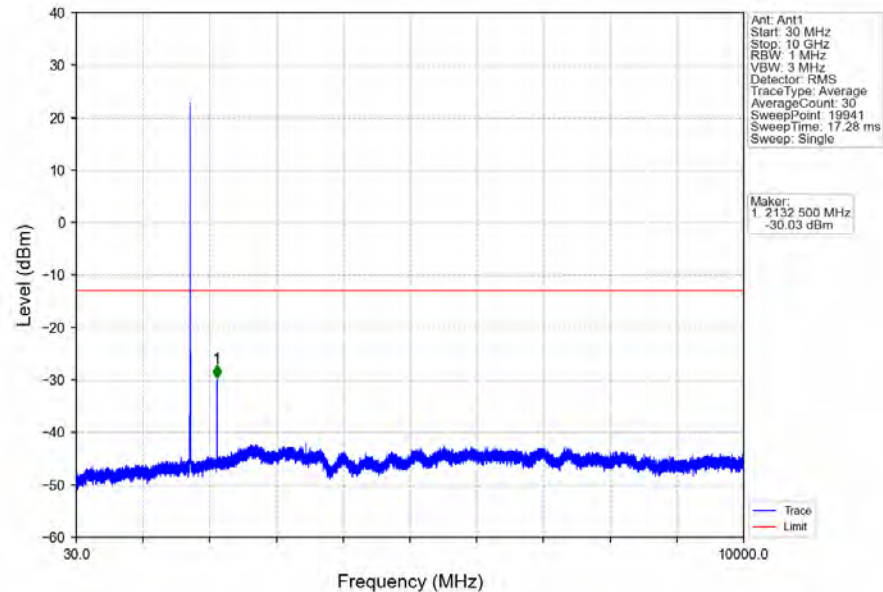
Band4_5MHz_16QAM_MCH_1732.5MHz_RB_1_0_NTNV
