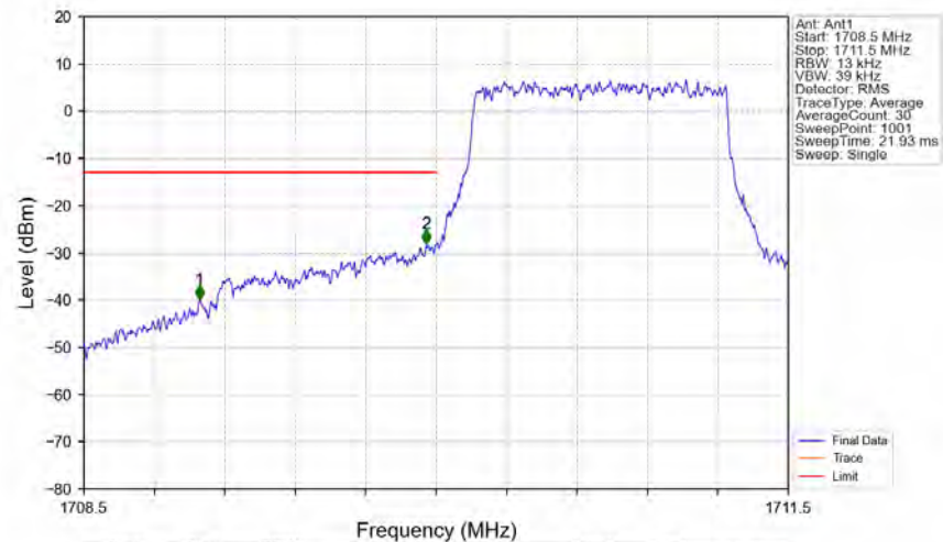
Band4_1.4MHz_QPSK_LCH_1710.7MHz_RB_6_0_NTNV
