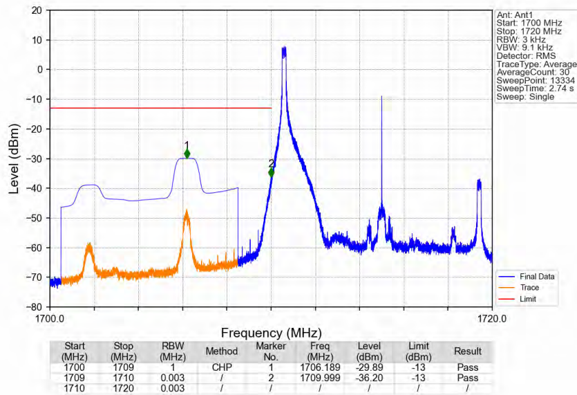
Band4_10MHz_16QAM_LCH_1715MHz_RB_1_0_NTNV
