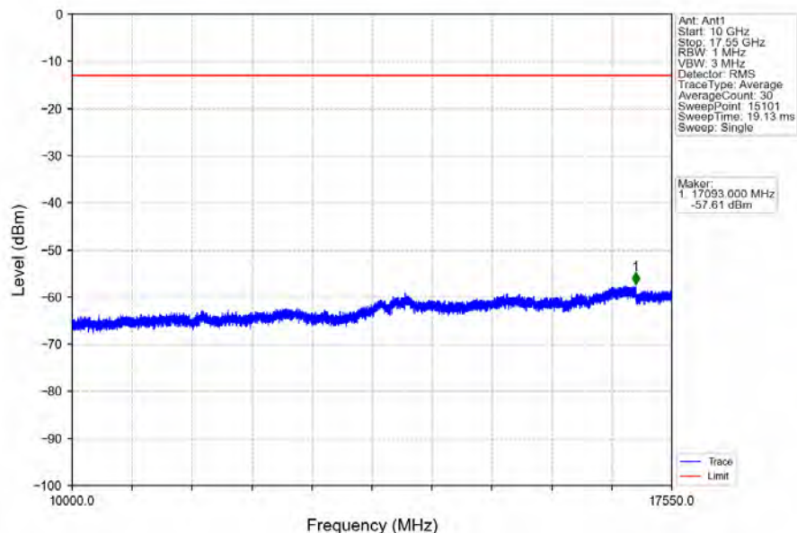
Band4_1.4MHz_64QAM_MCH_1732.5MHz_RB_1_0_NTNV
