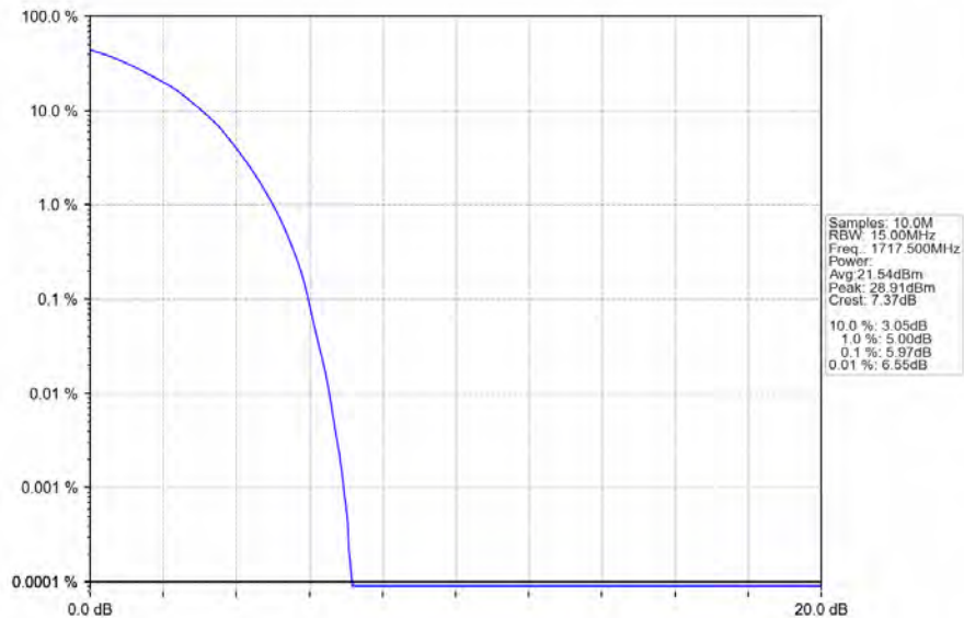
Band4_15MHz_64QAM_LCH_1717.5MHz_RB_75_0_NTNV
