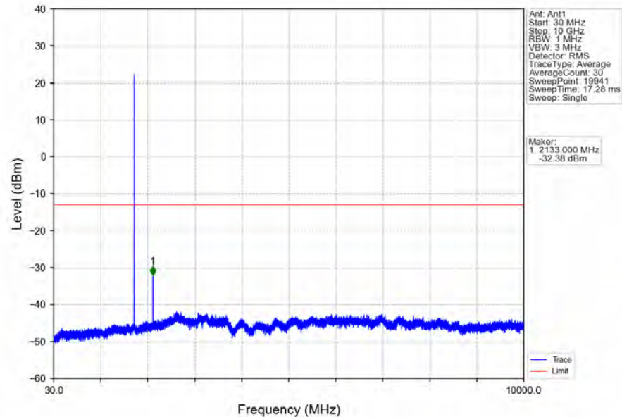
Band4_1.4MHz_16QAM_MCH_1732.5MHz_RB_1_0_NTNV
