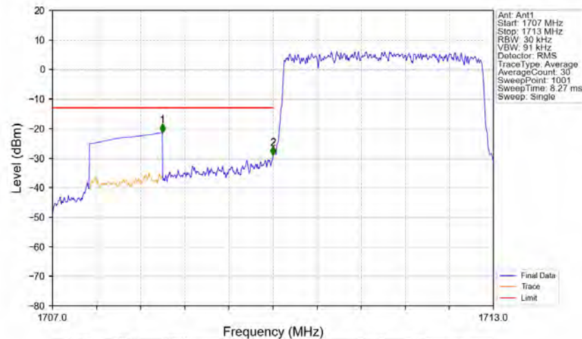
Band4_3MHz_QPSK_LCH_1711.5MHz_RB_15_0_NTNV
