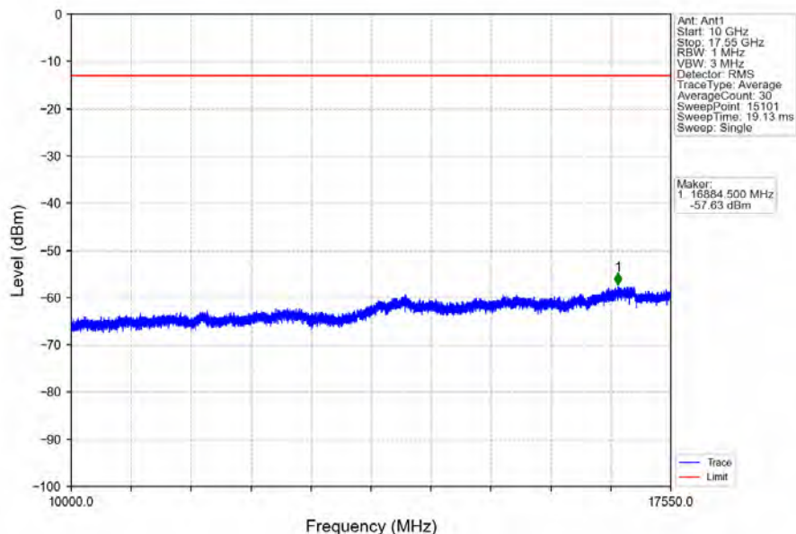
Band4_5MHz_64QAM_HCH_1752.5MHz_RB_1_0_NTNV
