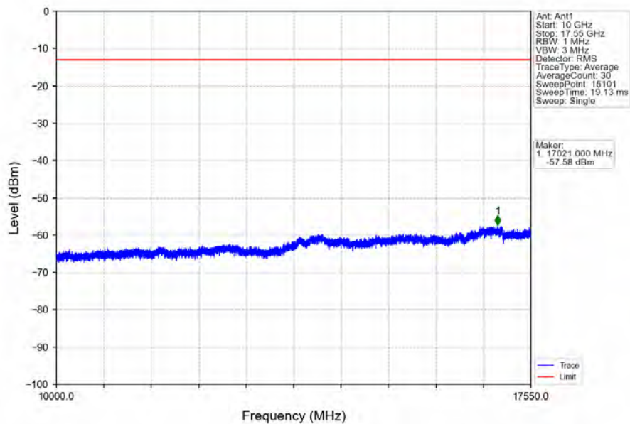
Band4_15MHz_QPSK_HCH_1747.5MHz_RB_1_0_NTNV
