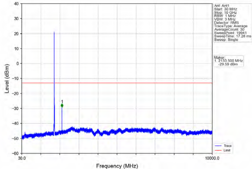
Band4_15MHz_64QAM_MCH_1732.5MHz_RB_1_0_NTNV
