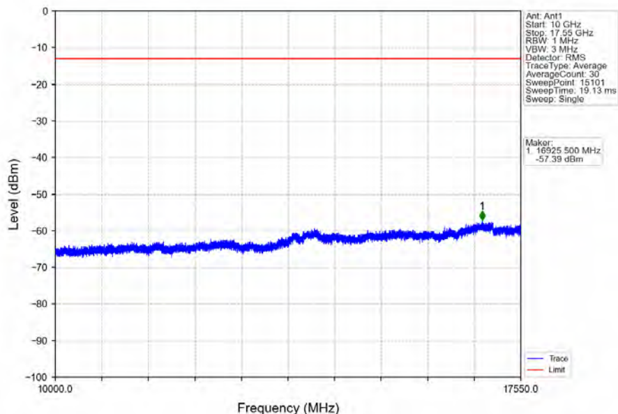
Band4_5MHz_16QAM_HCH_1752.5MHz_RB_1_0_NTNV
