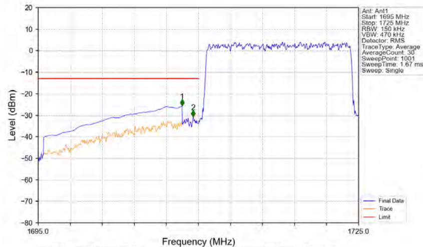
Band4_15MHz_64QAM_LCH_1717.5MHz_RB_75_0_NTNV
