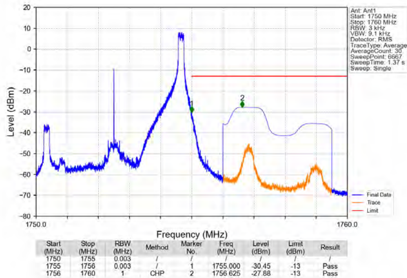
Band4_5MHz_QPSK_HCH_1752.5MHz_RB_1_24_NTNV
