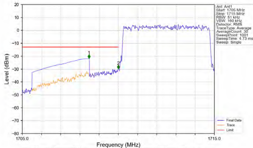
Band4_5MHz_64QAM_LCH_1712.5MHz_RB_25_0_NTNV
