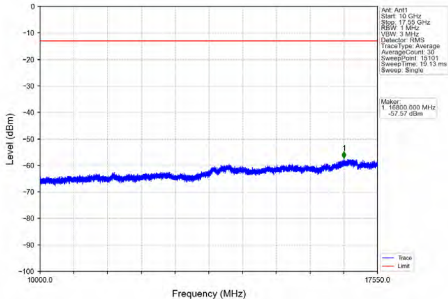
Band4_10MHz_16QAM_LCH_1715MHz_RB_50_0_NTNV
