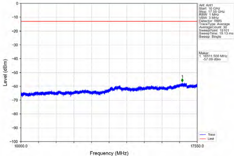
Band4_1.4MHz_QPSK_LCH_1710.7MHz_RB_6_0_NTNV
