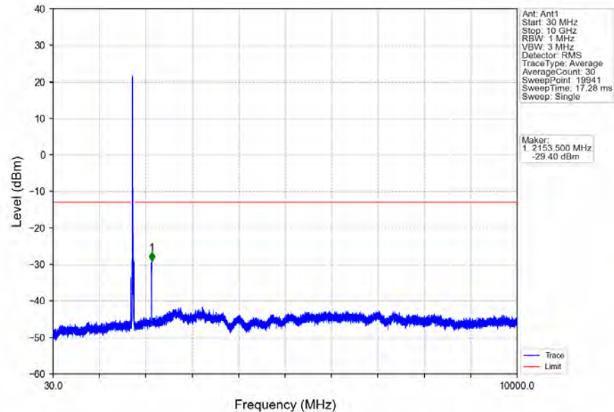
Band4_20MHz_16QAM_HCH_1745MHz_RB_1_0_NTNV
