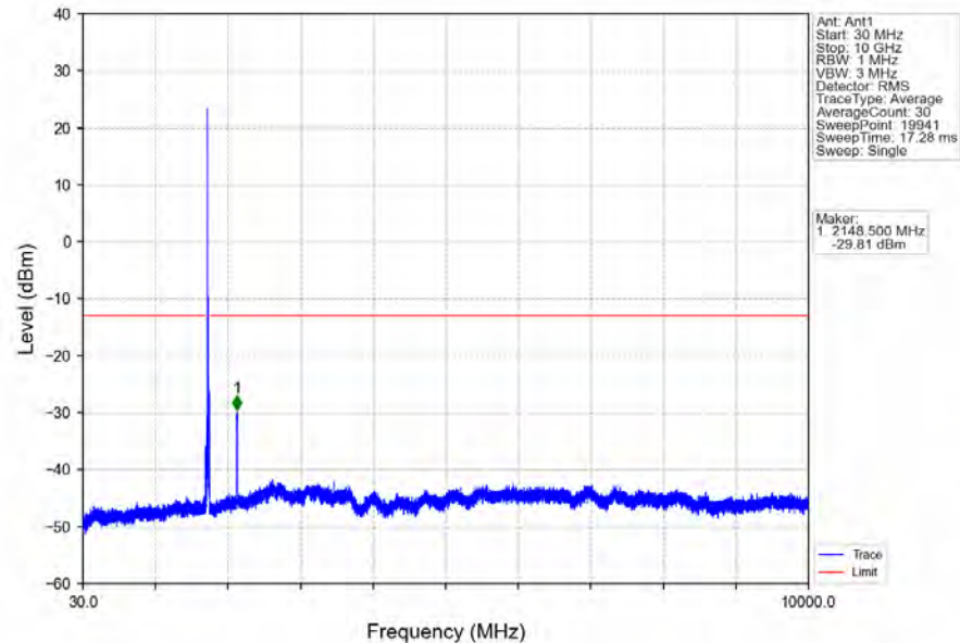
Band4_15MHz_QPSK_HCH_1747.5MHz_RB_1_0_NTNV
