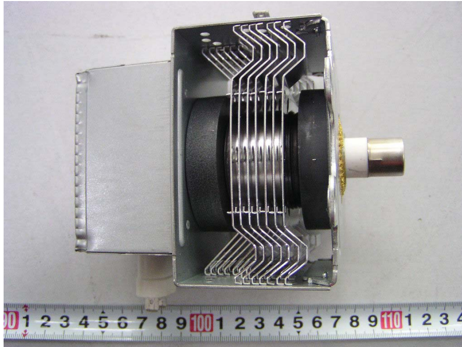
EUT-Magnetron Right View
