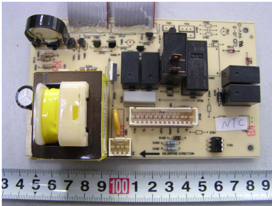
EUT-Control Unit Power PCB Top View
