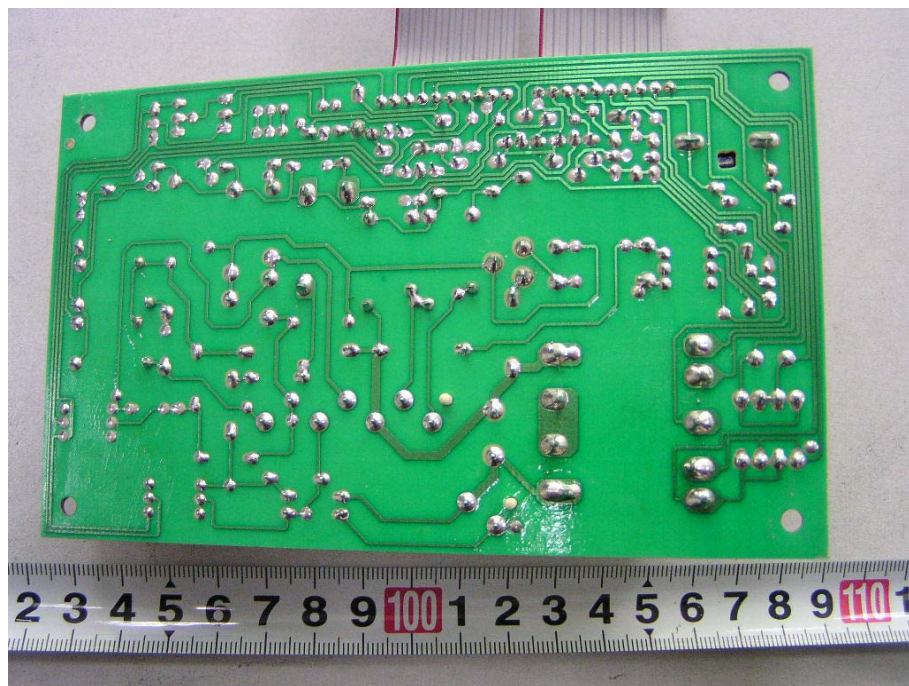
EUT-Control Unit Power PCB Bottom View
