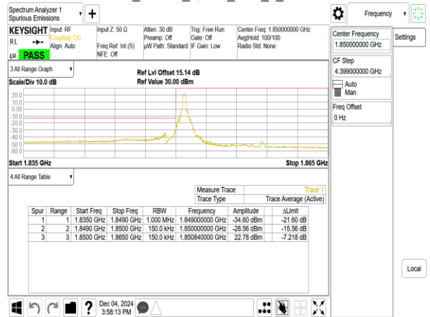
Band2_15MHz_QPSK_RB75_0_CH18675
