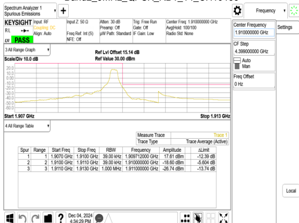
Band2_3MHz_QPSK_RB15_0_CH19185
