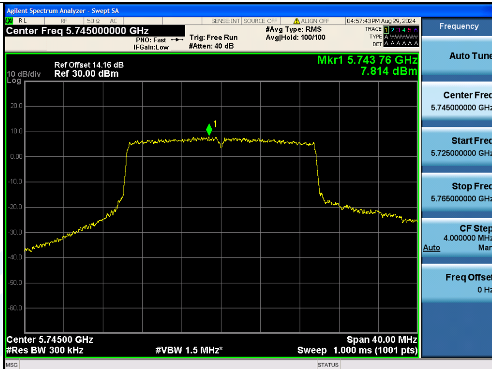
11AX20MIMO-Ant2-5745-PASS
