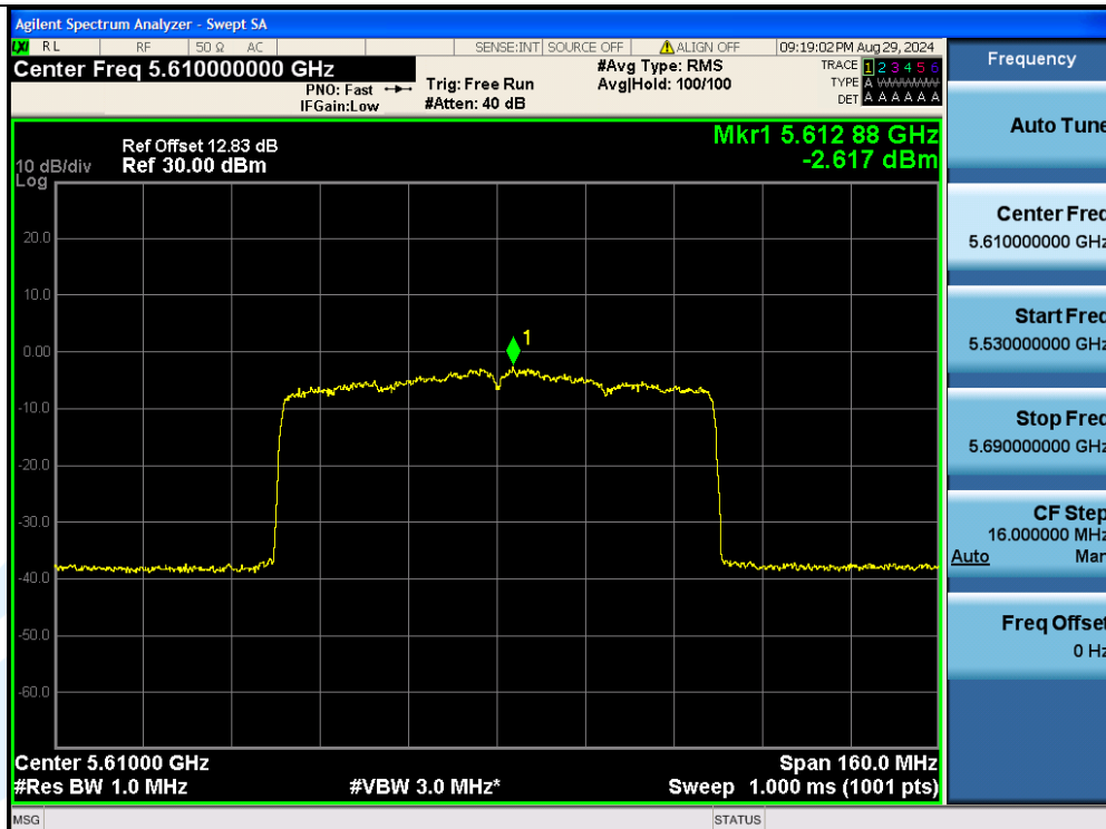
11AX80MIMO-Ant2-5610-PASS
