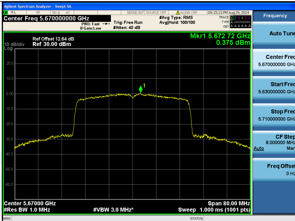
11AX40MIMO-Ant2-5670-PASS
