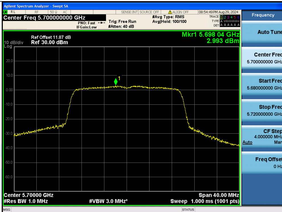
11AX20MIMO-Ant2-5700-PASS
