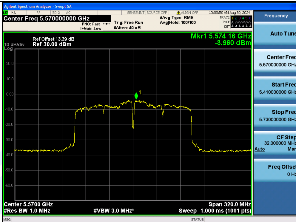
11AC160MIMO-Ant1-5570-PASS
