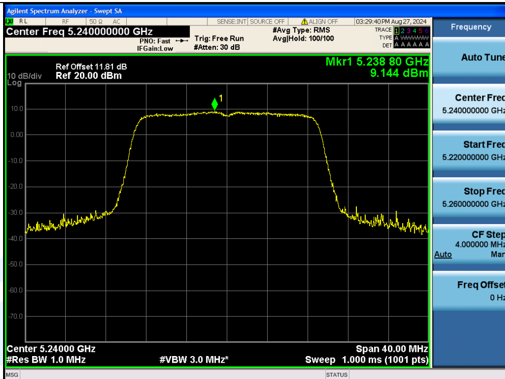
11N20MIMO-Ant3-5240-PASS
