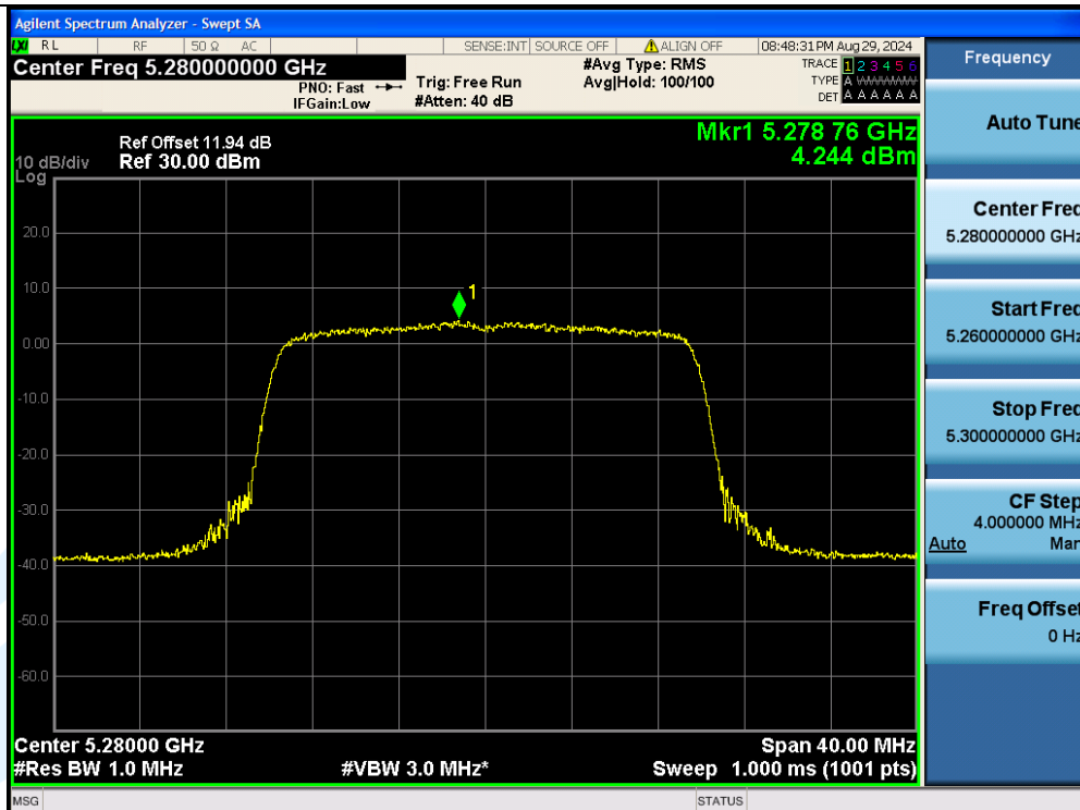
11AX20MIMO-Ant2-5280-PASS
