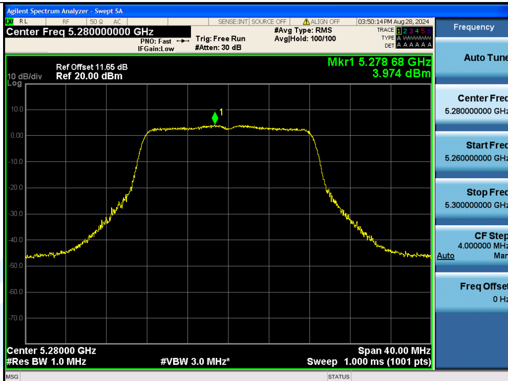
11A-Ant3-5280-PASS
