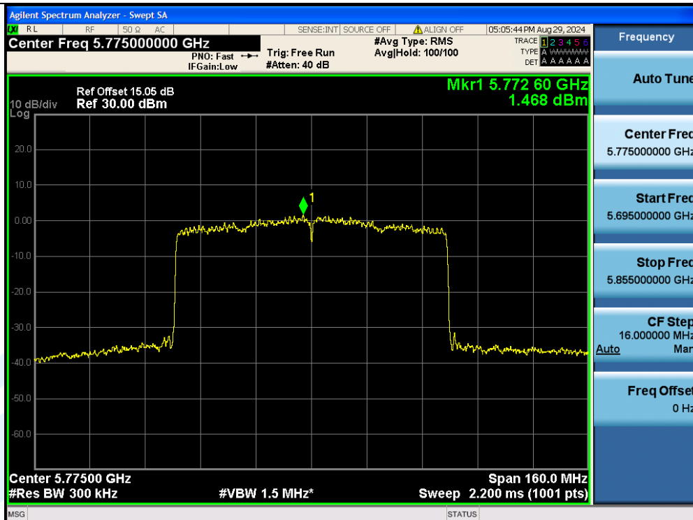
11AX80MIMO-Ant2-5775-PASS
