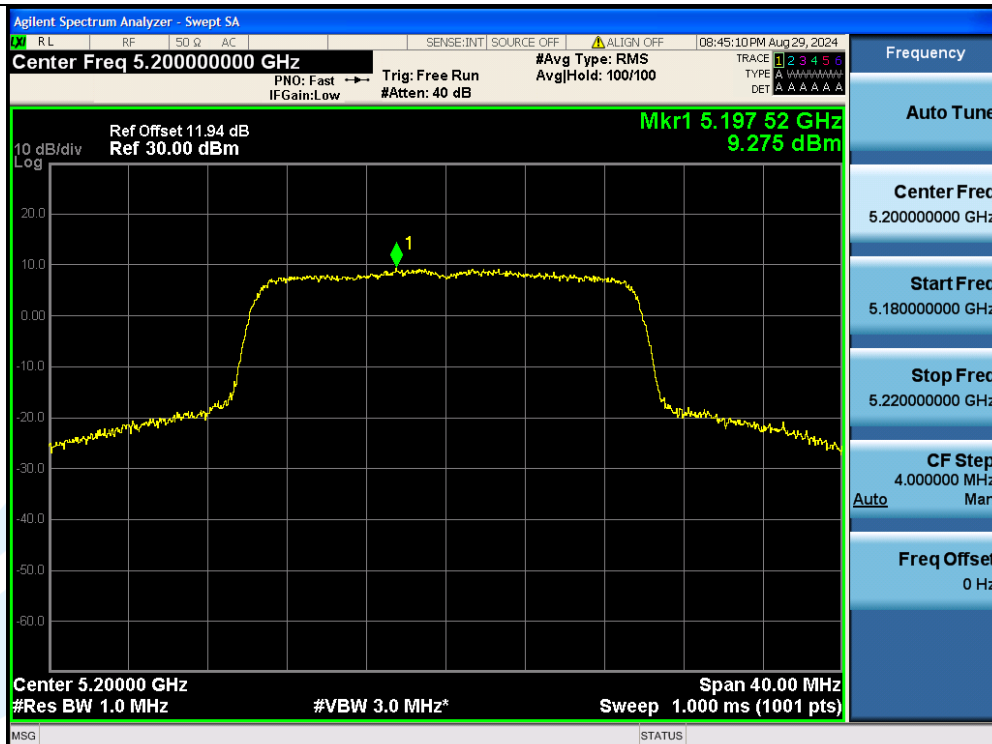
11AX20MIMO-Ant2-5200-PASS
