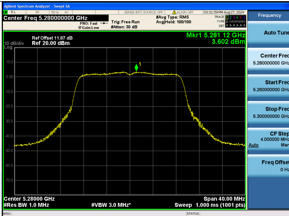
11N20MIMO-Ant3-5280-PASS
