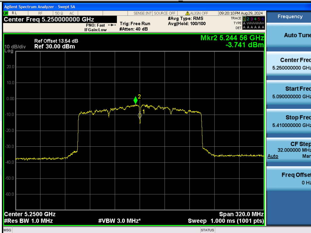
11AX160MIMO-Ant2-5250_UNII-2A-PASS
