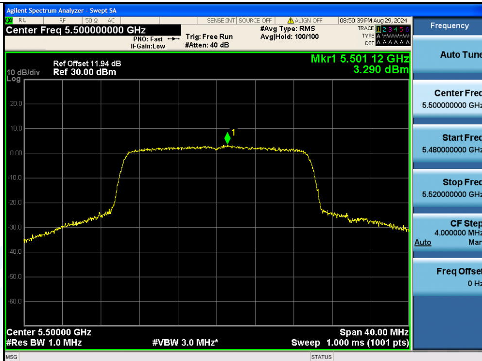
11AX20MIMO-Ant2-5500-PASS
