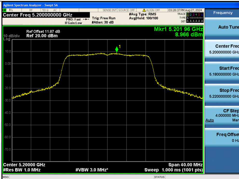
11N20MIMO-Ant3-5200-PASS
