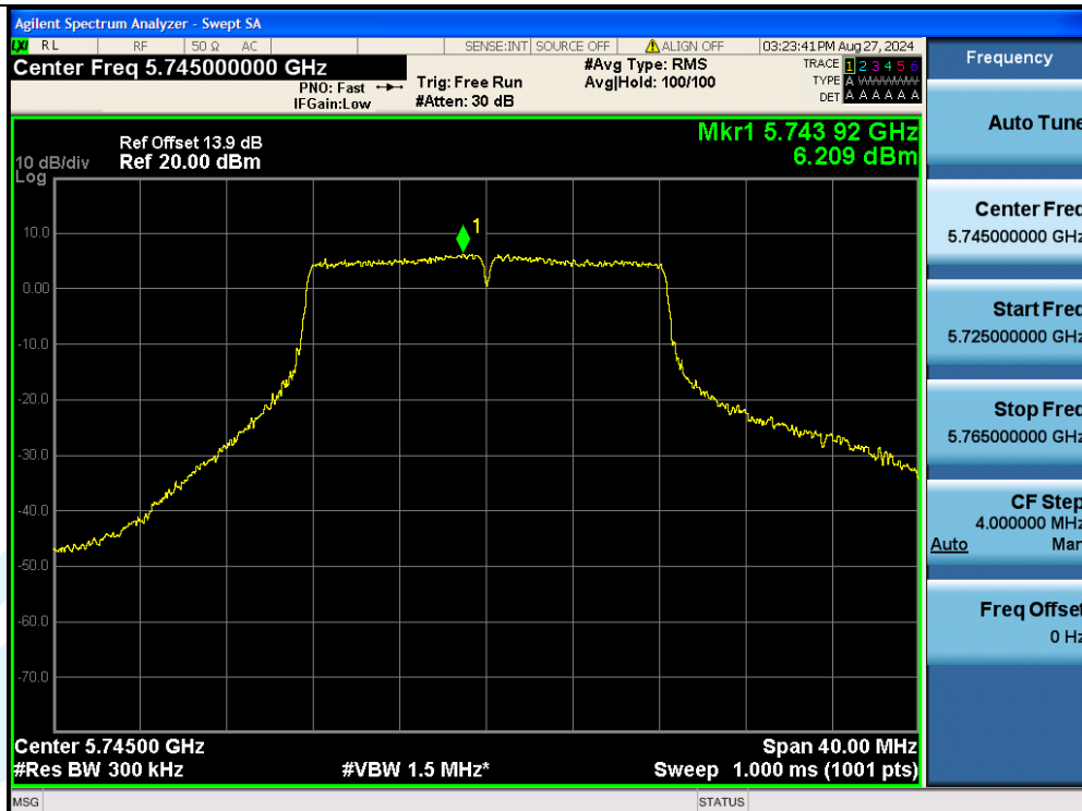
11A-Ant3-5745-PASS
