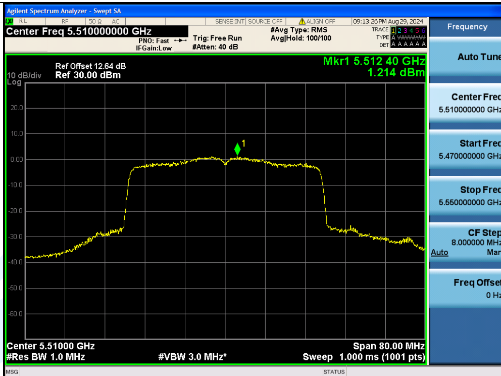
11AX40MIMO-Ant2-5510-PASS
