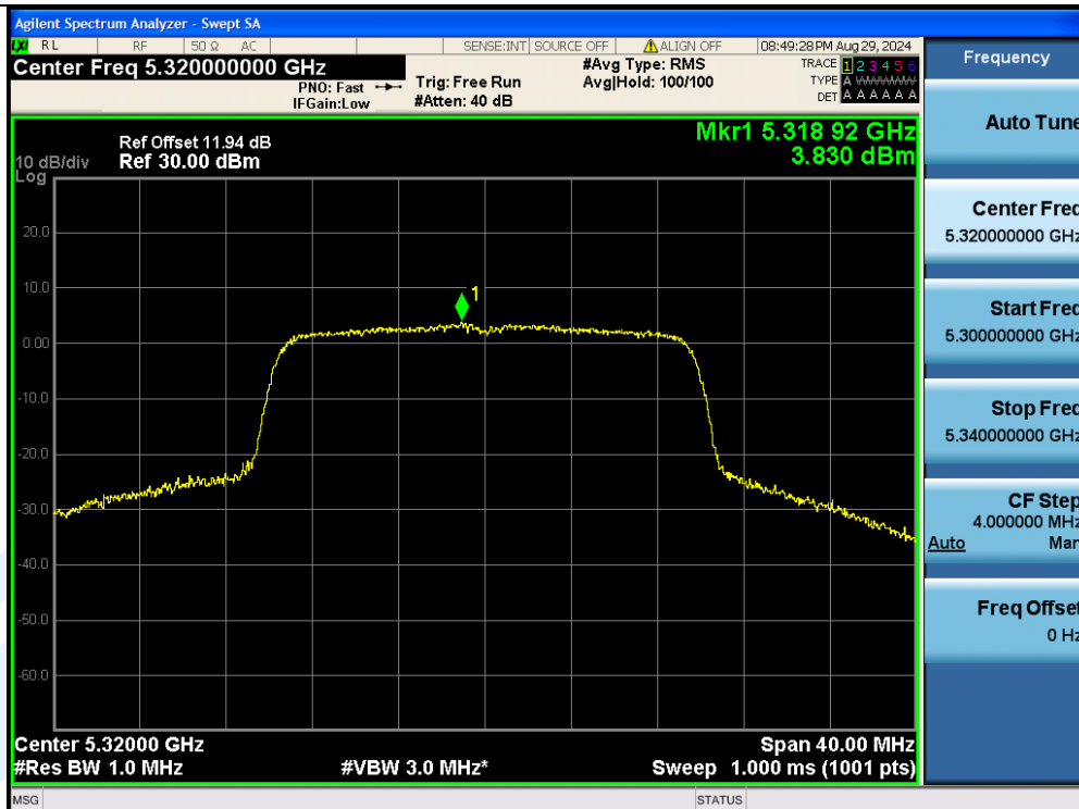
11AX20MIMO-Ant2-5320-PASS
