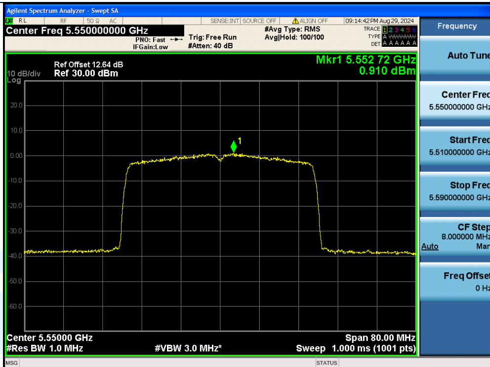
11AX40MIMO-Ant2-5550-PASS
