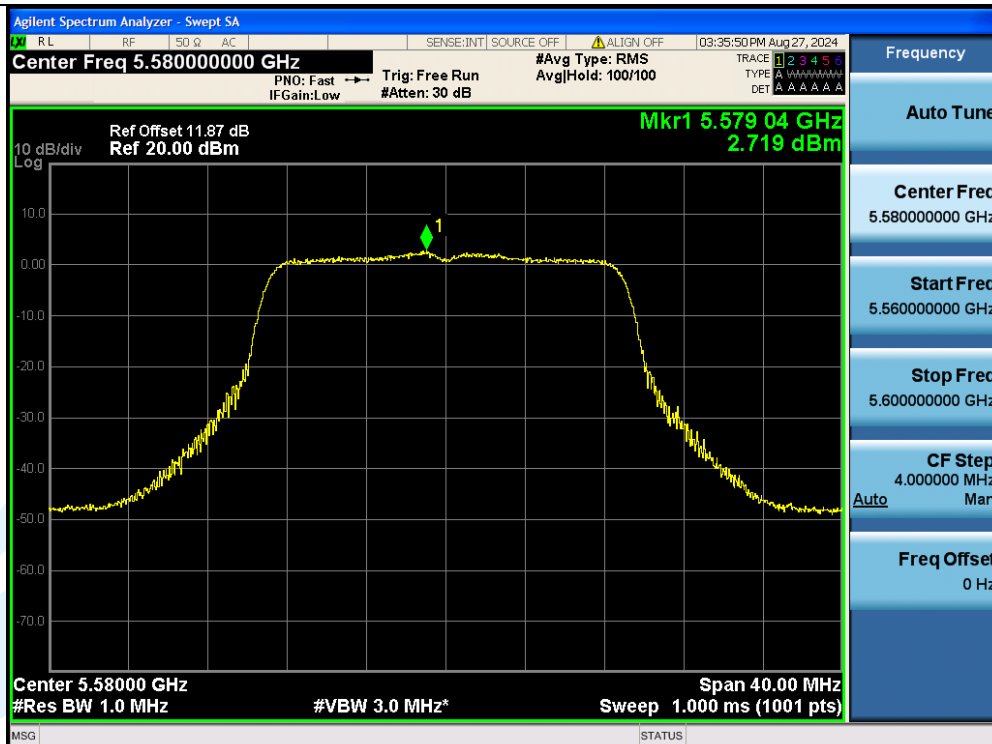
11N20MIMO-Ant3-5580-PASS
