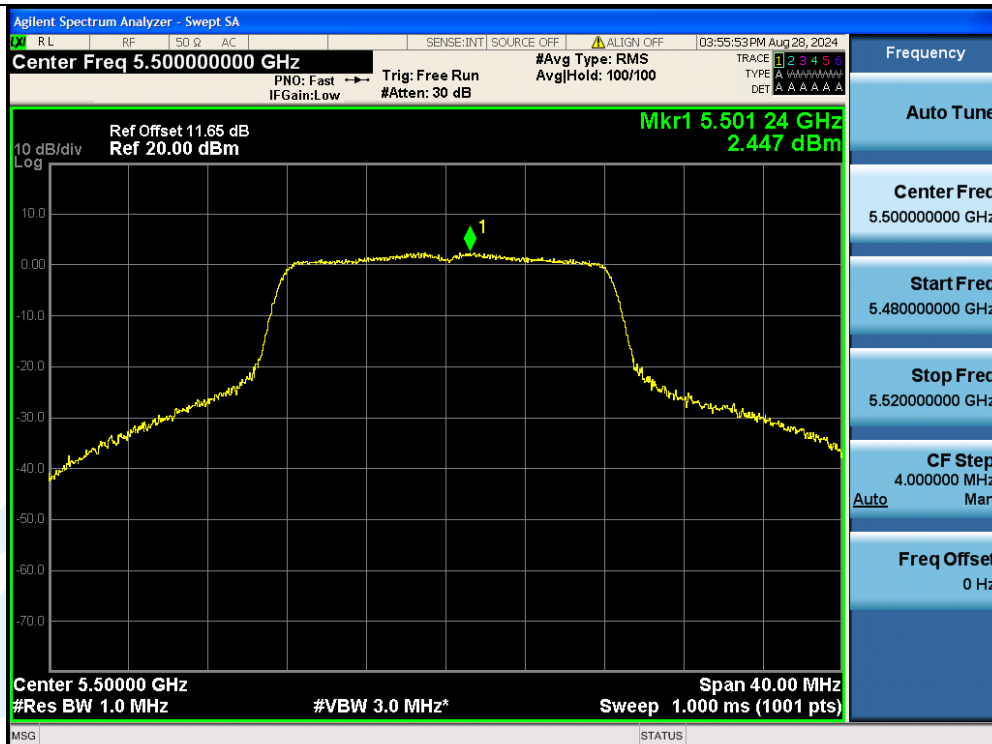
11A-Ant3-5500-PASS
