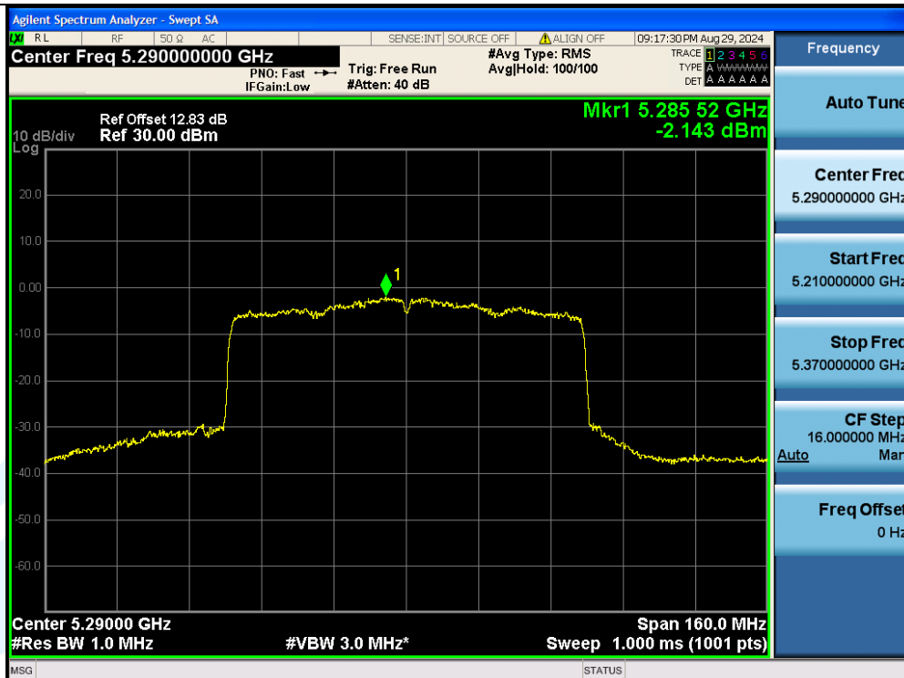
11AX80MIMO-Ant2-5290-PASS
