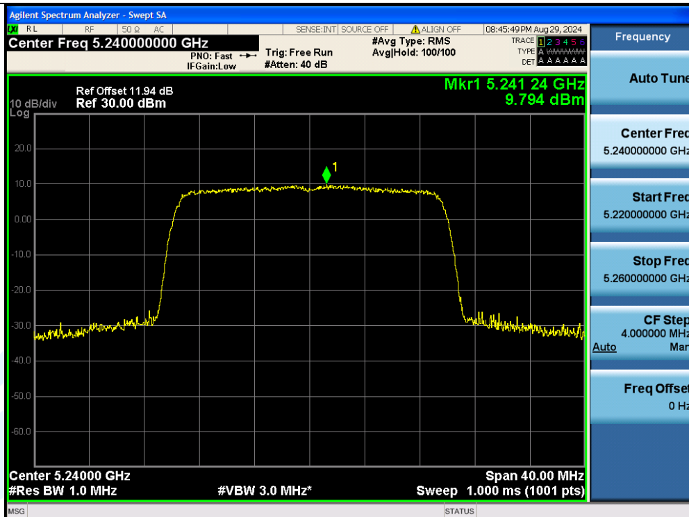
11AX20MIMO-Ant2-5240-PASS
