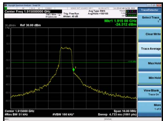
LTE Band 25 1.4MHz 16QAM 100%RB CH-High
