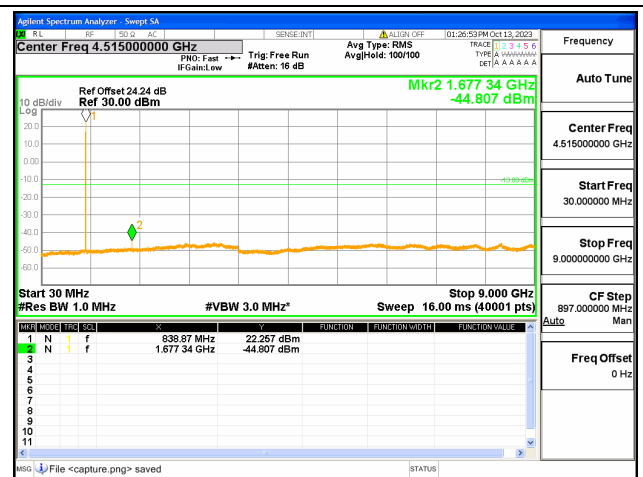
5B / 10+5MHz / QPSK / Mid CH / 1#49-1#0
