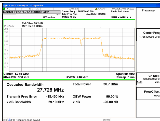
66C / 20+10MHz / 64QAM/ High CH
