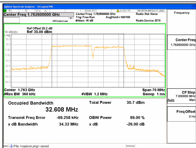
66C / 20+15MHz / 64QAM/ High CH
