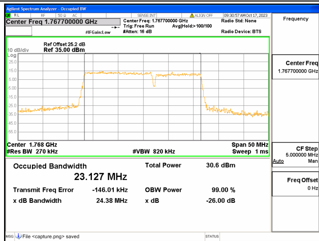
66C / 15+10MHz / 64QAM/ High CH
