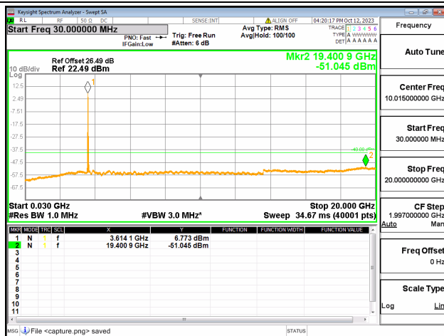
48C-30M-20G / 20+5MHz / QPSK / Mid CH / 1#0-1#24
