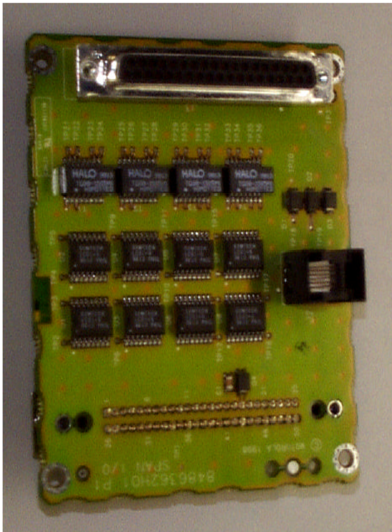
IHET5BL1 SC4812T @ 800MHz Span I/O Back
