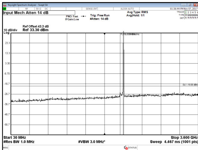
Figure 8.2-107: Conducted spurious emissions within 30–3600 MHz, Port C, LTE, 2 carriers: 5 MHz each at the top of the band, QPSK
