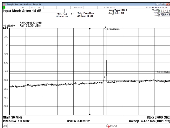
Figure 8.2-135: Conducted spurious emissions within 30–3600 MHz, Port B, LTE, 2 carriers: 15 MHz each at the top of the band, QPSK
