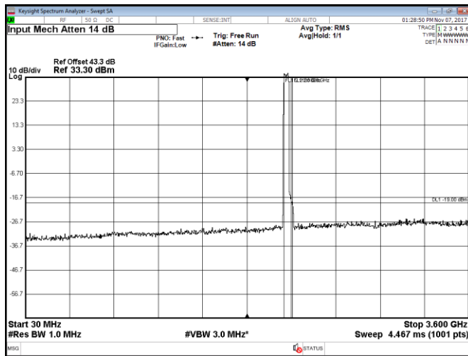
Figure 8.2-157: Conducted spurious emissions within 30–3600 MHz, Port D, LTE, 2 carriers: 20 MHz each at the bottom of the band, QPSK
