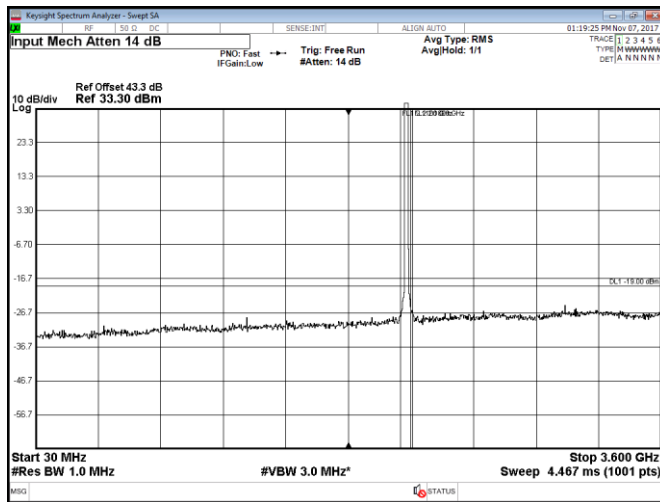
Figure 8.2-93: Conducted spurious emissions within 30–3600 MHz, Port D, LTE, 20 MHz mid channel, QPSK
