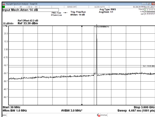
Figure 8.2-111: Conducted spurious emissions within 30–3600 MHz, Port D, LTE, 2 carriers: 5 MHz each at the top of the band, QPSK
