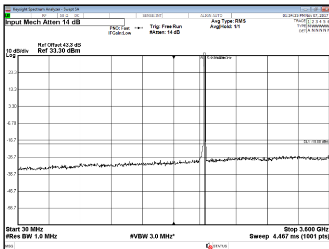
Figure 8.2-115: Conducted spurious emissions within 30–3600 MHz, Port A, LTE, 2 carriers: 10 MHz each at the top of the band, QPSK
