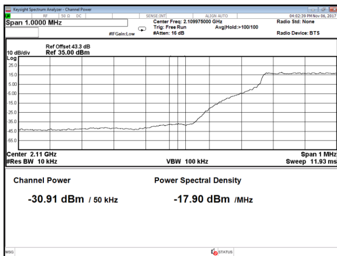
Figure 8.2-195: Conducted band edge emission at 2110 MHz, Port B, LTE, 5 MHz channel, 2 bottom carriers, QPSK (RBW = 1% of EBW)
