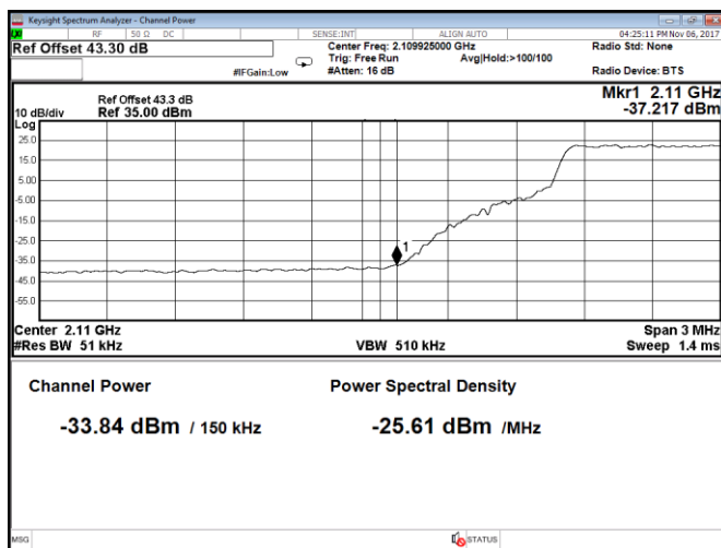
Figure 8.2-179: Conducted band edge emission at 2110 MHz, Port B, LTE, 15 MHz channel, QPSK (RBW = 1% of EBW)
