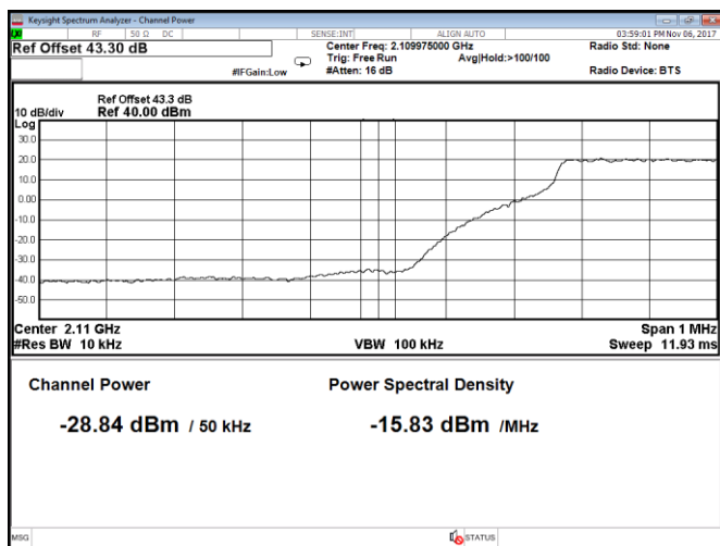
Figure 8.2-163: Conducted band edge emission at 2110 MHz, Port B, LTE, 5 MHz channel, QPSK (RBW = 1% of EBW)
