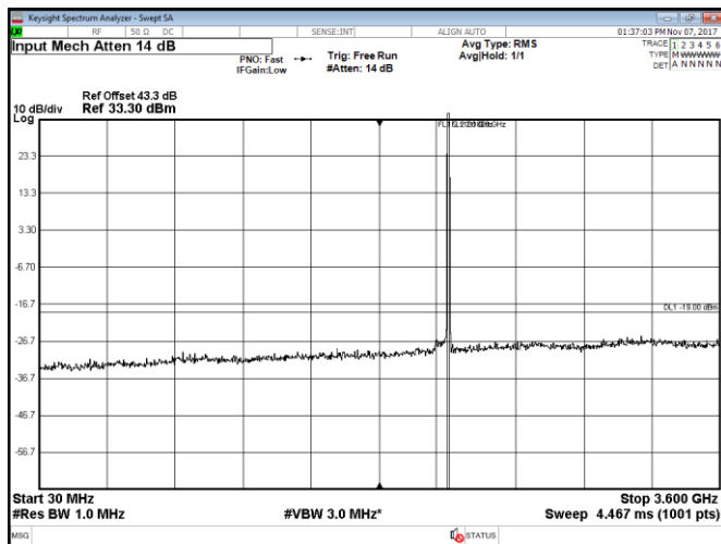
Figure 8.2-99: Conducted spurious emissions within 30–3600 MHz, Port A, LTE, 2 carriers: 5 MHz each at the top of the band, QPSK
