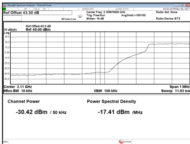
Figure 8.2-199: Conducted band edge emission at 2110 MHz, Port D, LTE, 5 MHz channel, 2 bottom carriers, QPSK (RBW = 1% of EBW)
