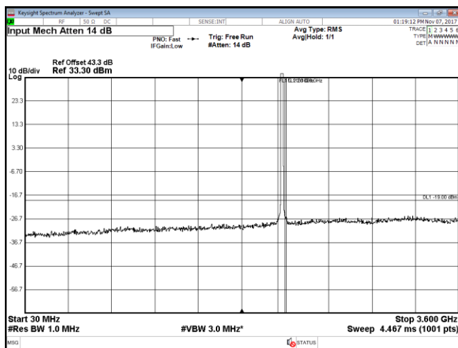
Figure 8.2-87: Conducted spurious emissions within 30–3600 MHz, Port C, LTE, 20 MHz mid channel, QPSK
