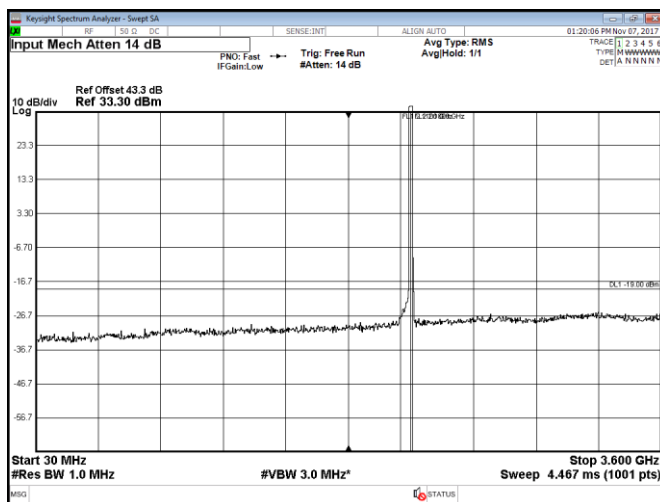
Figure 8.2-95: Conducted spurious emissions within 30–3600 MHz, Port D, LTE, 20 MHz high channel, QPSK
