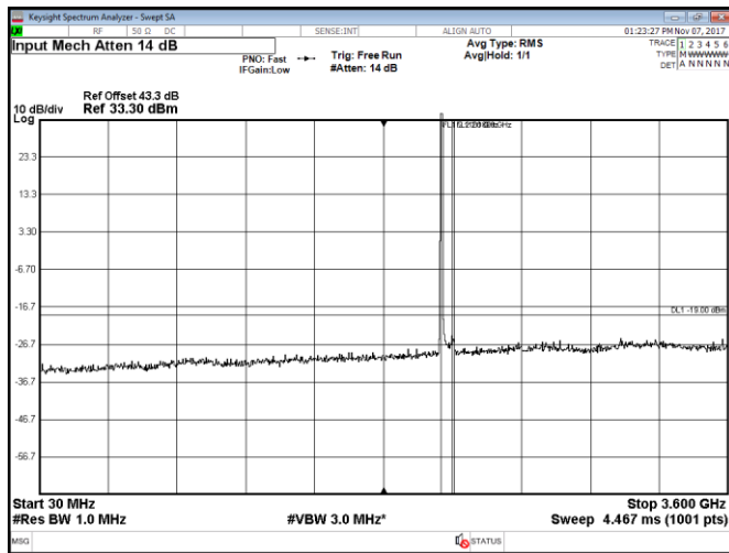
Figure 8.2-97: Conducted spurious emissions within 30–3600 MHz, Port A, LTE, 2 carriers: 5 MHz each at the bottom of the band, QPSK
