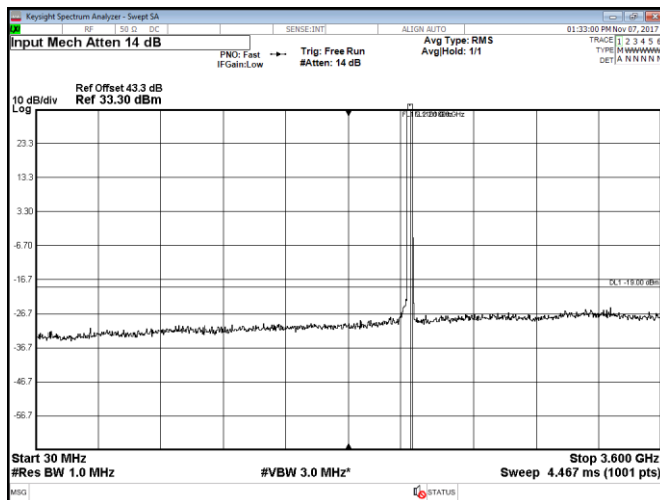
Figure 8.2-131: Conducted spurious emissions within 30–3600 MHz, Port A, LTE, 2 carriers: 15 MHz each at the top of the band, QPSK
