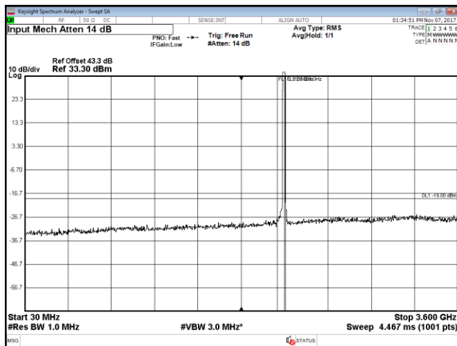
Figure 8.2-119: Conducted spurious emissions within 30–3600 MHz, Port B, LTE, 2 carriers: 10 MHz each at the top of the band, QPSK
