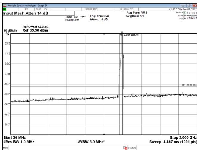
Figure 8.2-143: Conducted spurious emissions within 30–3600 MHz, Port D, LTE, 2 carriers: 15 MHz each at the top of the band, QPSK
