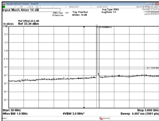
Figure 8.2-85: Conducted spurious emissions within 30–3600 MHz, Port C, LTE, 20 MHz low channel, QPSK
