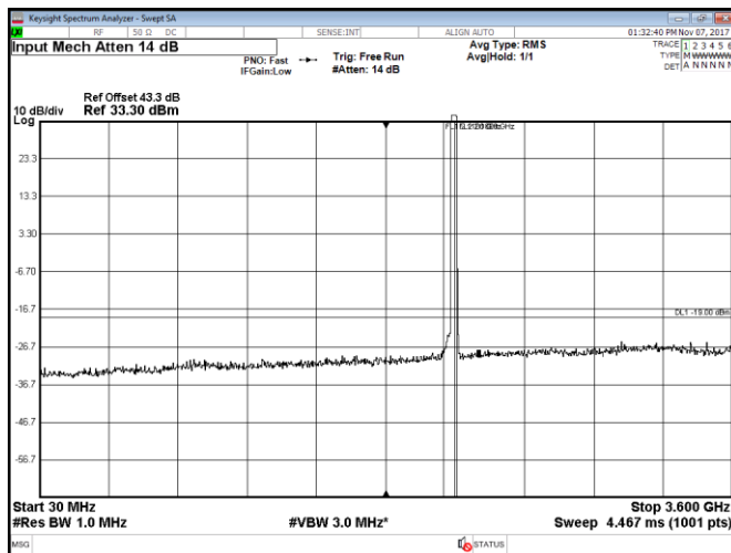
Figure 8.2-139: Conducted spurious emissions within 30–3600 MHz, Port C, LTE, 2 carriers: 15 MHz each at the top of the band, QPSK
