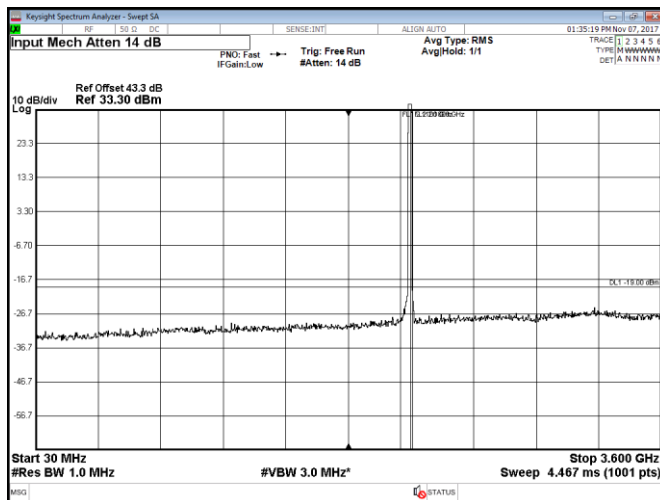
Figure 8.2-127: Conducted spurious emissions within 30–3600 MHz, Port D, LTE, 2 carriers: 10 MHz each at the top of the band, QPSK
