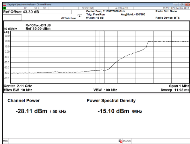
Figure 8.2-161: Conducted band edge emission at 2110 MHz, Port A, LTE, 5 MHz channel, QPSK (RBW = 1% of EBW)
