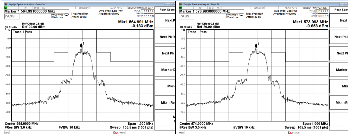
Channel 0 / 565 MHz
