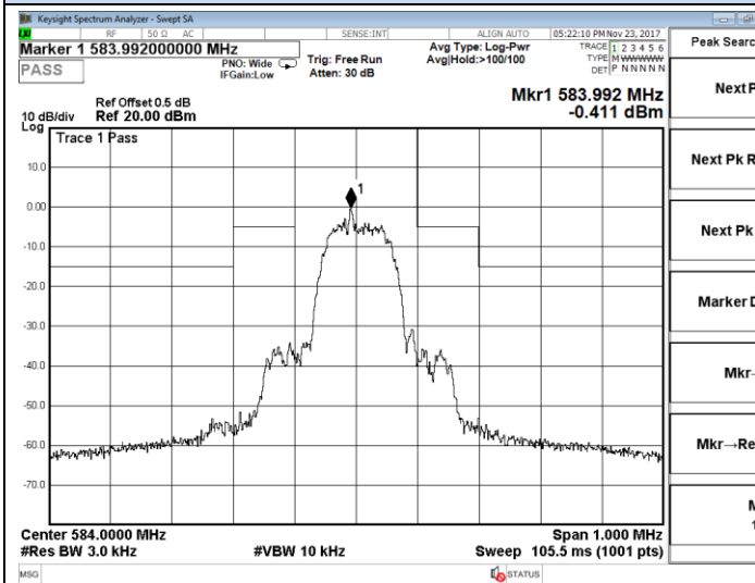
Channel 19 / 584 MHz
