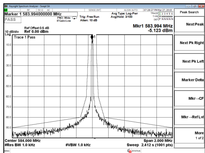
Channel 19 / 584 MHz
