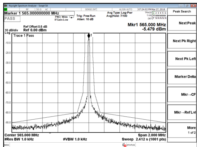
Channel 0 / 565 MHz
