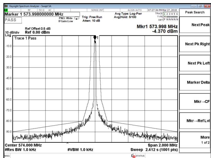
Channel 09 / 574 MHz
