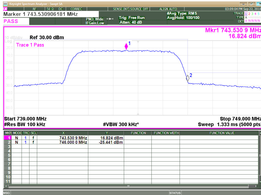
Plot 3.4.3: Band Edge test results, AWGN 4.1MHz, F_c = 743.5 MHz, single test signal
