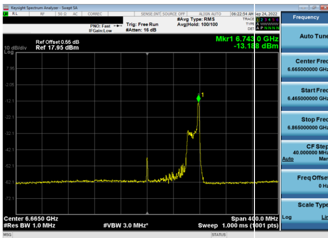
Plot 7-349. Power Spectral Density Plot SDM Antenna WF5t (160MHz 802.11ax RU26 (UNII Band 7) – Ch. 143)
