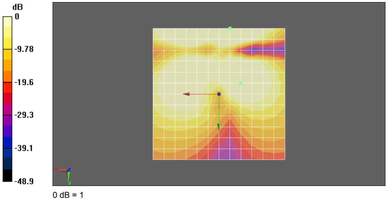
Figure 17 T-Coil GSM 1900 Y transversal
