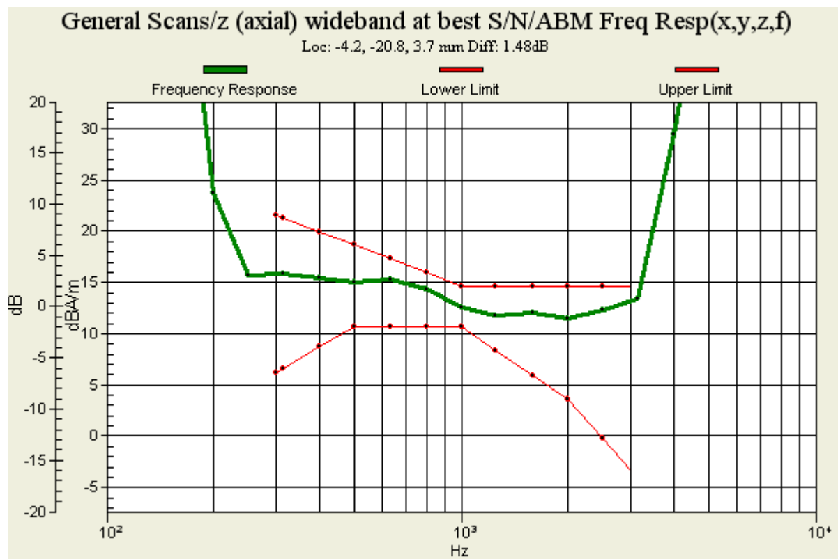
Figure 26 T-Coil WCDMA Band IV Z Axial
