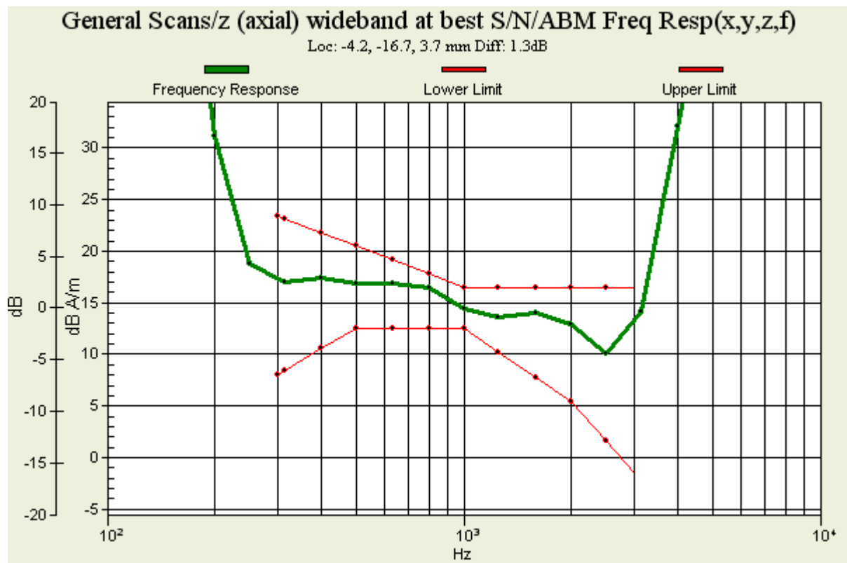
Figure 14 T-Coil GSM 850 Z Axial
