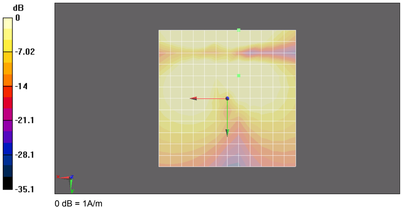
Figure 27 T-Coil WCDMA Band V Y transversal
