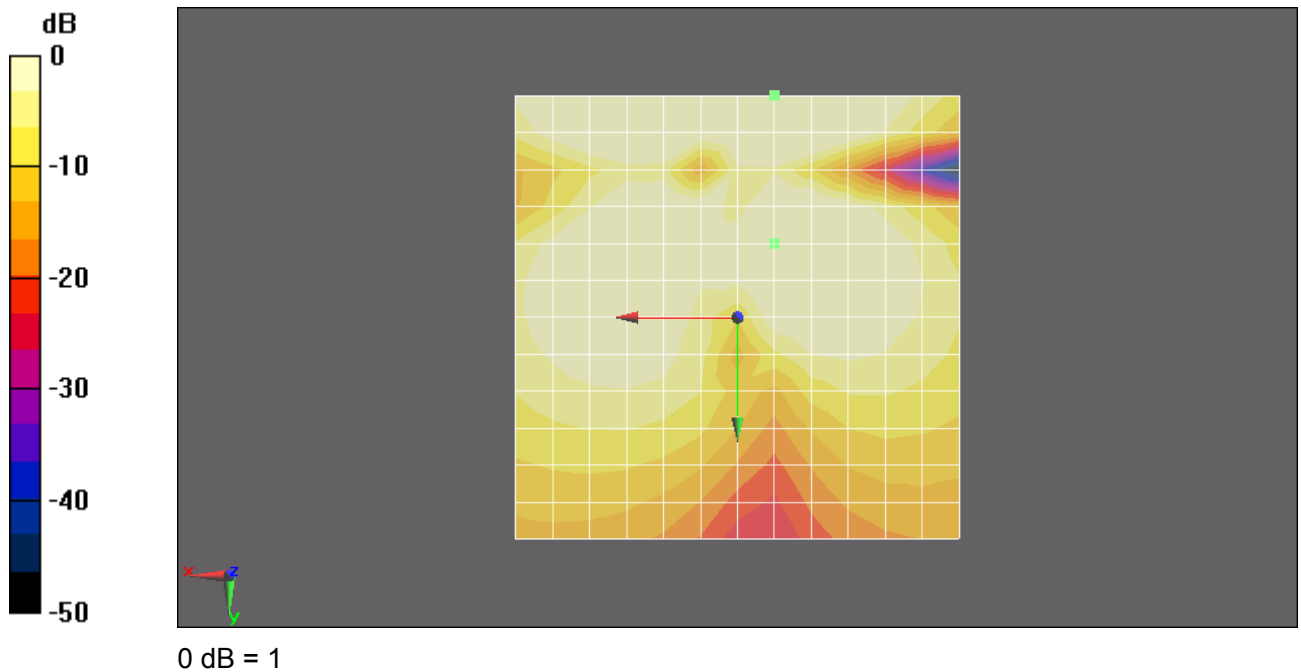
Figure 21 T-Coil WCDMA Band II Y transversal
