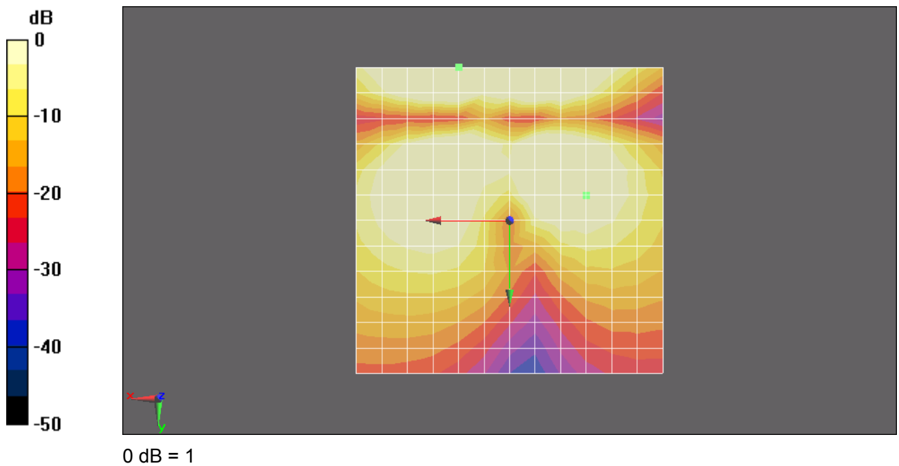
Figure 11 T-Coil GSM 850 Y transversal
