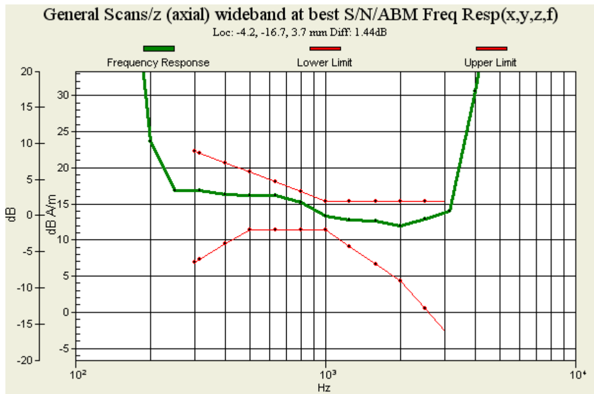
Figure 30 T-Coil WCDMA Band V Z Axial
