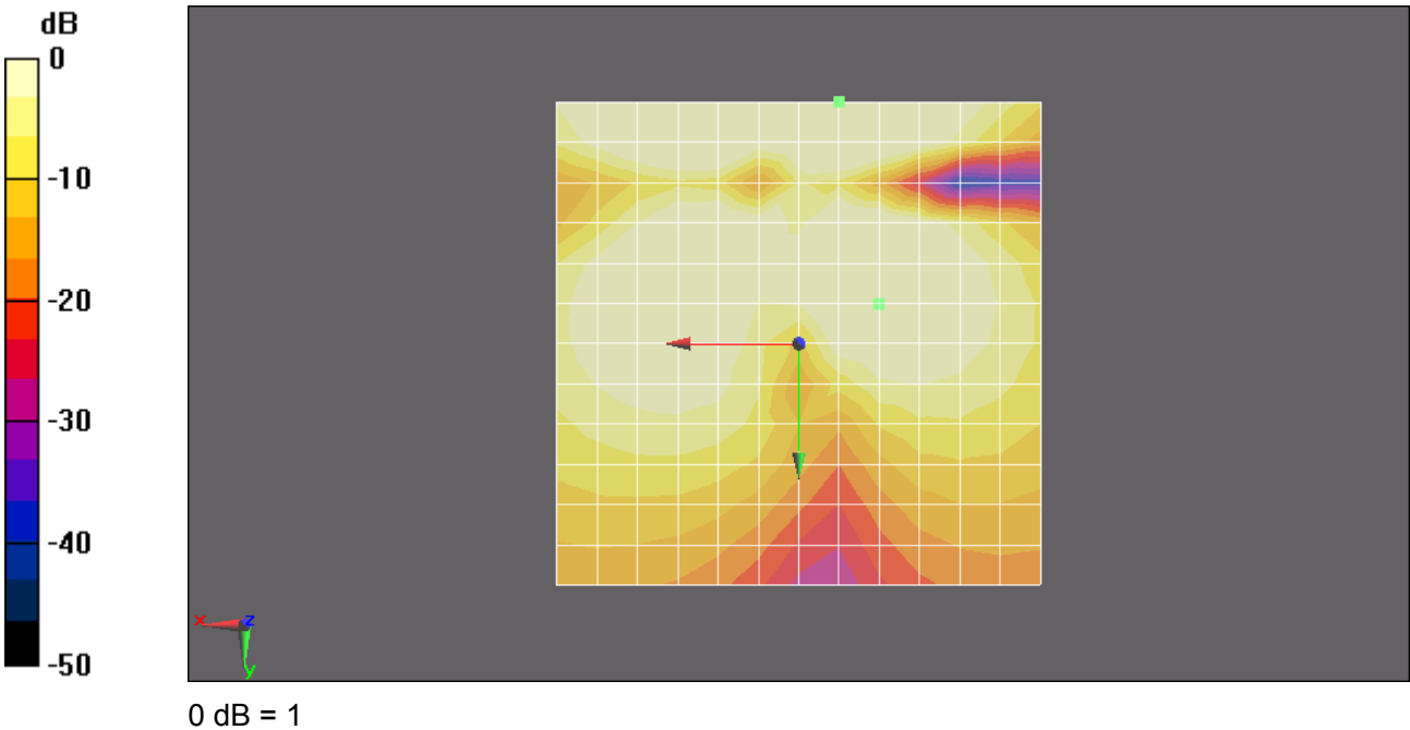
Figure 13 T-Coil GSM 850 Y transversal
