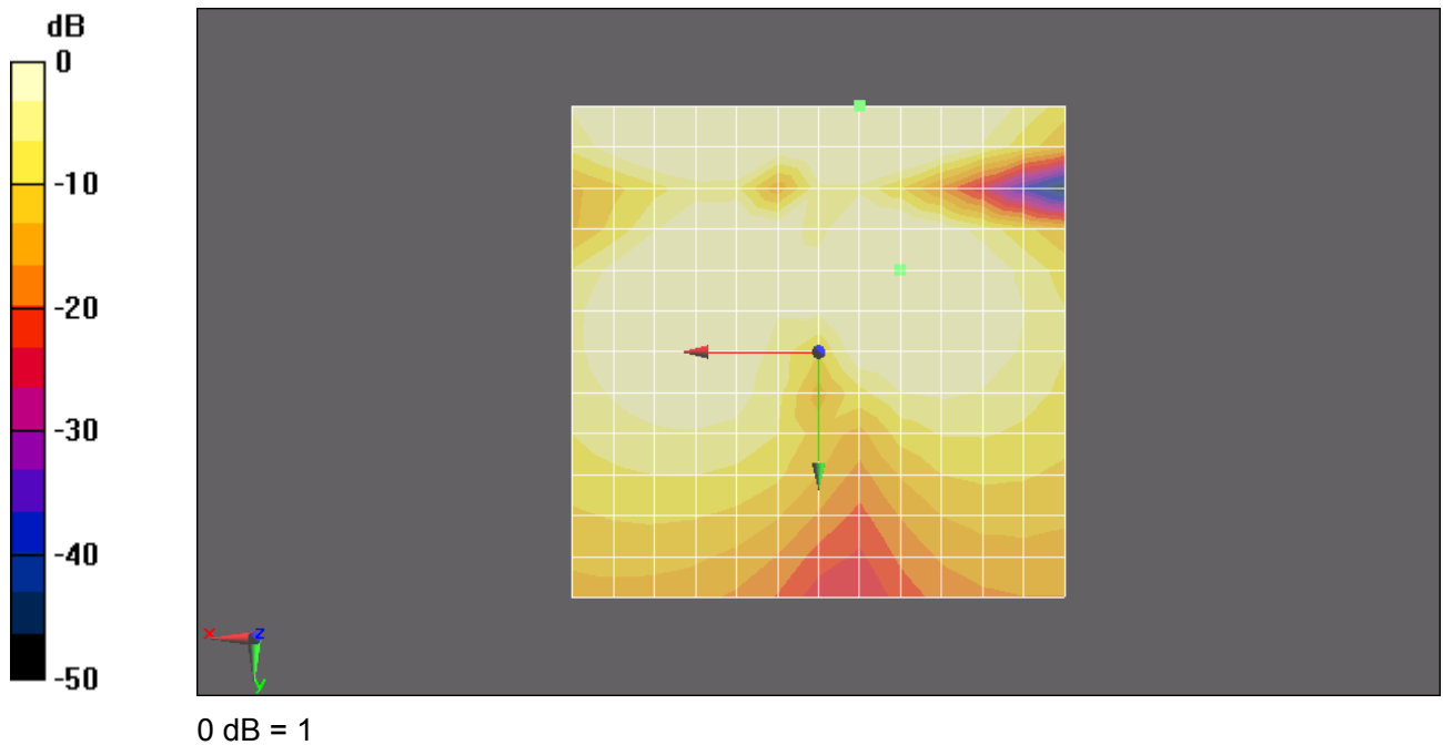
Figure 19 T-Coil WCDMA Band II Y transversal
