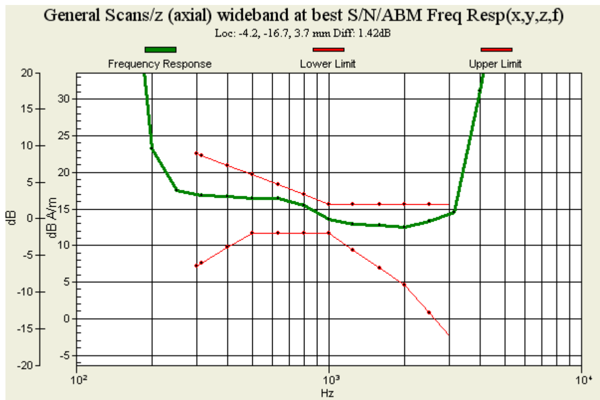
Figure 28 T-Coil WCDMA Band V Z Axial
