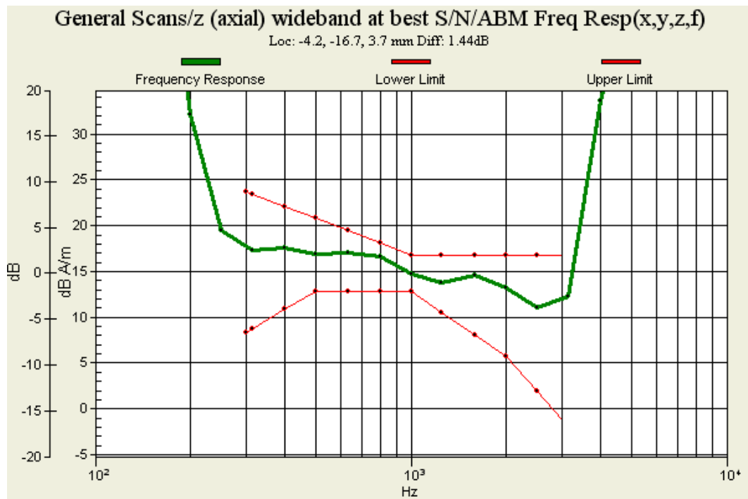
Figure 18 T-Coil GSM 1900 Z Axial
