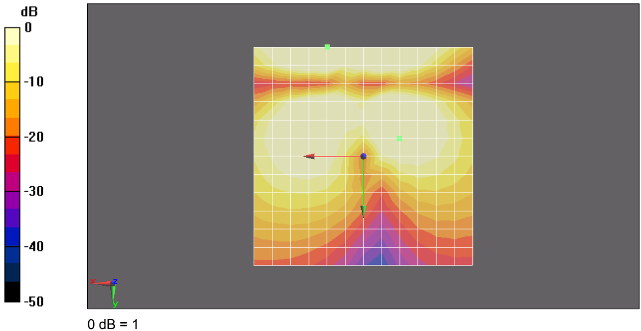
Figure 15 T-Coil GSM 1900 Y transversal
