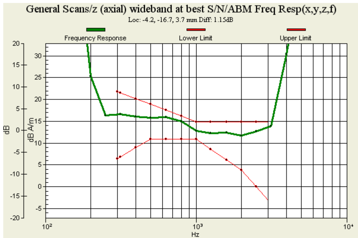
Figure 20 T-Coil WCDMA Band II Z Axial
