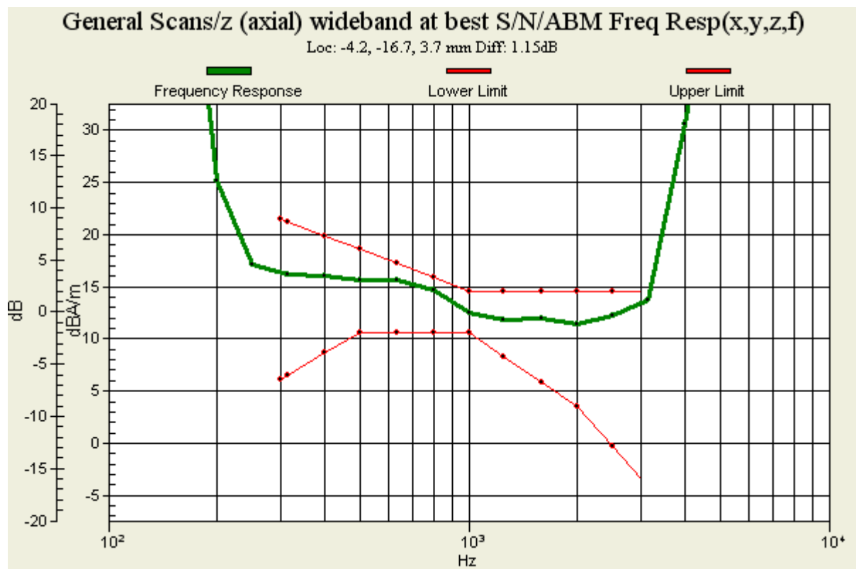
Figure 24 T-Coil WCDMA Band IV Z Axial
