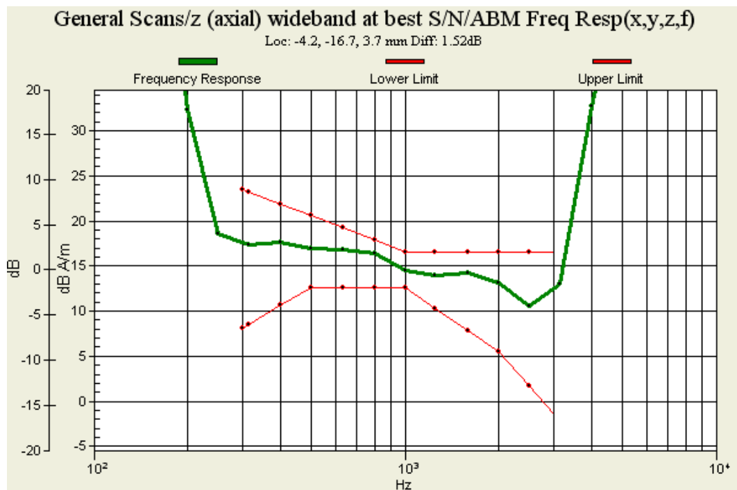
Figure 12 T-Coil GSM 850 Z Axial
