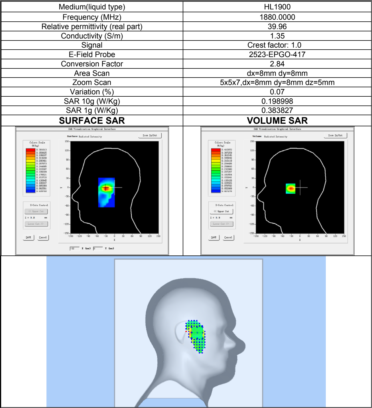
Plot 5: WCDMA BAND II, Middle channel (Left Head Cheek) Product Description: Smart Phone Test Date: 2024-10-12
