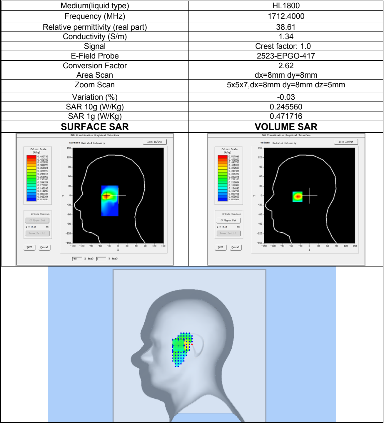
Plot 7: WCDMA BAND IV, Low channel (Right Head Cheek) Product Description: Smart Phone Test Date: 2024-10-21
