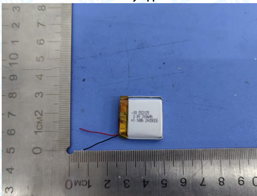
Photo 10 Battery Appearance
