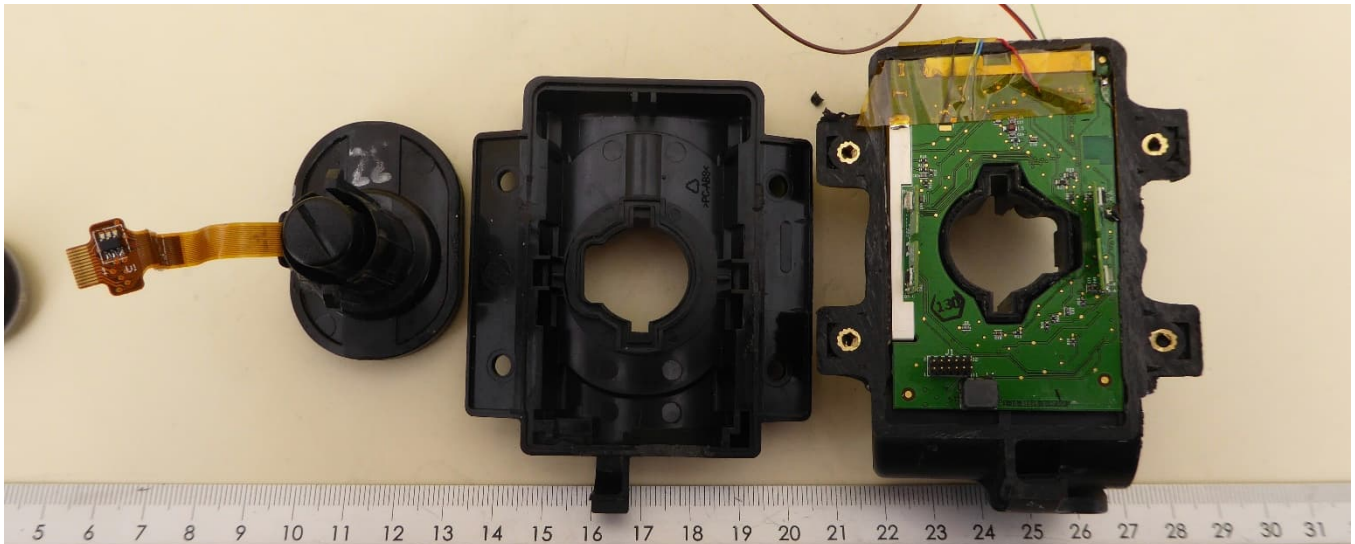
EUT opened
