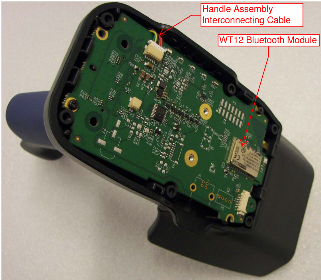
Top Cover Removed
