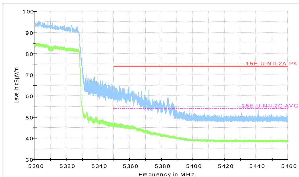
Fig.53 Band Edges (802.11ac-HT80 Ch58, 5290MHz)
