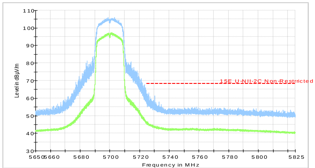
Fig.47 Band Edges (802.11ac-HT20 Ch140, 5700MHz)
