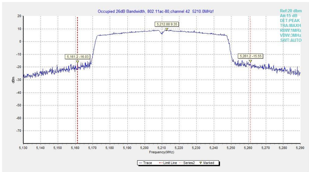
Fig.28 Occupied 26dB Bandwidth (802. 11ac-HT80, 5210MHz)
