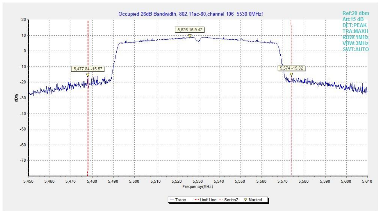
Fig.30 Occupied 26dB Bandwidth (802. 11ac-HT80, 5530MHz)
