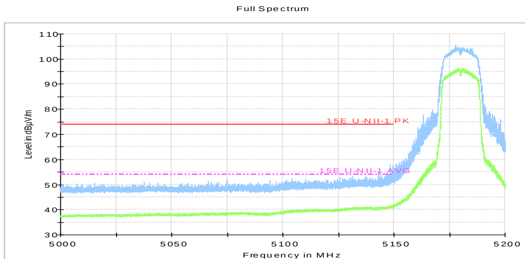
Fig.32 Band Edges (802.11a Ch36, 5180MHz)
