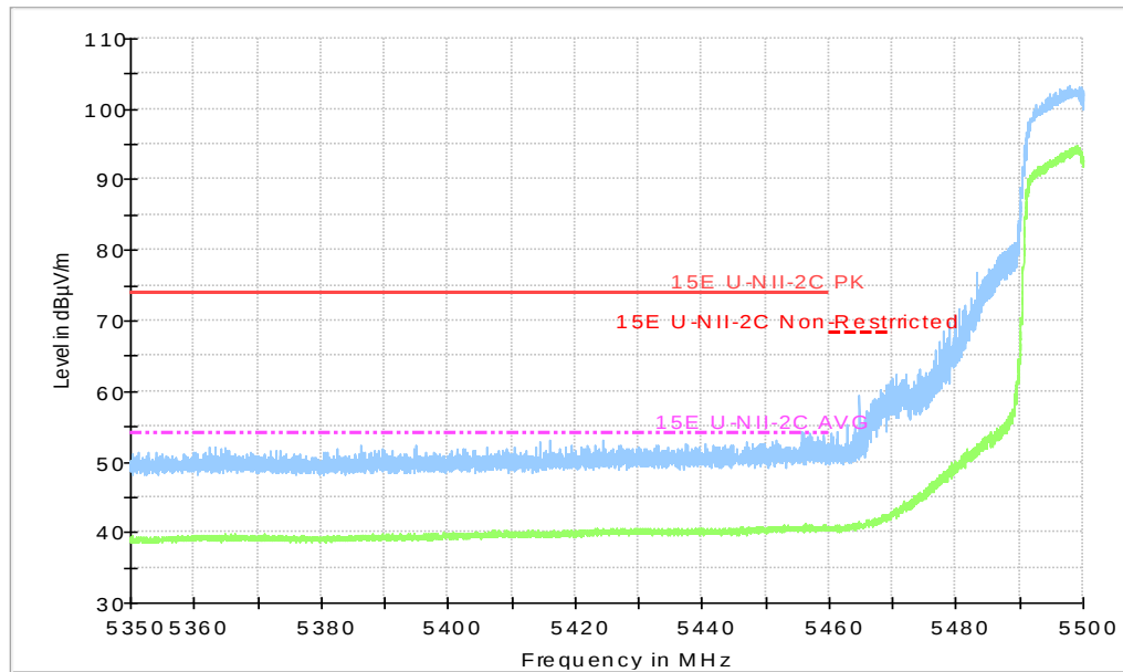
Fig.38 Band Edges (802.11n-HT20 Ch100, 5500MHz)
