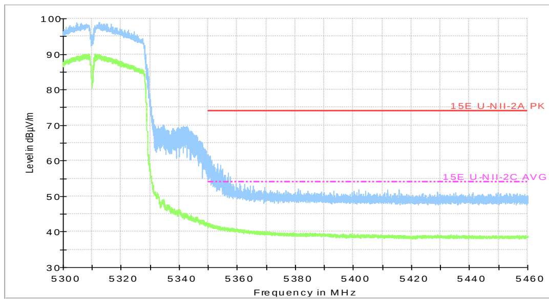
Fig.41 Band Edges (802.11n-HT40 Ch62, 5310MHz)
