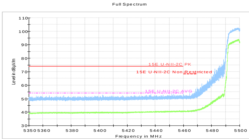
Fig.34 Band Edges (802.11a Ch100, 5500MHz)
