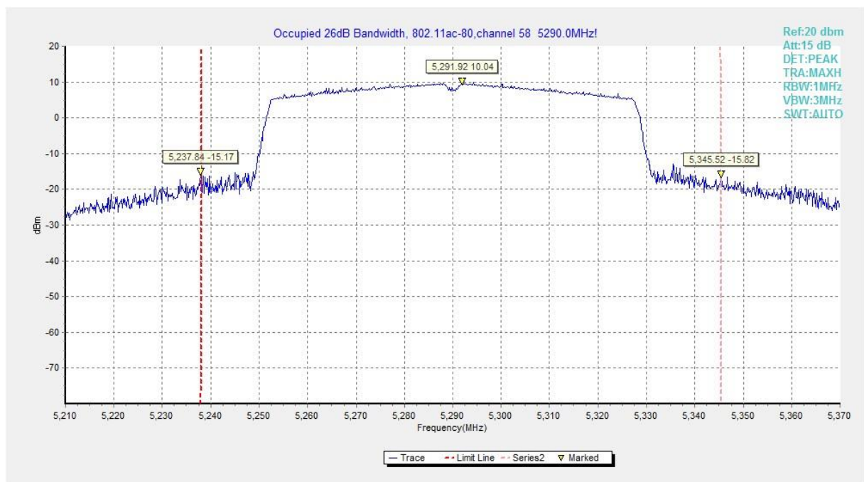
Fig.29 Occupied 26dB Bandwidth (802. 11ac-HT80, 5290MHz)
