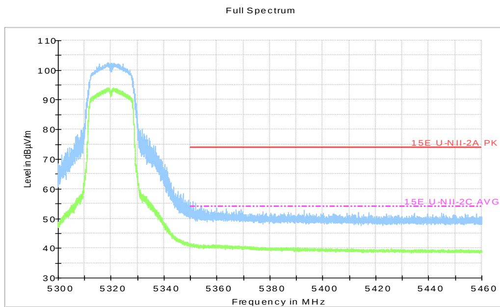
Fig.33 Band Edges (802.11a Ch64, 5320MHz)
