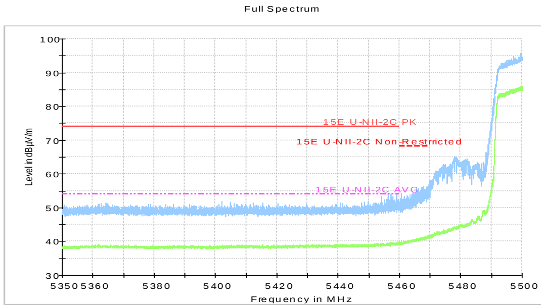
Fig.42 Band Edges (802.11n-HT40 Ch102, 5510MHz)
