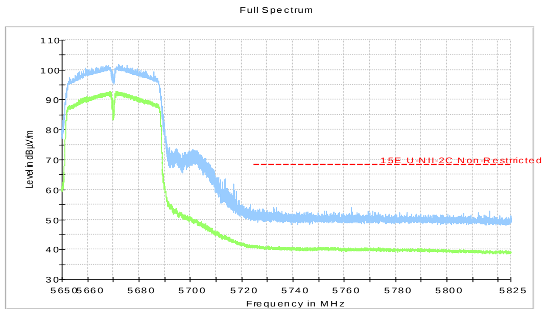
Fig.43 Band Edges (802.11n-HT40 Ch134, 5670MHz)
