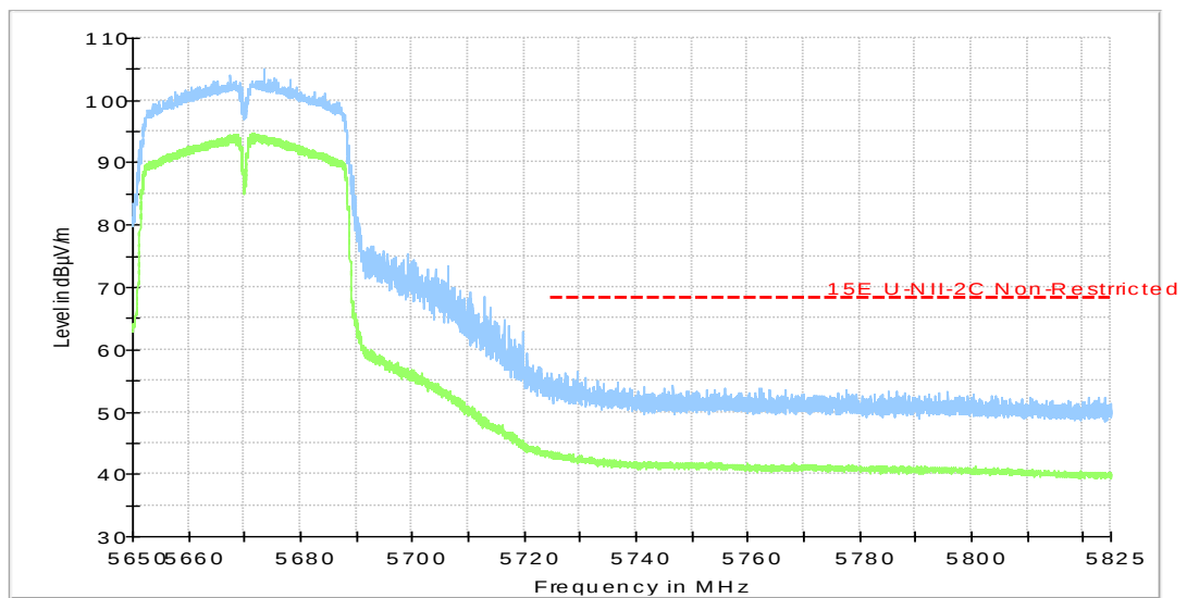
Fig.51 Band Edges (802.11ac-HT40 Ch134, 5670MHz)
