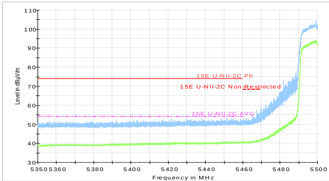
Fig.46 Band Edges (802.11ac-HT20 Ch100, 5500MHz)
