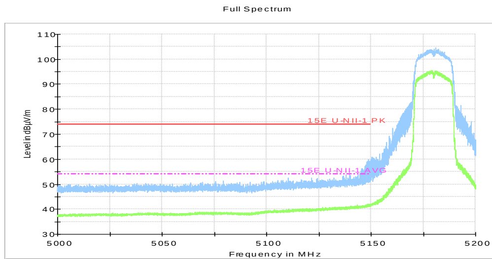
Fig.36 Band Edges (802.11n-HT20 Ch36, 5180MHz)
