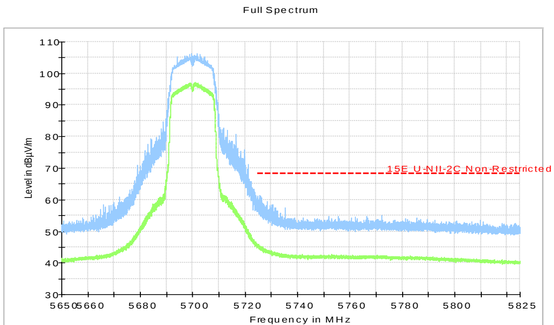
Fig.35 Band Edges (802.11a Ch140, 5700MHz)
