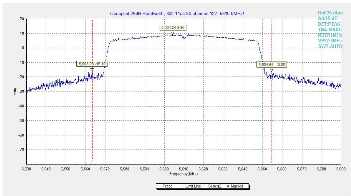
Fig.31 Occupied 26dB Bandwidth (802. 11ac-HT80, 5610MHz)
