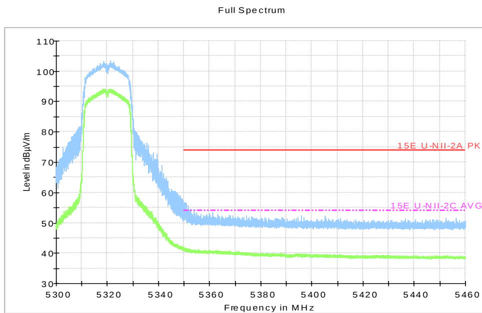
Fig.37 Band Edges (802.11n-HT20 Ch64, 5320MHz)
