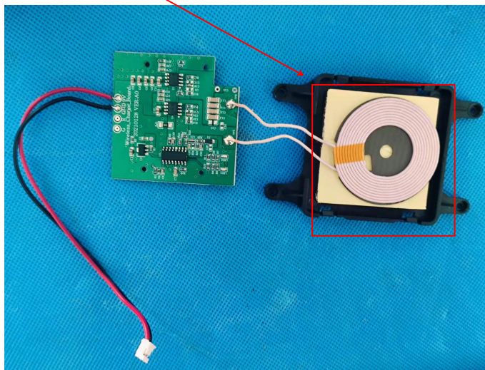
Coil Antenna
