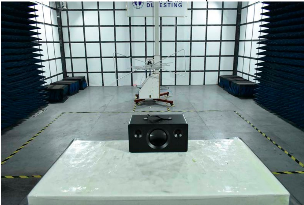
RadiatedEmission(Below 1G)
