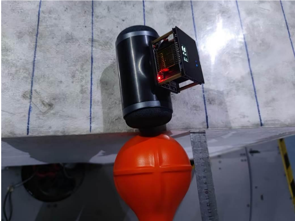
H-Field &amp; E-Field Strength_ Position F
