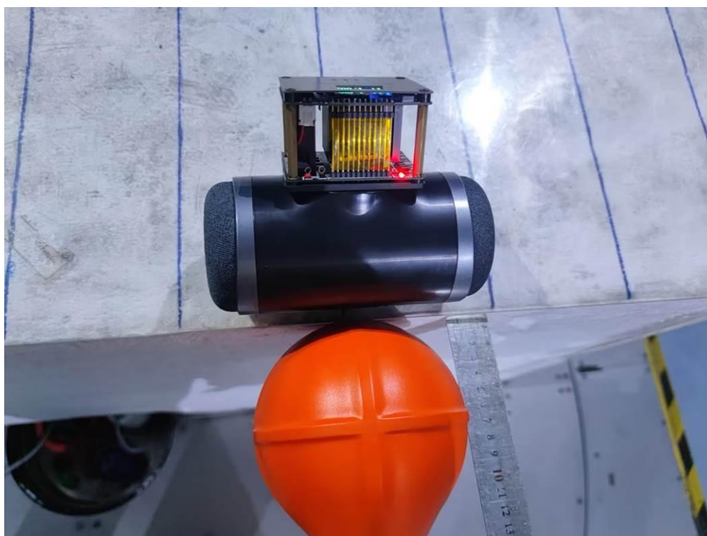
H-Field &amp; E-Field Strength_ Position D
