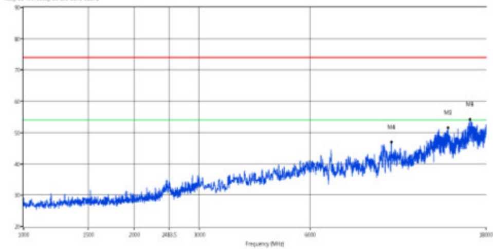
RSE_FCC Test Case_FCC 15C 1GHz-18GHz
