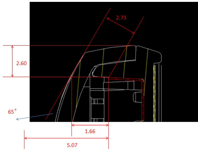
The device exterior radius dimension
