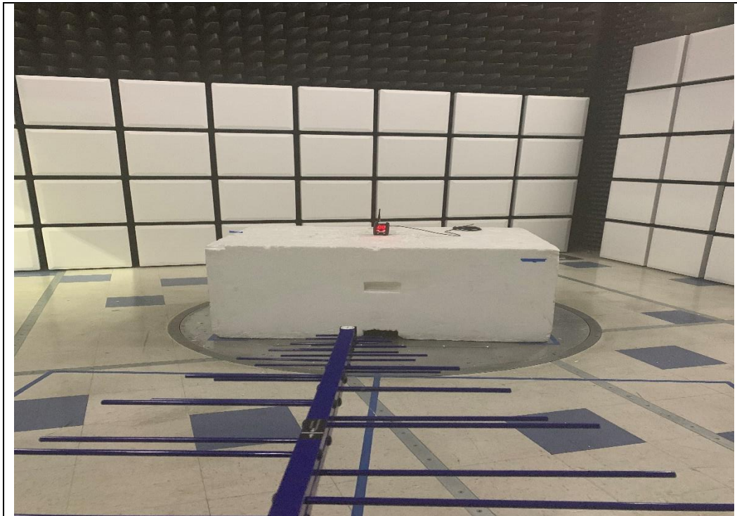
RF Radiated #2 1-18 GHz
