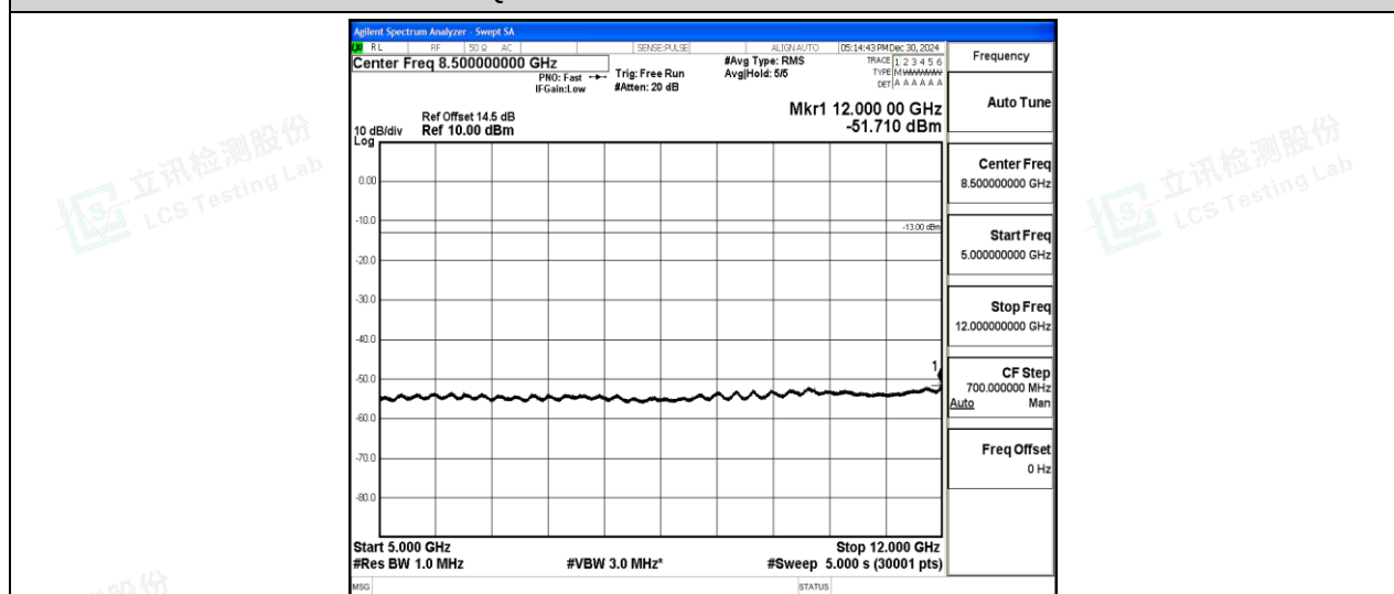
Band2-5MHz-QPSK-18900-1-0-Low-5000-12000--51.71-PASS
