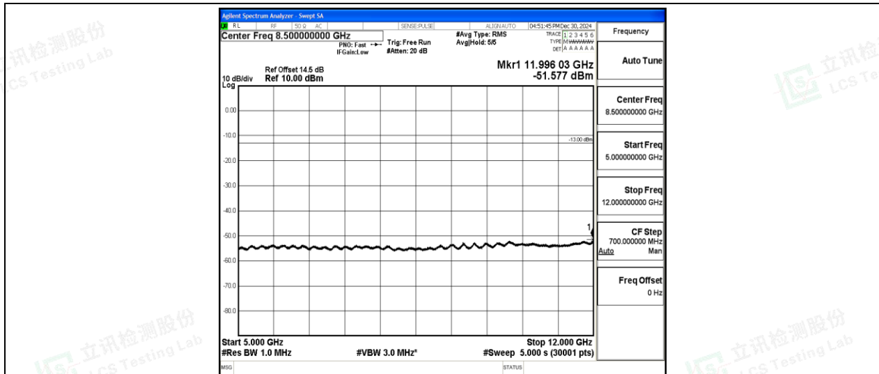
Band2-3MHz-QPSK-19185-1-0-High-5000-12000--51.58-PASS
