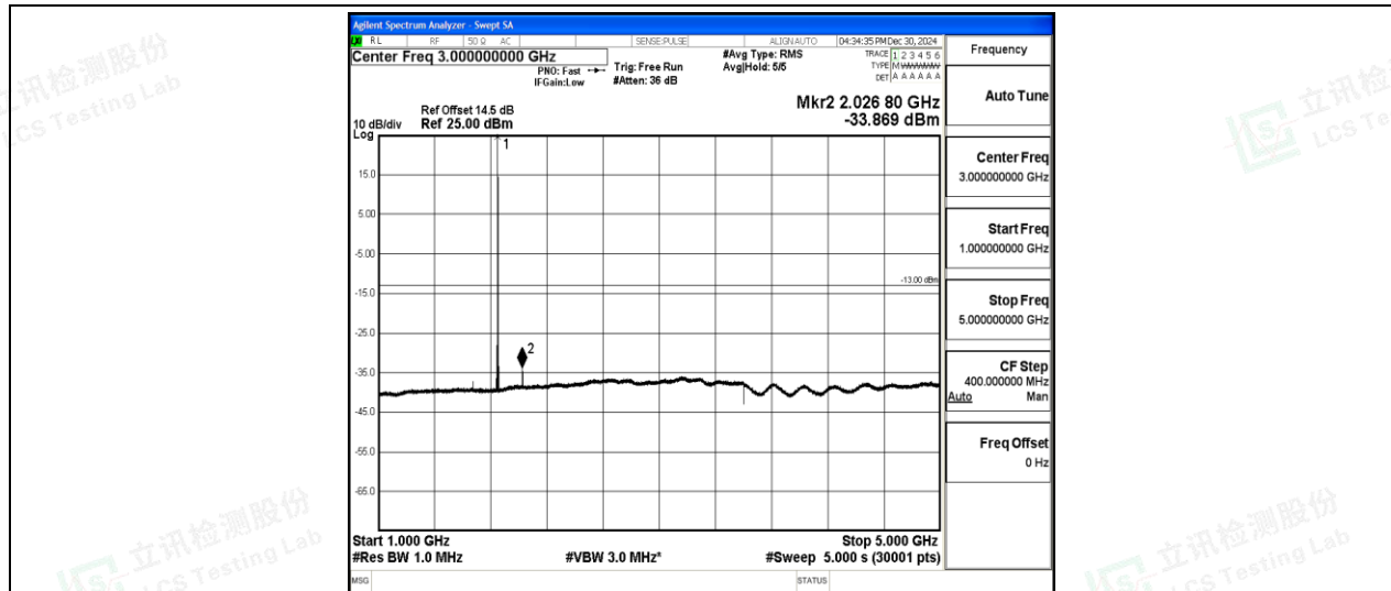
Band2-3MHz-16QAM-18615-1-0-Low-1000-5000--33.87-PASS
