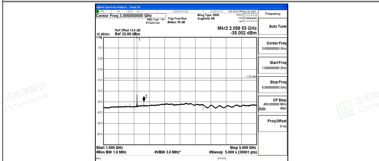
Band2-5MHz-16QAM-18900-1-0-Low-1000-5000--35-PASS
