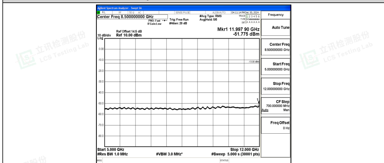
Band2-1.4MHz-16QAM-18900-1-0-Low-5000-12000--51.78-PASS
