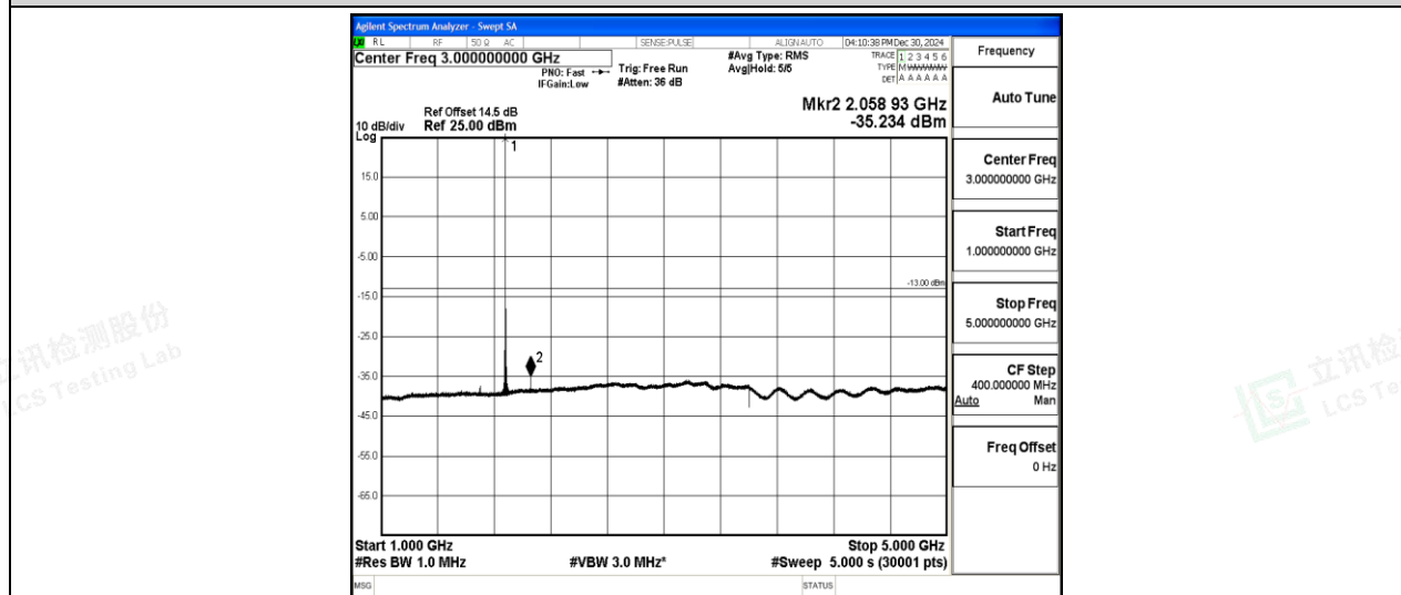
Band2-1.4MHz-16QAM-18900-1-0-Low-1000-5000--35.23-PASS
