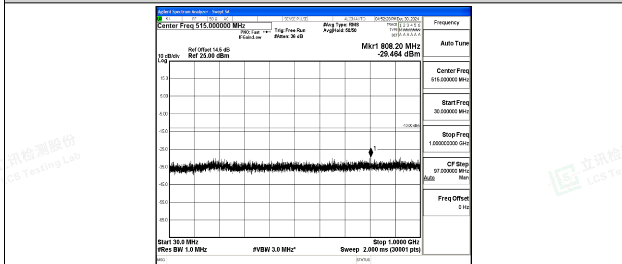
Band2-3MHz-16QAM-19185-1-0-High-30-1000--29.46-PASS
