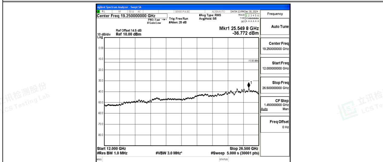
Band2-3MHz-16QAM-19185-1-0-High-12000-26500--36.77-PASS
