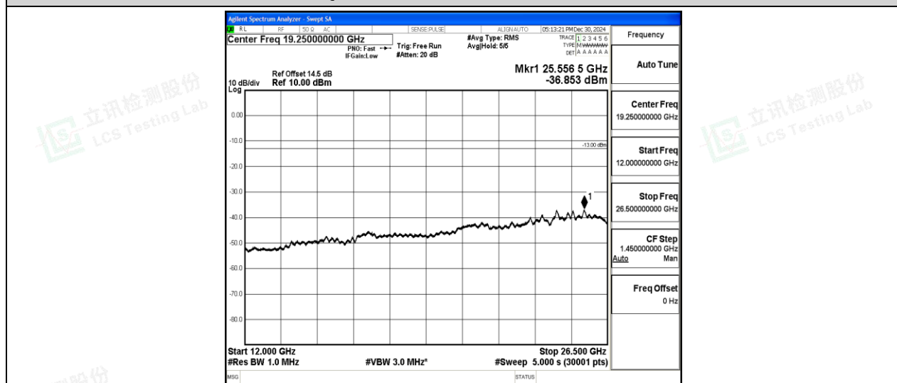
Band2-5MHz-16QAM-18625-1-0-Low-12000-26500--36.85-PASS
