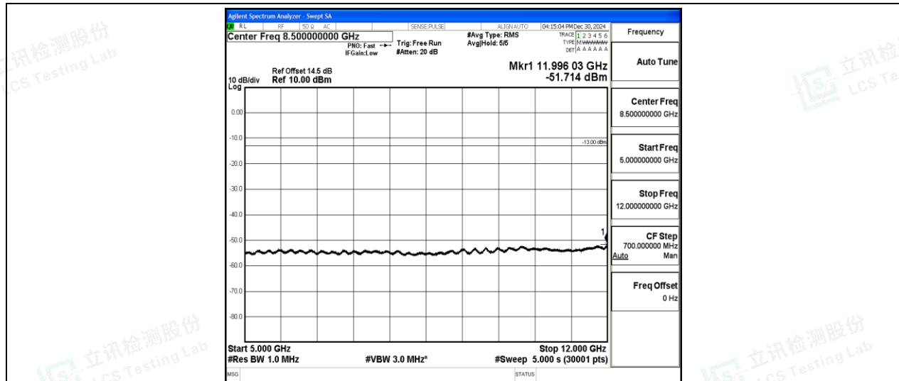
Band2-1.4MHz-16QAM-19193-1-0-High-5000-12000--51.71-PASS
