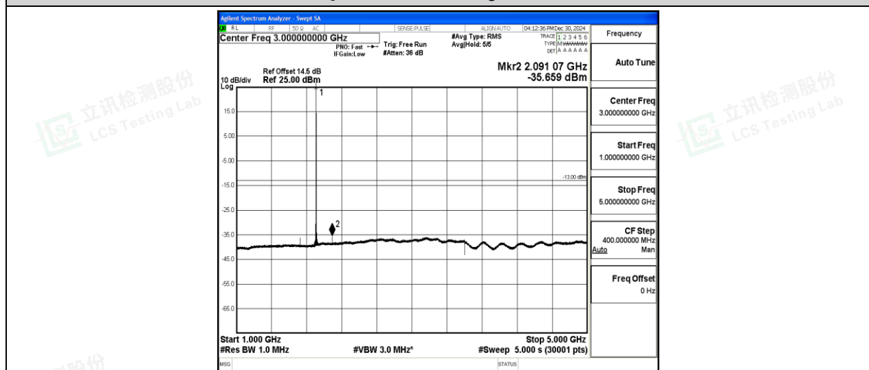
Band2-1.4MHz-QPSK-19193-1-0-High-1000-5000--35.66-PASS
