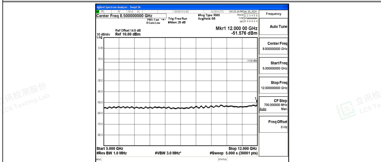
Band2-3MHz-QPSK-18615-1-0-Low-5000-12000--51.58-PASS
