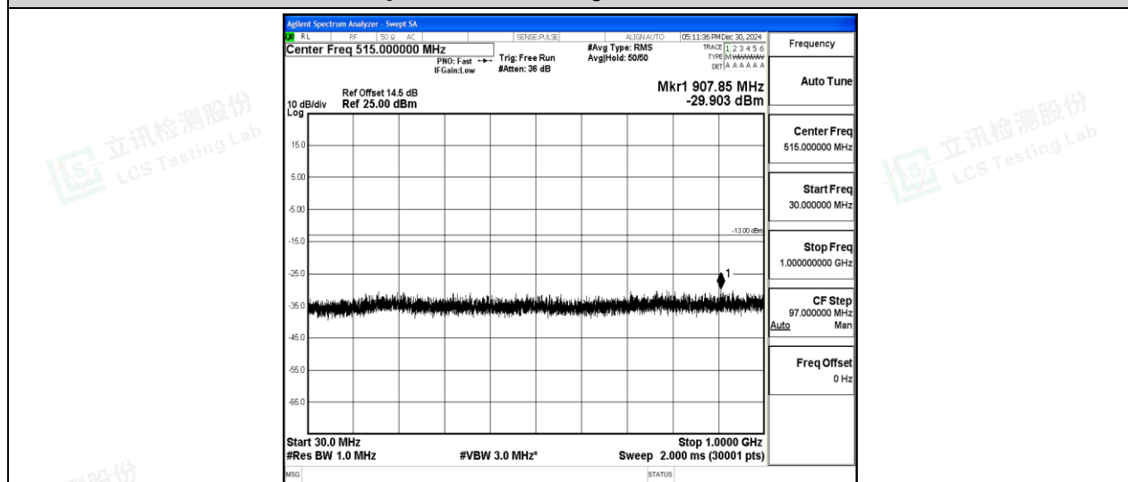
Band2-5MHz-16QAM-18625-1-0-Low-30-1000--29.9-PASS
