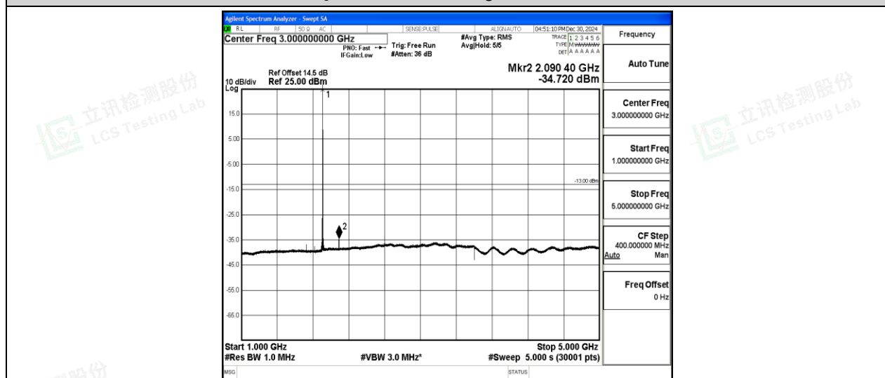
Band2-3MHz-QPSK-19185-1-0-High-1000-5000--34.72-PASS
