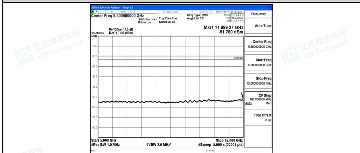
Band2-3MHz-QPSK-18900-1-0-Low-5000-12000--51.78-PASS
