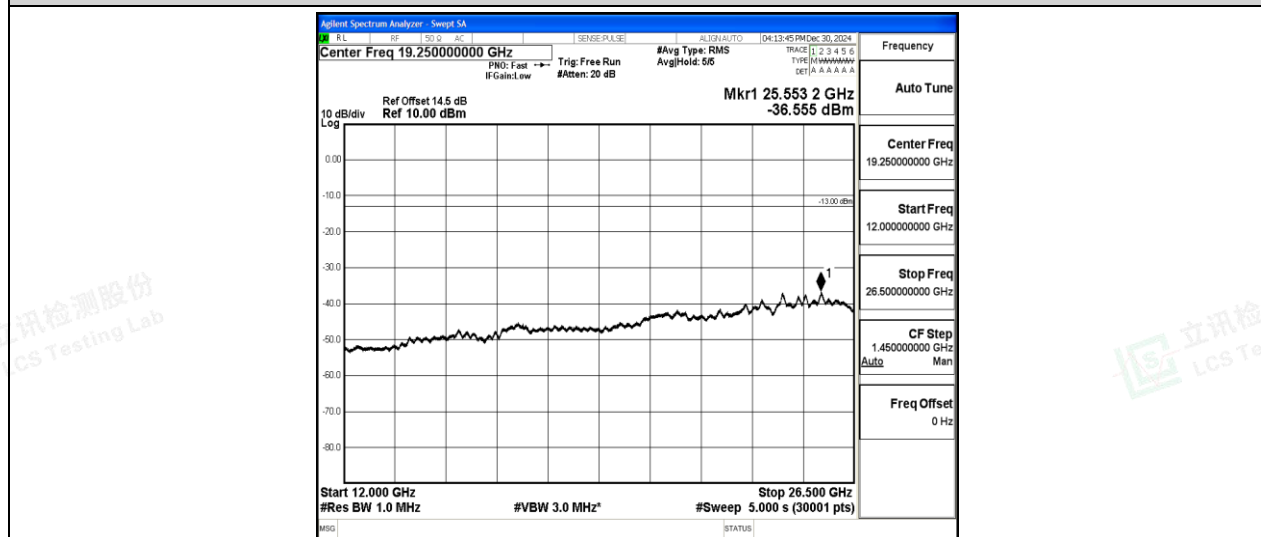
Band2-1.4MHz-QPSK-19193-1-0-High-12000-26500--36.56-PASS
