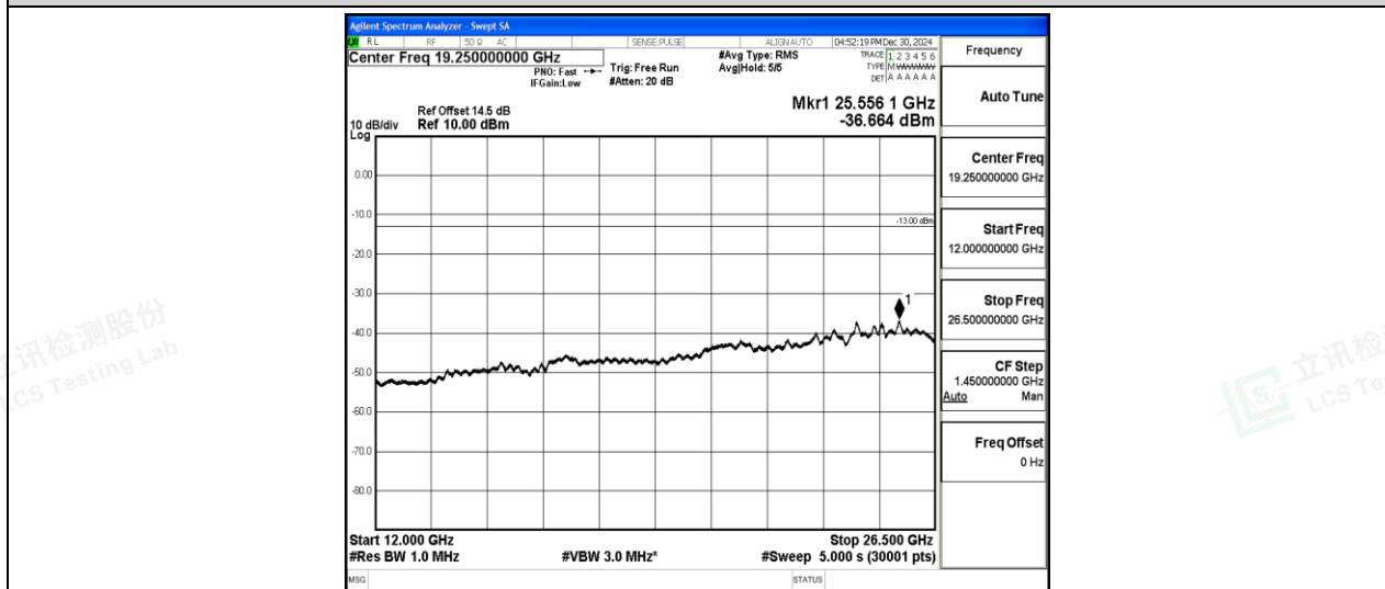
Band2-3MHz-QPSK-19185-1-0-High-12000-26500--36.66-PASS
