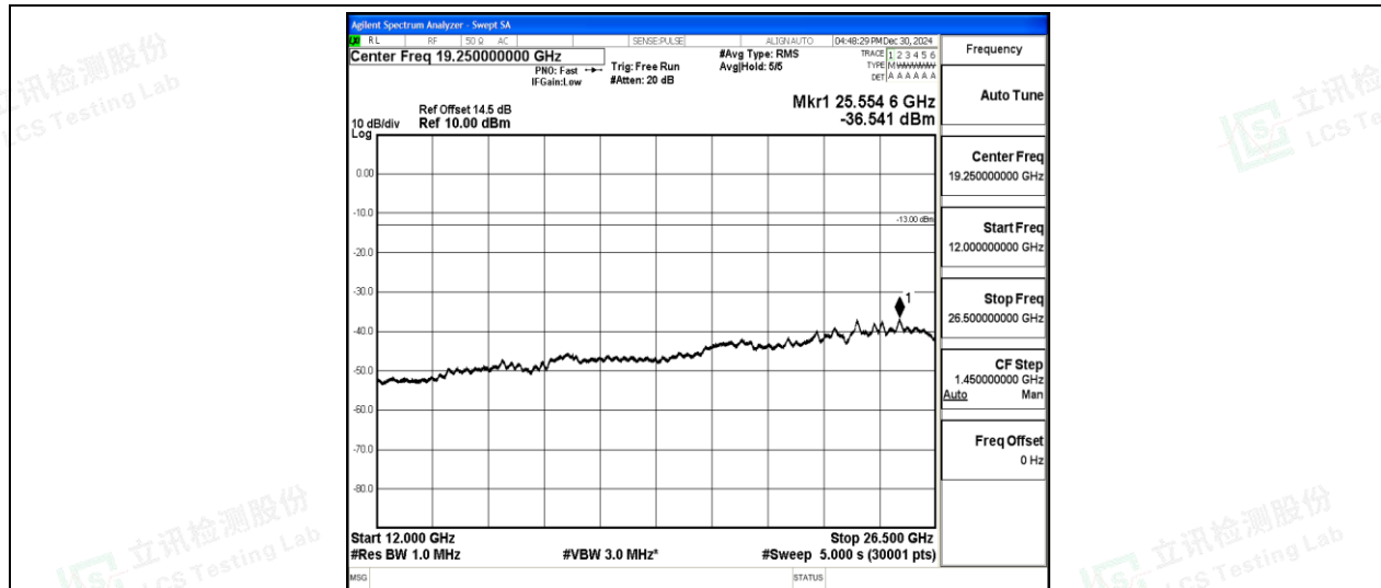
Band2-3MHz-QPSK-18900-1-0-Low-12000-26500--36.54-PASS
