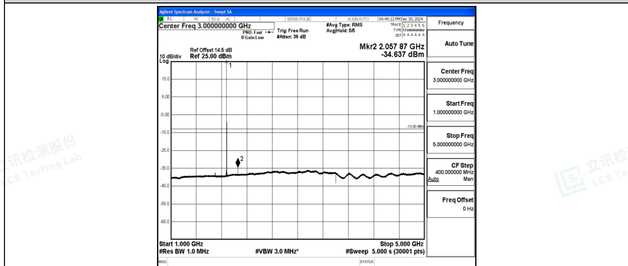
Band2-3MHz-16QAM-18900-1-0-Low-1000-5000--34.64-PASS
