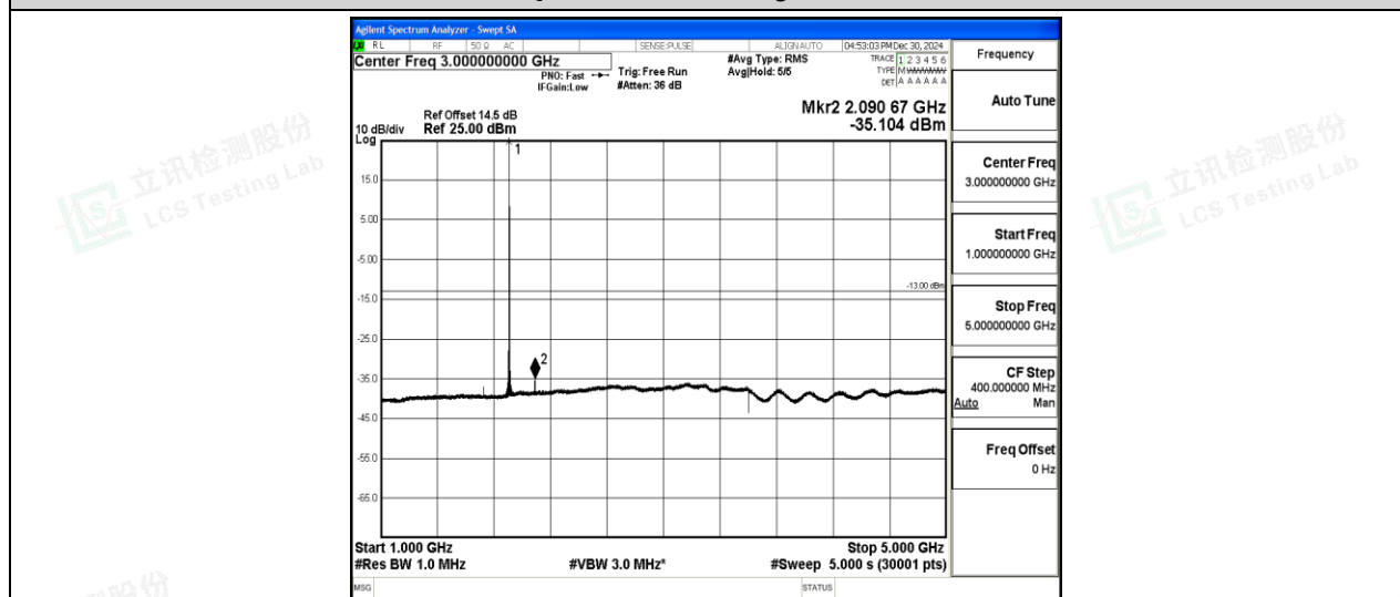
Band2-3MHz-16QAM-19185-1-0-High-1000-5000--35.1-PASS
