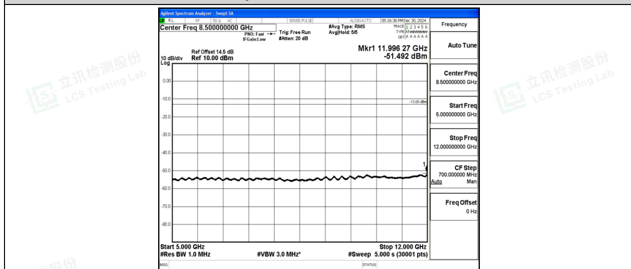
Band2-5MHz-16QAM-18900-1-0-Low-5000-12000--51.49-PASS
