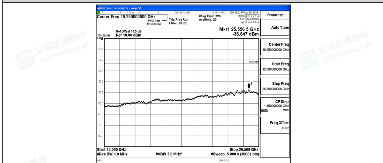
Band2-3MHz-QPSK-18615-1-0-Low-12000-26500--36.65-PASS
