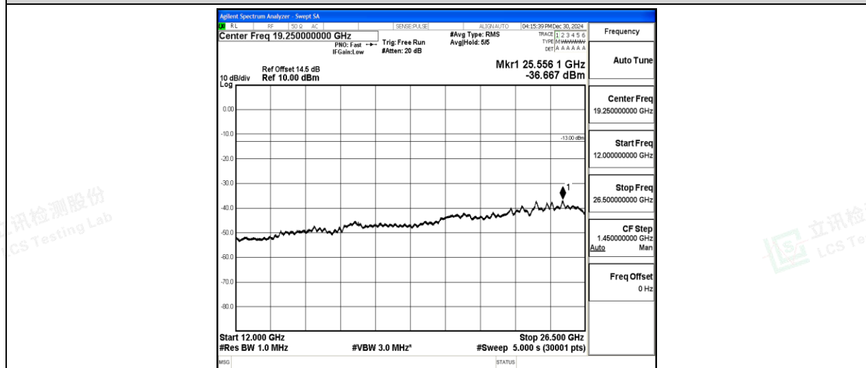
Band2-1.4MHz-16QAM-19193-1-0-High-12000-26500--36.67-PASS
