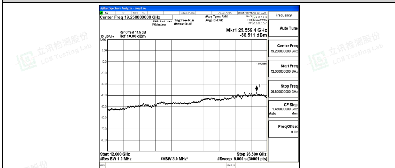
Band2-3MHz-16QAM-18615-1-0-Low-12000-26500--36.51-PASS
