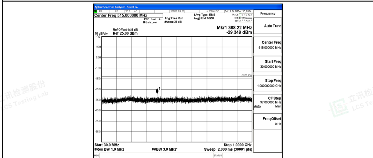
Band2-1.4MHz-16QAM-19193-1-0-High-30-1000--29.35-PASS
