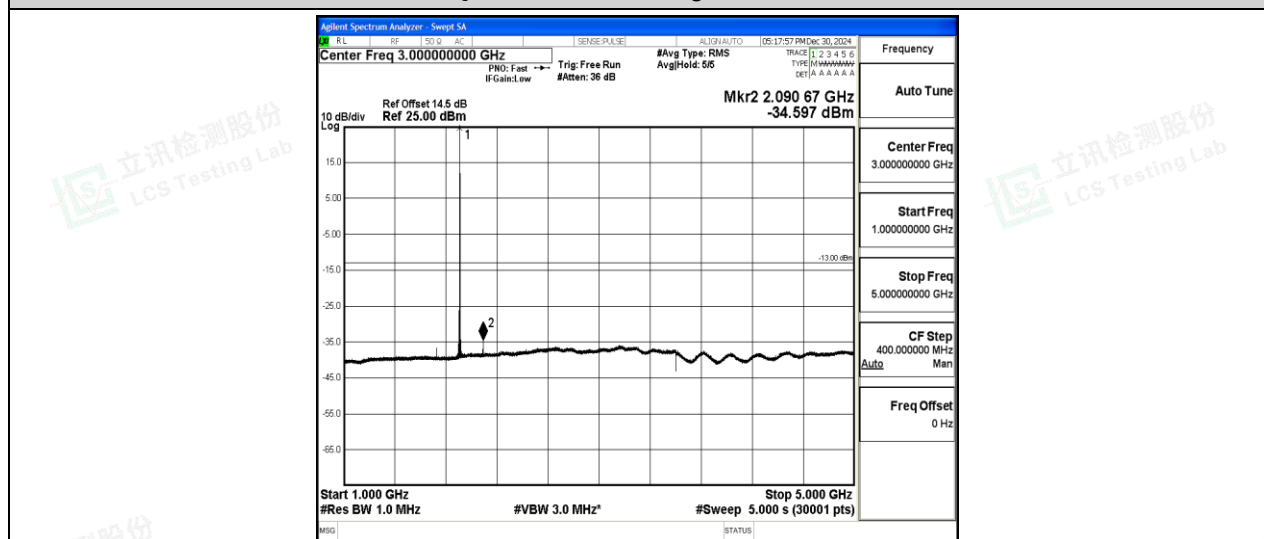
Band2-5MHz-QPSK-19175-1-0-High-1000-5000--34.6-PASS
