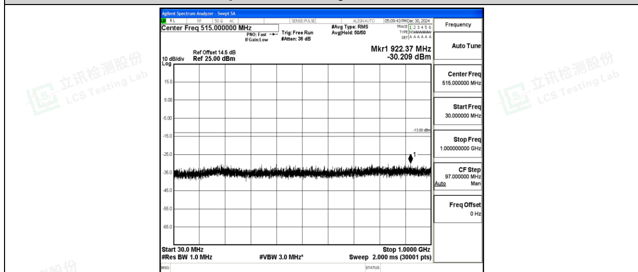
Band2-5MHz-QPSK-18625-1-0-Low-30-1000--30.21-PASS
