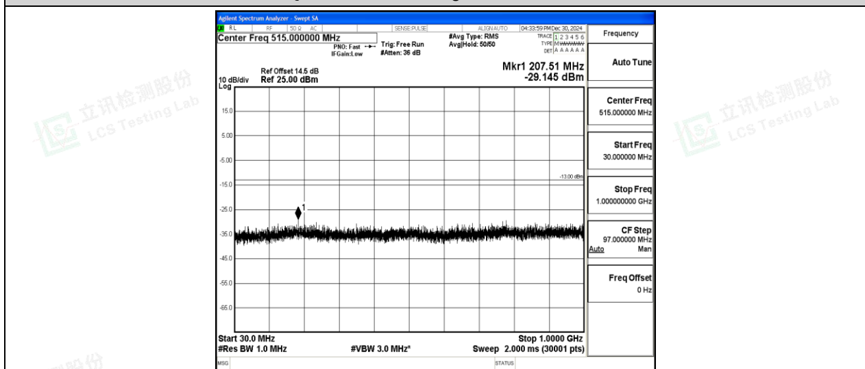
Band2-3MHz-16QAM-18615-1-0-Low-30-1000--29.15-PASS
