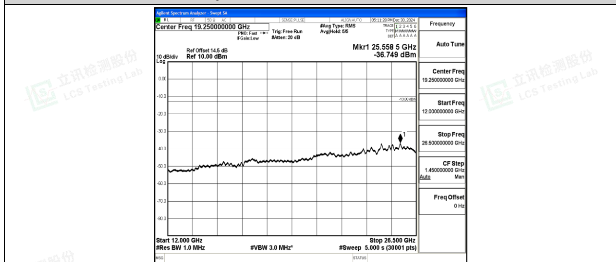
Band2-5MHz-QPSK-18625-1-0-Low-12000-26500--36.75-PASS
