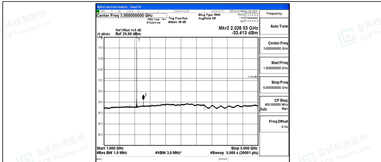
Band2-5MHz-16QAM-18625-1-0-Low-1000-5000--33.41-PASS
