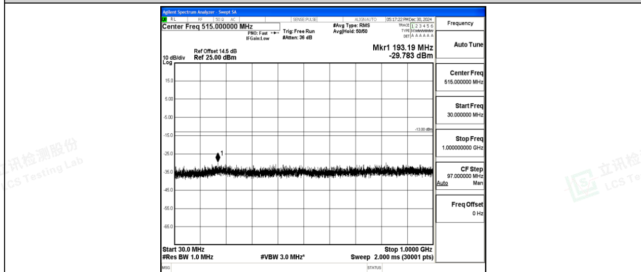
Band2-5MHz-QPSK-19175-1-0-High-30-1000--29.78-PASS
