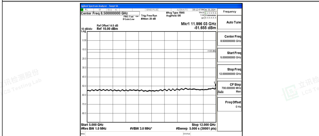
Band2-5MHz-16QAM-18625-1-0-Low-5000-12000--51.66-PASS
