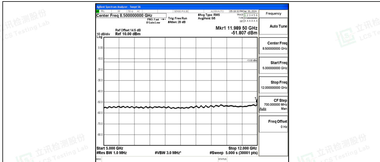
Band2-5MHz-QPSK-19175-1-0-High-5000-12000--51.81-PASS
