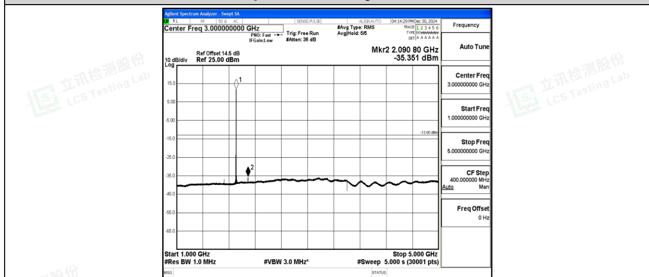
Band2-1.4MHz-16QAM-19193-1-0-High-1000-5000--35.35-PASS
