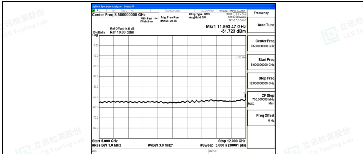
Band2-1.4MHz-QPSK-19193-1-0-High-5000-12000--51.72-PASS
