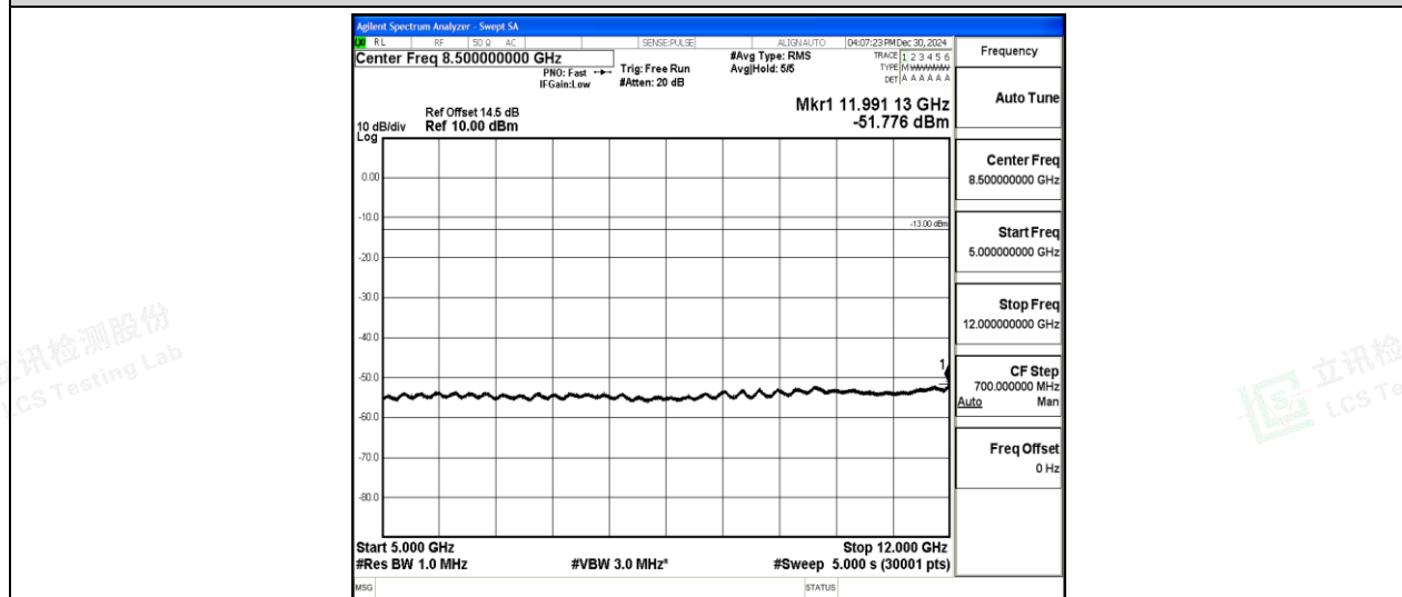
Band2-1.4MHz-16QAM-18607-1-0-Low-5000-12000--51.78-PASS
