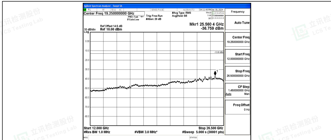
Band2-1.4MHz-16QAM-18900-1-0-Low-12000-26500--36.76-PASS
