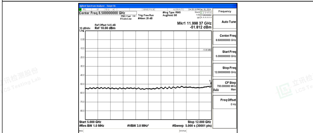
Band2-3MHz-16QAM-18615-1-0-Low-5000-12000--51.81-PASS
