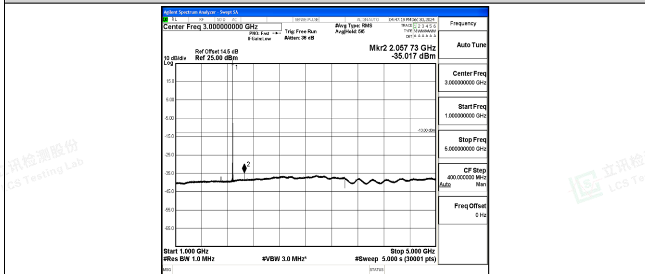
Band2-3MHz-QPSK-18900-1-0-Low-1000-5000--35.02-PASS
