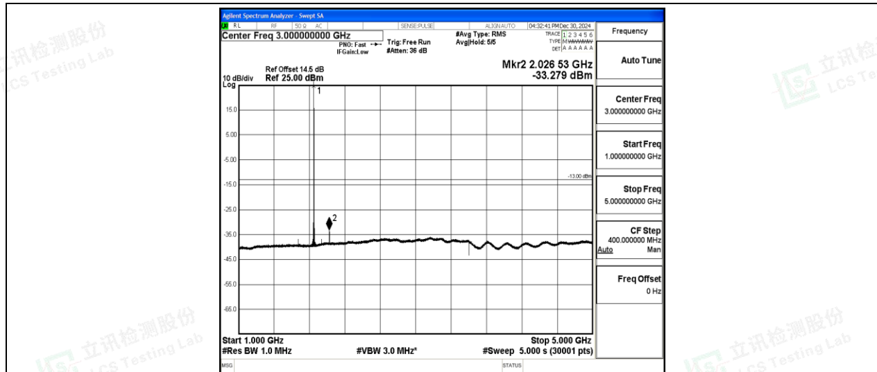
Band2-3MHz-QPSK-18615-1-0-Low-1000-5000--33.28-PASS
