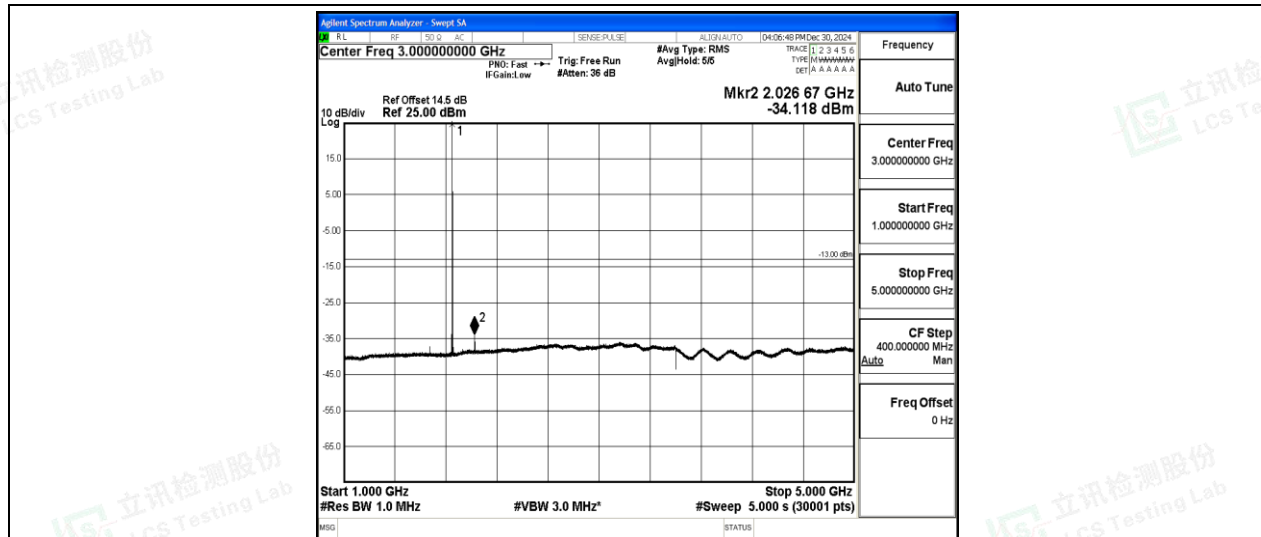
Band2-1.4MHz-16QAM-18607-1-0-Low-1000-5000--34.12-PASS
