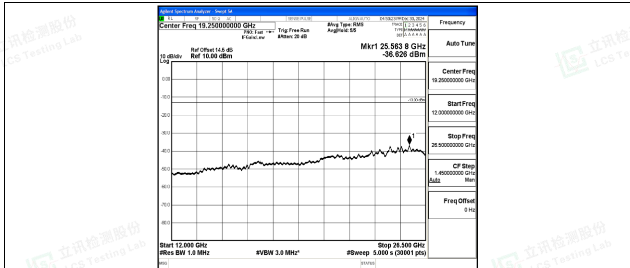
Band2-3MHz-16QAM-18900-1-0-Low-12000-26500--36.63-PASS
