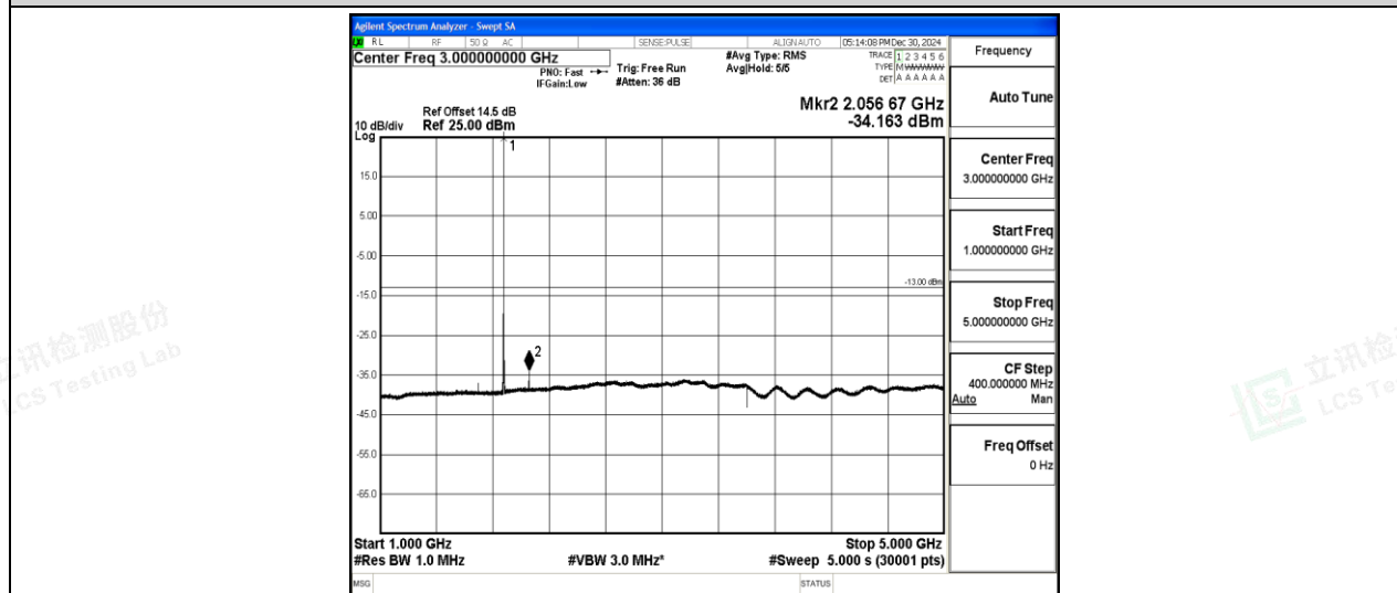
Band2-5MHz-QPSK-18900-1-0-Low-1000-5000--34.16-PASS
