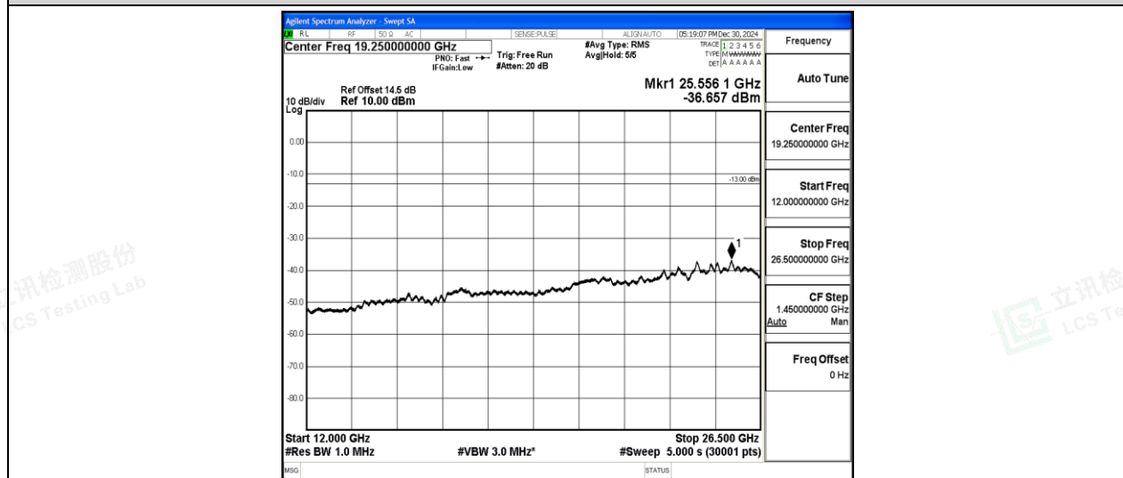
Band2-5MHz-QPSK-19175-1-0-High-12000-26500--36.66-PASS
