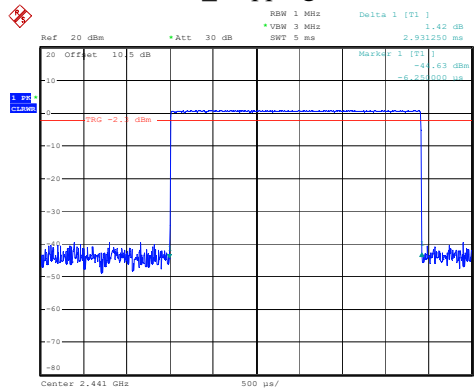
DH5_Hopping 2.931ms
