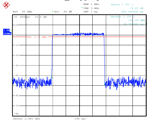
2DH1_Hopping 0.400ms
