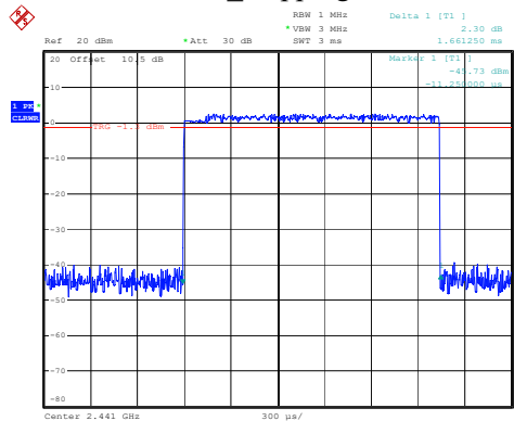
2DH3_Hopping 1.661ms
