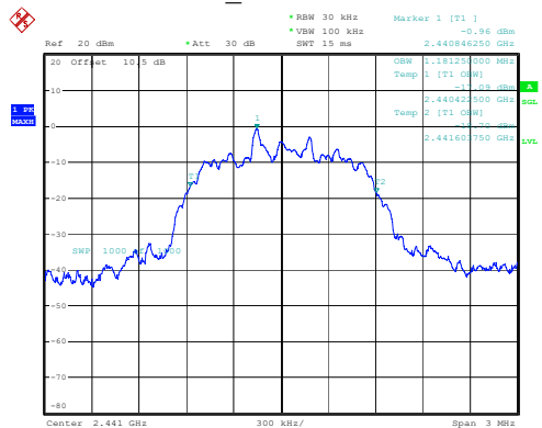
2DH1_Middle 1.181MHz
