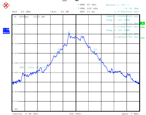
DH1_High 0.851MHz
