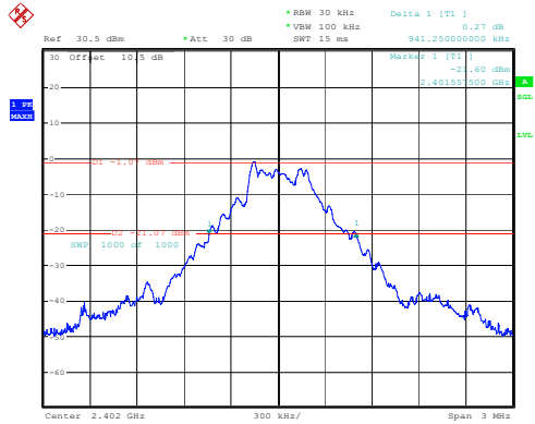
DH1_Low 0.941MHz
