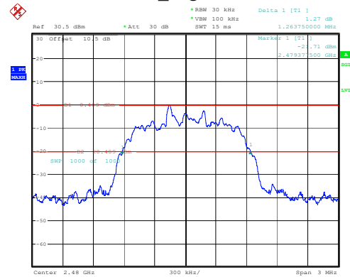
2DH1_High 1.264MHz
