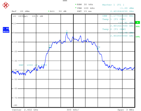
2DH1_Low 1.178MHz
