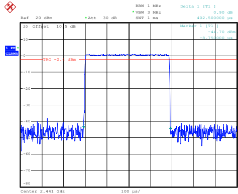
DH1_Hopping 0.403ms
