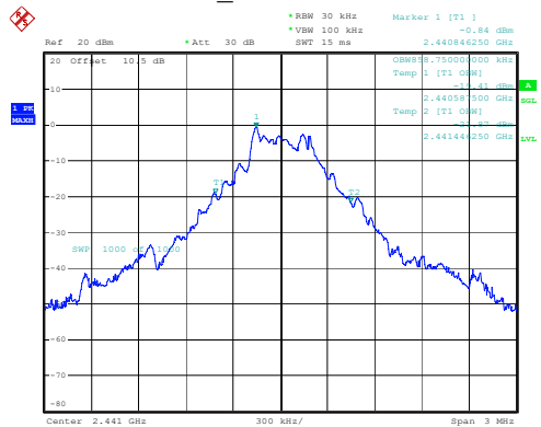
DH1_Middle 0.859MHz
