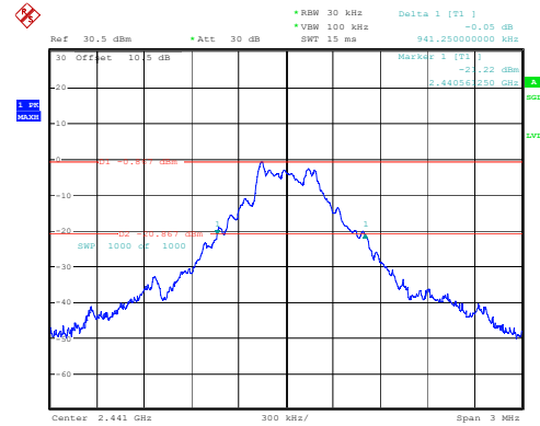
DH1_Middle 0.941MHz
