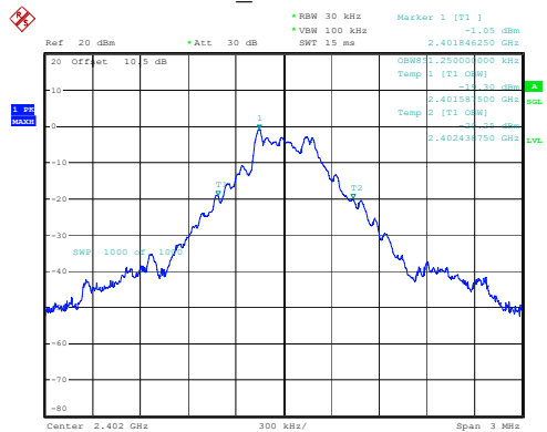
DH1_Low 0.851MHz
