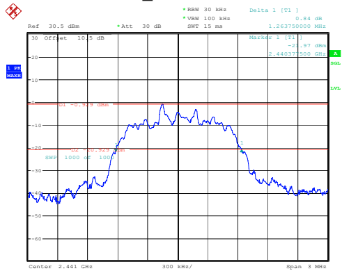
2DH1_Middle 1.264MHz
