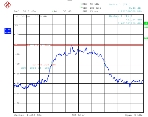
2DH1_Low 1.253MHz
