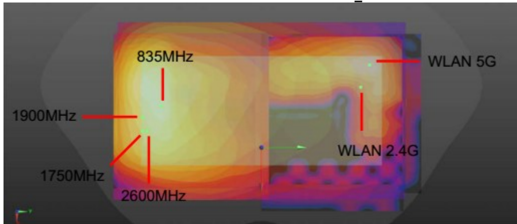
WWAN + WLAN 5GHz/2.4GHz Back_0mm
