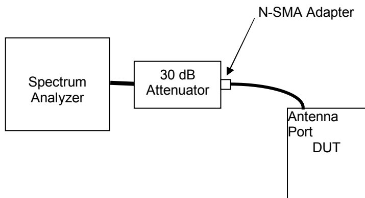
Figure C-1 - Setup Drawing
