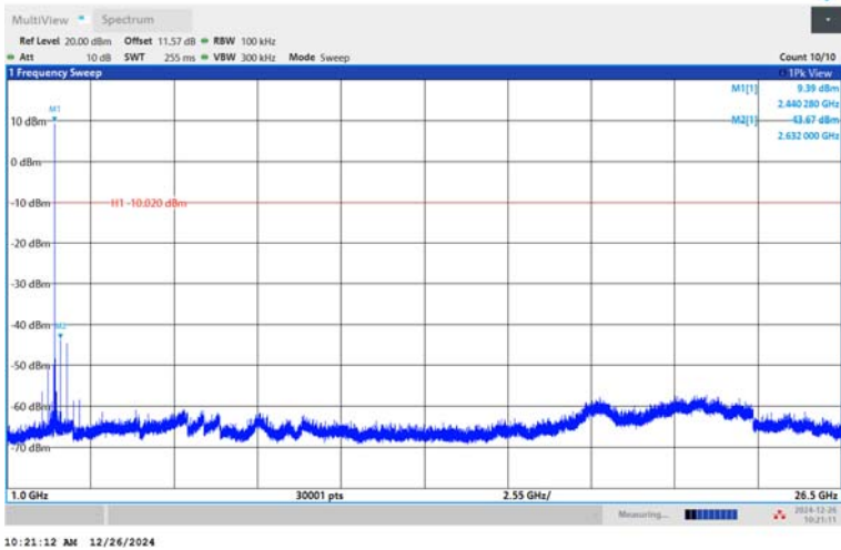
BLE_1M-Ant1-2440-1000~26500-PASS
