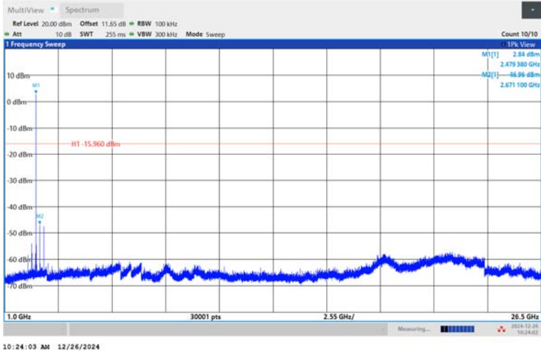
BLE_1M-Ant1-2480-1000~26500-PASS
