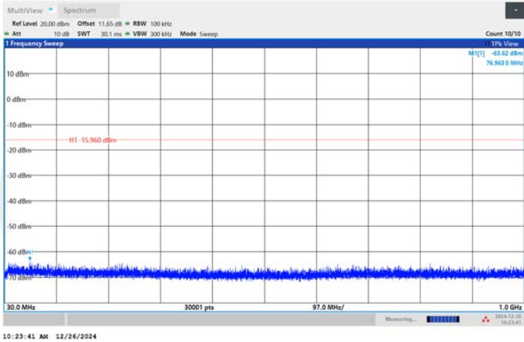
BLE_1M-Ant1-2480-30~1000-PASS
