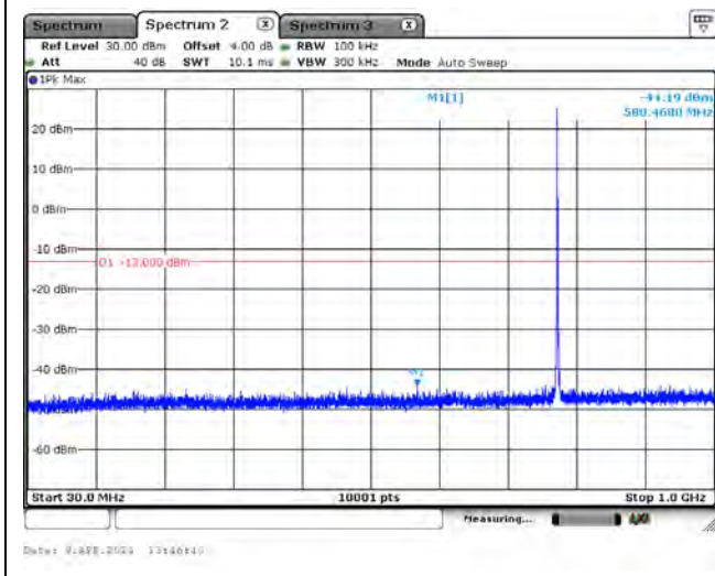
CH23230_10M_QPSK_1RB0_Below 1G
