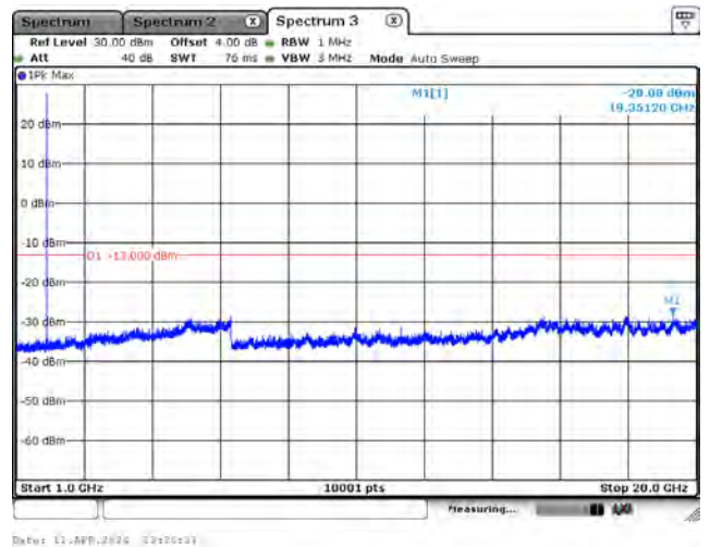
CH26365_10M_QPSK_1RB0_Above 1G
