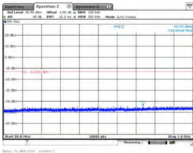
CH132622_10M_QPSK_1RB0_Below 1G
