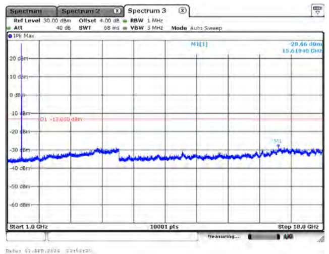
CH132622_10M_QPSK_1RB0_Above 1G
