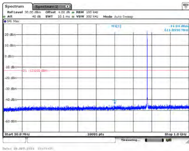
CH23278_15k_BPSK_1RB0_Below 1G
