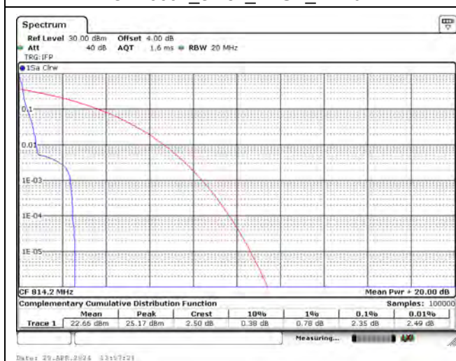
CH26692_3.75k_BPSK_1RB0
