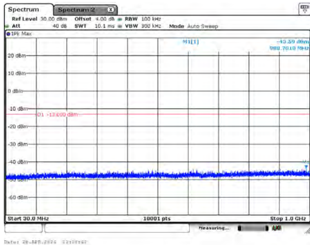
CH132322_3.75k_QPSK_1RB0_Below 1G
