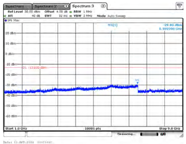
CH27025_3M_QPSK_1RB0_Above 1G
