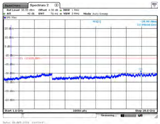
CH26688_15k_BPSK_1RB0_Above 1G
