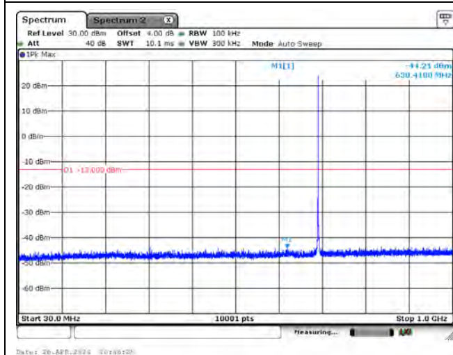
CH23012_3.75k_BPSK_1RB0_Below 1G
