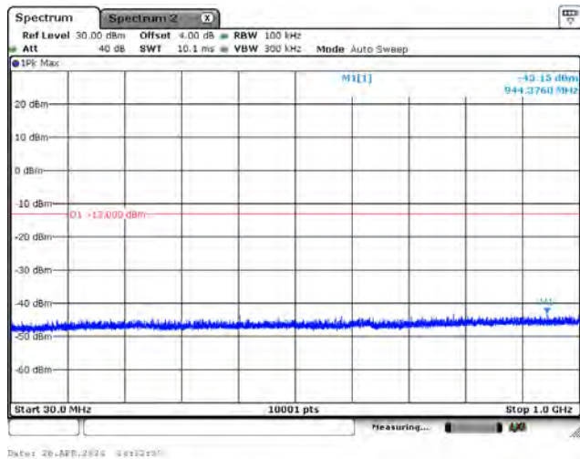
CH133047_15k_BPSK_1RB0_Below 1G
