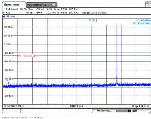
CH23230_15k_BPSK_1RB0_Below 1G
