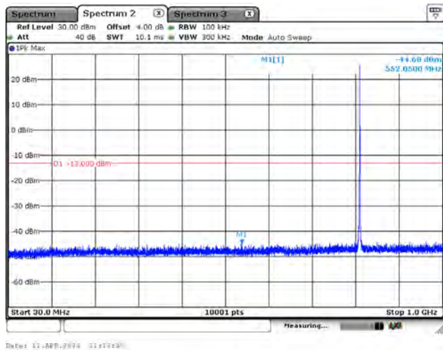
CH26740_5M_QPSK_1RB0_Below 1G
