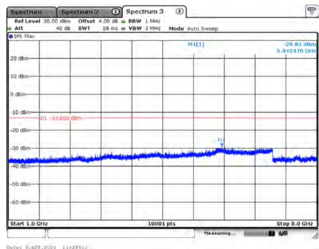
CH23165_3M_QPSK_1RB0_Above 1G
