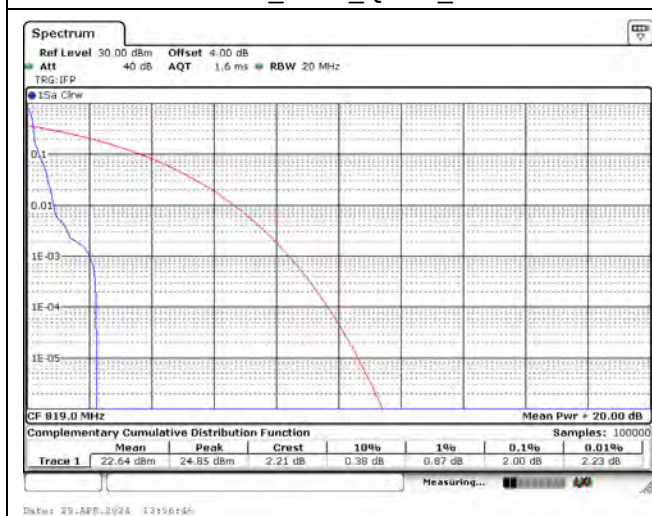
CH26740_3.75k_QPSK_1RB0
