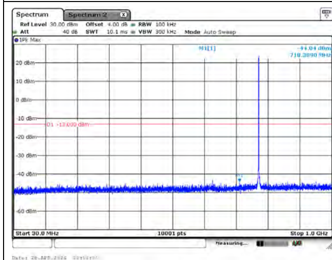
CH23182_3.75k_BPSK_1RB0_Below 1G
