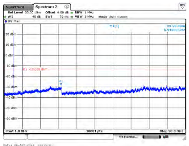
CH26688_15k_QPSK_1RB0_Above 1G
