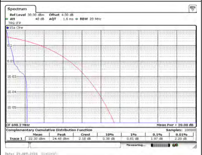
CH134004_3.75k_QPSK_1RB0
