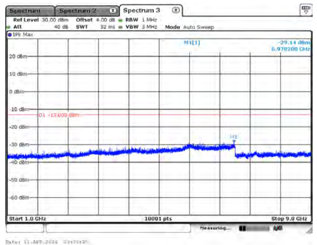
CH27015_5M_QPSK_1RB0_Above 1G
