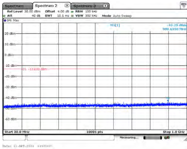
CH132597_15M_QPSK_1RB0_Below 1G
