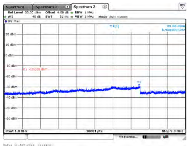
CH26765_5M_QPSK_1RB0_Above 1G
