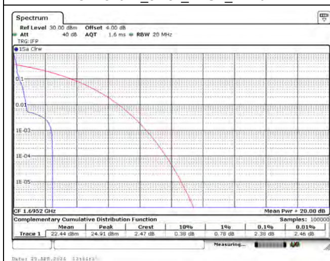
CH132974_3.75k_BPSK_1RB0
