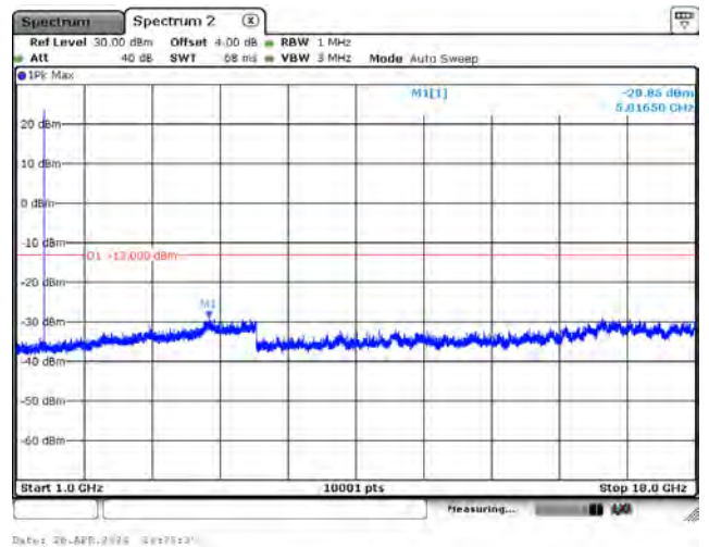
CH133047_15k_QPSK_1RB0_Above 1G
