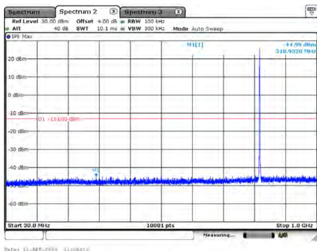
CH26775_3M_QPSK_1RB0_Below 1G
