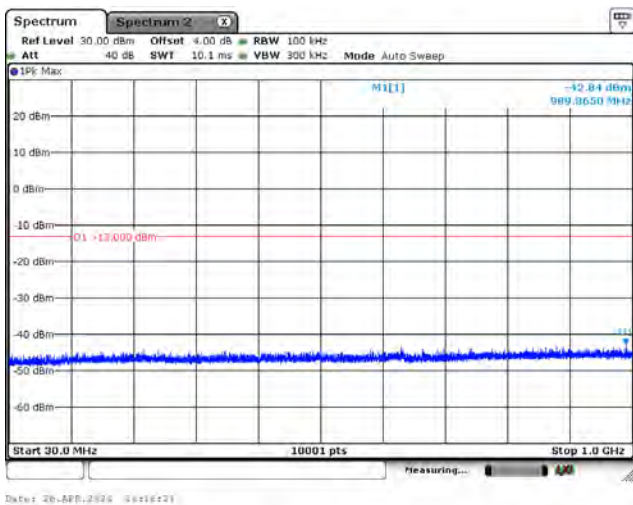
CH133120_3.75k_QPSK_1RB0_Below 1G
