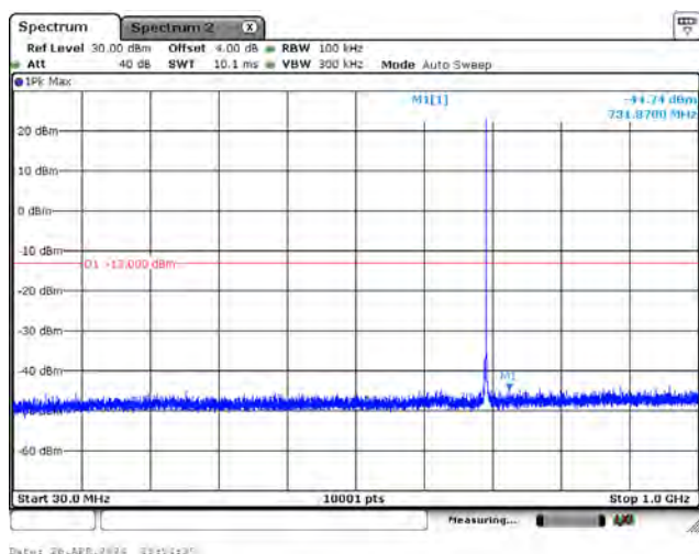
CH23095_15k_BPSK_1RB0_Below 1G
