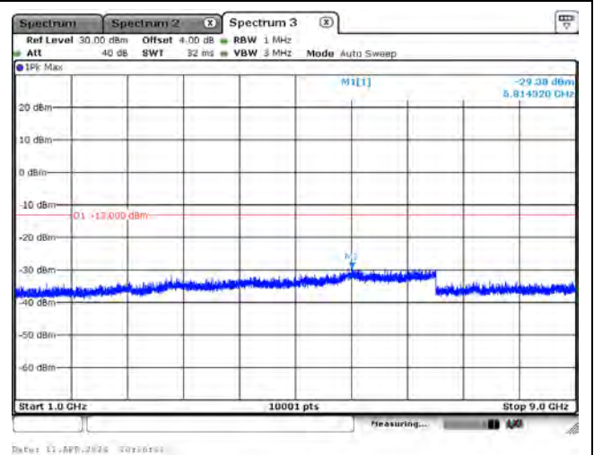
CH26740_1.4M_QPSK_1RB0_Above 1G
