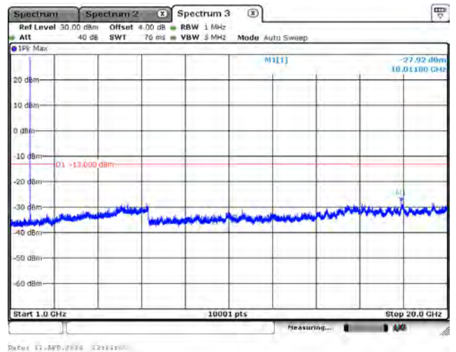
CH26365_15M_QPSK_1RB0_Above 1G
