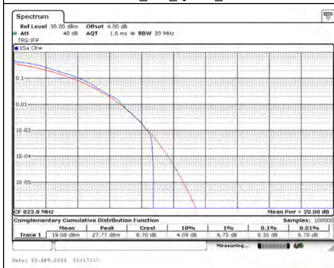
CH26788_15k_QPSK_12RB0
