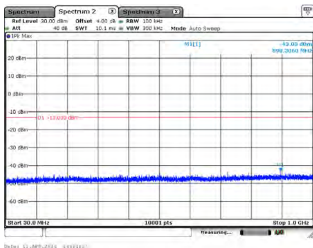
CH132647_5M_QPSK_1RB0_Below 1G
