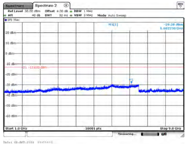
CH26740_15k_QPSK_1RB0_Above 1G
