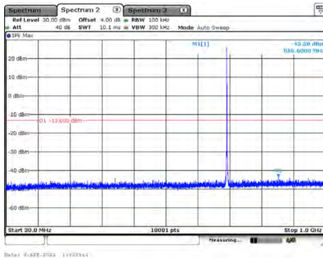
CH23095_3M_QPSK_1RB0_Below 1G
