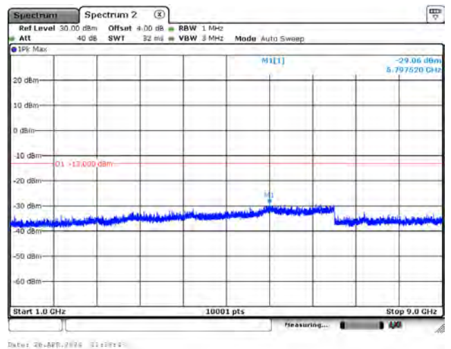
CH26788_3.75k_QPSK_1RB0_Above 1G
