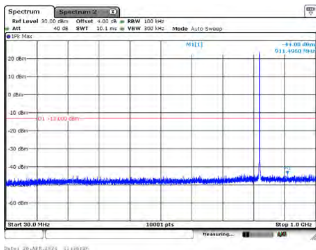
CH26788_3.75k_QPSK_1RB0_Below 1G
