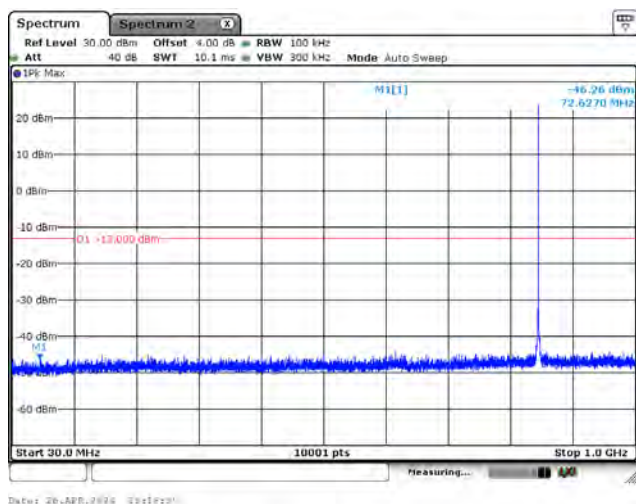
CH27038_15k_BPSK_1RB0_Below 1G
