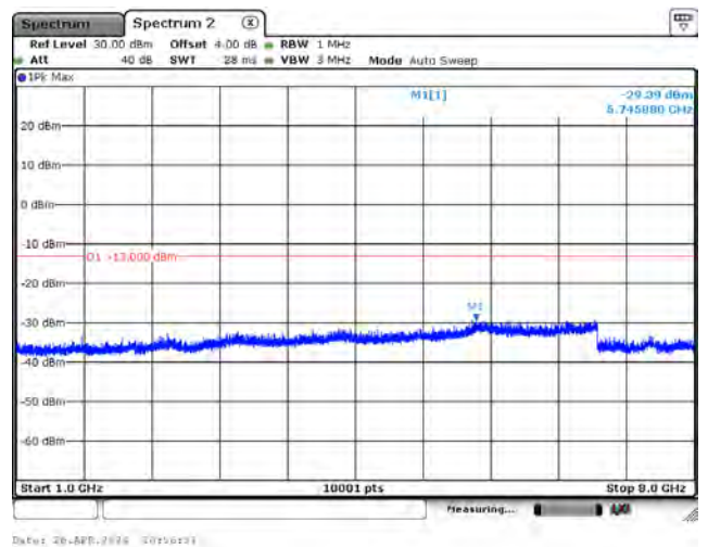
CH23178_3.75k_QPSK_1RB0_Above 1G
