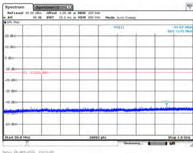
CH26688_15k_BPSK_1RB0_Below 1G
