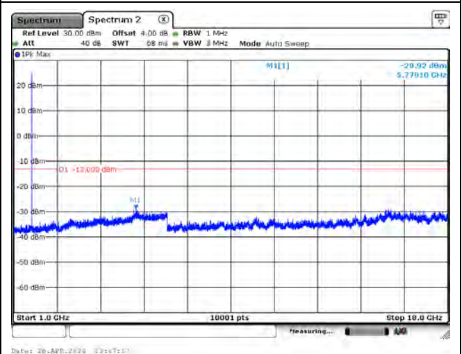
CH132974_3.75k_BPSK_1RB0_Above 1G
