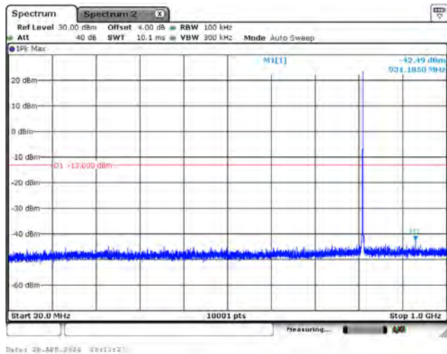
CH26740_15k_BPSK_1RB0_Below 1G
