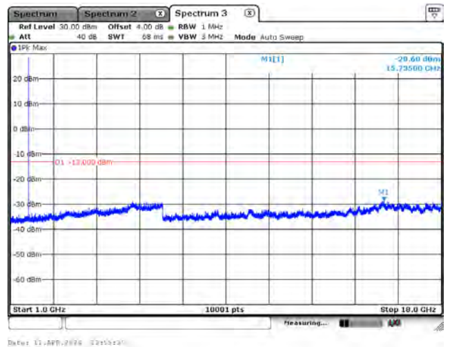
CH132322_10M_QPSK_1RB0_Above 1G
