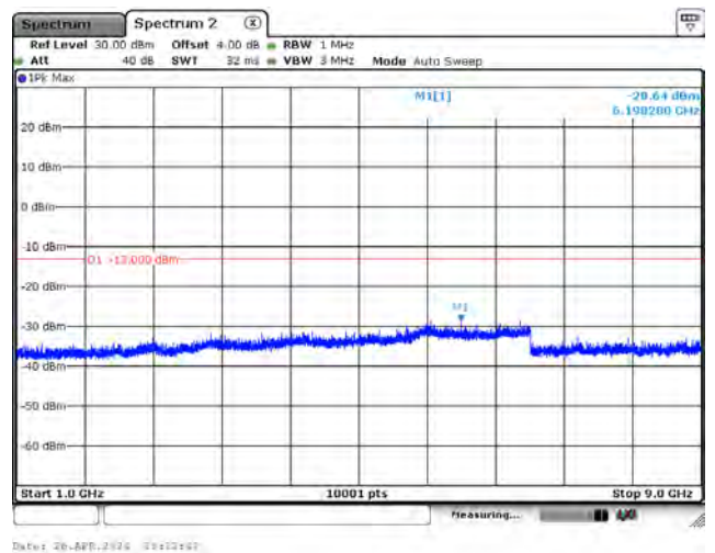
CH27038_15k_BPSK_1RB0_Above 1G
