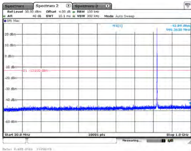
CH26915_3M_QPSK_1RB0_Below 1G
