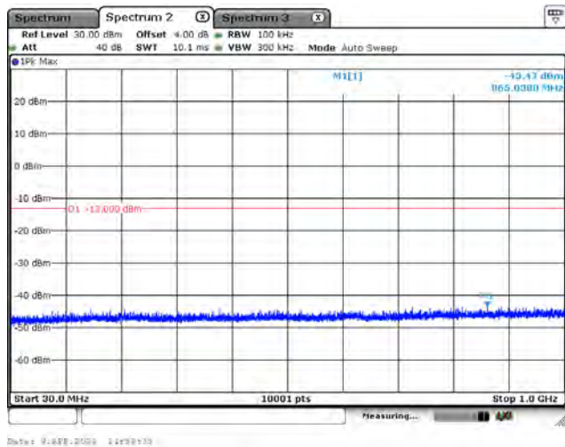
CH26365_15M_QPSK_1RB0_Below 1G
