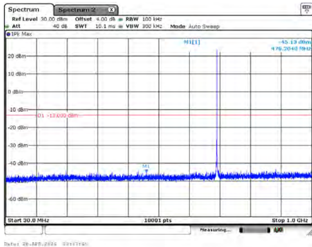
CH23095_3.75k_QPSK_1RB0_Below 1G
