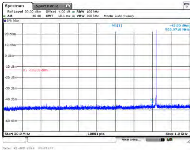
CH26915_15k_BPSK_1RB0_Below 1G
