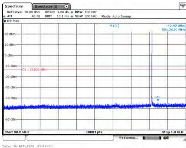
CH26788_15k_QPSK_1RB0_Below 1G
