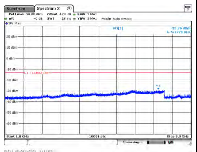
CH134004_3.75k_BPSK_1RB0_Above 1G
