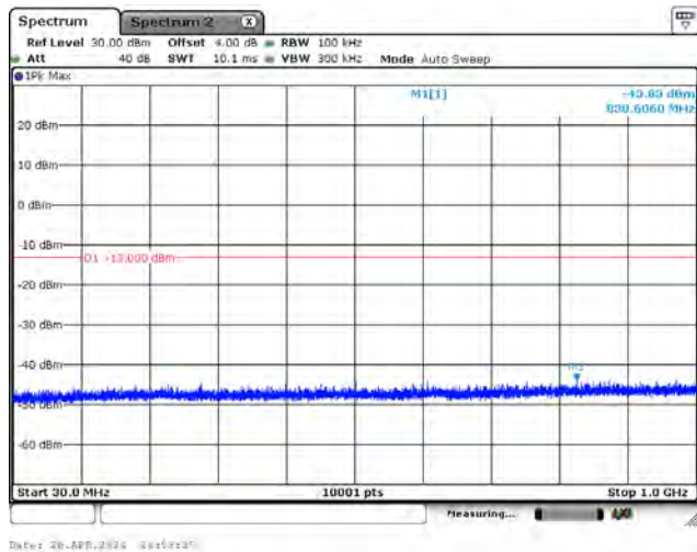
CH26365_15k_BPSK_1RB0_Below 1G
