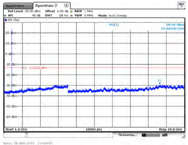
CH133047_QPSK_3.75k_1RB0_Above 1G
