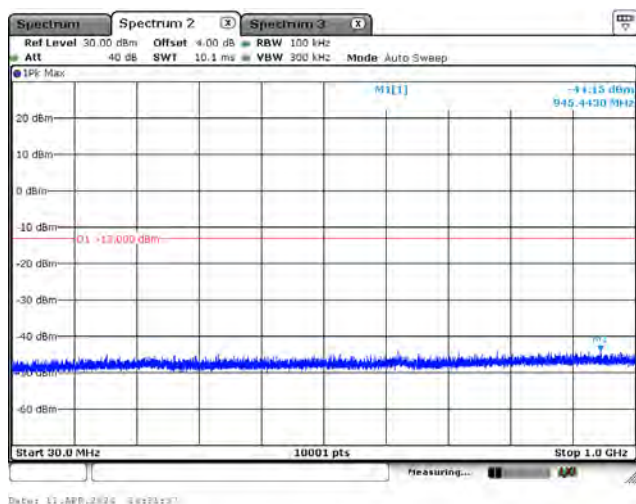
CH132657_3M_QPSK_1RB0_Below 1G
