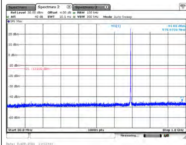
CH23095_1.4M_QPSK_1RB0_Below 1G
