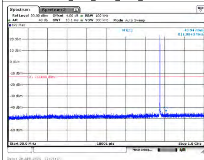
CH23278_3.75k_BPSK_1RB0_Below 1G
