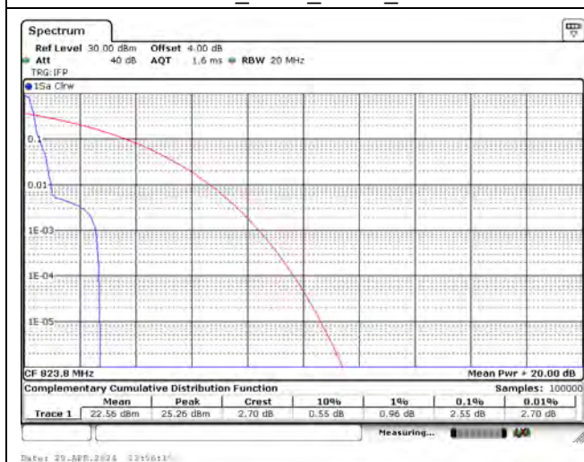
CH26788_3.75k_BPSK_1RB47
