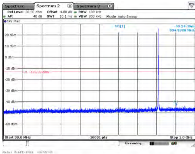
CH26740_3M_QPSK_1RB0_Below 1G
