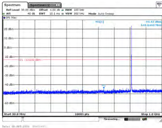
CH26740_15k_QPSK_1RB0_Below 1G
