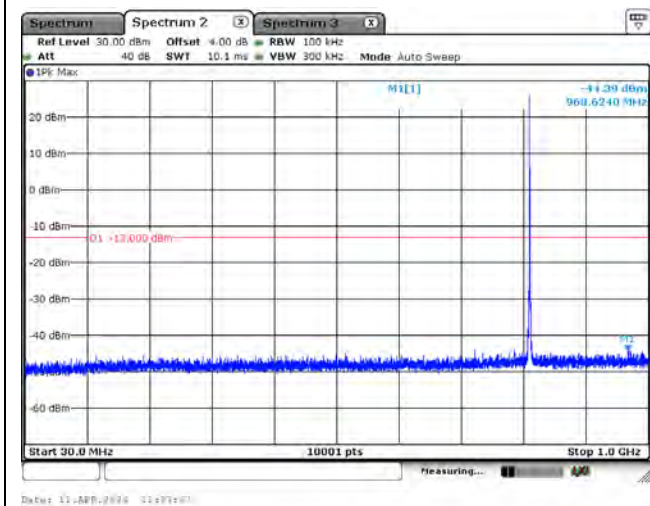
CH26740_10M_QPSK_1RB0_low_Below 1G
