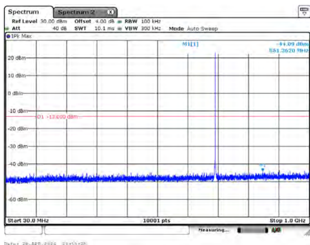
CH23095_15k_QPSK_1RB0_Below 1G
