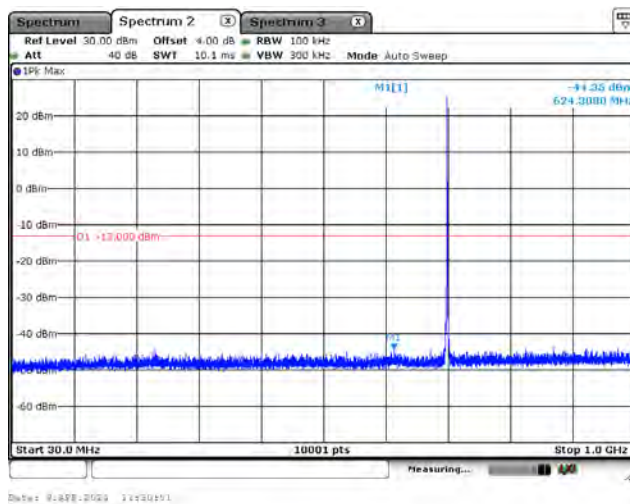
CH23165_3M_QPSK_1RB0_Below 1G
