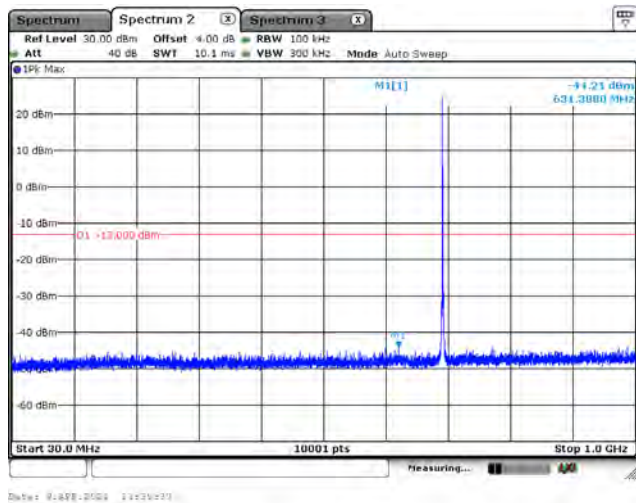
CH23095_5M_QPSK_1RB0_Below 1G
