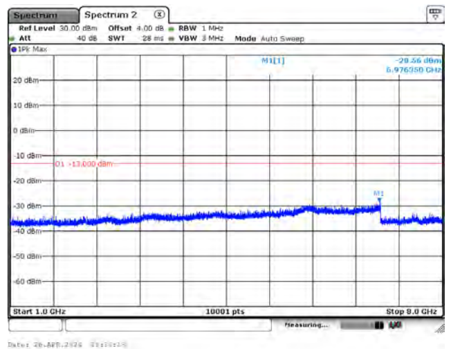
CH134180_15k_BPSK_1RB0_Above 1G
