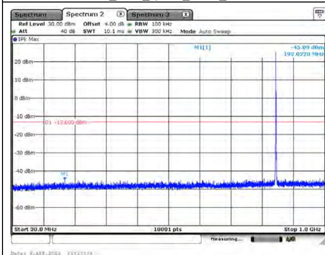
CH27033_1.4M_QPSK_1RB0_Below 1G
