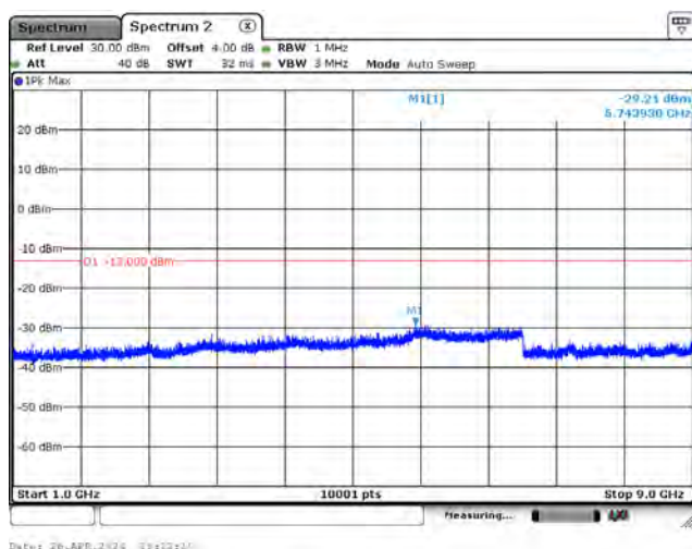
CH26915_15k_QPSK_1RB0_Above 1G
