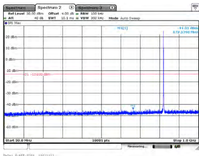
CH26915_10M_QPSK_1RB0_Below 1G
