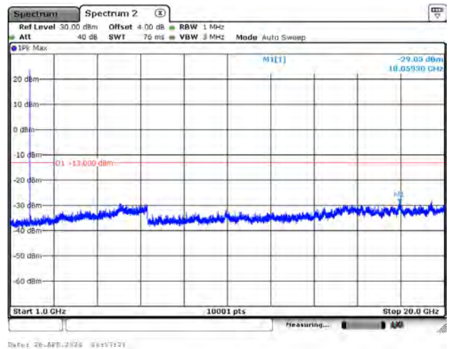
CH26365_15k_BPSK_1RB0_Above 1G
