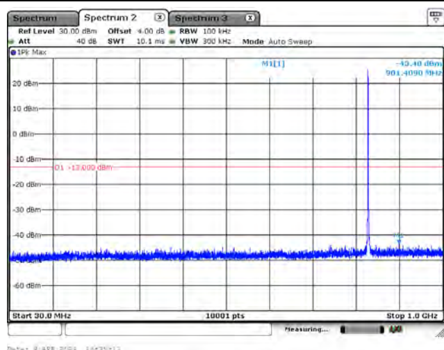
CH26990_10M_QPSK_1RB0_Below 1G
