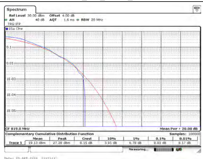
CH26740_15k_QPSK_12RB0
