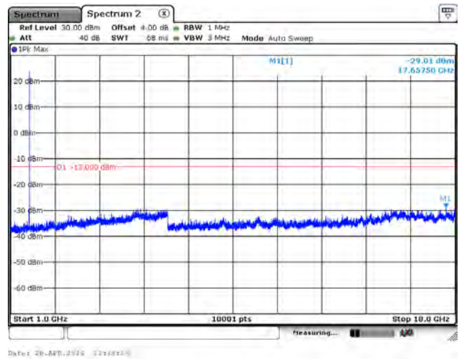
CH133120_3.75k_QPSK_1RB0_Above 1G
