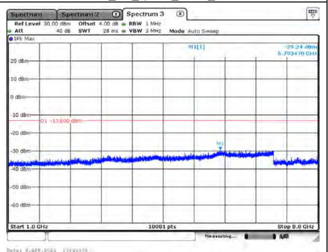
CH23255_5M_QPSK_1RB0_Above 1G
