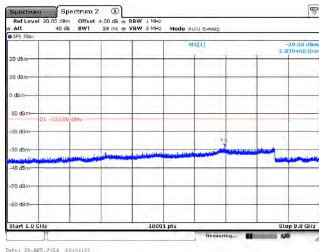
CH23178_15k_BPSK_1RB0_Above 1G
