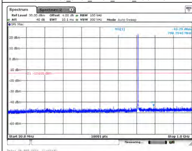
CH134180_3.75k_BPSK_1RB0_Below 1G
