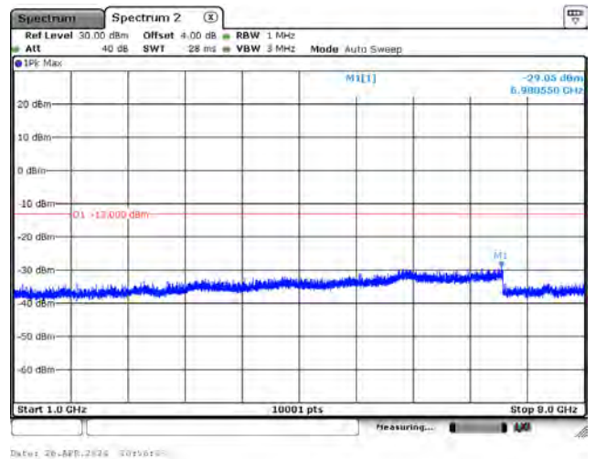
CH23095_3.75k_QPSK_1RB0_Above 1G
