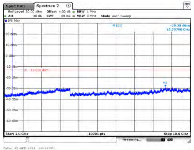
CH132322_15k_BPSK_1RB0_Above 1G
