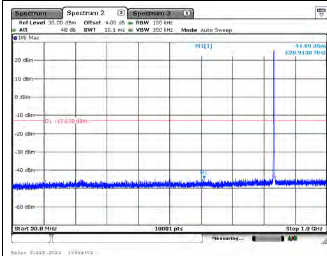
CH26915_1.4M_QPSK_1RB0_Below 1G
