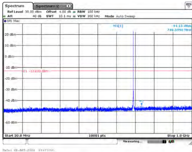
CH134092_15k_BPSK_1RB0_Below 1G
