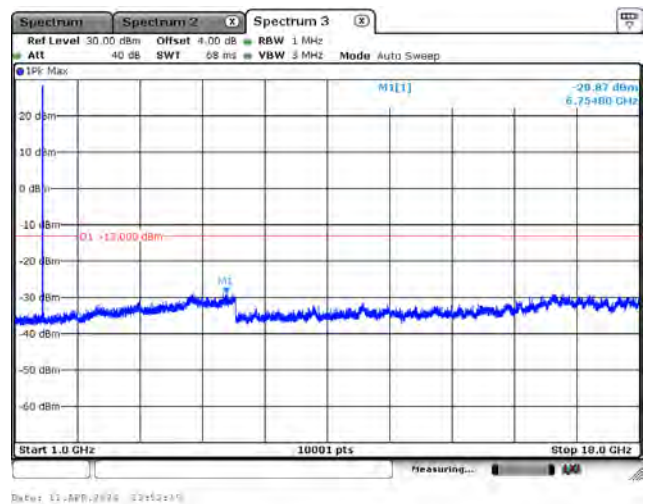
CH132647_5M_QPSK_1RB0_Above 1G
