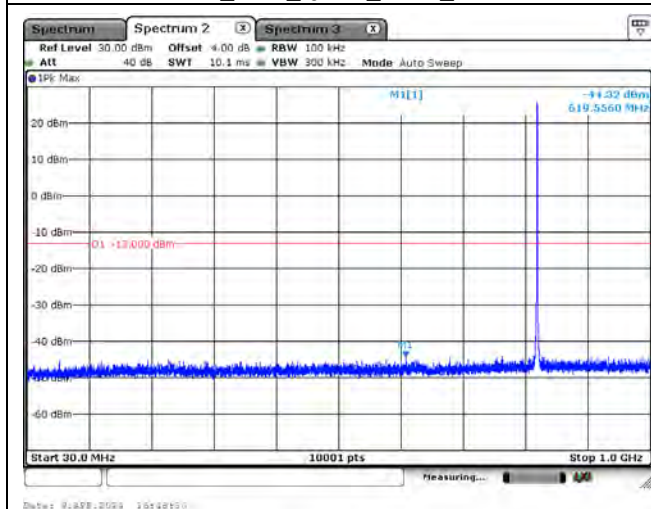
CH26783_1.4M_QPSK_1RB0_Below 1G
