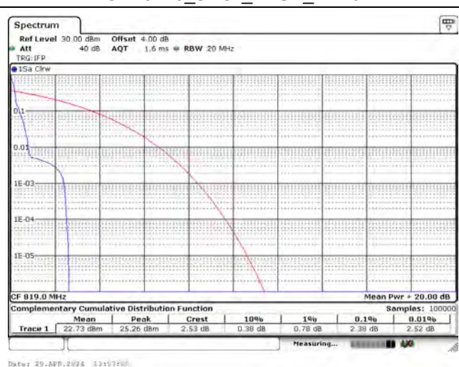
CH26740_3.75k_BPSK_1RB0
