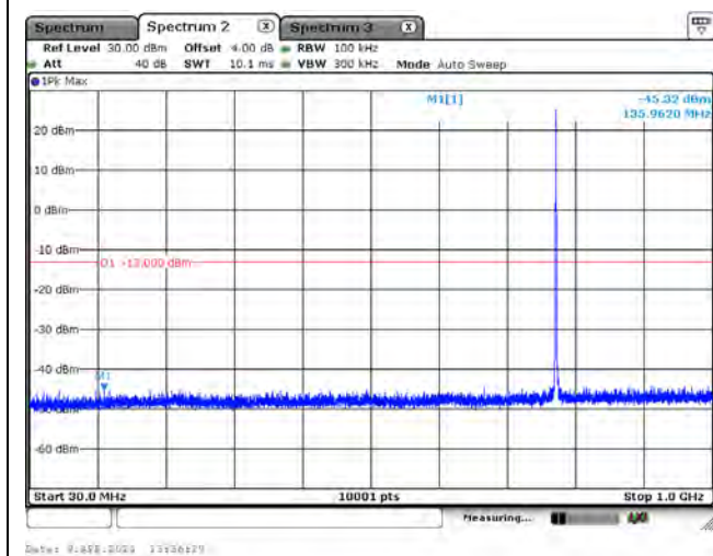
CH23230_5M_QPSK_1RB0_Below 1G
