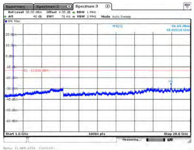
CH26640_10M_QPSK_1RB0_Above 1G
