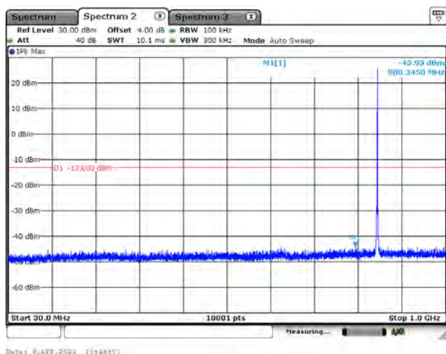
CH27025_3M_QPSK_1RB0_Below 1G
