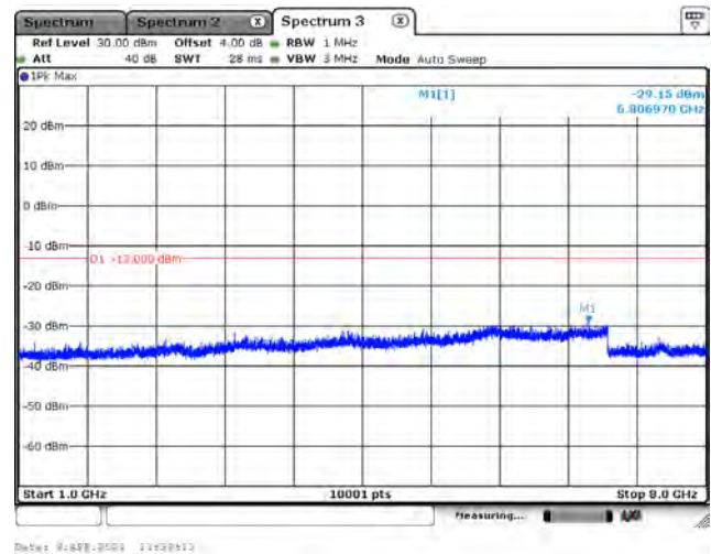
CH23095_3M_QPSK_1RB0_Above 1G
