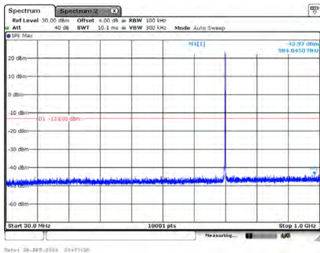
CH134180_15k_BPSK_1RB0_Below 1G
