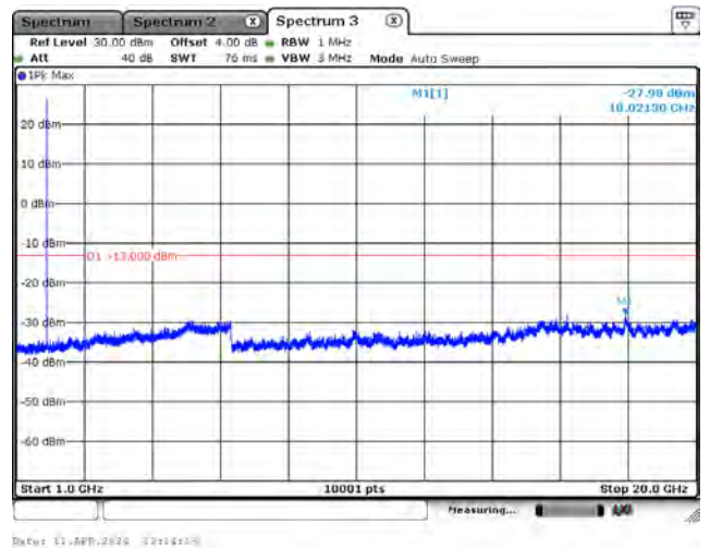
CH26365_3M_QPSK_1RB0_Above 1G
