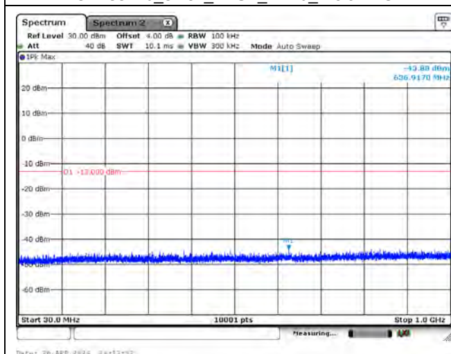
CH133120_3.75k_BPSK_1RB0_Below 1G
