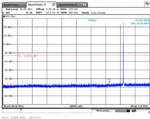
CH26915_5M_QPSK_1RB0_Below 1G
