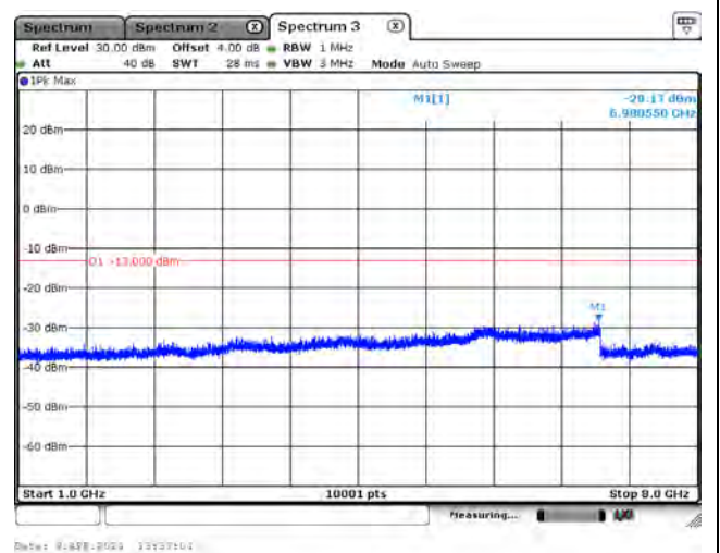
CH23230_5M_QPSK_1RB0_Above 1G
