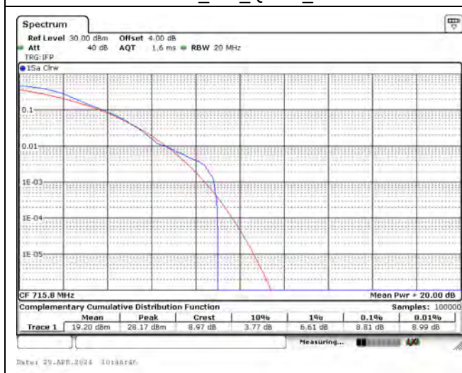
CH134180_15k_QPSK_12RB0
