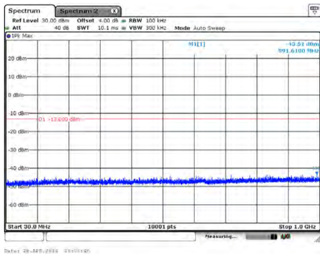
CH26688_15k_QPSK_1RB0_Below 1G
