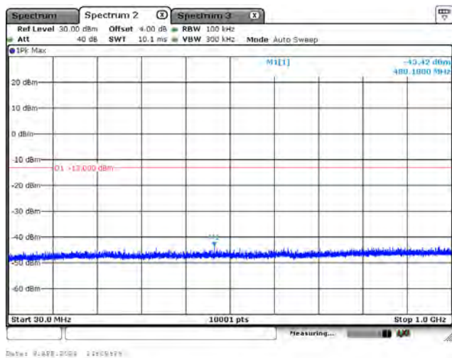
CH26675_3M_QPSK_1RB0_Below 1G
