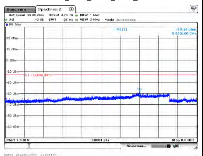
CH134180_3.75k_BPSK_1RB0_Above 1G
