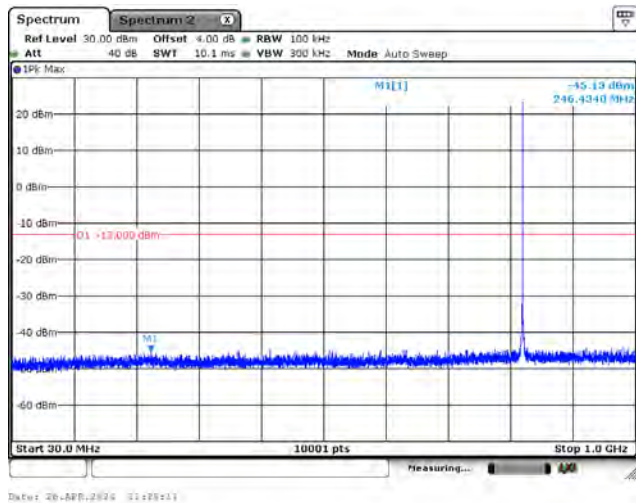
CH26915_3.75k_QPSK_1RB0_Below 1G
