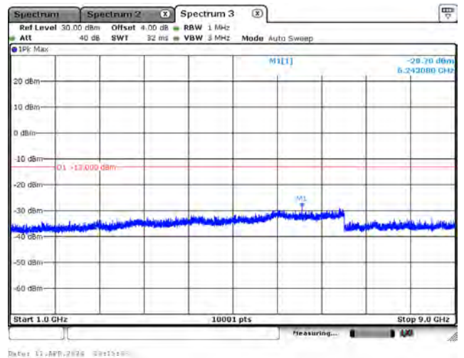
CH26915_3M_QPSK_1RB0_Above 1G
