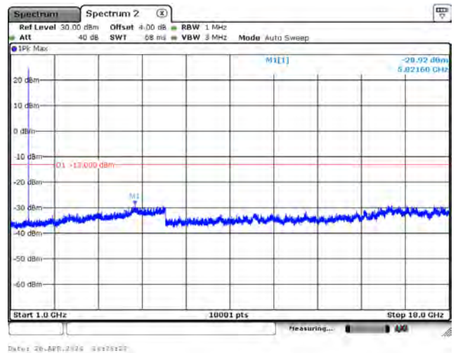
CH133047_15k_BPSK_1RB0_Above 1G
