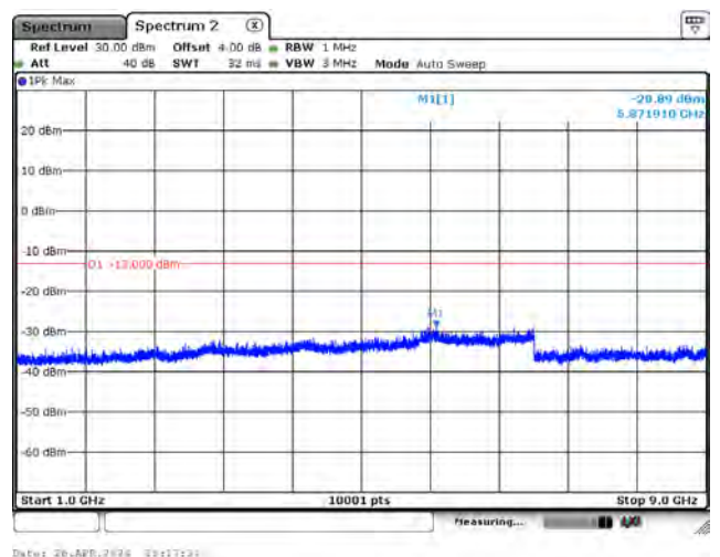
CH26788_15k_QPSK_1RB0_Above 1G
