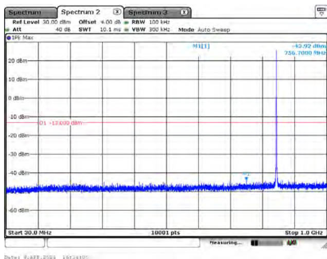
CH26965_15M_QPSK_1RB0_Below 1G
