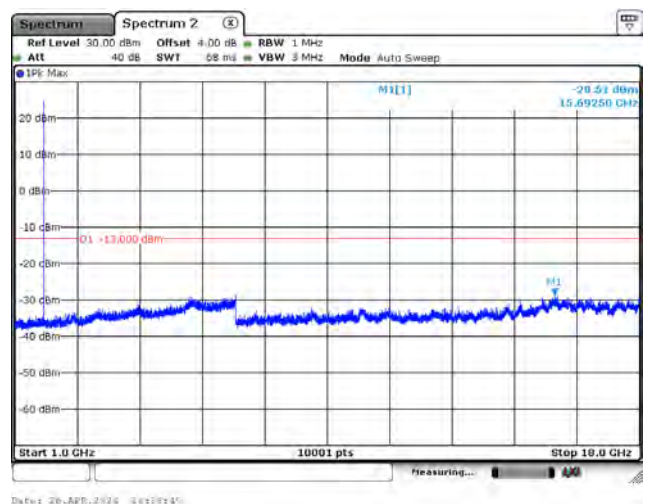
CH132670_15k_QPSK_1RB0_Above 1G
