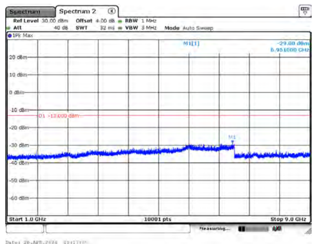
CH26788_15k_BPSK_1RB0_Above 1G
