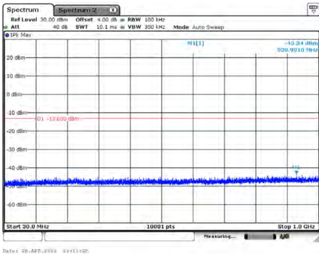
CH133047_3.75k_QPSK_1RB0_Below 1G
