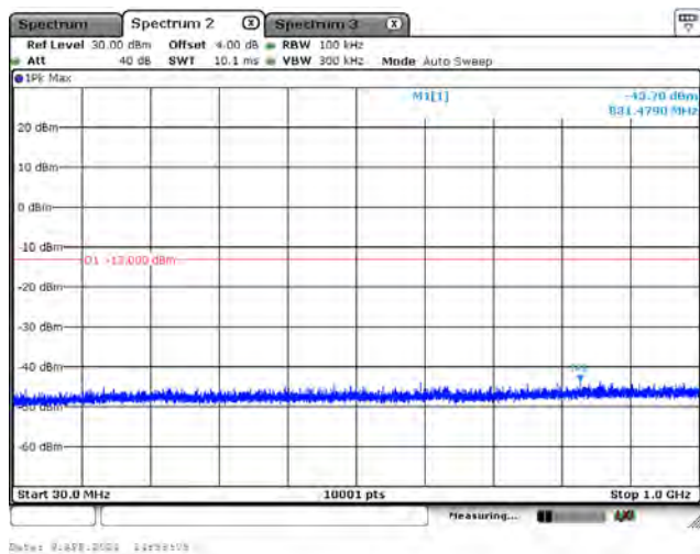
CH26615_15M_QPSK_1RB0_Below 1G
