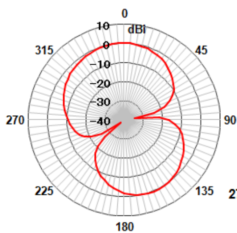
Horizontal Polarization
