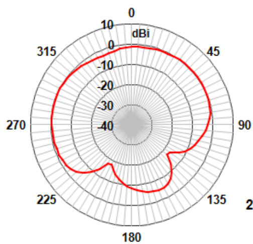
Horizontal Polarization
