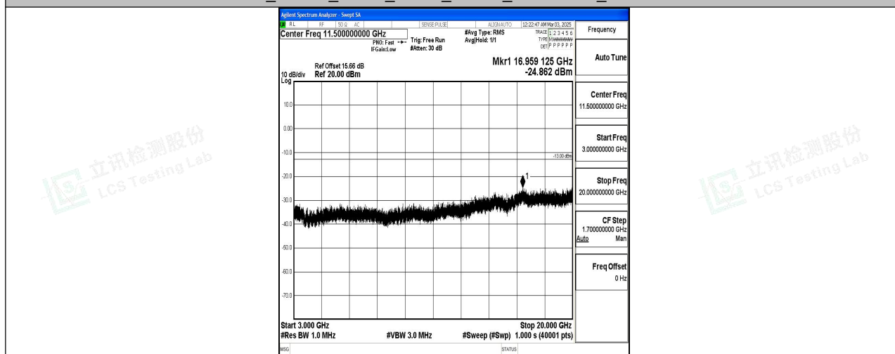
Band4_20MHz_QPSK_20300_1RB#0_3000~20000_3000~20000
