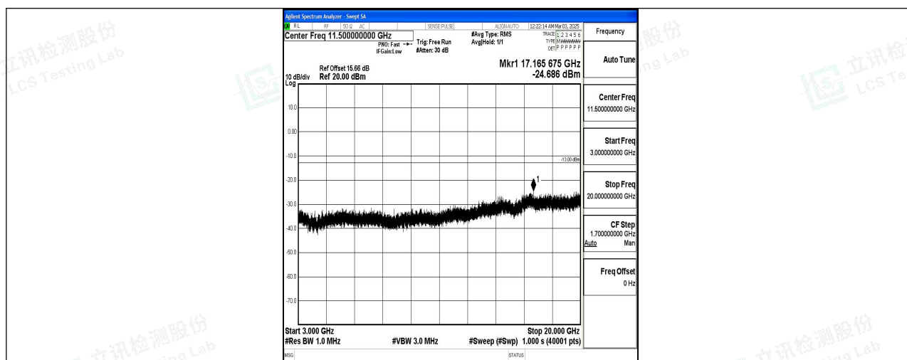
Band4 20MHz 16QAM 20175 1RB#0 3000~20000 3000~20000
