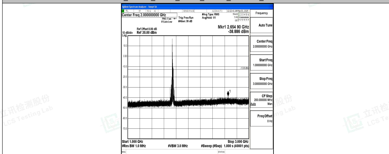
Band4_20MHz_QPSK_20300_1RB#0_1000~3000_1000~3000
