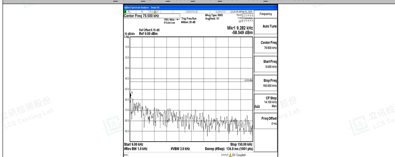
Band4 20MHz 16QAM 20050 1RB#0 0.009~0.15 0.009~0.15
