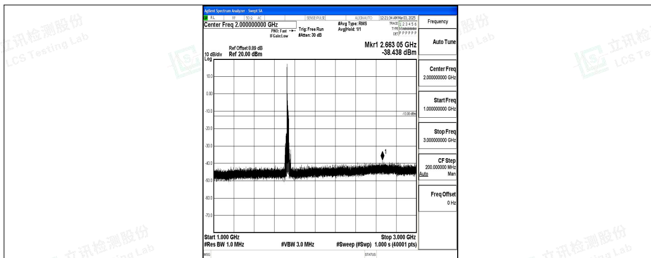
Band4_20MHz_QPSK_20175_1RB#0_1000~3000_1000~3000
