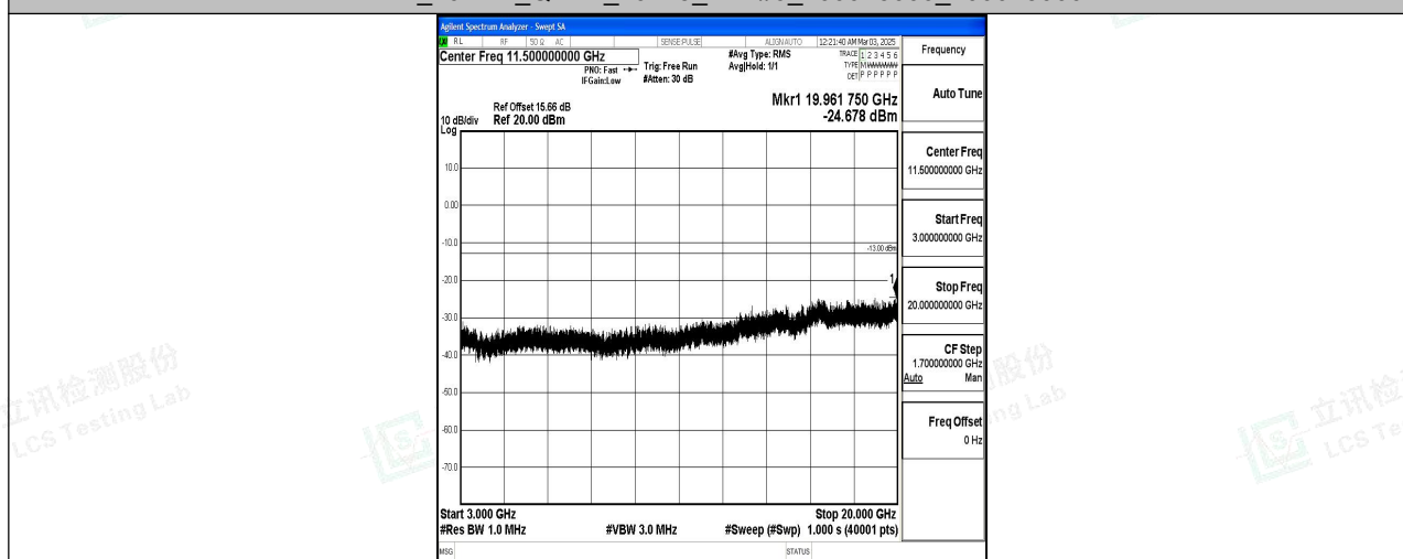
Band4_20MHz_QPSK_20175_1RB#0_3000~20000_3000~20000
