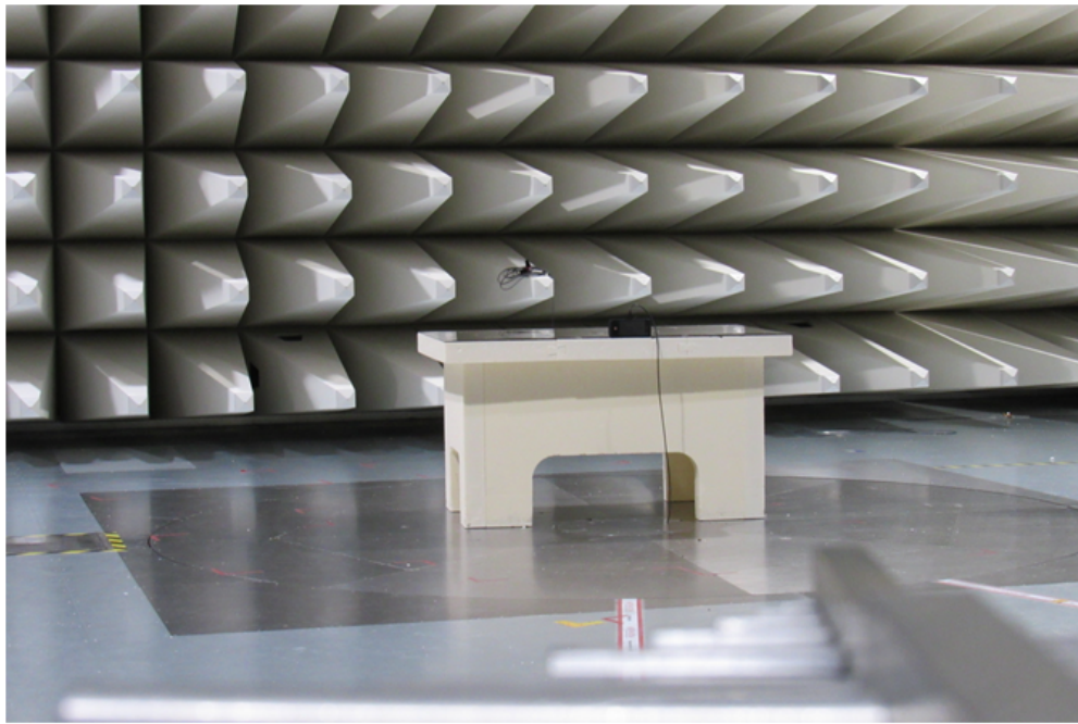
TEST SETUP (A)
