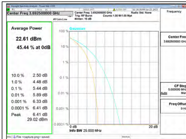
Band48 / 15MHz / High CH / QPSK
