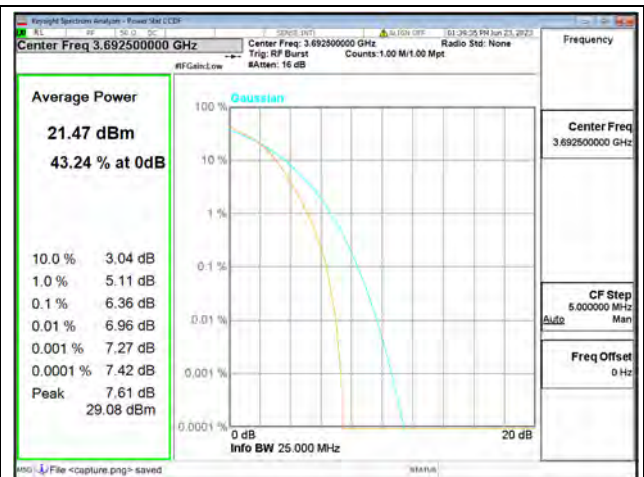
Band48 / 15MHz / High CH / 16QAM
