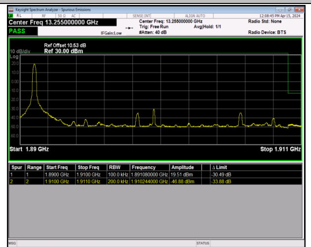
Band2_20MHz_QPSK_19100_1RB#0
