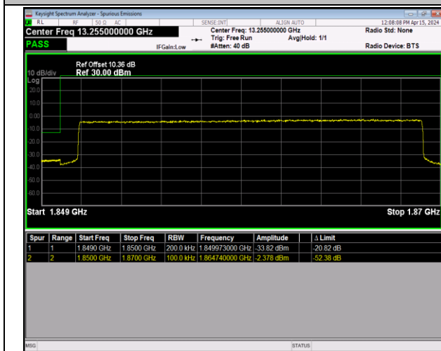
Band2_20MHz_QPSK_18700_100RB#0
