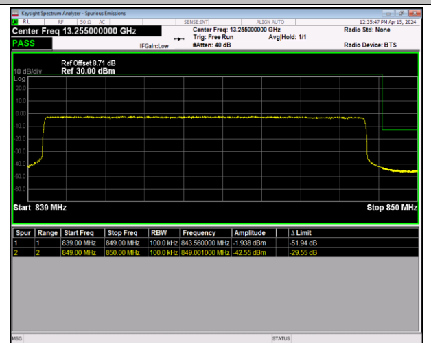
Band5_10MHz_64QAM_20600_50RB#0
