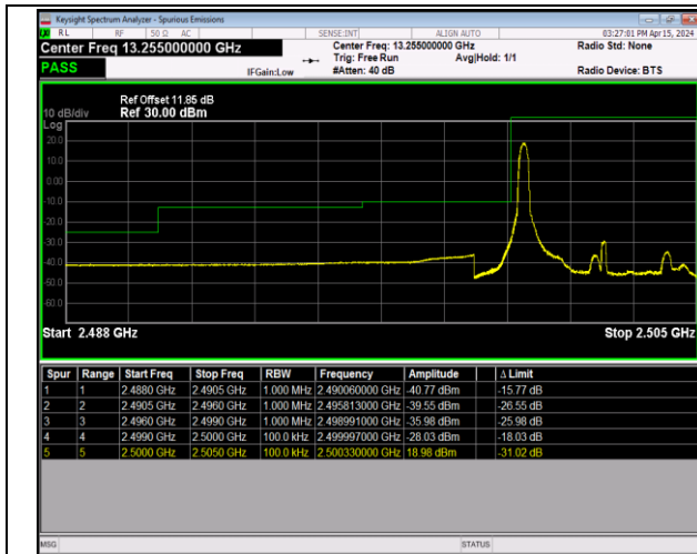
Band7_5MHz_QPSK_20775_1RB#0
