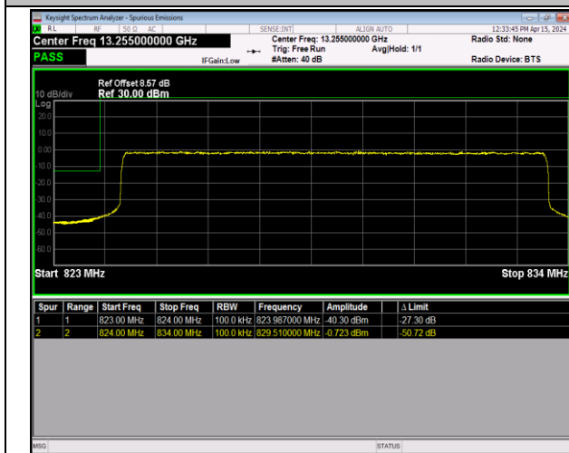
Band5_10MHz_16QAM_20450_50RB#0
