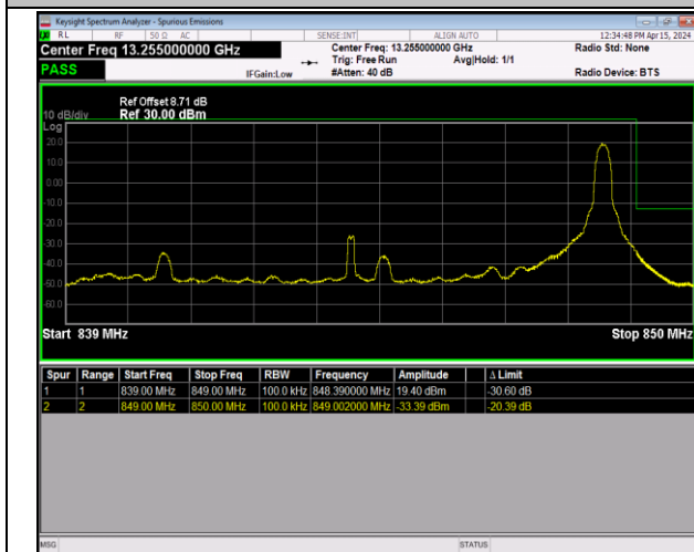
Band5_10MHz_QPSK_20600_1RB#49
