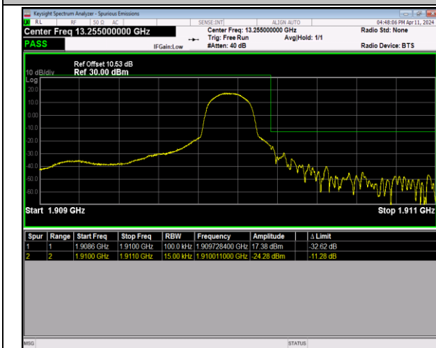
Band2_1.4MHz_64QAM_19193_1RB#5
