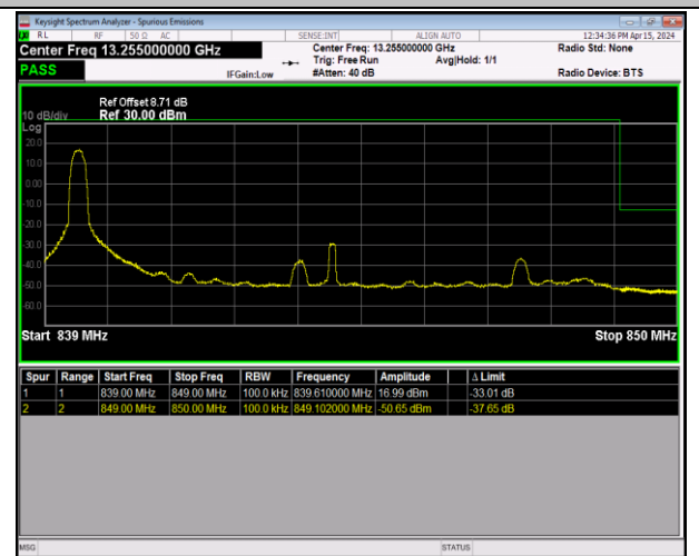
Band5_10MHz_64QAM_20600_1RB#0
