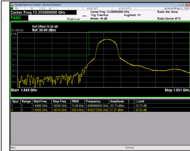
Band2_1.4MHz_64QAM_18607_1RB#0
