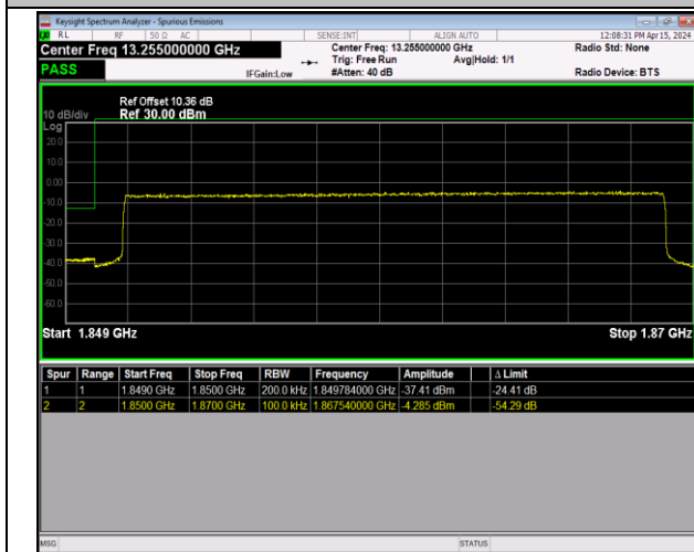
Band2_20MHz_64QAM_18700_100RB#0
