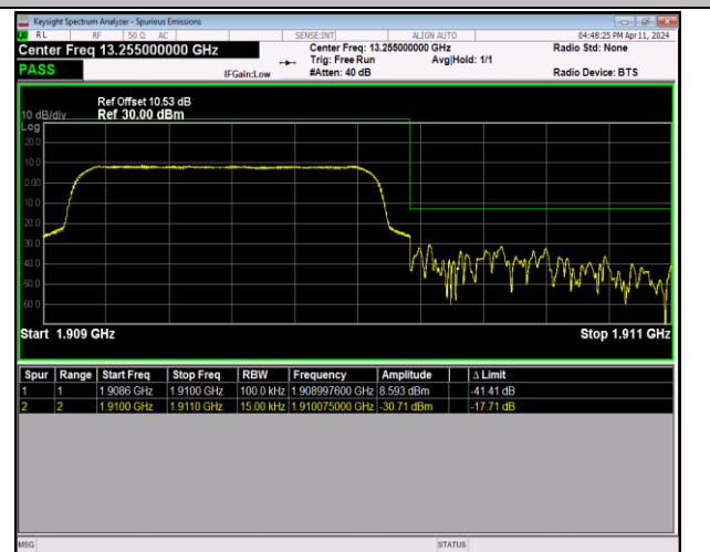
Band2_1.4MHz_16QAM_19193_6RB#0
