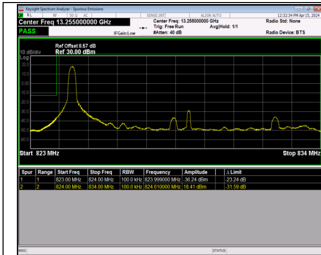
Band5_10MHz_16QAM_20450_1RB#0
