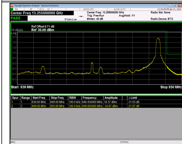
Band5_10MHz_16QAM_20600_1RB#49
