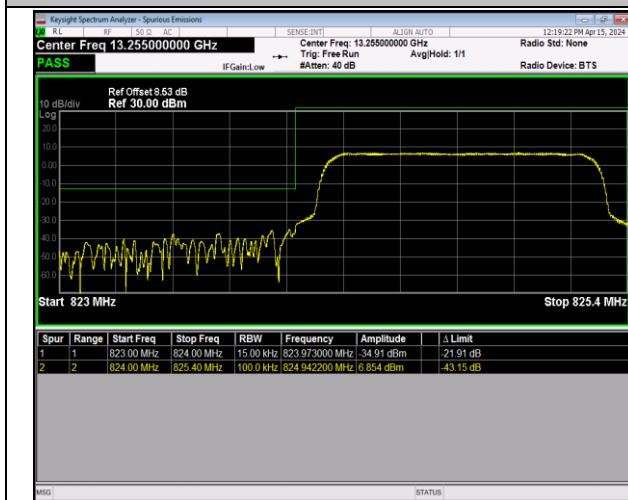
Band5_1.4MHz_64QAM_20407_6RB#0
