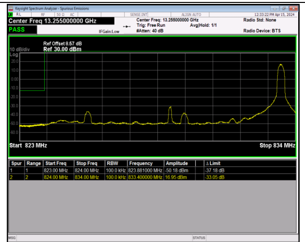
Band5_10MHz_64QAM_20450_1RB#49
