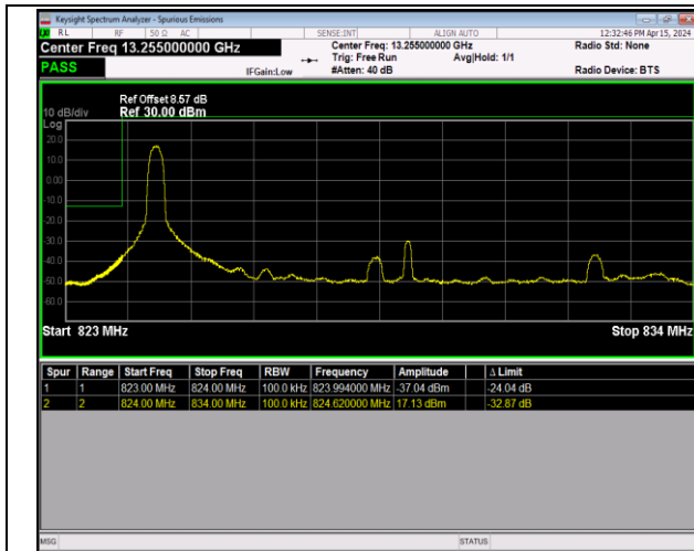
Band5_10MHz_64QAM_20450_1RB#0
