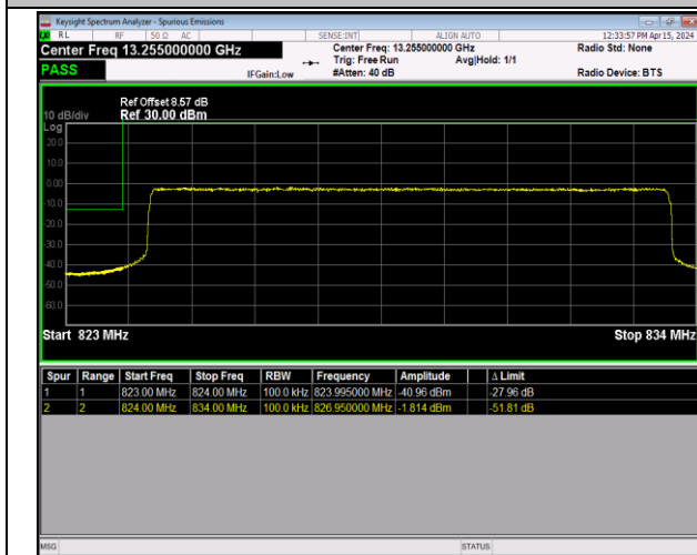
Band5_10MHz_64QAM_20450_50RB#0
