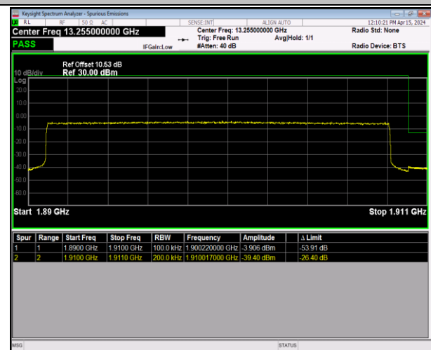
Band2_20MHz_64QAM_19100_100RB#0
