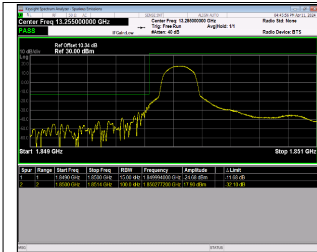
Band2_1.4MHz_16QAM_18607_1RB#0
