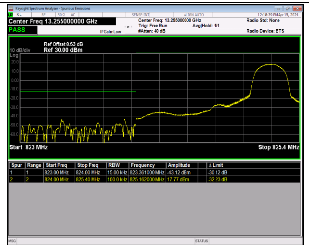
Band5_1.4MHz_16QAM_20407_1RB#5
