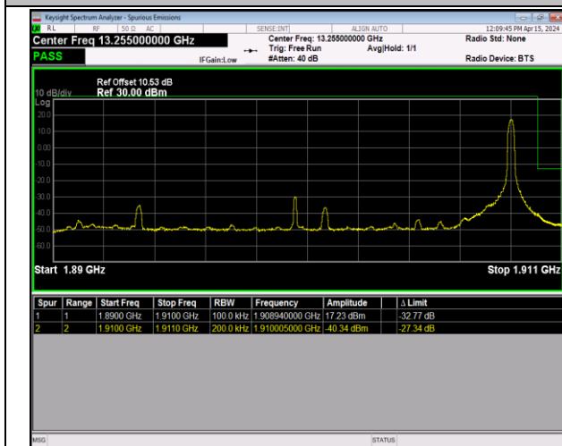
Band2_20MHz_64QAM_19100_1RB#99
