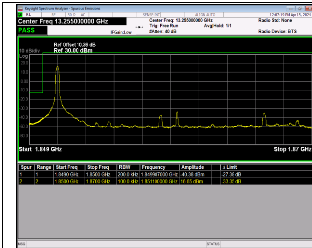
Band2_20MHz_64QAM_18700_1RB#0
