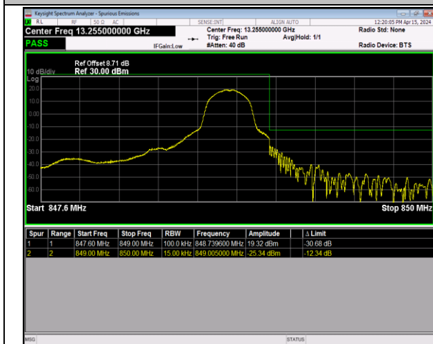
Band5_1.4MHz_QPSK_20643_1RB#5
