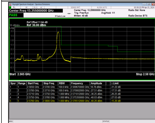
Band7_5MHz_16QAM_21425_1RB#24
