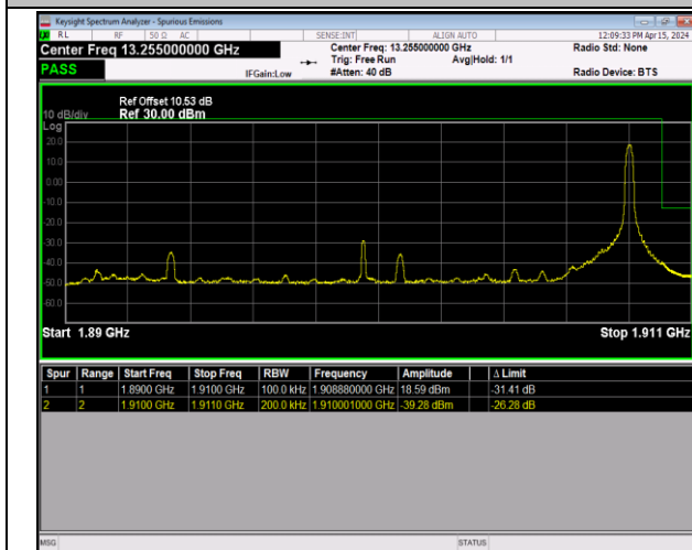
Band2_20MHz_16QAM_19100_1RB#99
