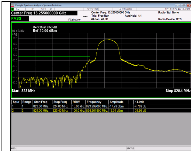
Band5_1.4MHz_16QAM_20407_1RB#0
