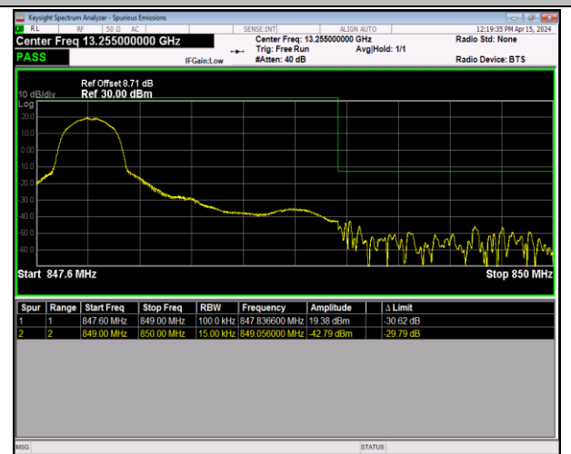
Band5_1.4MHz_QPSK_20643_1RB#0
