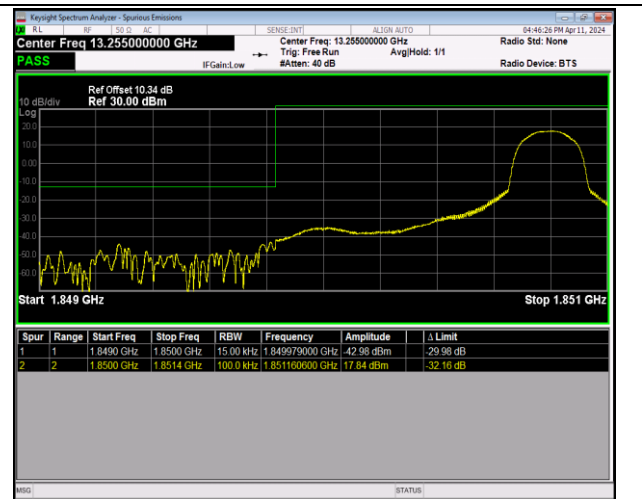
Band2_1.4MHz_16QAM_18607_1RB#5
