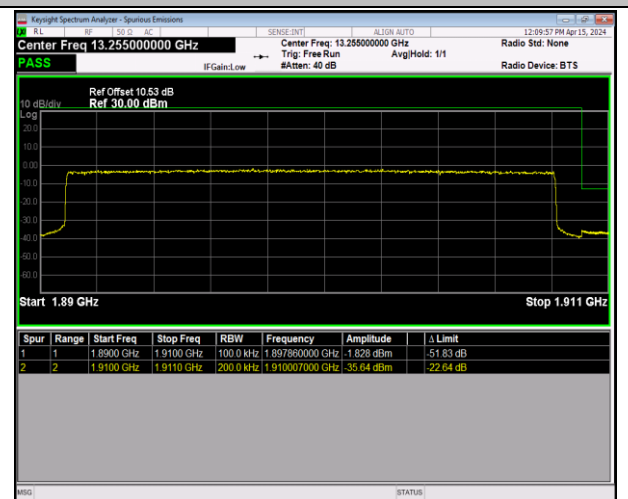
Band2_20MHz_QPSK_19100_100RB#0
