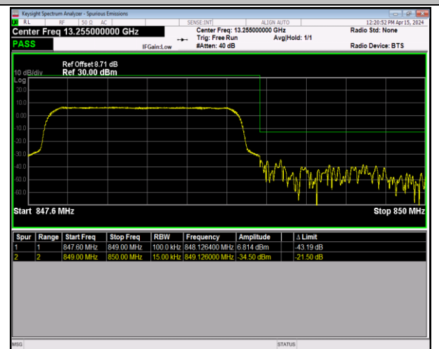
Band5_1.4MHz_64QAM_20643_6RB#0
