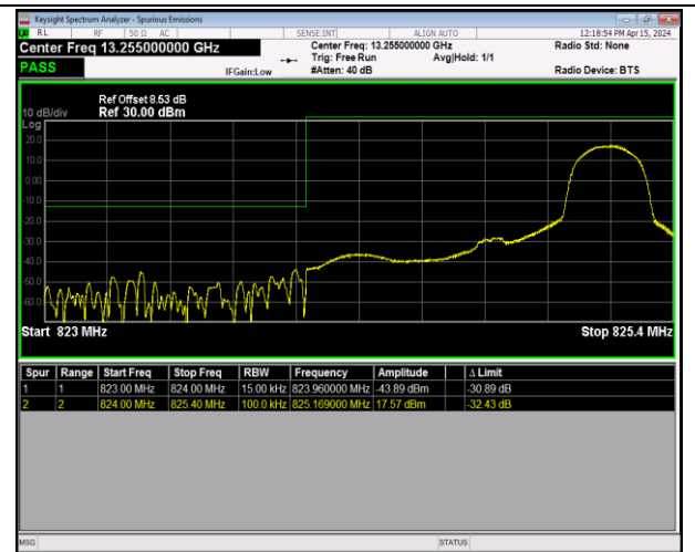
Band5_1.4MHz_64QAM_20407_1RB#5
