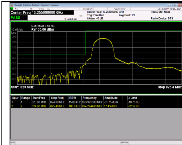
Band5_1.4MHz_64QAM_20407_1RB#0
