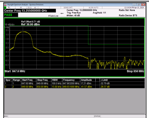
Band5_1.4MHz_64QAM_20643_1RB#0
