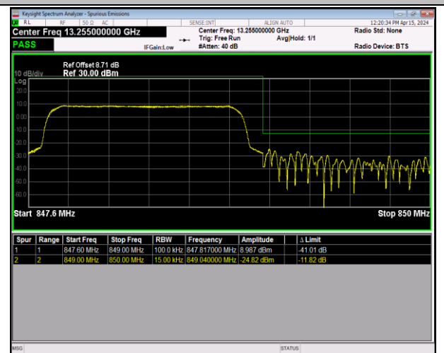
Band5_1.4MHz_QPSK_20643_6RB#0
