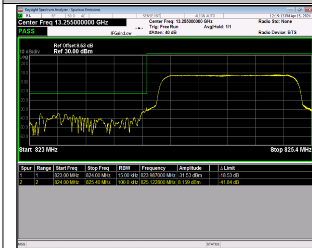
Band5_1.4MHz_16QAM_20407_6RB#0
