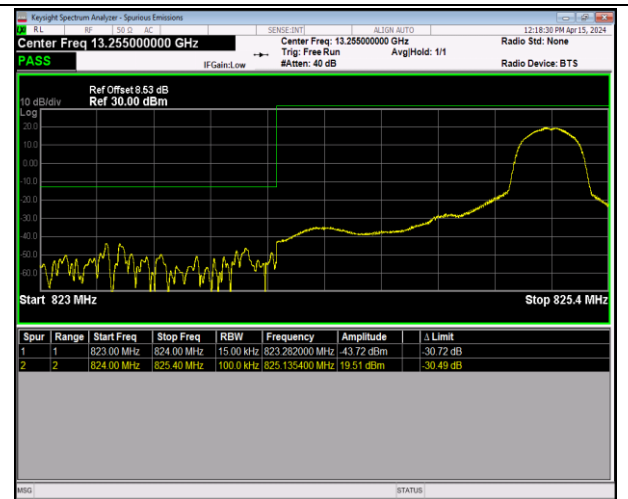
Band5_1.4MHz_QPSK_20407_1RB#5
