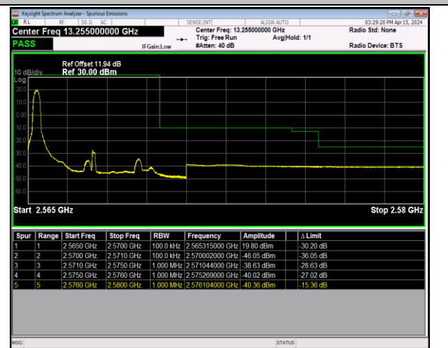
Band7_5MHz_QPSK_21425_1RB#0
