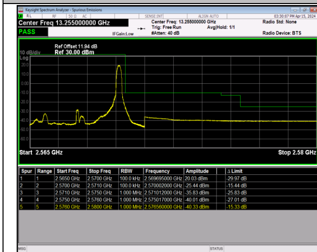
Band7_5MHz_QPSK_21425_1RB#24
