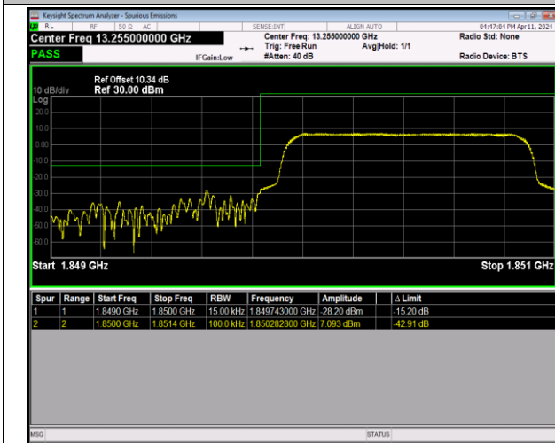
Band2_1.4MHz_64QAM_18607_6RB#0
