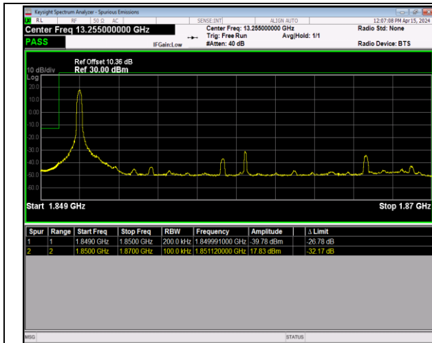
Band2_20MHz_16QAM_18700_1RB#0
