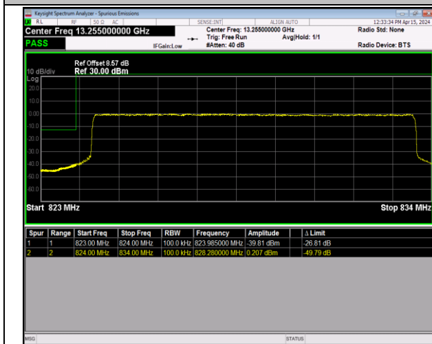
Band5_10MHz_QPSK_20450_50RB#0
