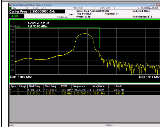
Band2_1.4MHz_16QAM_19193_1RB#5
