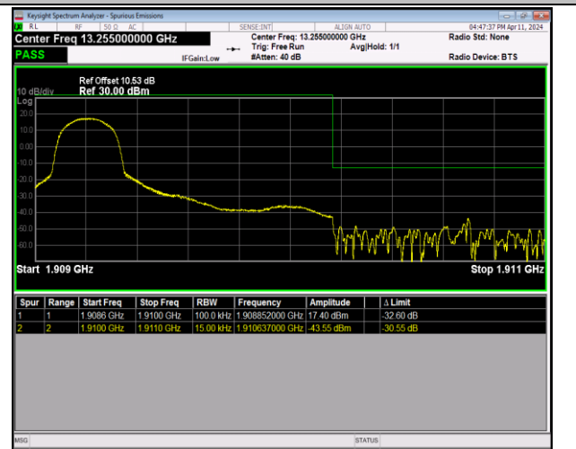
Band2_1.4MHz_64QAM_19193_1RB#0
