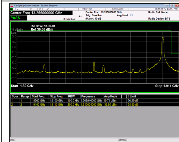
Band2_20MHz_QPSK_19100_1RB#99
