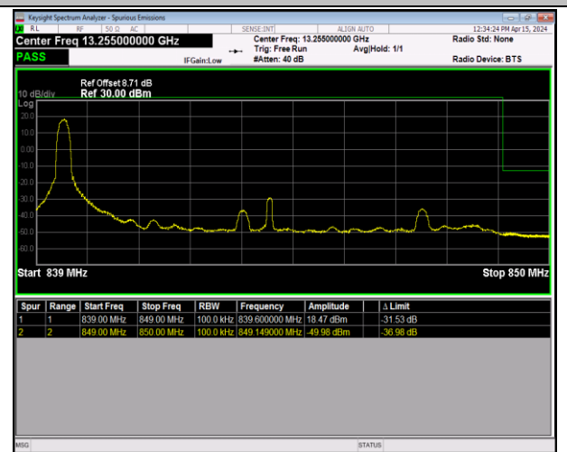
Band5_10MHz_16QAM_20600_1RB#0
