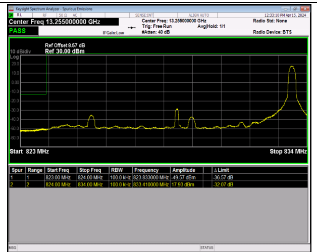
Band5_10MHz_16QAM_20450_1RB#49
