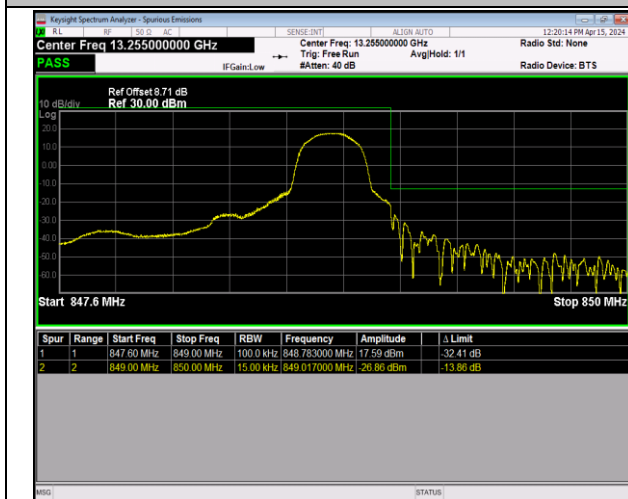
Band5_1.4MHz_16QAM_20643_1RB#5
