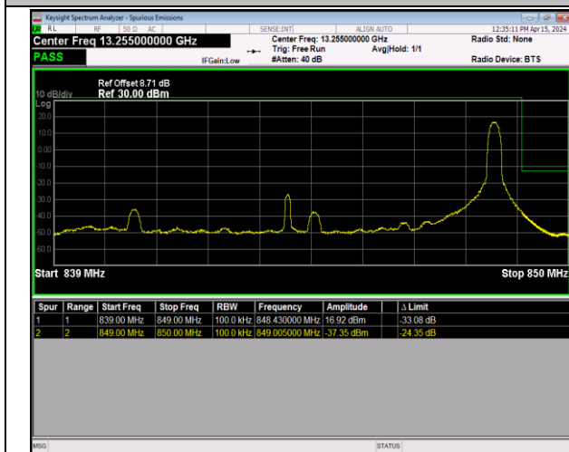
Band5_10MHz_64QAM_20600_1RB#49
