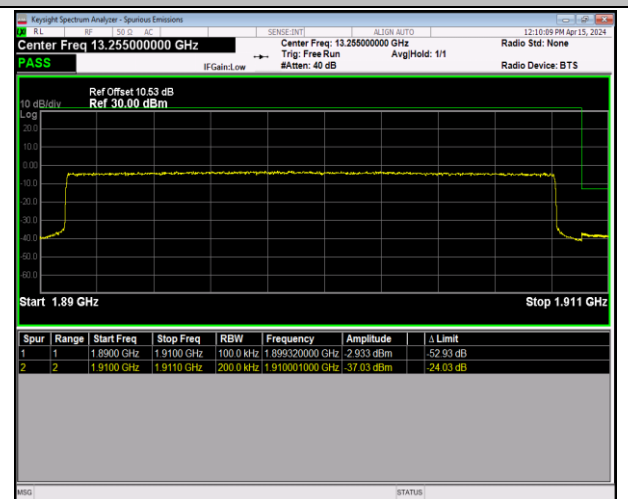
Band2_20MHz_16QAM_19100_100RB#0
