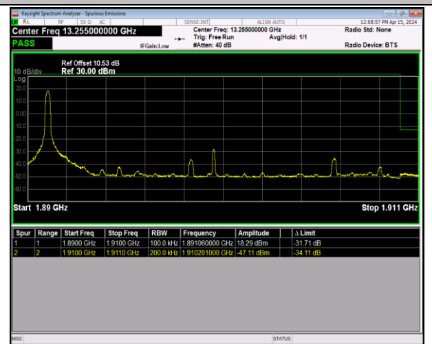
Band2_20MHz_16QAM_19100_1RB#0
