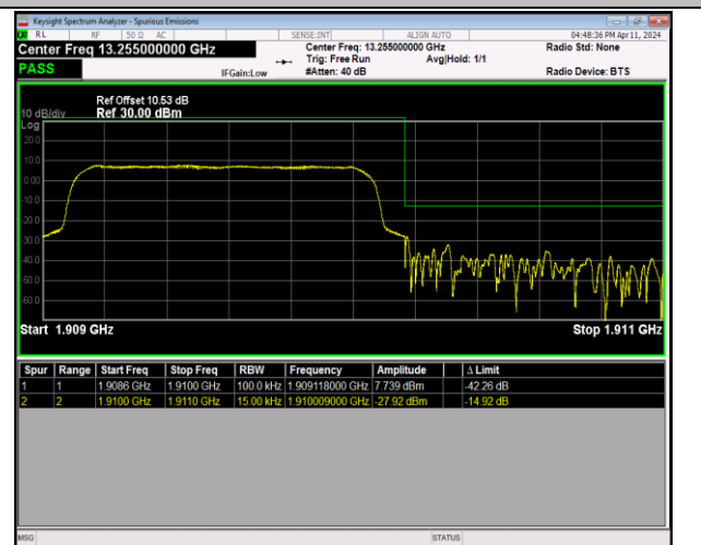
Band2_1.4MHz_64QAM_19193_6RB#0
