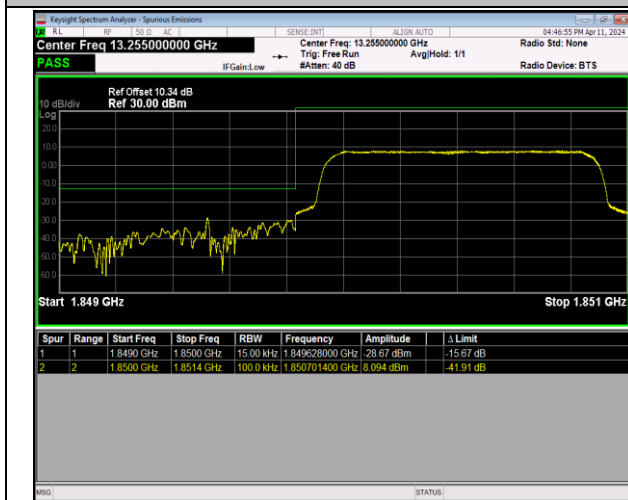
Band2_1.4MHz_16QAM_18607_6RB#0
