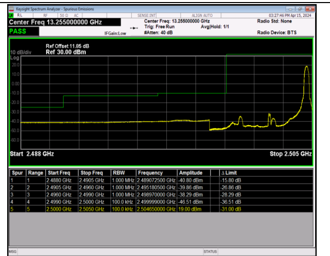
Band7_5MHz_QPSK_20775_1RB#24
