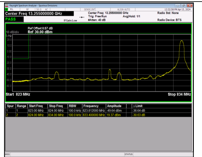
Band5_10MHz_QPSK_20450_1RB#49
