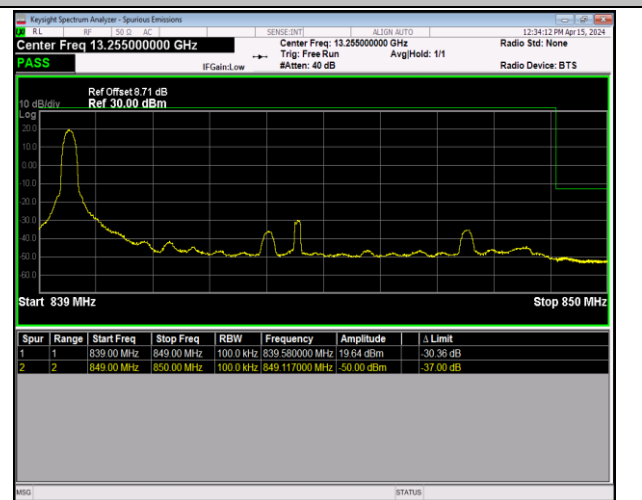
Band5_10MHz_QPSK_20600_1RB#0
