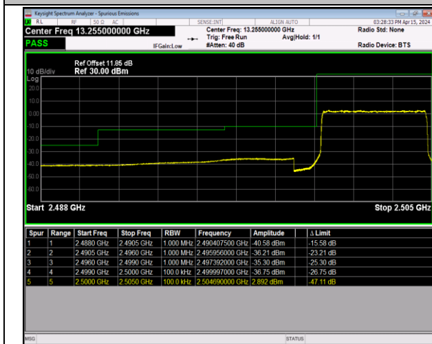
Band7_5MHz_QPSK_20775_25RB#0
