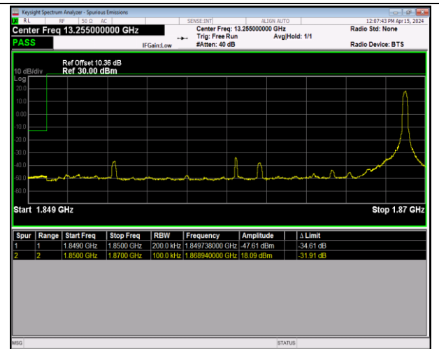
Band2_20MHz_16QAM_18700_1RB#99
