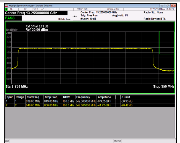
Band5_10MHz_16QAM_20600_50RB#0
