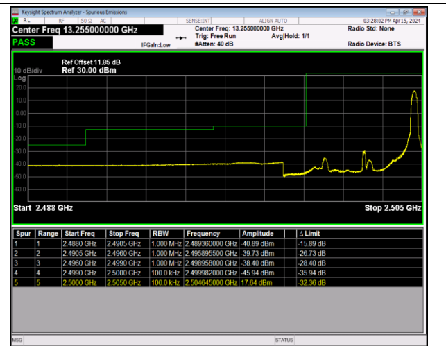
Band7_5MHz_16QAM_20775_1RB#24
