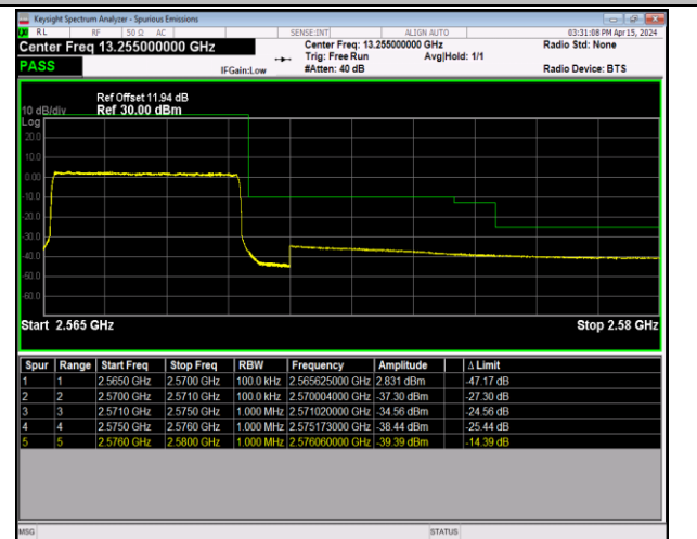
Band7_5MHz_16QAM_21425_25RB#0
