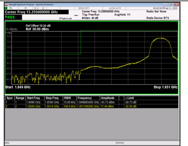
Band2_1.4MHz_64QAM_18607_1RB#5
