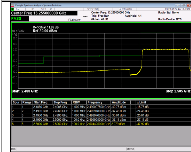
Band7_5MHz_16QAM_20775_25RB#0
