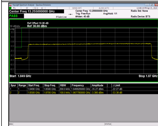
Band2_20MHz_16QAM_18700_100RB#0
