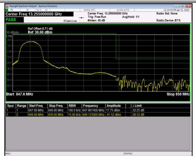
Band5_1.4MHz_16QAM_20643_1RB#0
