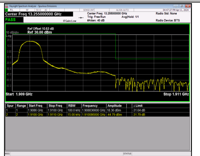
Band2_1.4MHz_16QAM_19193_1RB#0
