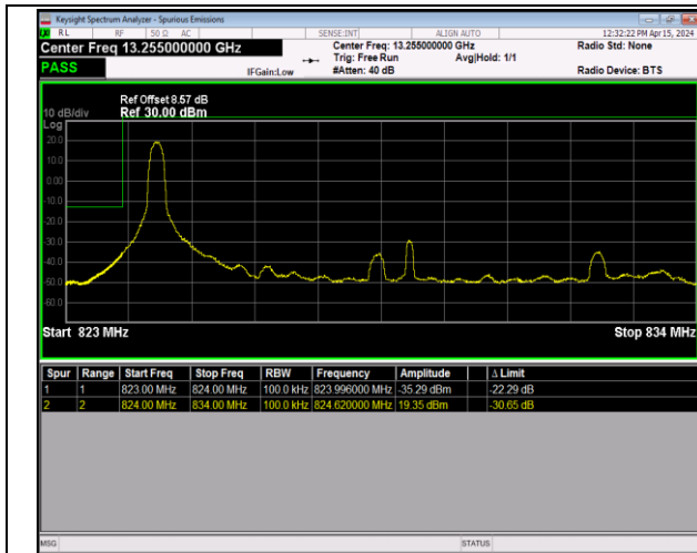
Band5_10MHz_QPSK_20450_1RB#0
