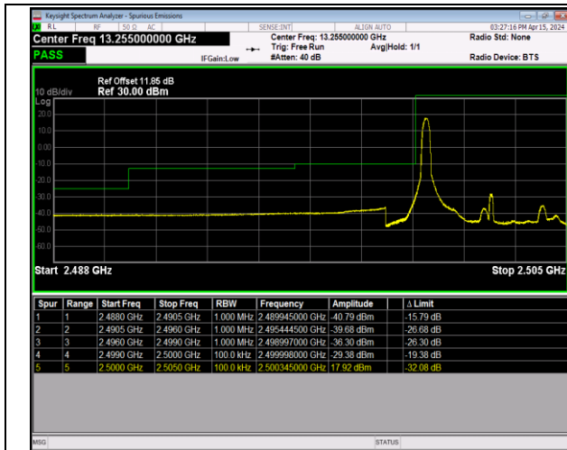
Band7_5MHz_16QAM_20775_1RB#0
