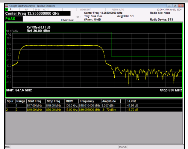
Band5_1.4MHz_16QAM_20643_6RB#0
