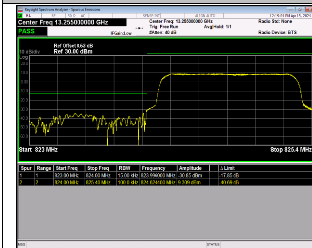
Band5_1.4MHz_QPSK_20407_6RB#0
