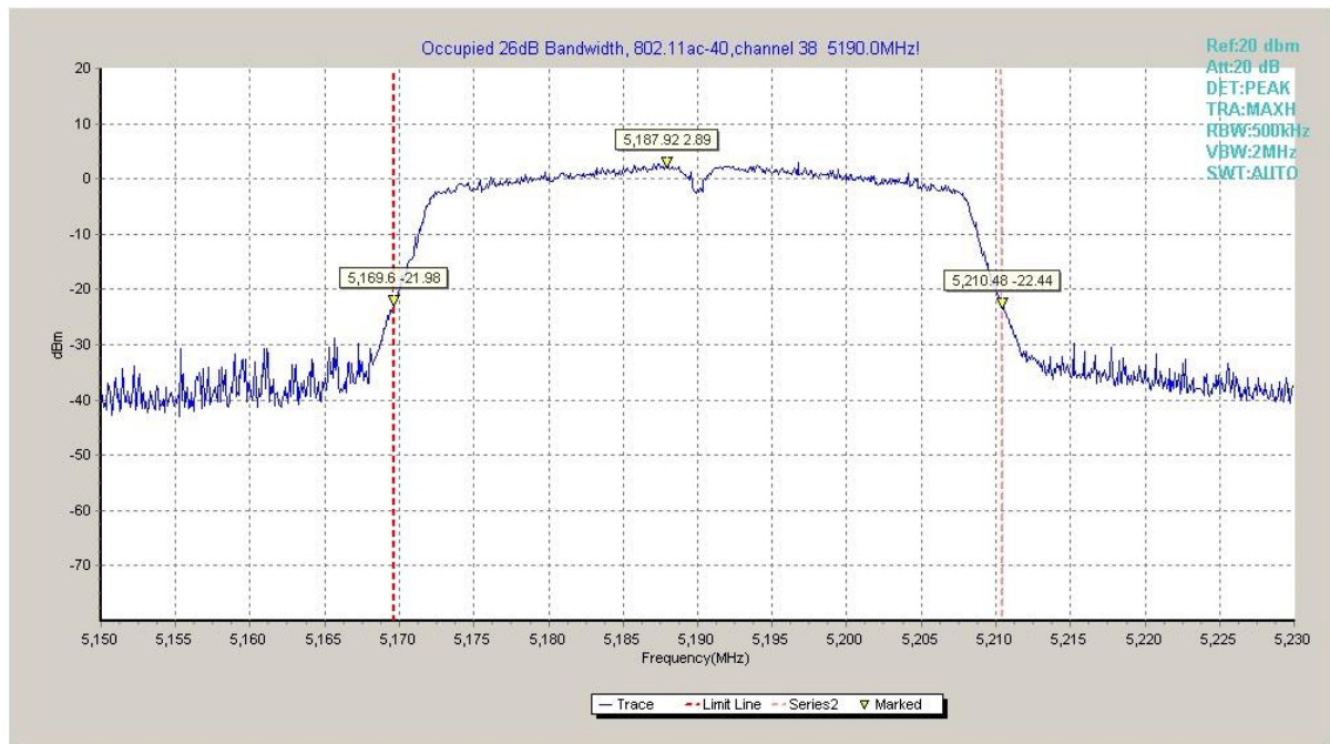
Fig. 39 Occupied 26dB Bandwidth (802.11ac40, 5190MHz)
