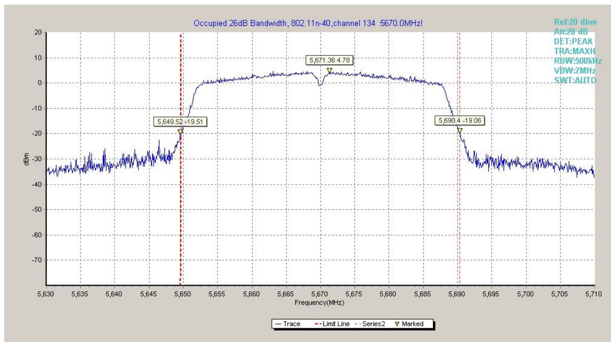
Fig. 37 Occupied 26dB Bandwidth (802.11n40, 5670MHz)
