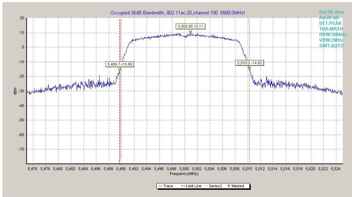
Fig. 27 Occupied 26dB Bandwidth (802.11ac20, 5500MHz)
