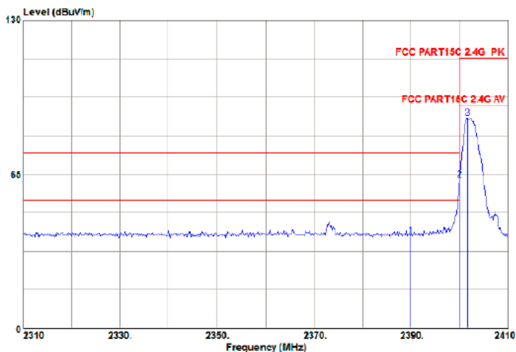
Left Band-Vertical-PK
