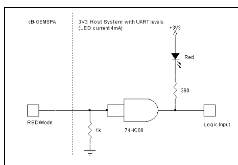
Figure 20: UART mode selected together with a red LED in a 3.3V host system. The status of the signal can also be used as input to a host controller.
