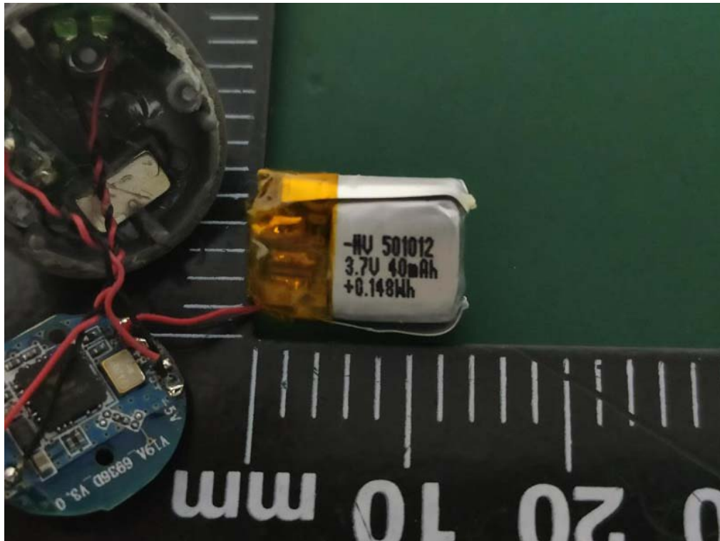
Internal Photos M/N: V19A
