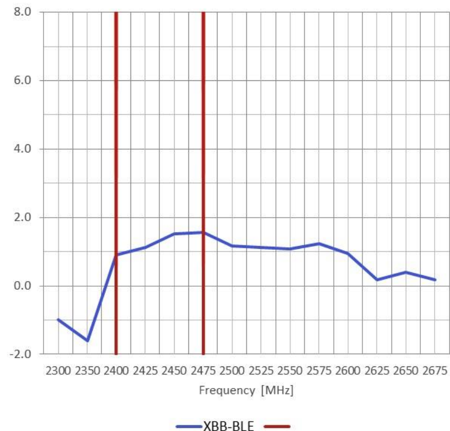
Peak Gain
