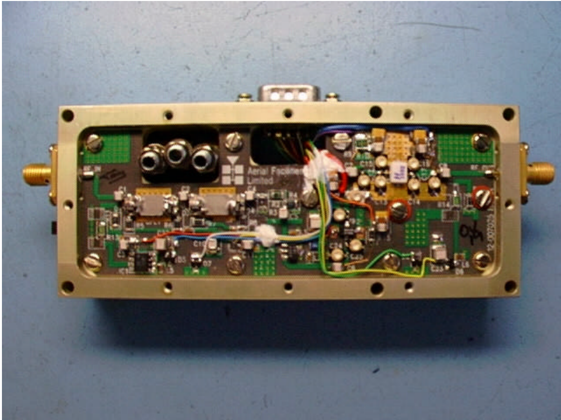
Photo 26 - Line Amp PA module bottom
