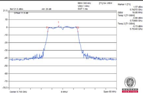
802.11n (HT20) / Chain 0 / CH 149
