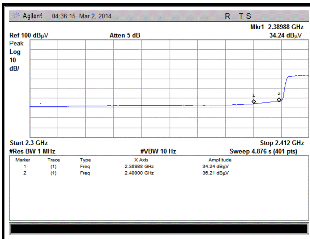
(Plot E2: Channel = 1 AVG @ 802.11n-20MHz)
