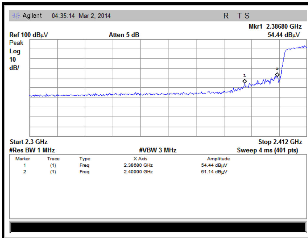
(Plot E1: Channel = 1 PEAK @ 802.11n-20MHz)
