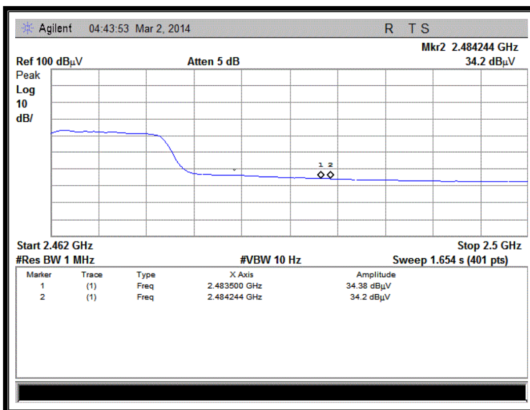
(Plot F2: Channel = 11 AVG @ 802.11n-20MHz)
