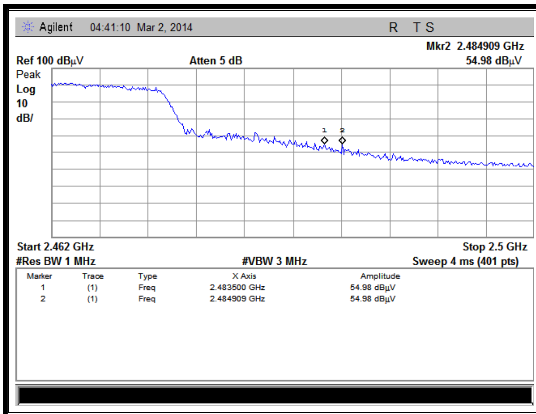
(Plot F1: Channel = 11 PEAK @ 802.11n-20MHz)
