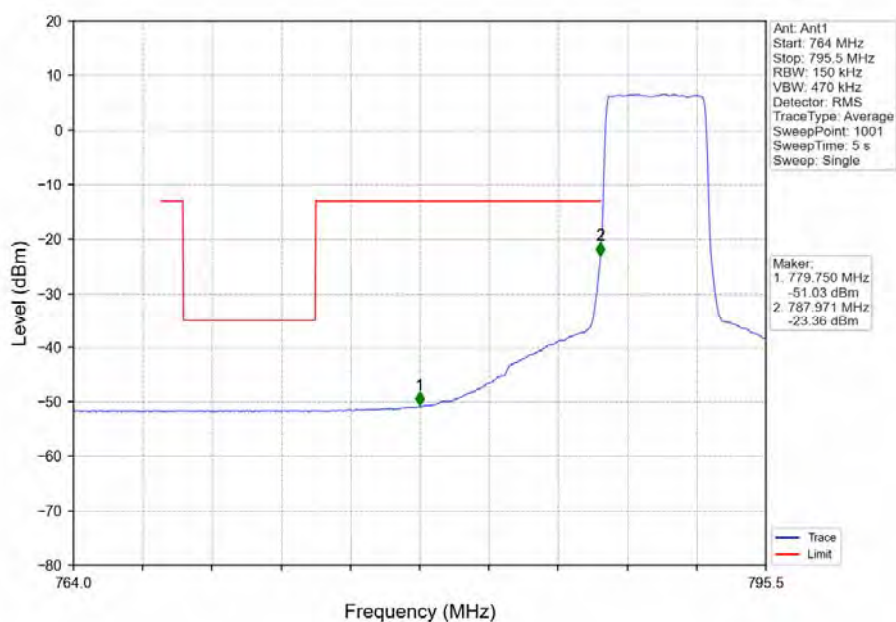
Band14_5MHz_16QAM_LCH_790.5MHz_RB_25_0_NTNV
