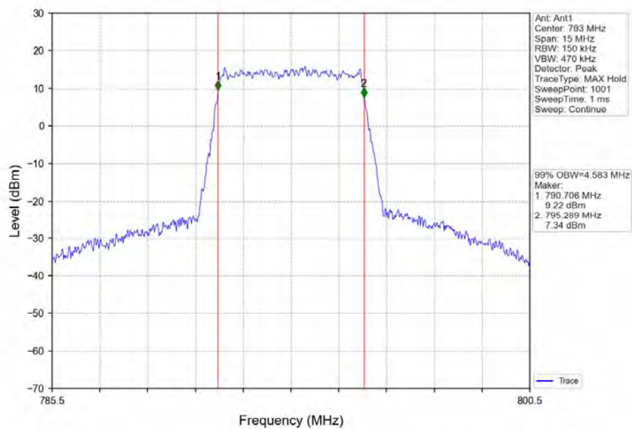
Band14_5MHz_64QAM_MCH_793MHz_RB_25_0_NTNV
