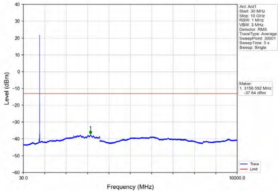
Band14_5MHz_16QAM_HCH_795.5MHz_RB_1_0_NTNV
