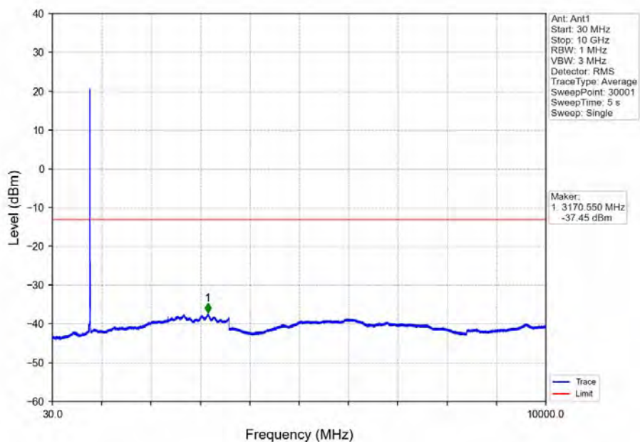
Band14_10MHz_64QAM_MCH_793MHz_RB_1_0_NTNV
