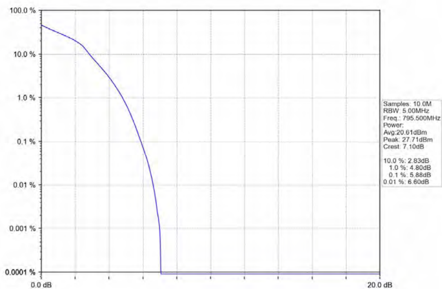
Band14_5MHz_16QAM_HCH_795.5MHz_RB_25_0_NTNV
