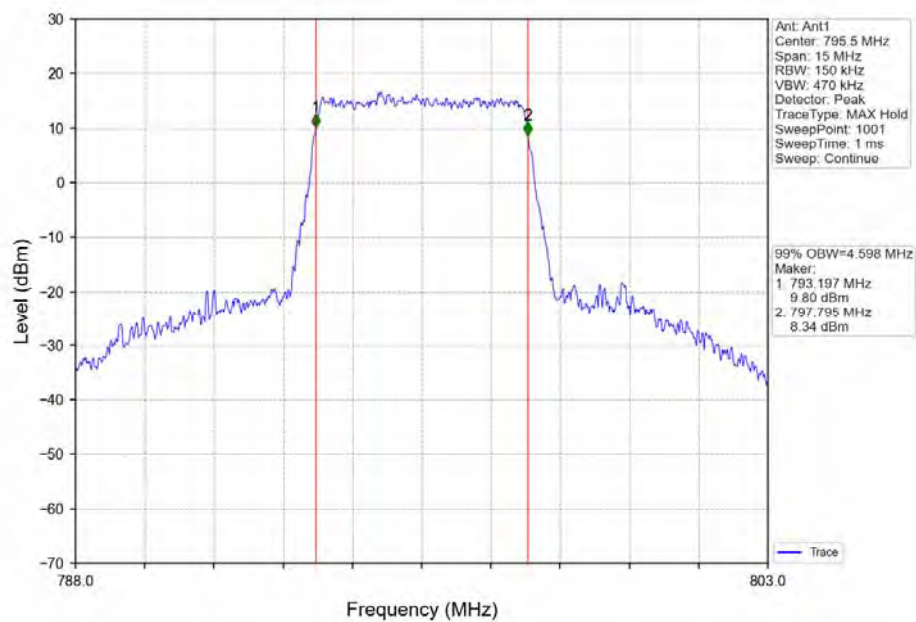
Band14_5MHz_16QAM_HCH_795.5MHz_RB_25_0_NTNV
