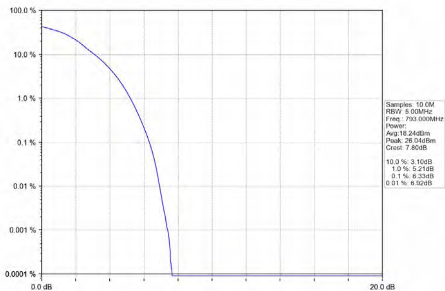
Band14_10MHz_64QAM_MCH_793MHz_RB_50_0_NTNV
