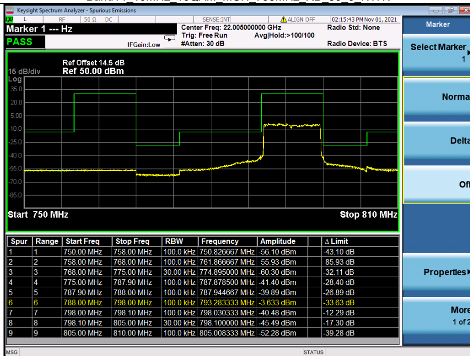
Band14_10MHz_16QAM_MCH_793MHz_RB_50_0_NTNV
