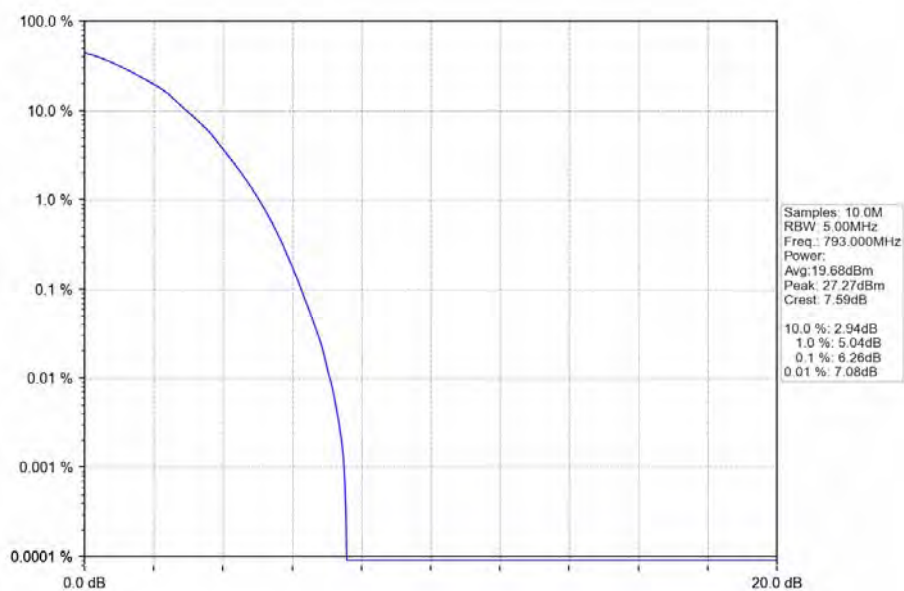
Band14_5MHz_64QAM_MCH_793MHz_RB_25_0_NTNV
