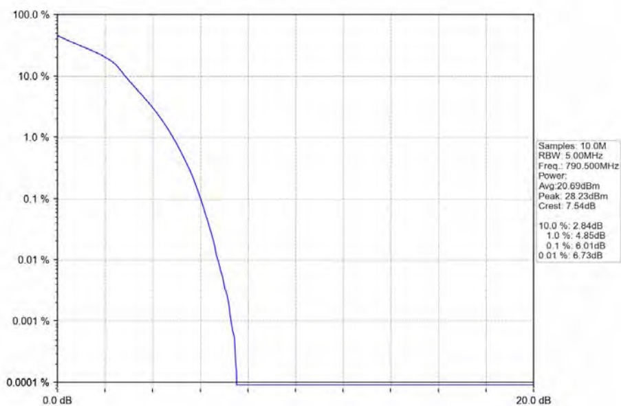
Band14_5MHz_16QAM_LCH_790.5MHz_RB_25_0_NTNV
