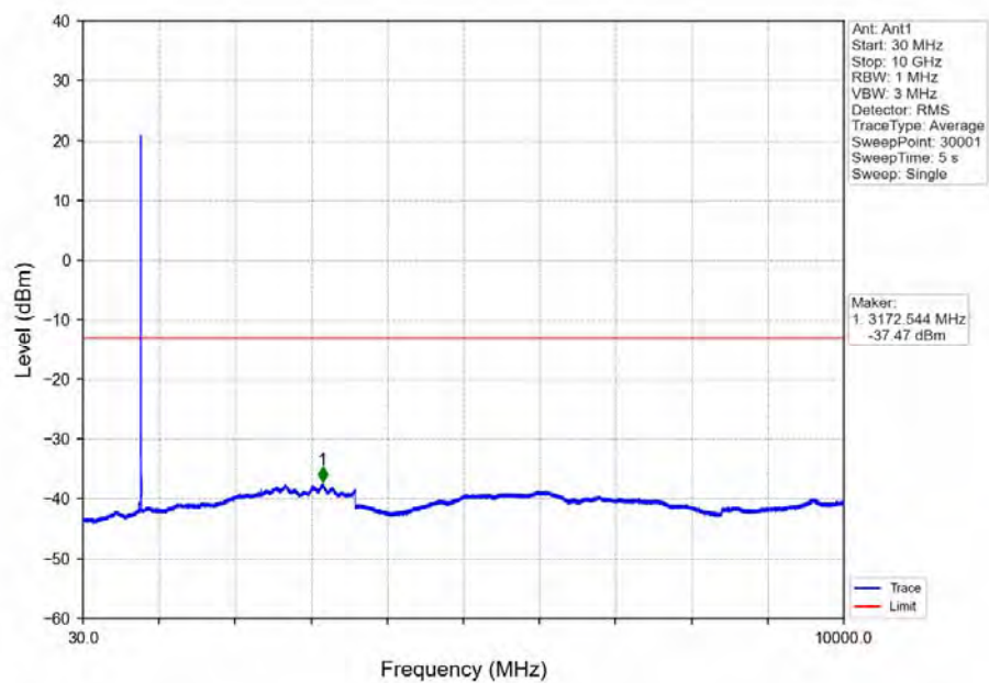
Band14_5MHz_64QAM_LCH_790.5MHz_RB_1_0_NTNV
