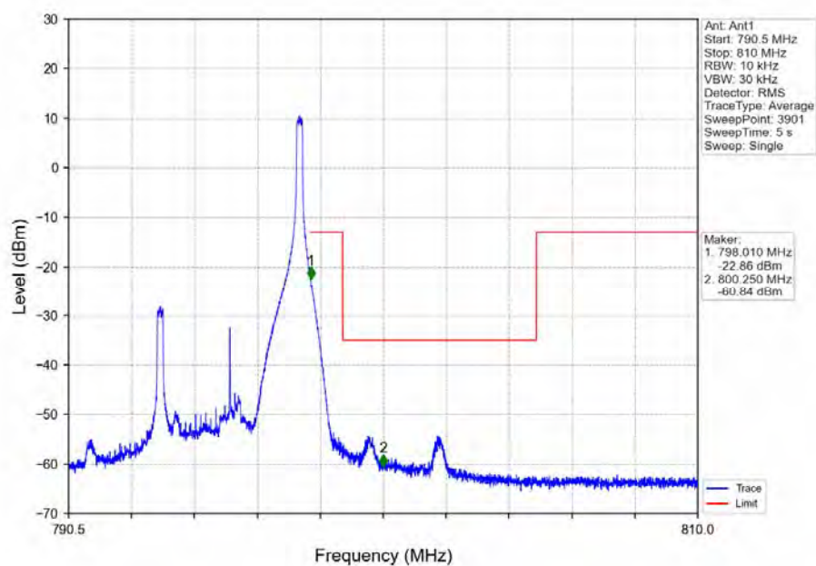
Band14_5MHz_16QAM_HCH_795.5MHz_RB_25_0_NTNV
