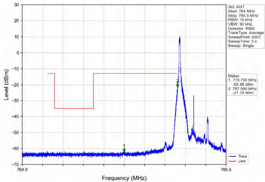
Band14_5MHz_64QAM_LCH_790.5MHz_RB_1_0_NTNV
