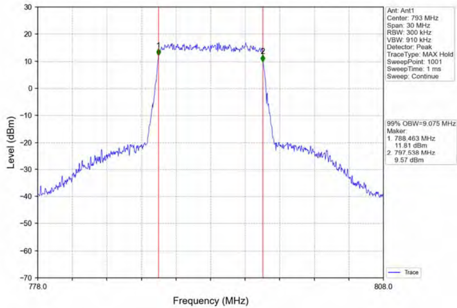
Band14_10MHz_64QAM_MCH_793MHz_RB_50_0_NTNV
