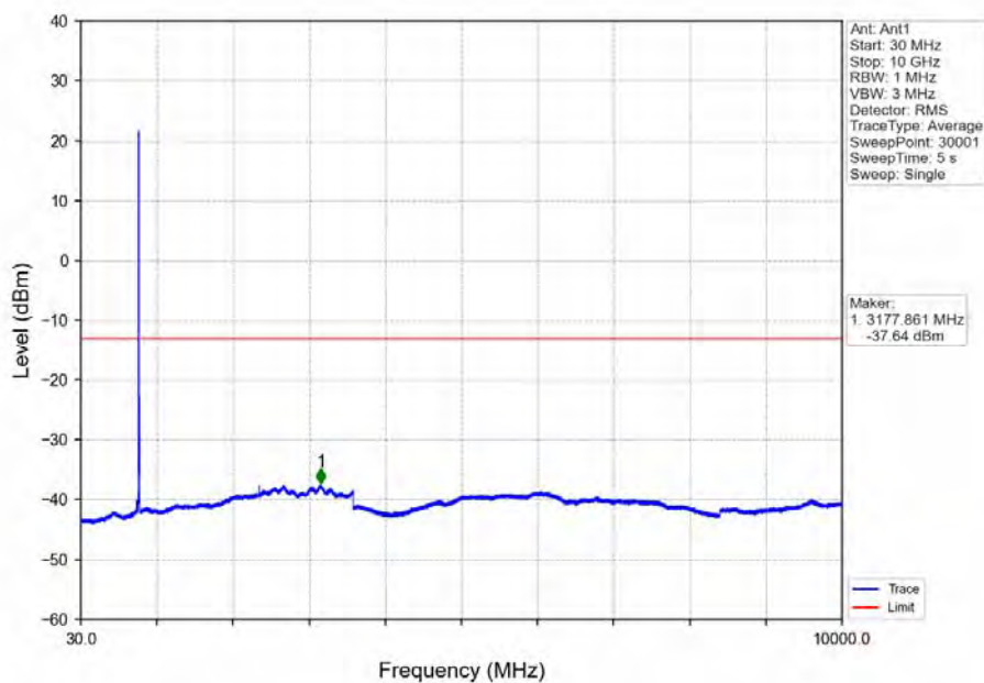
Band14_10MHz_16QAM_MCH_793MHz_RB_50_0_NTNV
