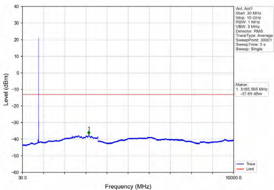
Band14_5MHz_64QAM_HCH_795.5MHz_RB_1_24_NTNV
