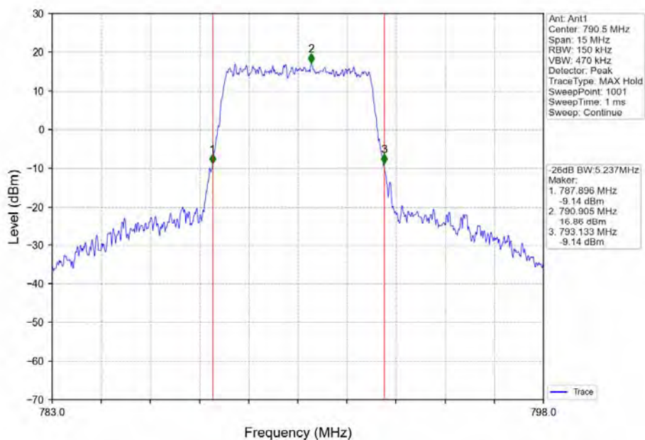
Band14_5MHz_16QAM_LCH_790.5MHz_RB_25_0_NTNV
