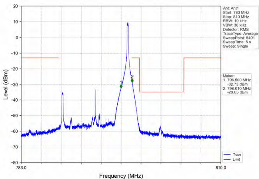
Band14_10MHz_64QAM_MCH_793MHz_RB_1_49_NTNV
