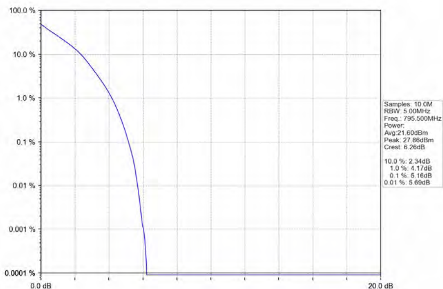
Band14_5MHz_QPSK_HCH_795.5MHz_RB_25_0_NTNV
