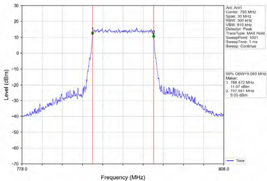
Band14_10MHz_64QAM_MCH_793MHz_RB_50_0_NTNV
