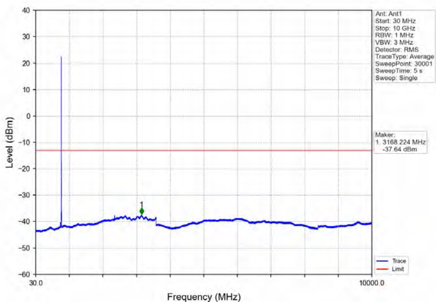
Band14_5MHz_QPSK_MCH_793MHz_RB_1_0_NTNV
