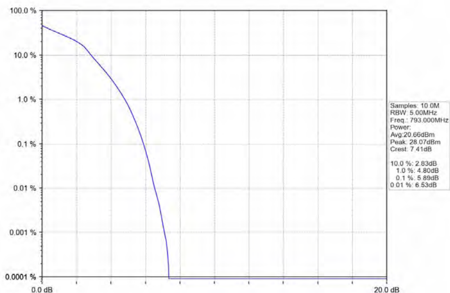
Band14_5MHz_16QAM_MCH_793MHz_RB_25_0_NTNV
