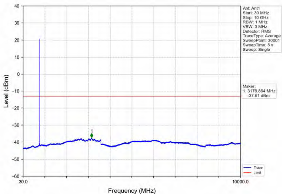
Band14_5MHz_64QAM_MCH_793MHz_RB_1_0_NTNV
