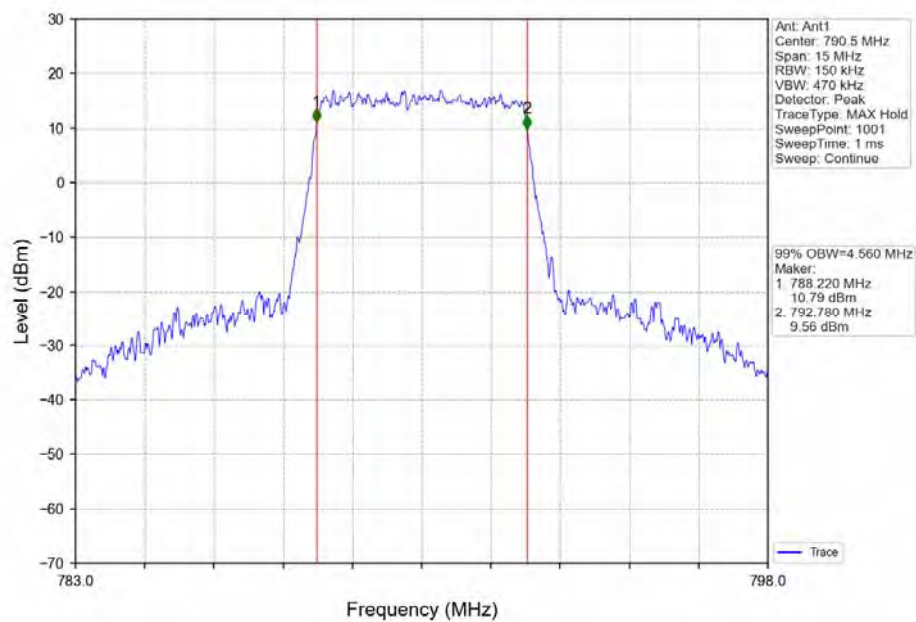
Band14_5MHz_16QAM_LCH_790.5MHz_RB_25_0_NTNV
