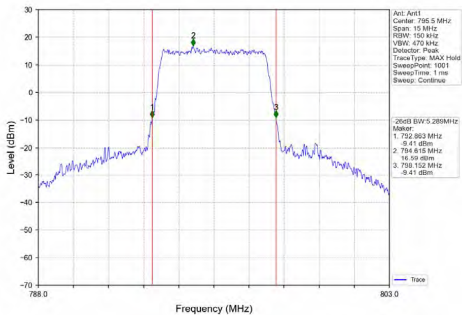
Band14_5MHz_16QAM_HCH_795.5MHz_RB_25_0_NTNV
