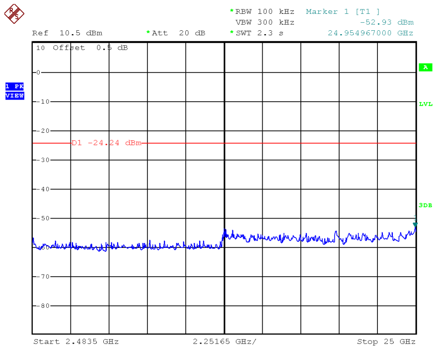
802.11g, Lowest Channel, Plot B
