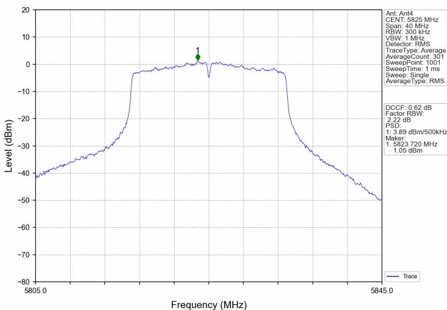
802.11ac(VHT20)_HCH_5825MHz_Ant4_NTNV
