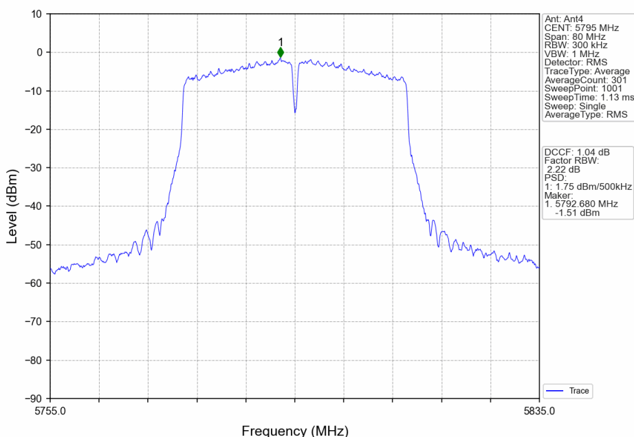
802.11ac(VHT40)_HCH_5795MHz_Ant4_NTNV
