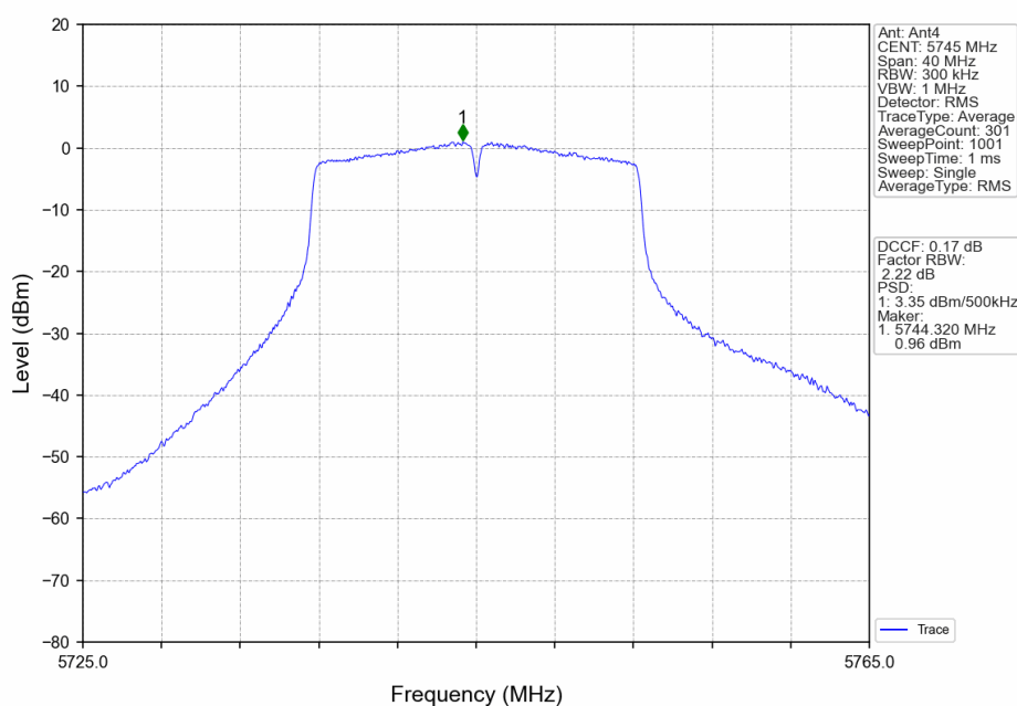
802.11a_LCH_5745MHz_Ant4_NTNV
