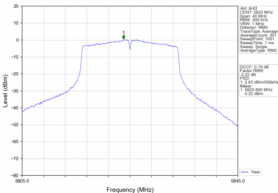
802.11n(HT20)_HCH_5825MHz_Ant3_NTNV
