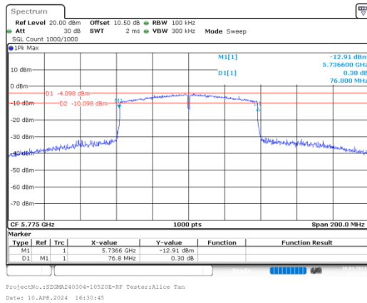
ac80_5775MHz_Chain 0
