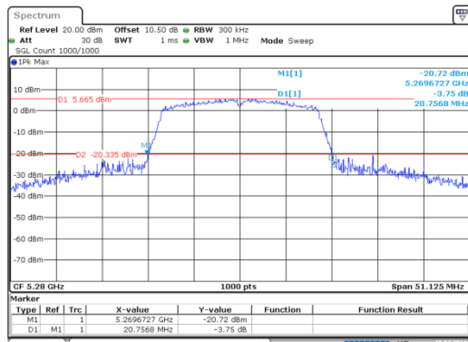
n20_5280MHz_Chain 0
