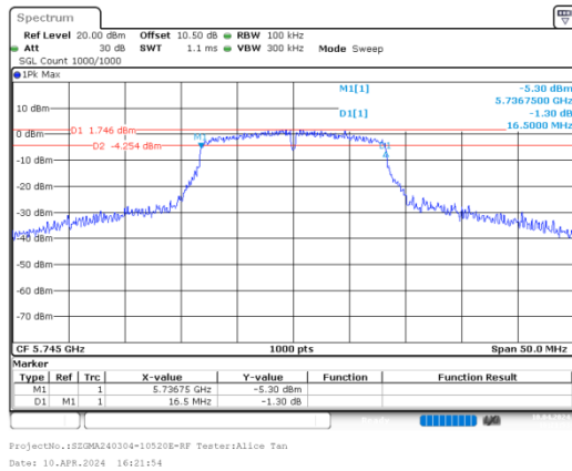
a_ 5745 MHz_Chain 0
