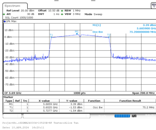
ac80_5690MHz_Chain 0
