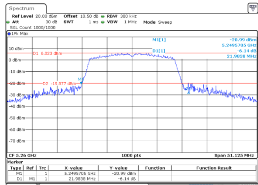
n20_5260MHz_Chain 0
