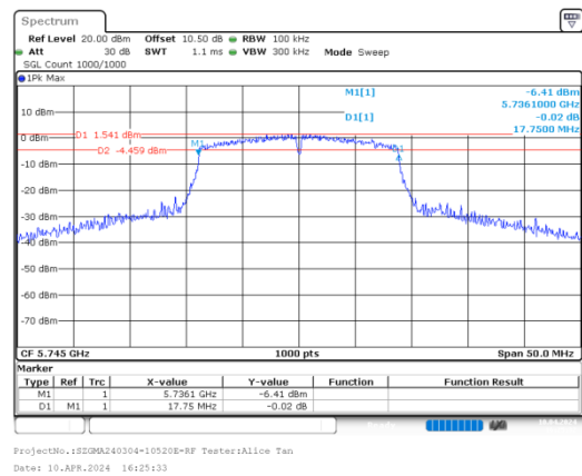
n20_ 5745MHz_Chain 0
